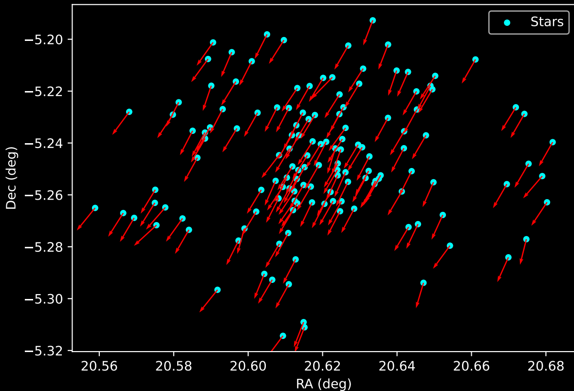
Gaia Cluster: [Deutsch_145] Proper Motion Vectors for Gaia Star Field (n= 138)
