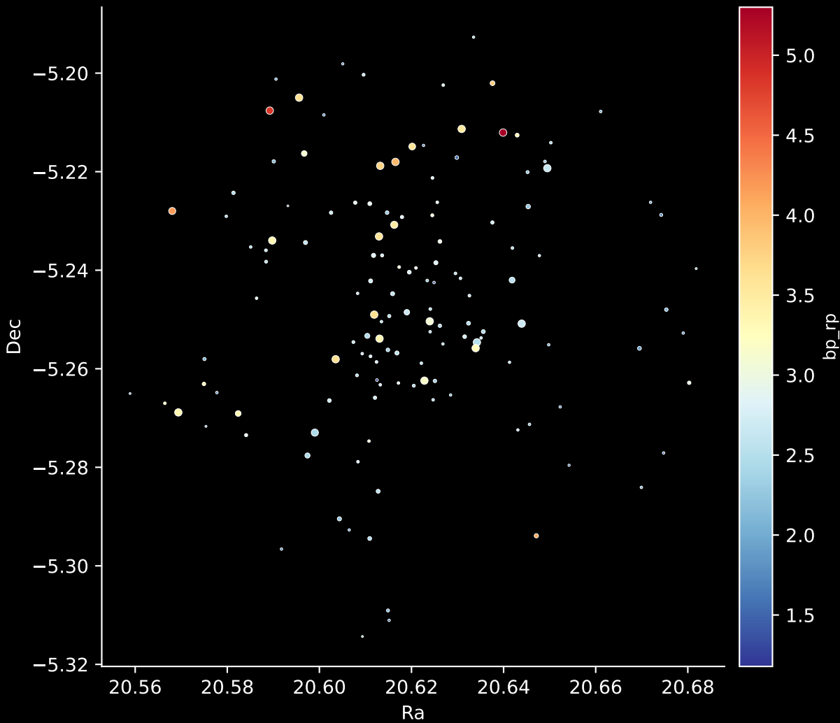
Gaia Cluster: [Teutsch_145] Stars: 138
