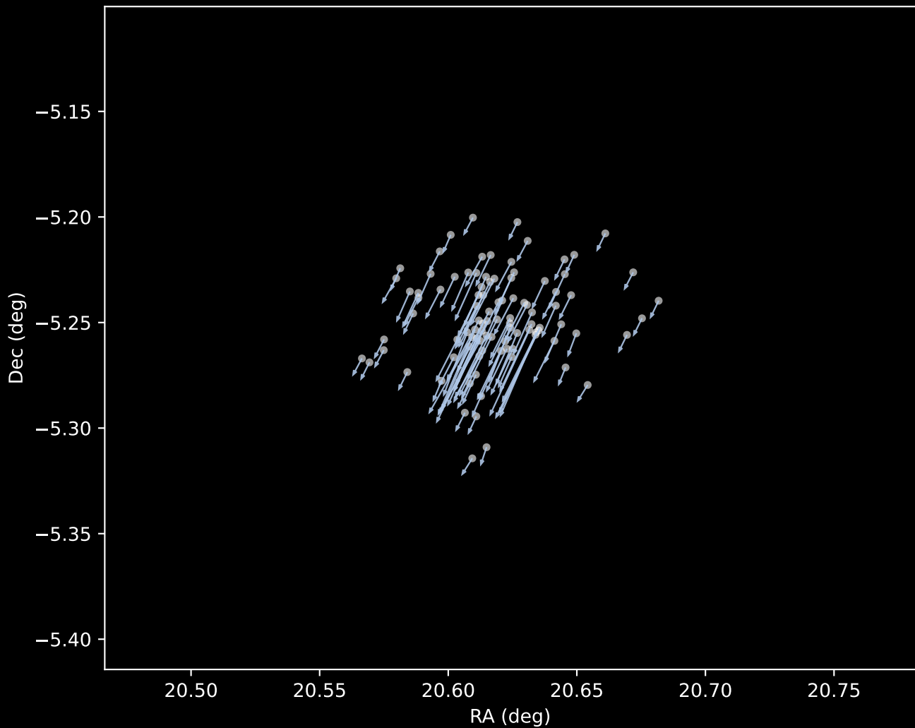
Gaia DR3 Cluster 1 Proper Motion Vectors (n=97)
