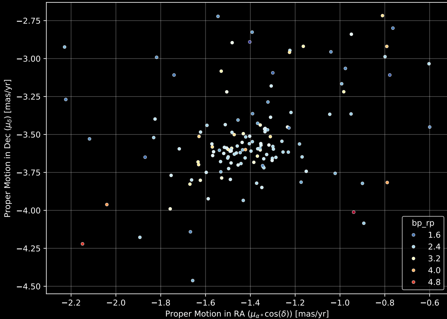
Gaia Cluster: [Teutsch_145] Proper Motion Diagram (n= 138)
