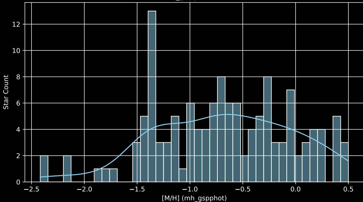
Gaia Cluster: [Deutsch_145 [M/H] (mh_gspphot) (n= 133)
