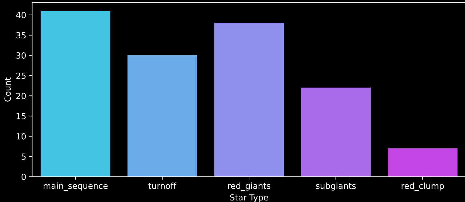
Gaia Cluster: [Teutsch_145] Count plot of Star Type
