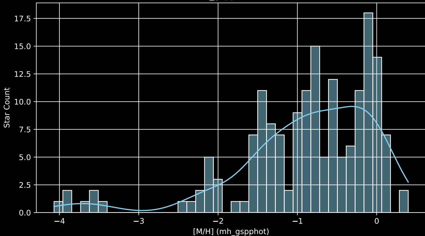
Gaia Cluster: [Teutsch_156 [M/H] (mh_gspphot) (n= 171)
