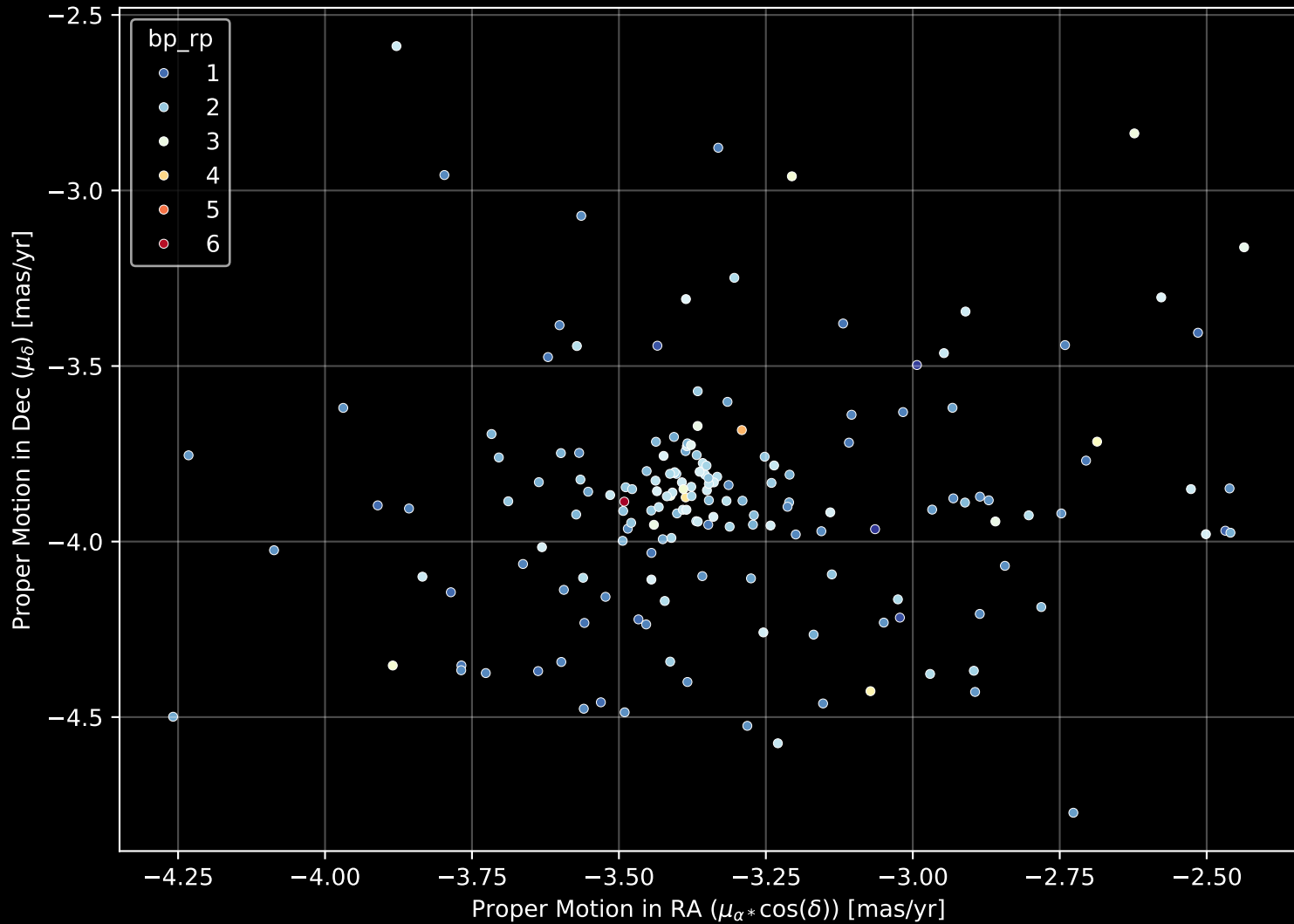
Gaia Cluster: [Teutsch_156] Proper Motion Diagram (n= 171)
