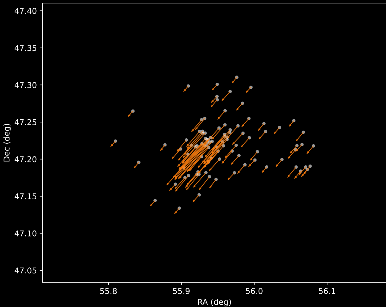
Gaia DR3 Cluster 2 Proper Motion Vectors (n=92)
