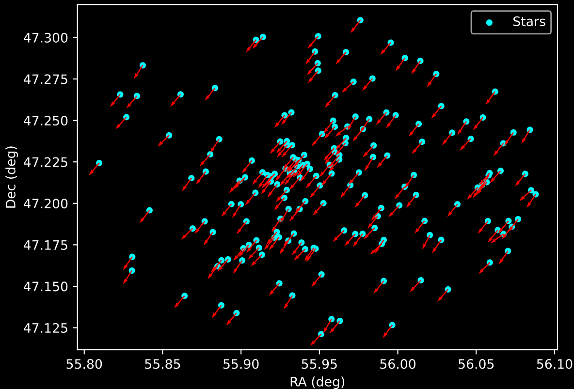
Gaia Cluster: [Teutsch_156] Proper Motion Vectors for Gaia Star Field (n= 171)
