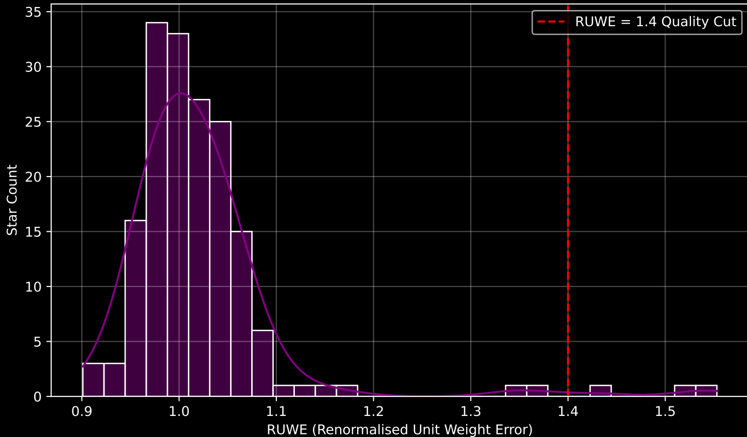
Gaia Cluster: [Teutsch_156] RUWE Distribution (n= 171)
