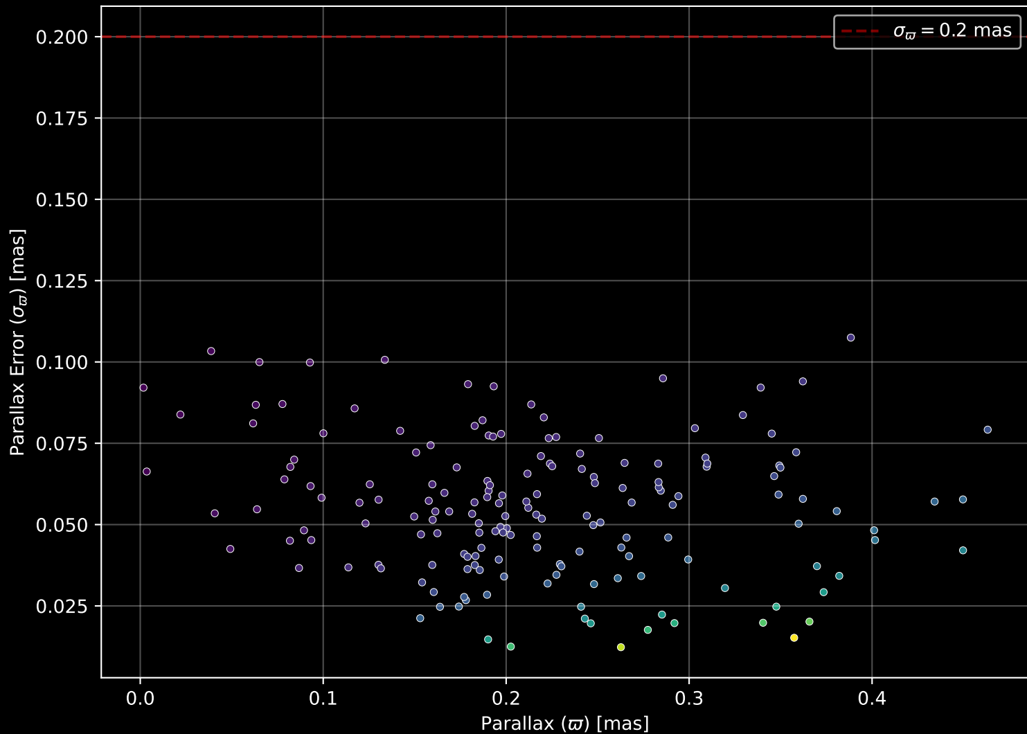
Gaia Cluster: [Teutsch_156] Parallax Quality (n= 171)
