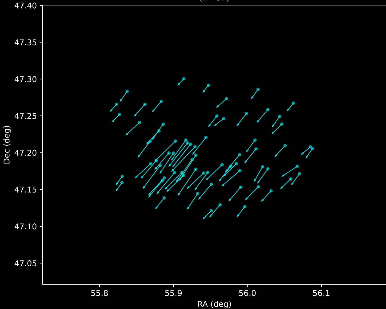
Gaia DR3 Noise Stream Proper Motion Vectors (n=67)
