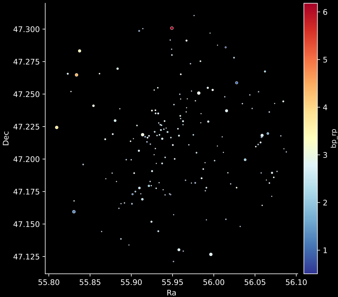
Gaia Cluster: [Teutsch_156] Stars: 171
