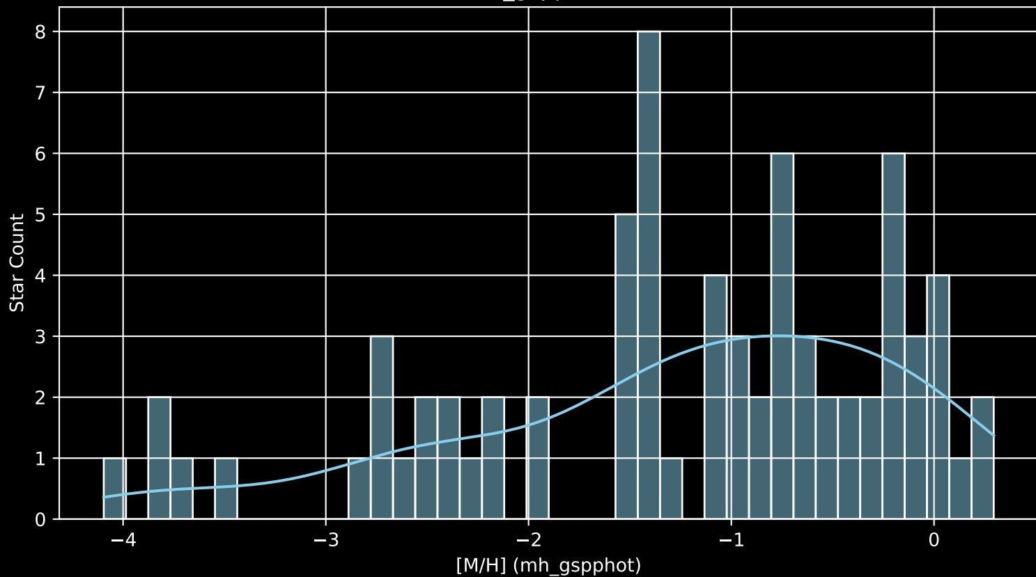
Gaia Cluster: [Teutsch_31 [M/H] (mh_gspphot) (n= 73)
