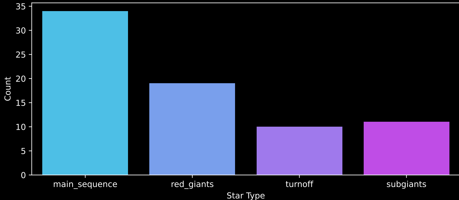
Gaia Cluster: [Teutsch_31] Count plot of Star Type
