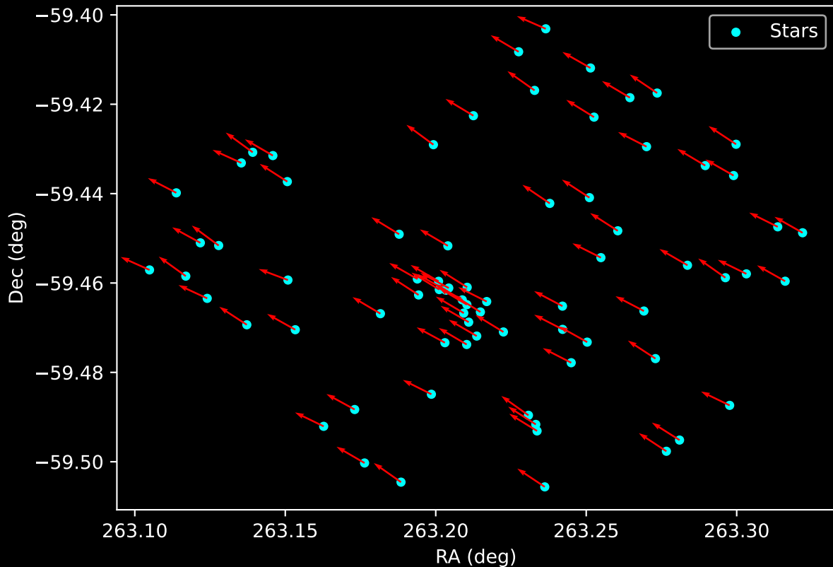
Gaia Cluster: [Teutsch_31] Proper Motion Vectors for Gaia Star Field (n= 74)
