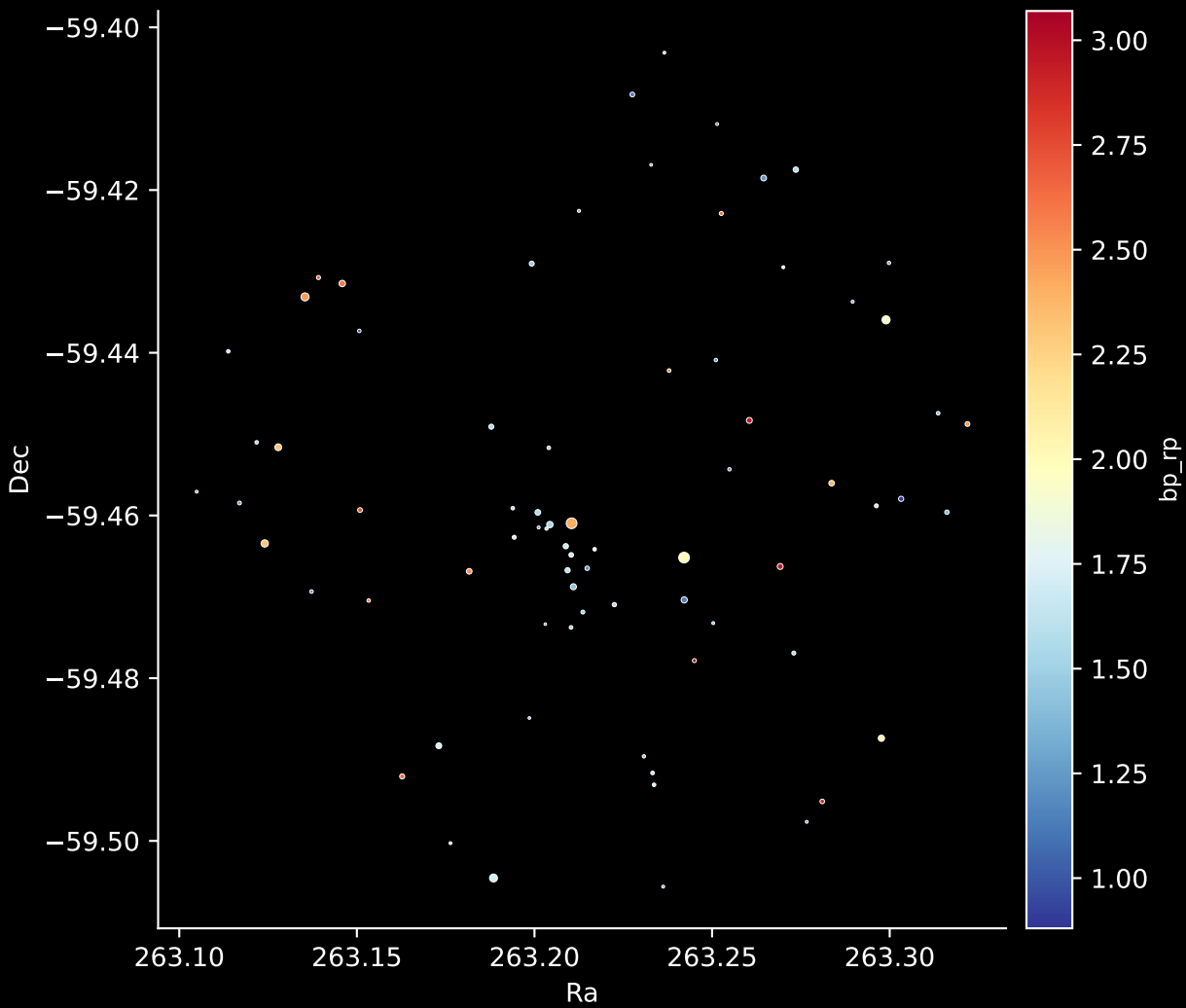
Gaia Cluster: [Teutsch_31] Stars: 74
