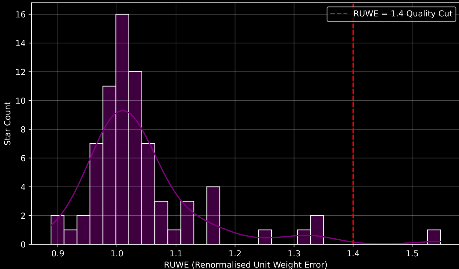
Gaia Cluster: [Teutsch_31] RUWE Distribution (n= 74)
