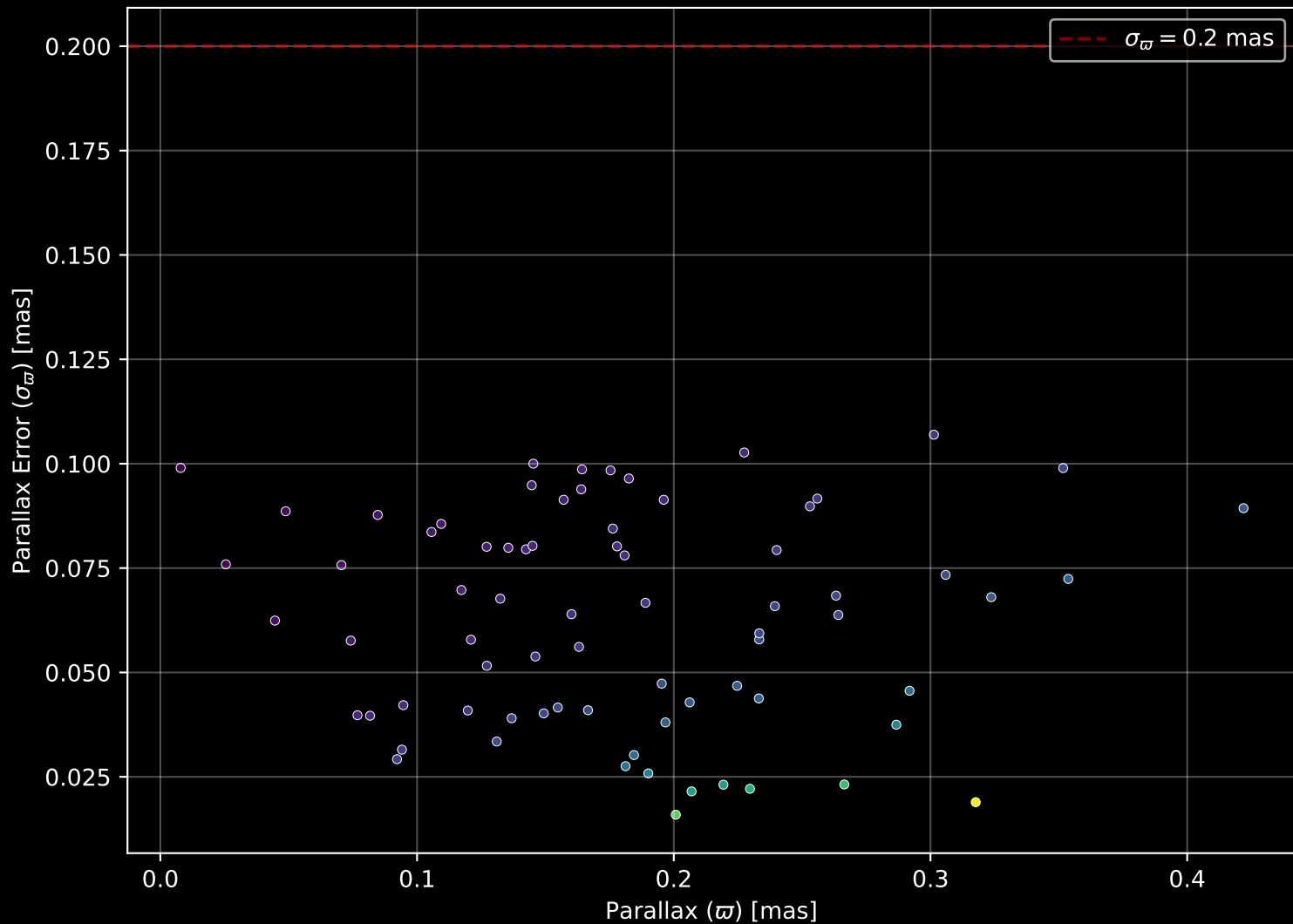
Gaia Cluster: [Teutsch_31] Parallax Quality (n= 74)
