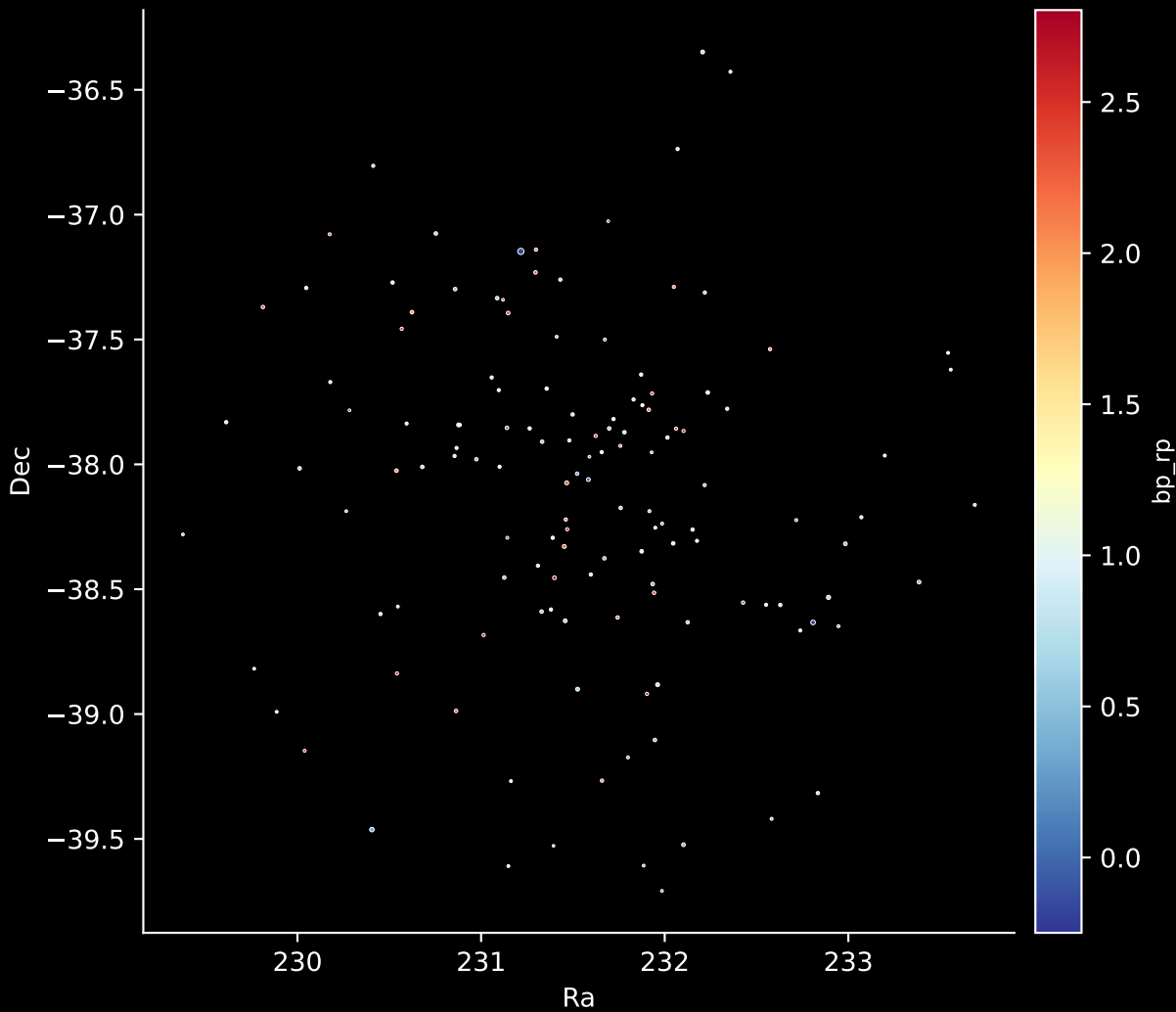
Gaia Cluster: [Teutsch_38] Stars: 133
