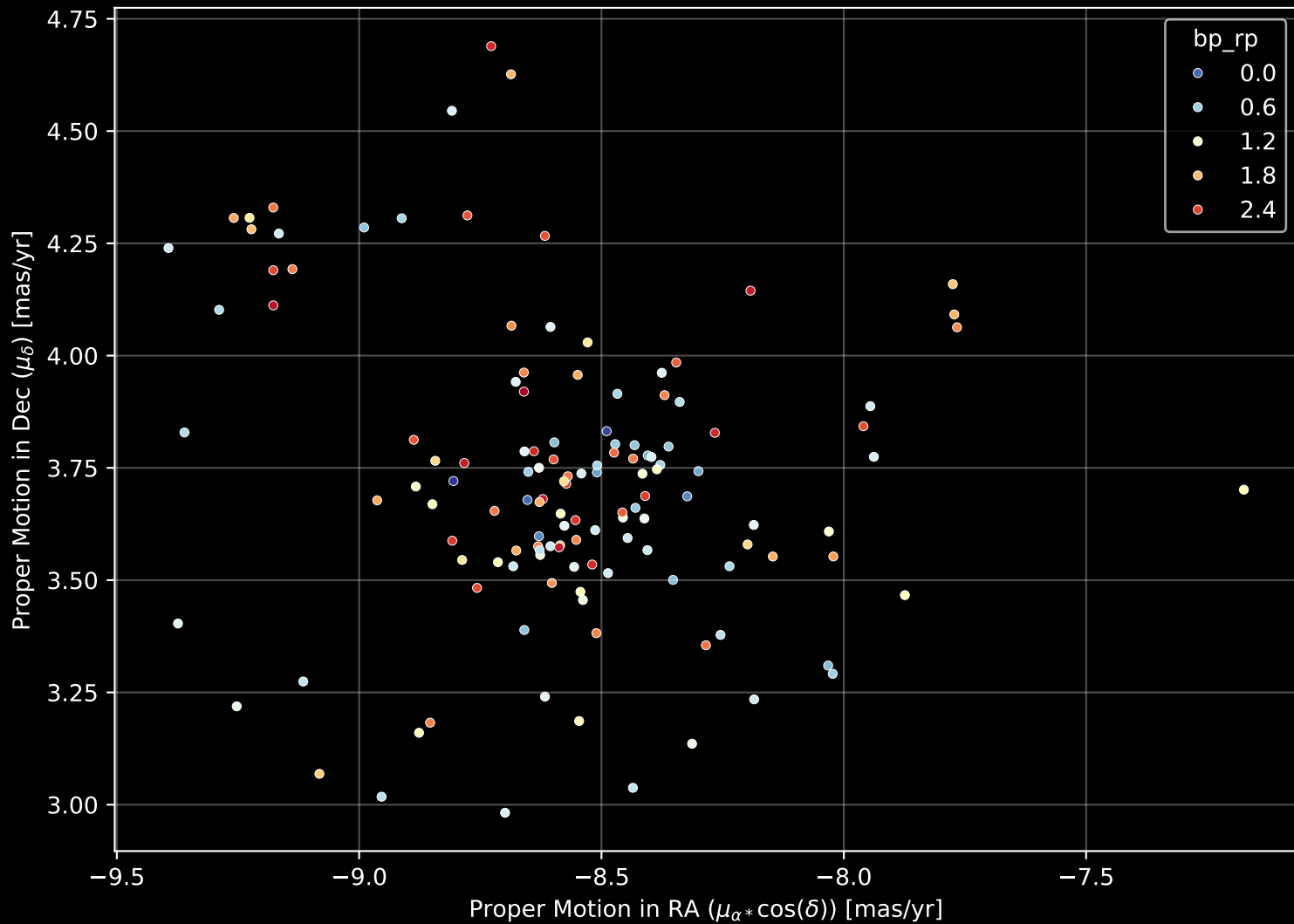
Gaia Cluster: [Teutsch_38] Proper Motion Diagram (n= 133)
