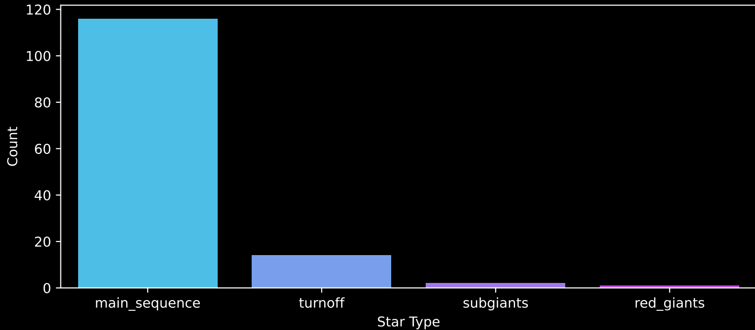
Gaia Cluster: [Teutsch_38] Count plot of Star Type
