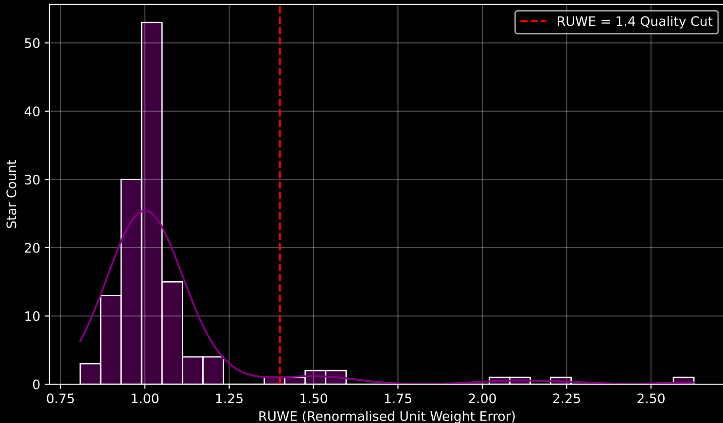
Gaia Cluster: [Teutsch_38] RUWE Distribution (n= 132)
