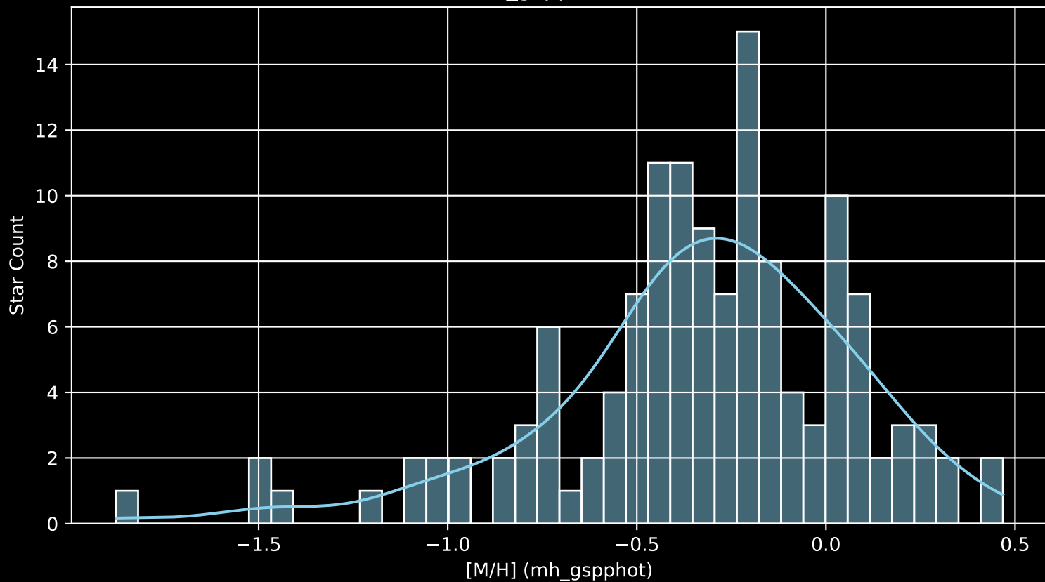
Gaia Cluster: [Teutsch_38 [M/H] (mh_gspphot) (n= 133)
