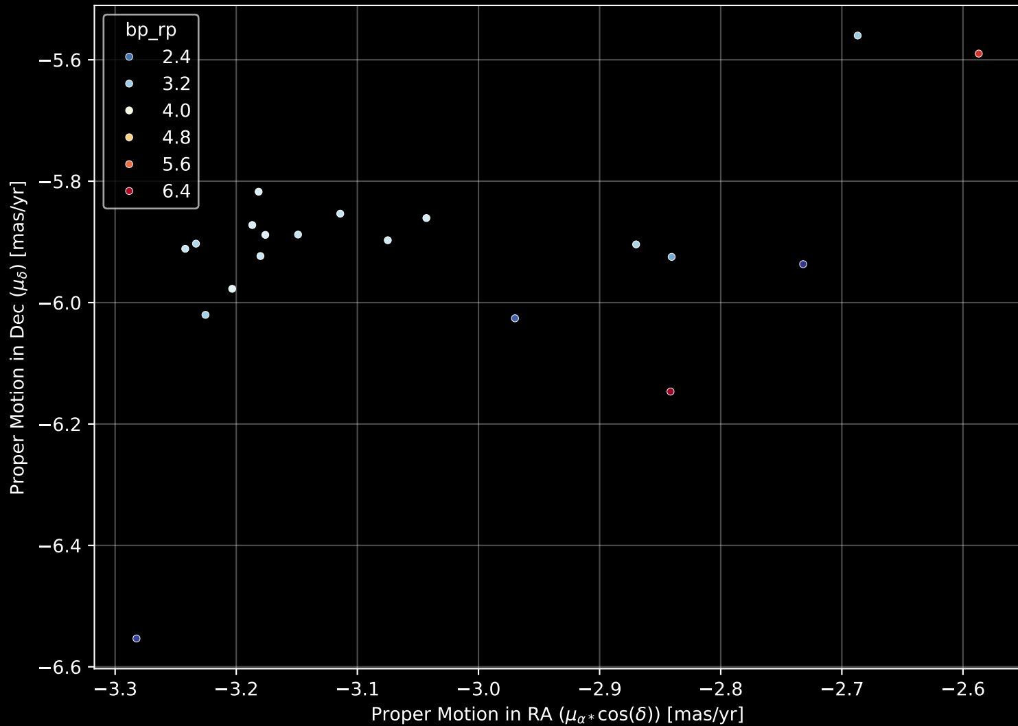
Gaia Cluster: [Teutsch_42] Proper Motion Diagram (n= 20)
