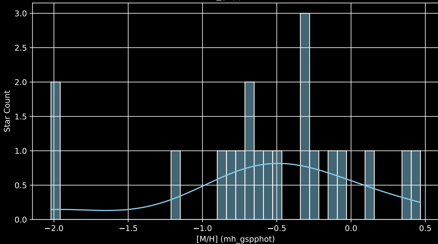
Gaia Cluster: [Teutsch_42 [M/H] (mh_gspphot) (n= 20)
