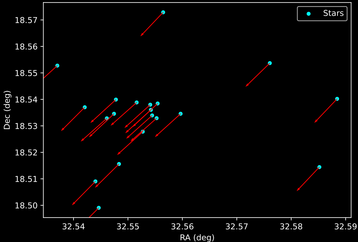
Gaia Cluster: [Teutsch_42] Proper Motion Vectors for Gaia Star Field (n= 20)
