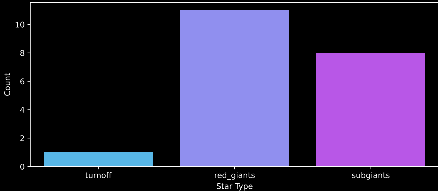
Gaia Cluster: [Teutsch_42] Count plot of Star Type
