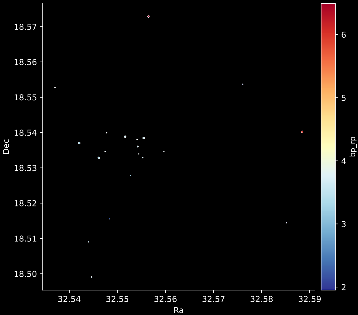
Gaia Cluster: [Teutsch_42] Stars: 20
