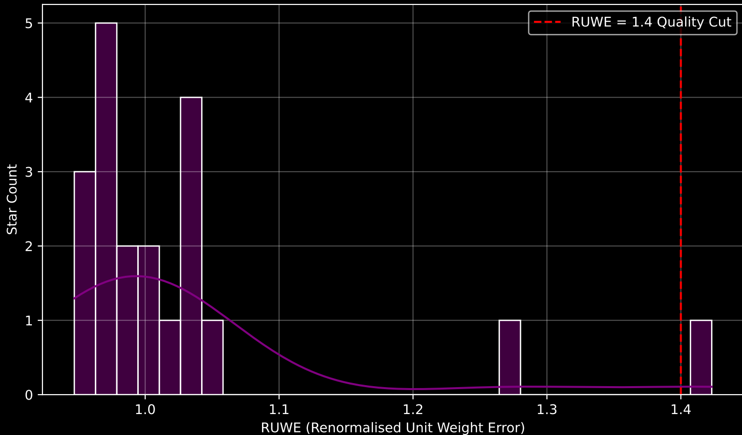
Gaia Cluster: [Teutsch_42] RUWE Distribution (n= 20)
