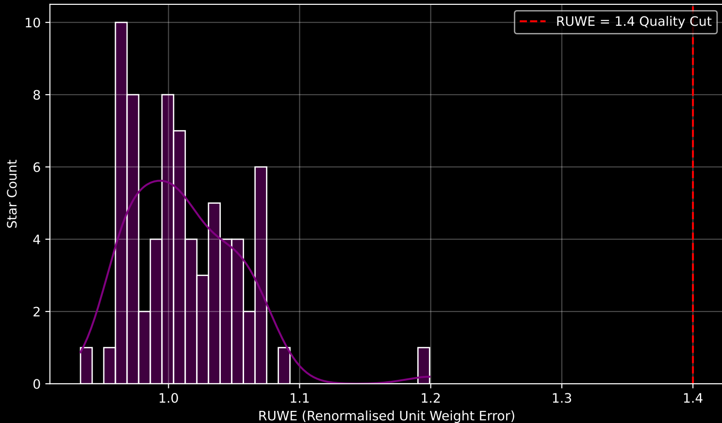
Gaia Cluster: [Teutsch_61] RUWE Distribution (n= 71)
