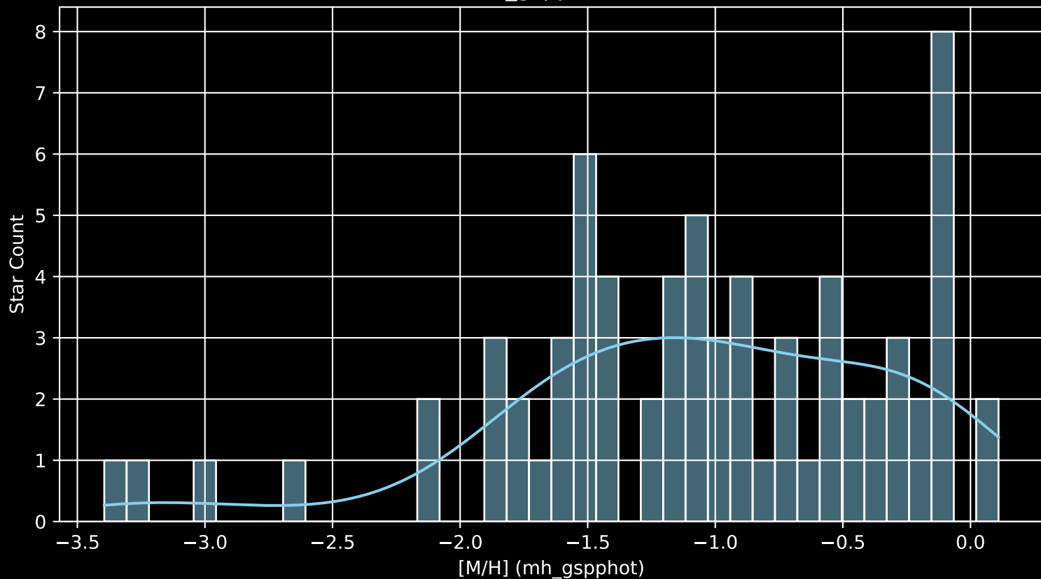
Gaia Cluster: [Teutsch_61 [M/H] (mh_gspphot) (n= 71)
