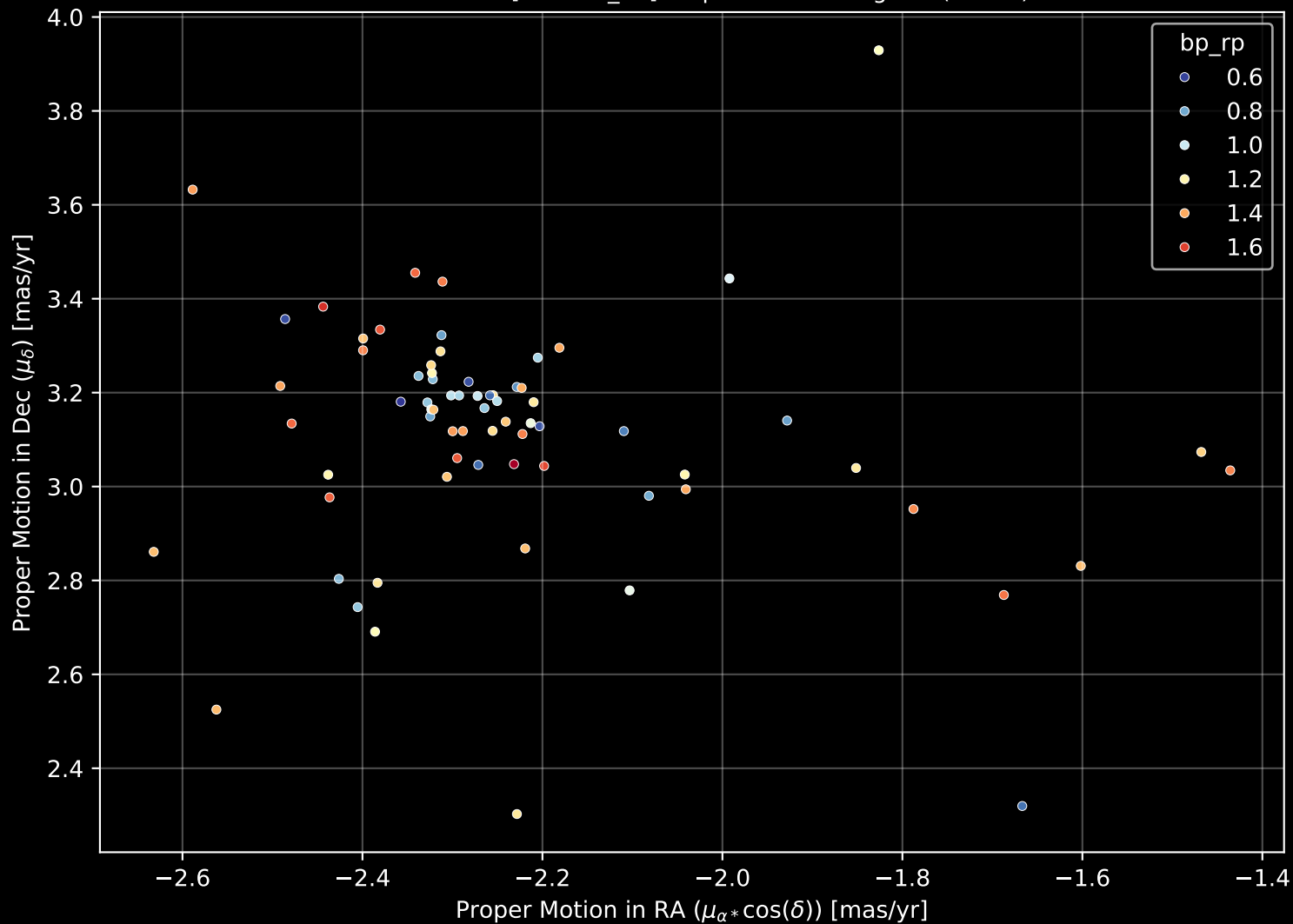
Gaia Cluster: [Deutsch_61] Proper Motion Diagram (n= 71)
