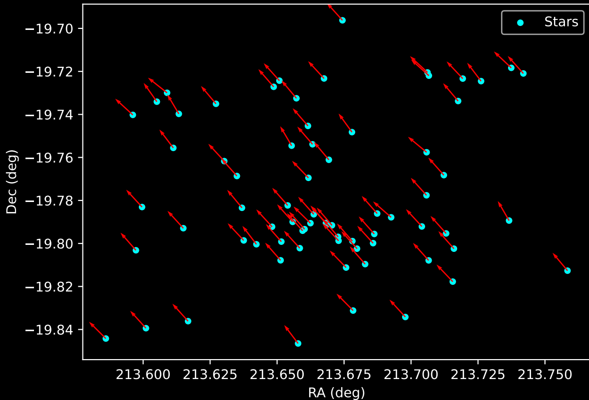
Gaia Cluster: [Teutsch_61] Proper Motion Vectors for Gaia Star Field (n= 71)
