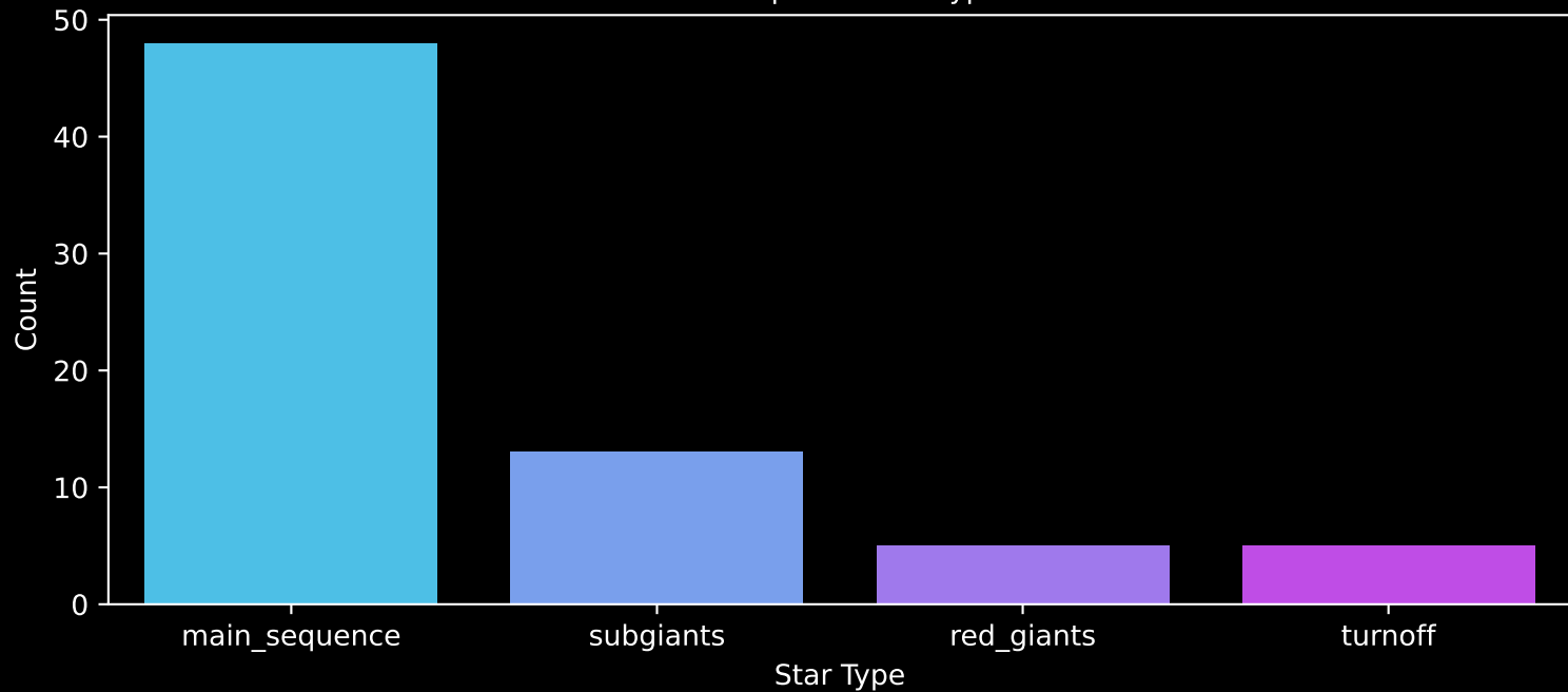
Gaia Cluster: [Teutsch_61] Count plot of Star Type
