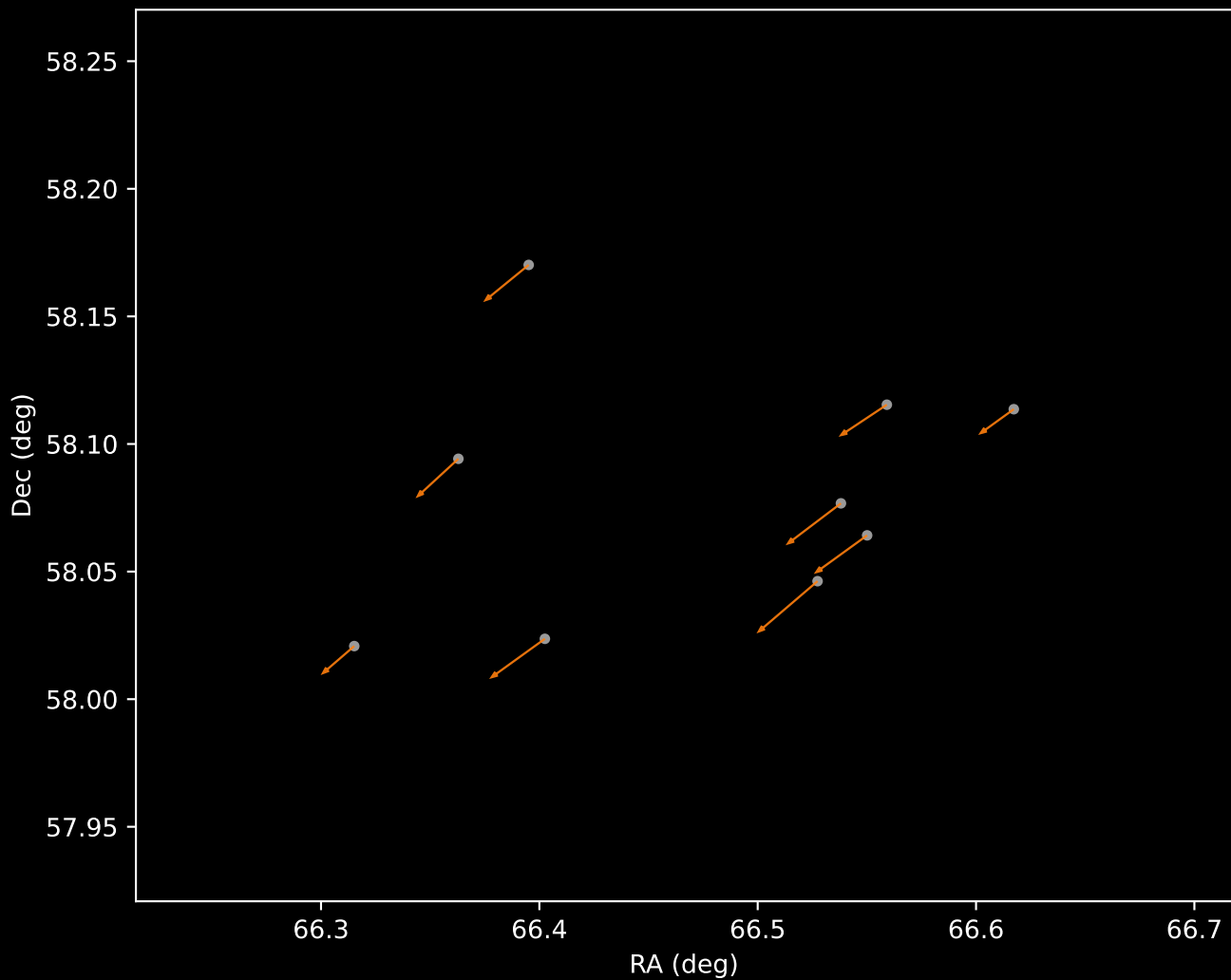
Gaia DR3 Cluster 2 Proper Motion Vectors (n=9)
