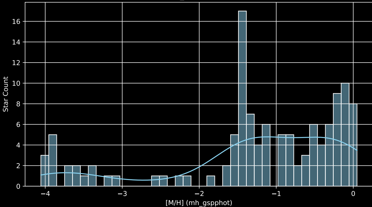
Gaia Cluster: [Teutsch_74 [M/H] (mh_gspphot) (n= 121)
