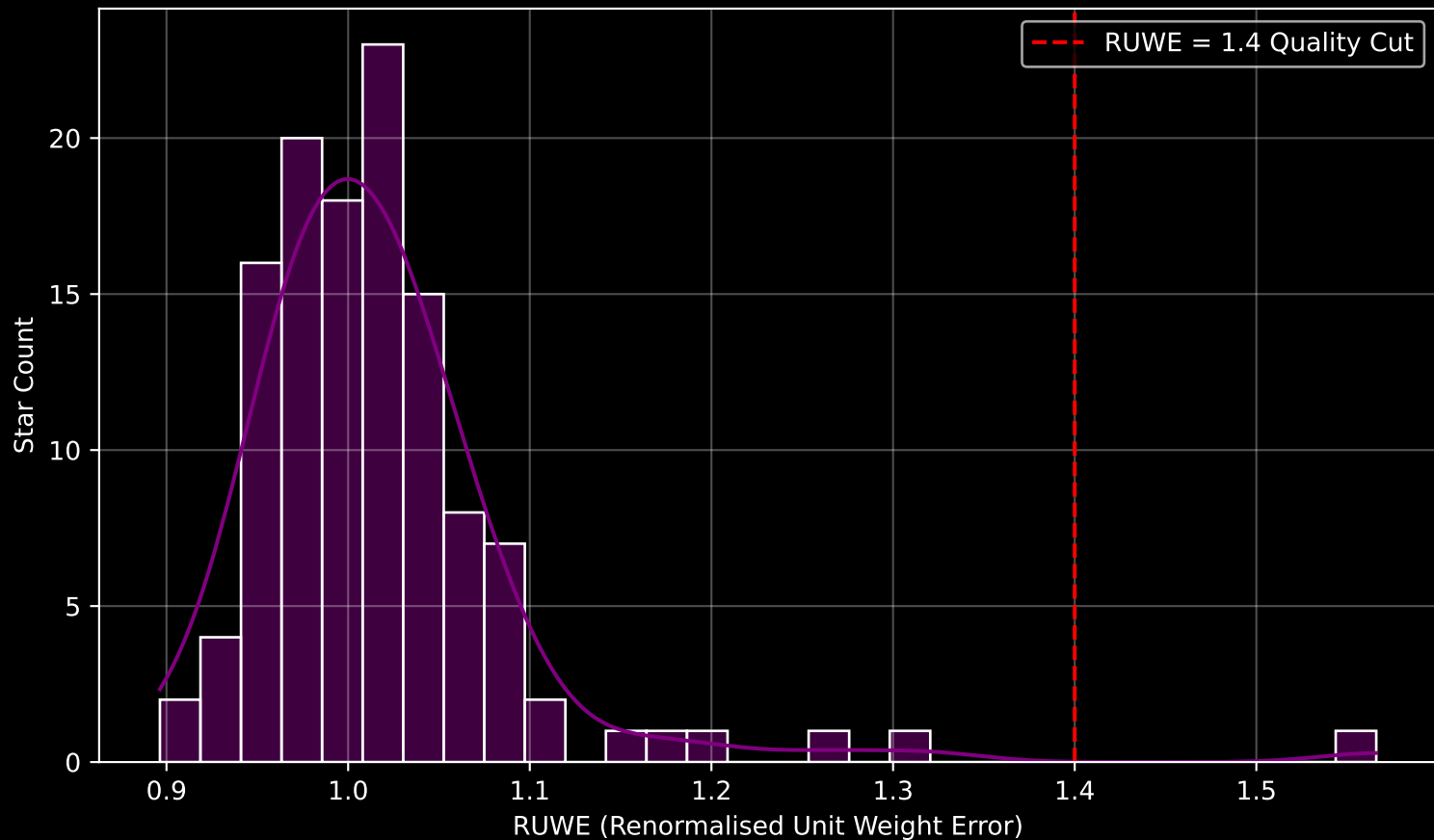
Gaia Cluster: [Teutsch_74] RUWE Distribution (n= 121)
