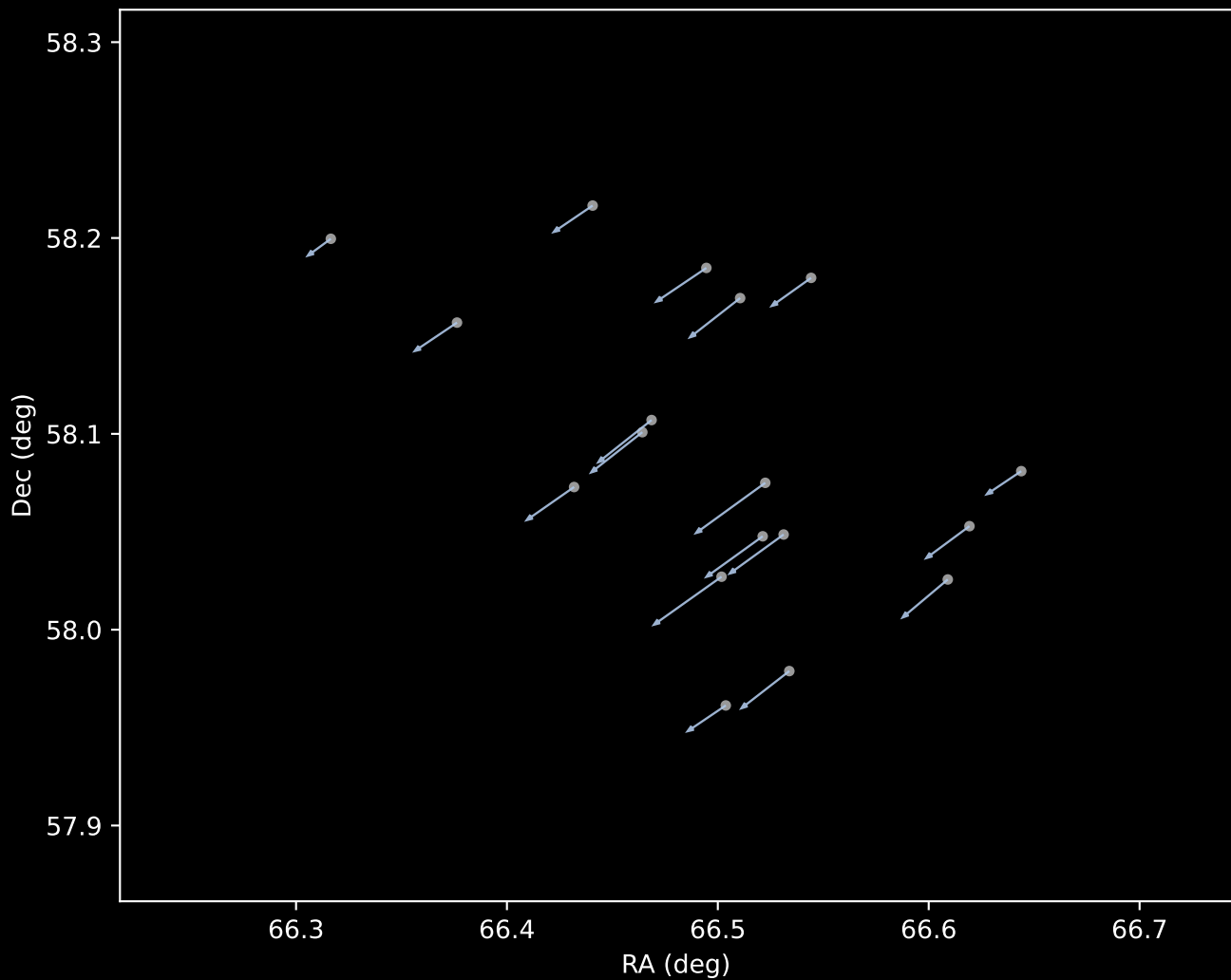
Gaia DR3 Cluster 1 Proper Motion Vectors (n=18)
