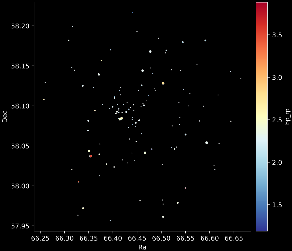
Gaia Cluster: [Teutsch_74] Stars: 121
