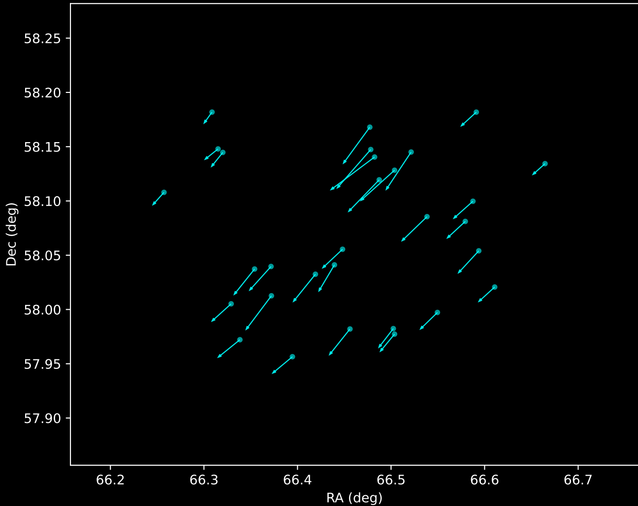
Gaia DR3 Noise Stream Proper Motion Vectors (n=30)
