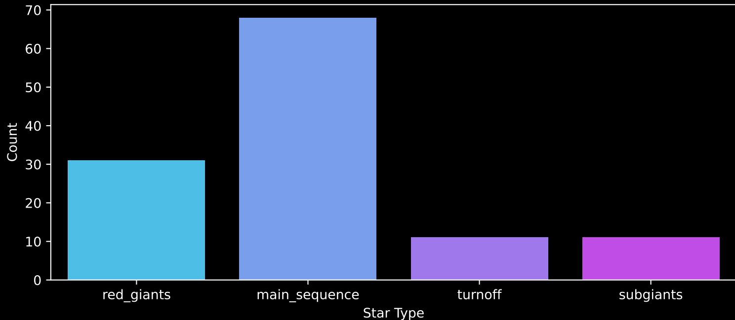
Gaia Cluster: [Teutsch_74] Count plot of Star Type
