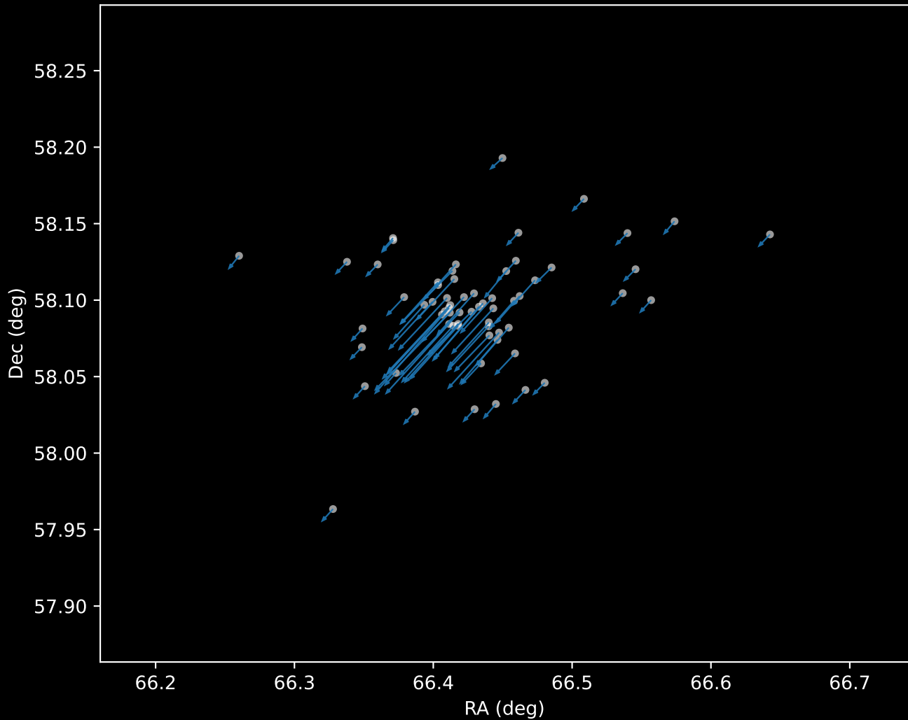
Gaia DR3 Cluster 0 Proper Motion Vectors (n=64)
