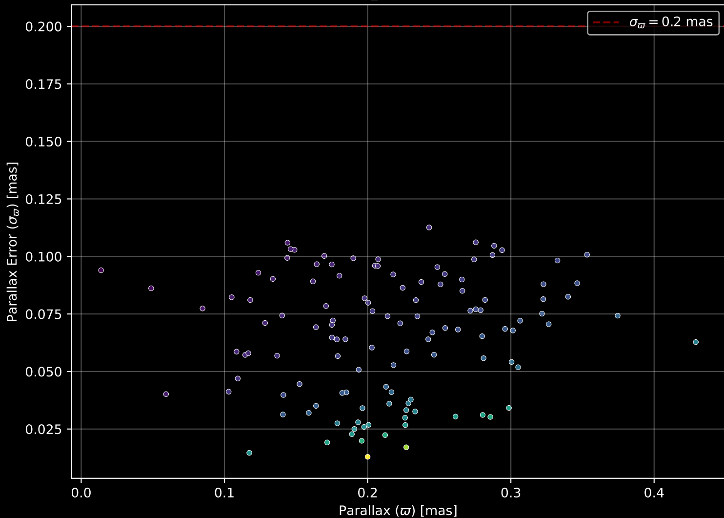
Gaia Cluster: [Teutsch_74] Parallax Quality (n= 121)
