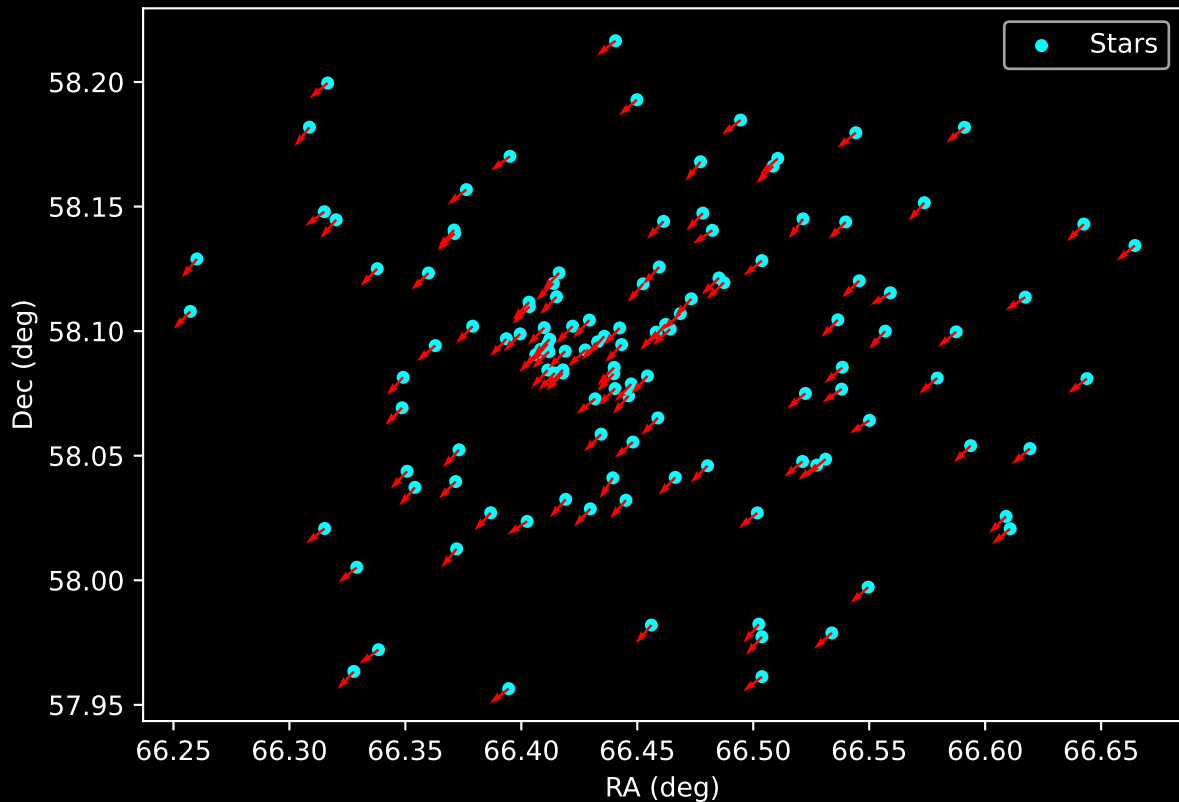
Gaia Cluster: [Teutsch_74] Proper Motion Vectors for Gaia Star Field (n= 121)
