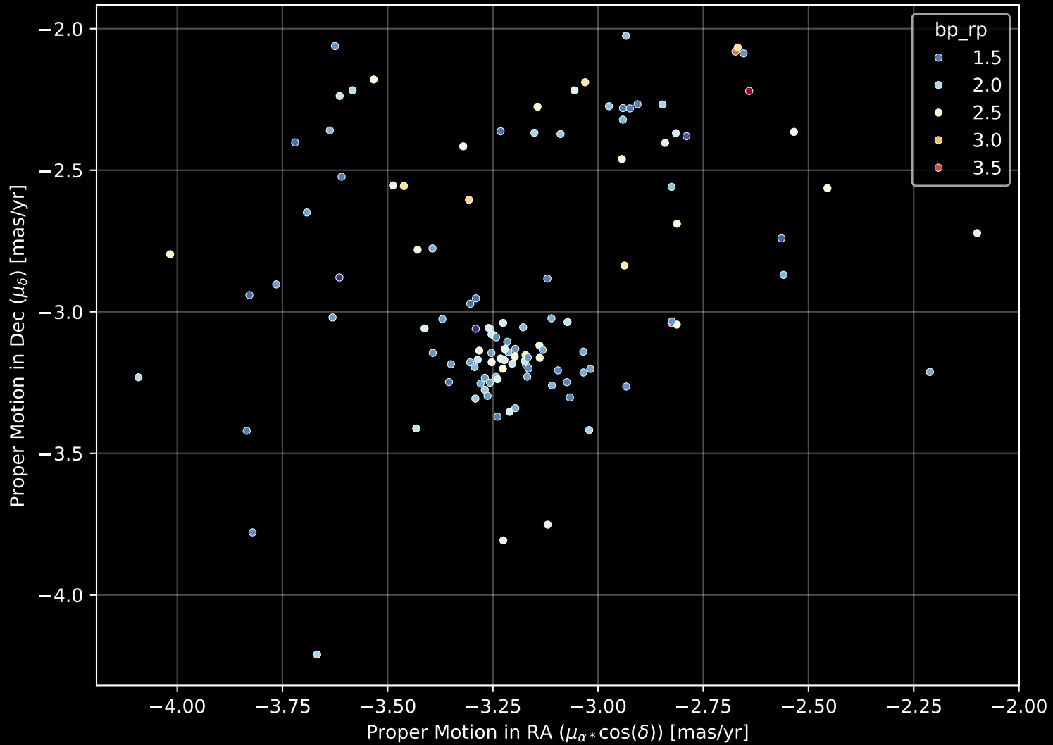
Gaia Cluster: [Teutsch_74] Proper Motion Diagram (n= 121)
