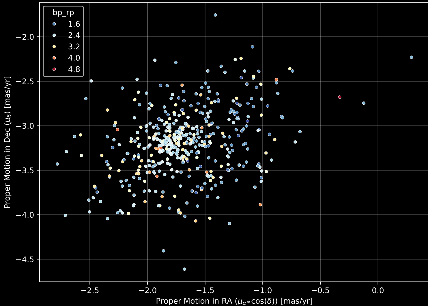
Gaia Cluster: [Teutsch_85] Proper Motion Diagram (n= 475)
