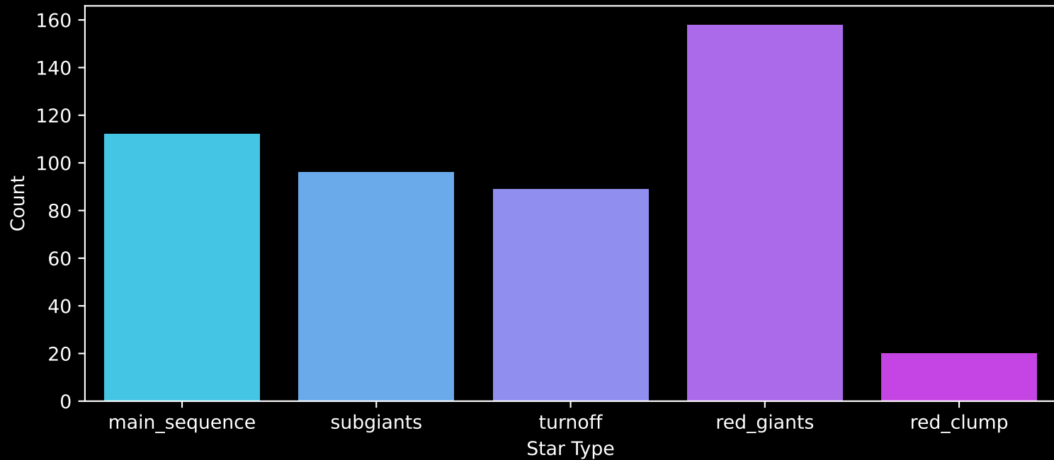
Gaia Cluster: [Teutsch_85] Count plot of Star Type
