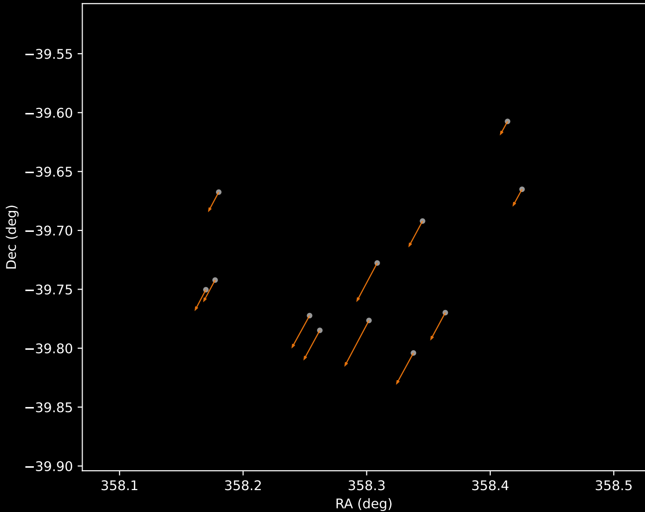
Gaia DR3 Cluster 22 Proper Motion Vectors (n=12)
