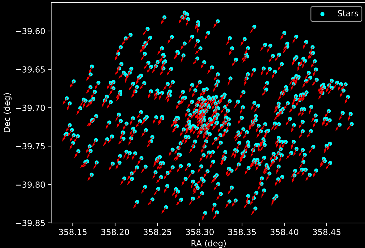
Gaia Cluster: [Teutsch_85] Proper Motion Vectors for Gaia Star Field (n= 475)
