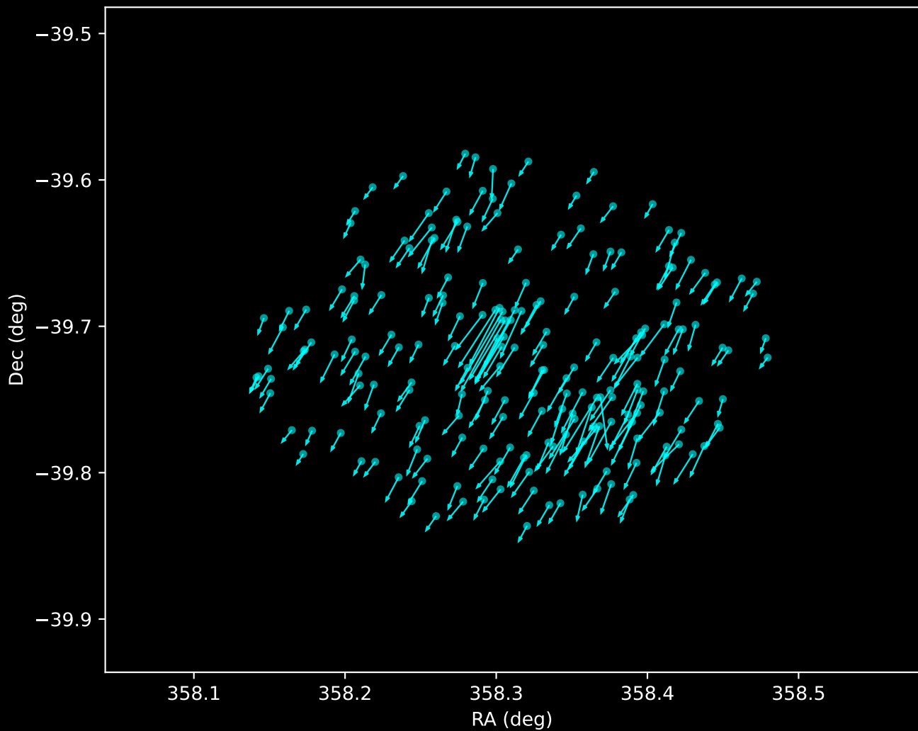
Gaia DR3 Noise Stream Proper Motion Vectors (n=210)
