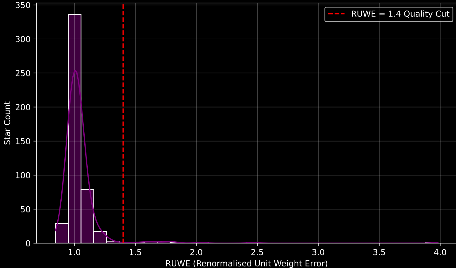
Gaia Cluster: [Teutsch_85] RUWE Distribution (n= 475)
