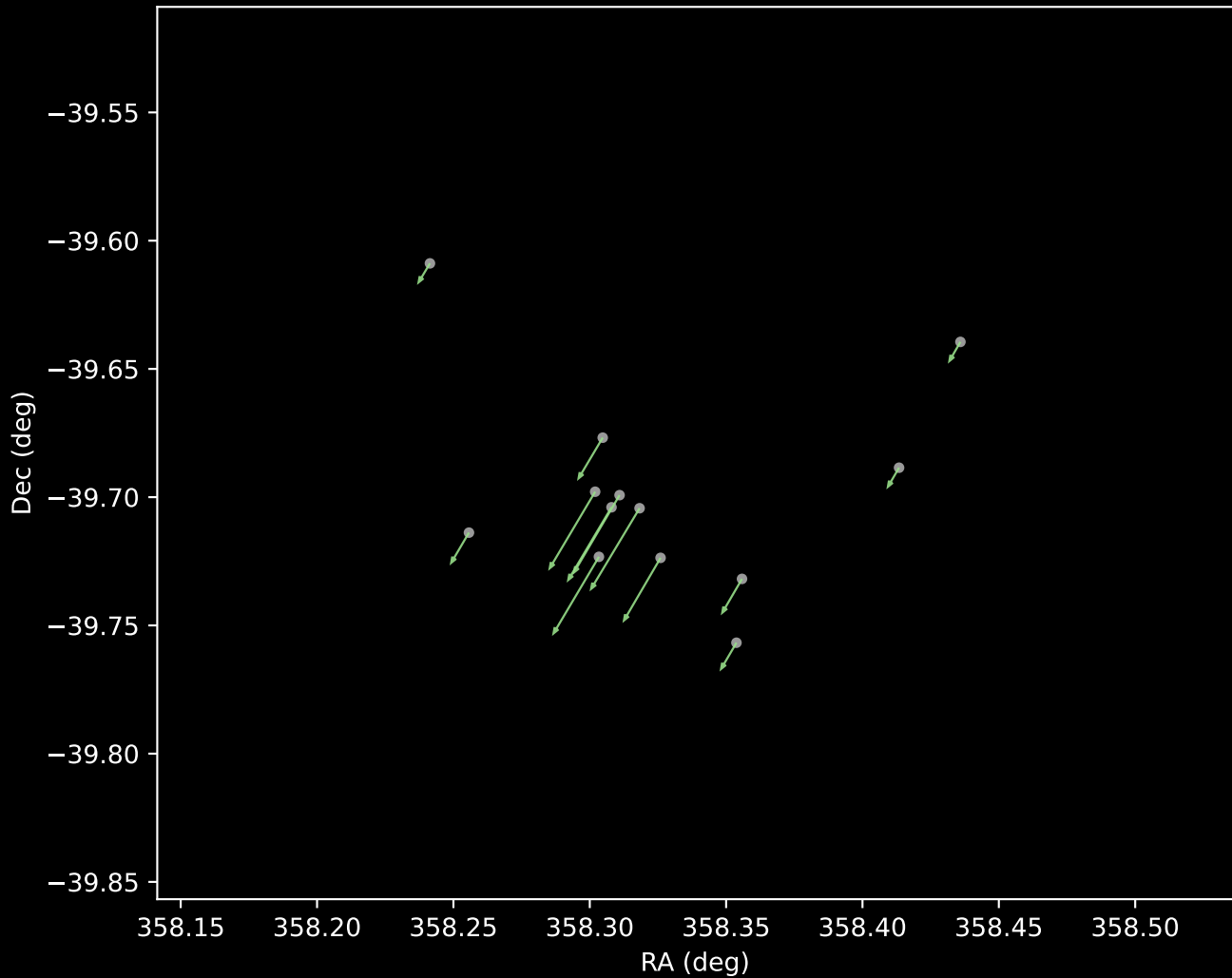
Gaia DR3 Cluster 25 Proper Motion Vectors (n=13)
