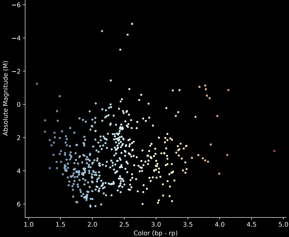
Gaia Cluster: [Teutsch_85] Stars (n= 475) Hertzsprung-Russel Diagram
