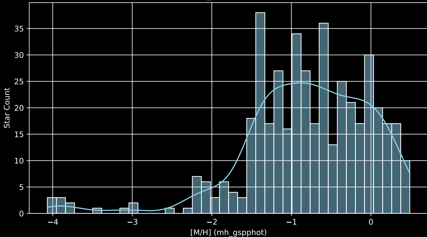
Gaia Cluster: [Teutsch_85 [M/H] (mh_gspphot) (n= 443)
