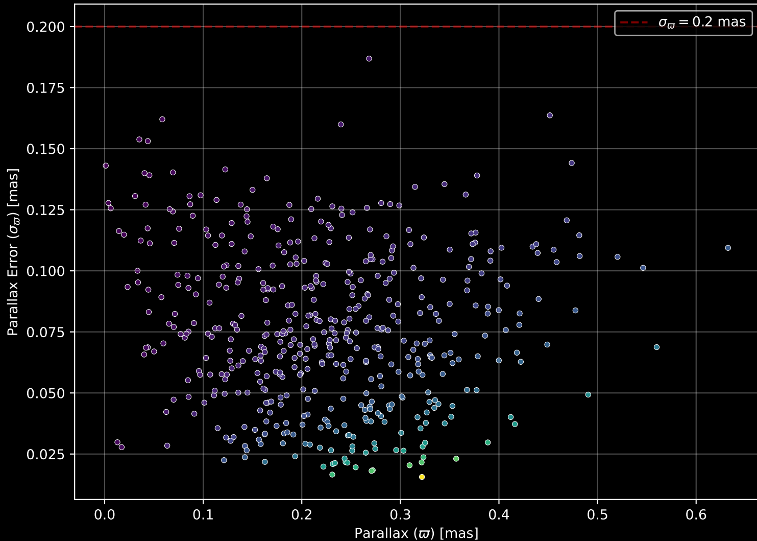
Gaia Cluster: [Teutsch_85] Parallax Quality (n= 475)
