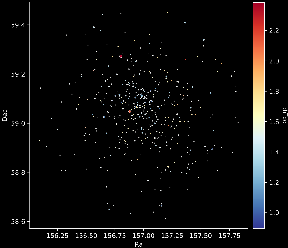
Gaia Cluster: [Tombaugh_5] Stars: 450
