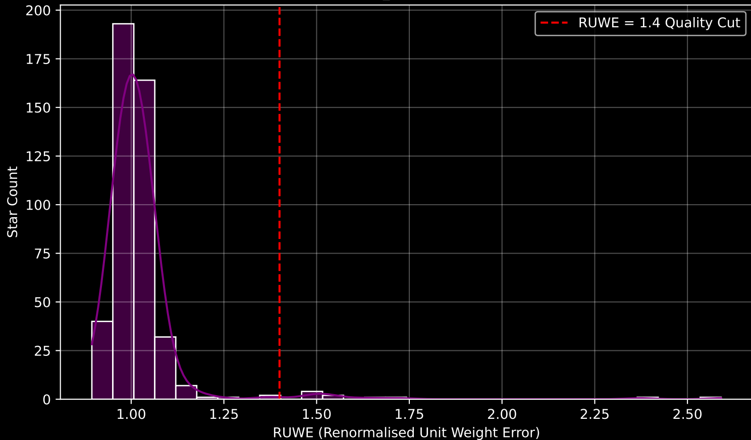
Gaia Cluster: [Tombaugh_5] RUWE Distribution (n= 450)
