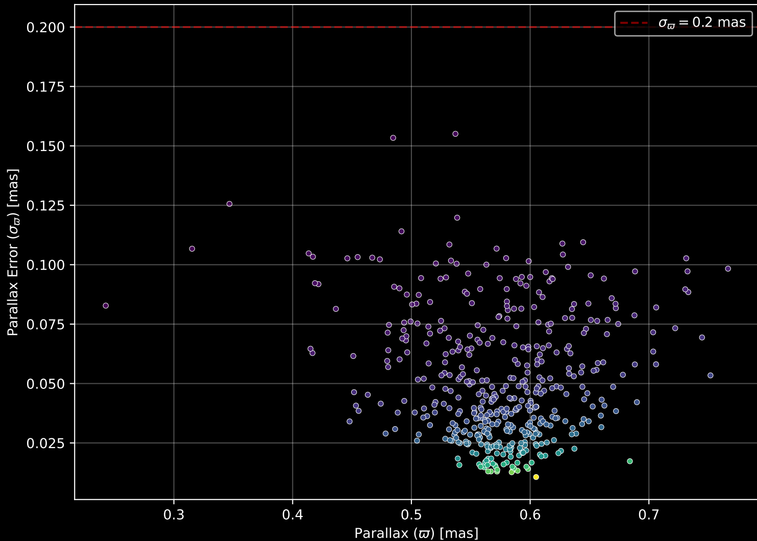
Gaia Cluster: [Tombaugh_5] Parallax Quality (n= 450)
