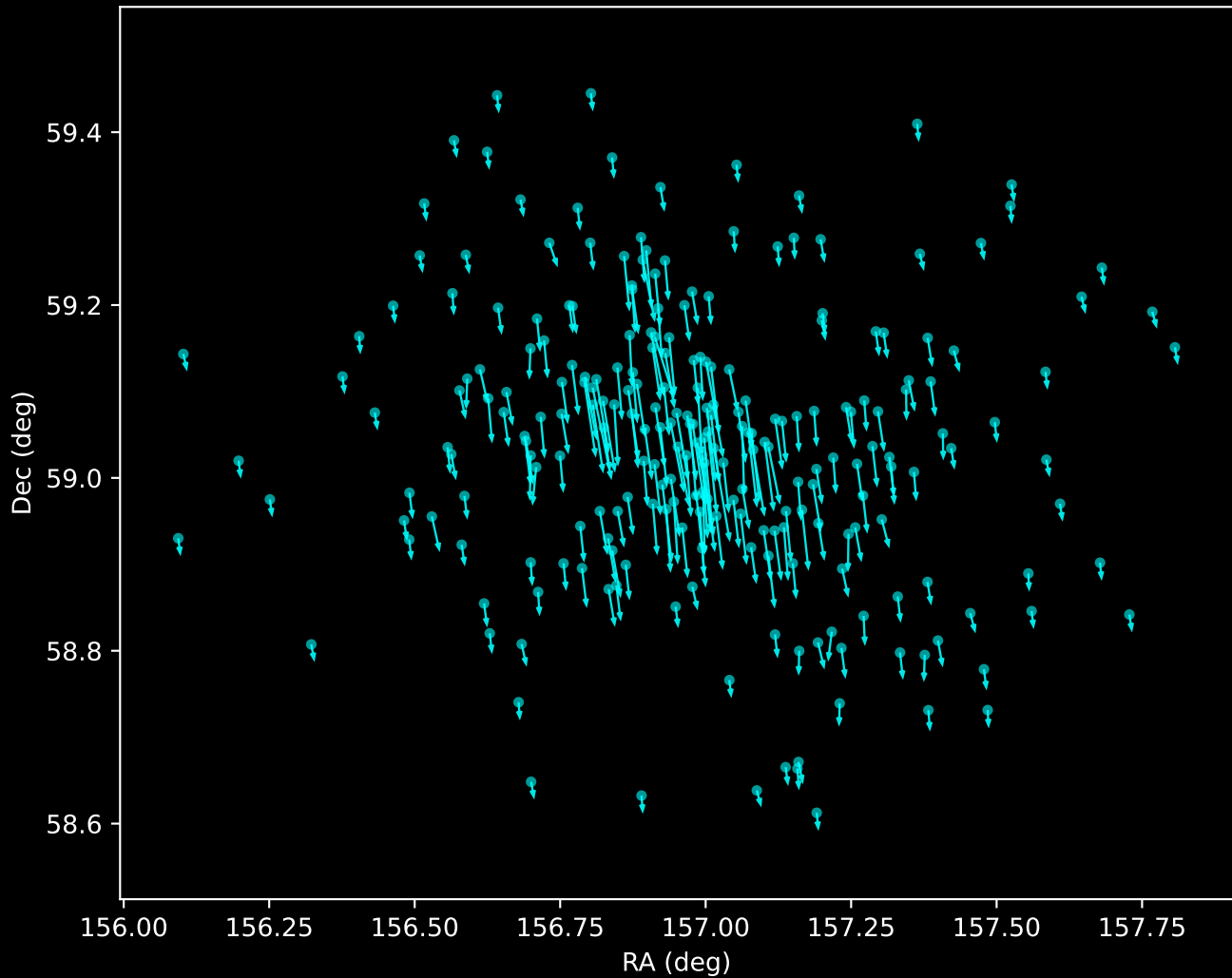
Gaia DR3 Noise Stream Proper Motion Vectors (n=243)
