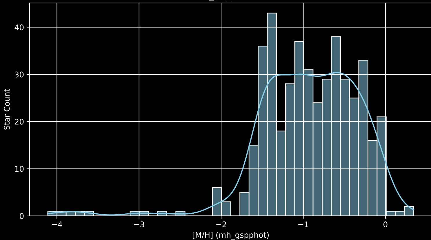
Gaia Cluster: [Tombaugh_5 [M/H] (mh_gspphot) (n= 450)
