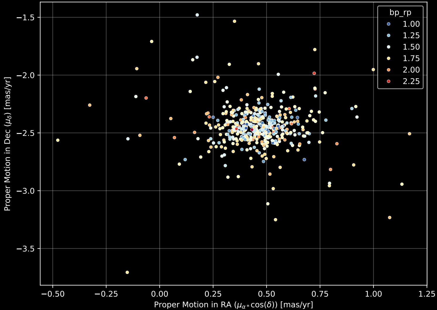
Gaia Cluster: [Tombaugh_5] Proper Motion Diagram (n= 450)
