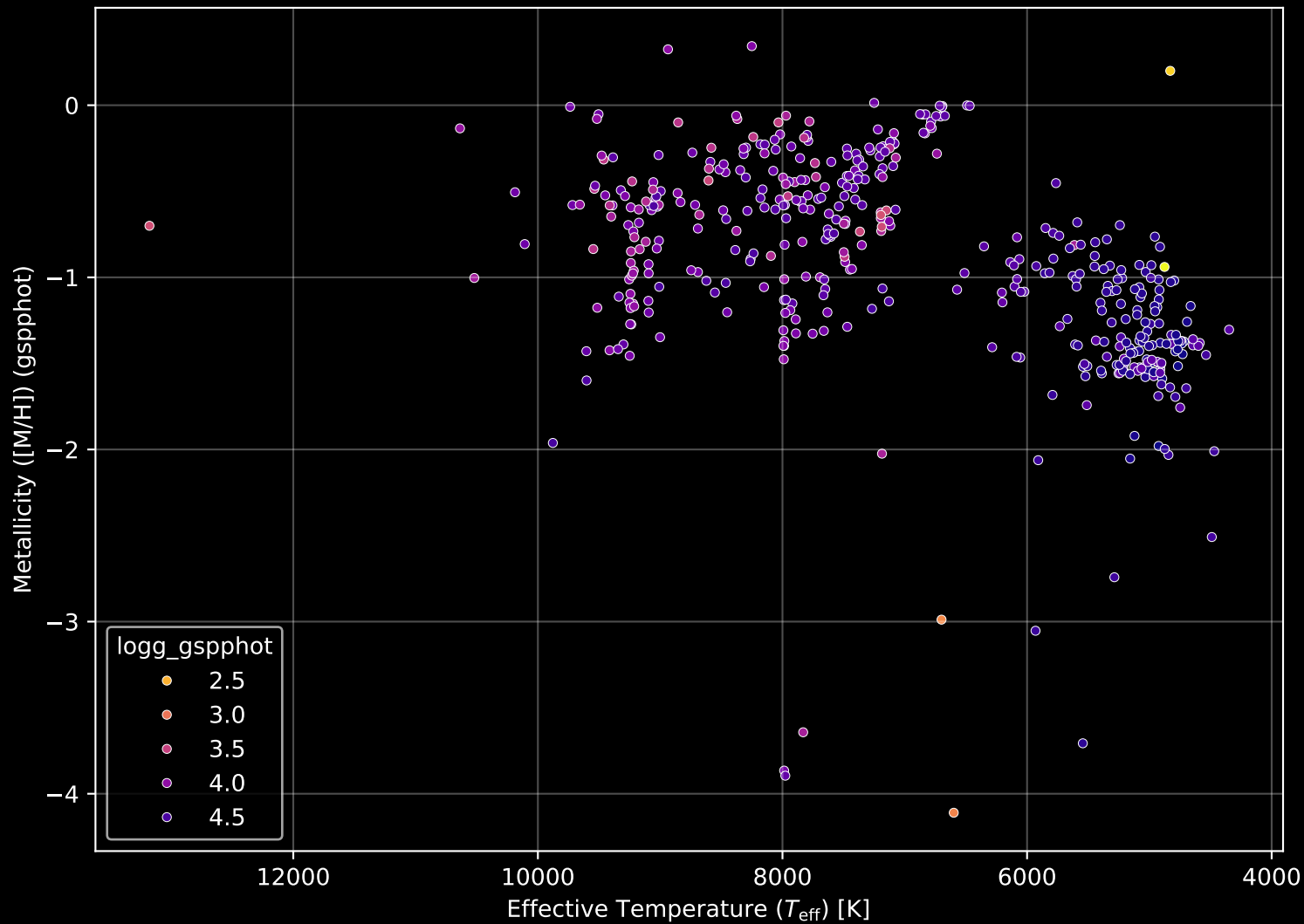
Gaia Cluster: [Tombaugh_5] Stellar Population Parameters (n= 450)
