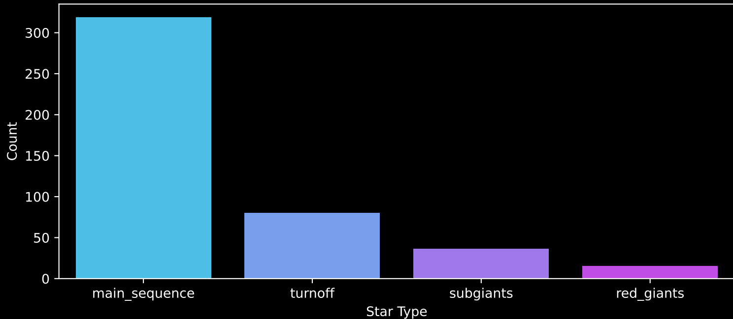
Gaia Cluster: [Tombaugh_5] Count plot of Star Type
