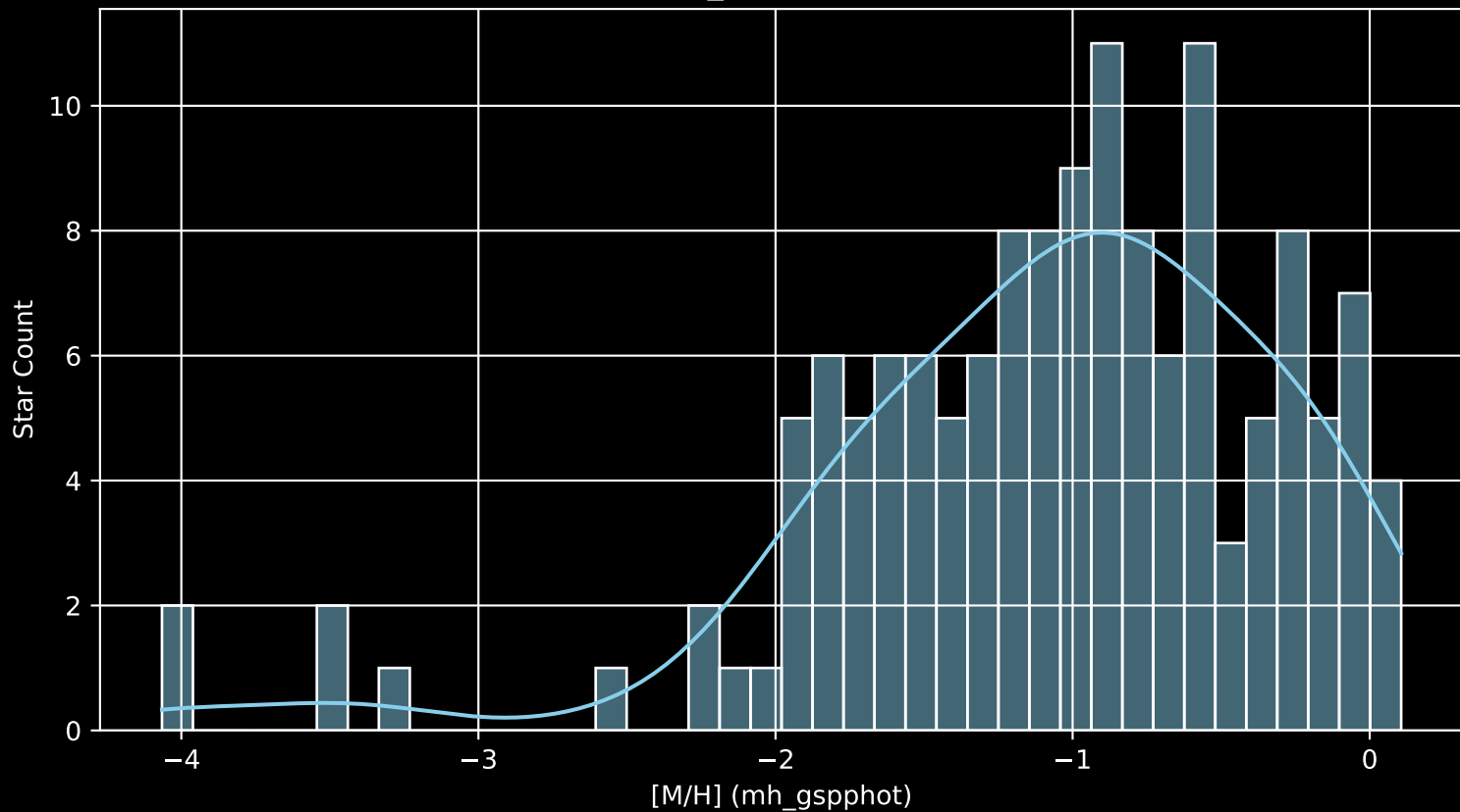
Gaia Cluster: [Trumpler_1 [M/H] (mh_gspphot) (n= 142)
