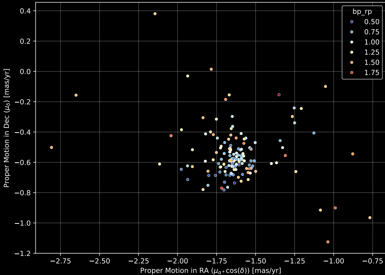
Gaia Cluster: [Trumpler_1] Proper Motion Diagram (n= 142)
