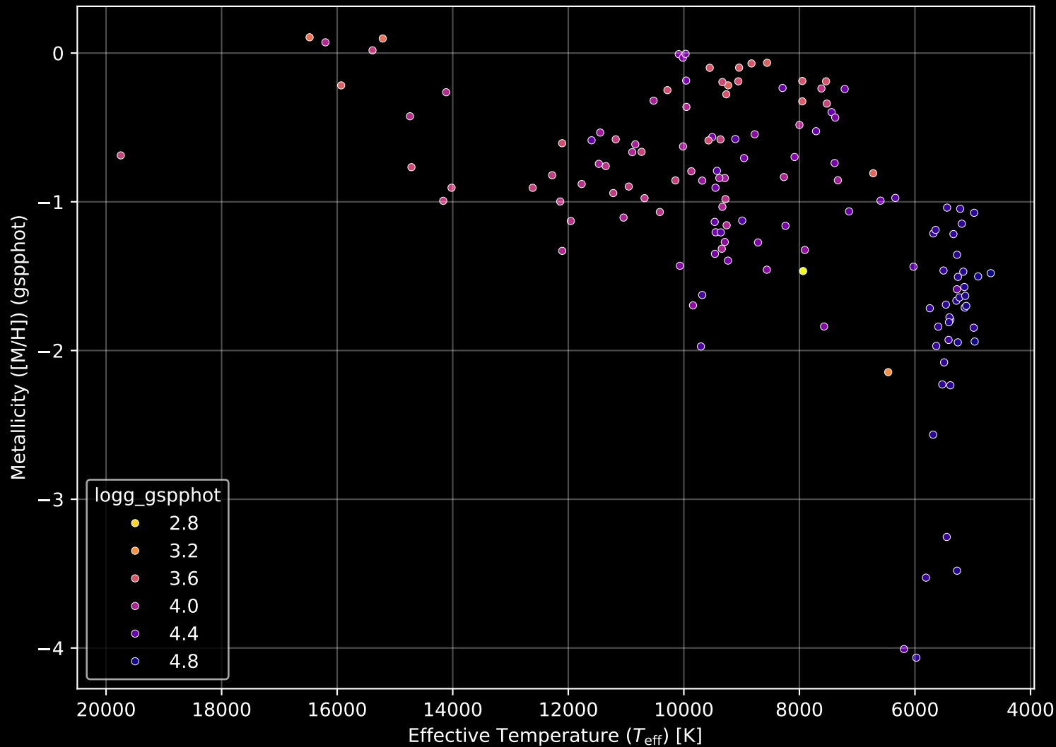
Gaia Cluster: [Trumpler_1] Stellar Population Parameters (n= 142)
