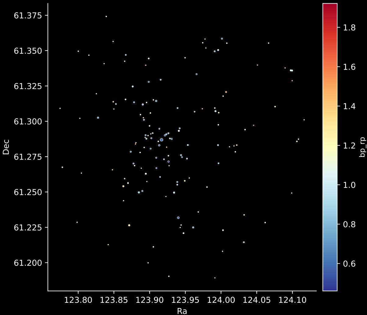
Gaia Cluster: [Trumpler_1] Stars: 142
