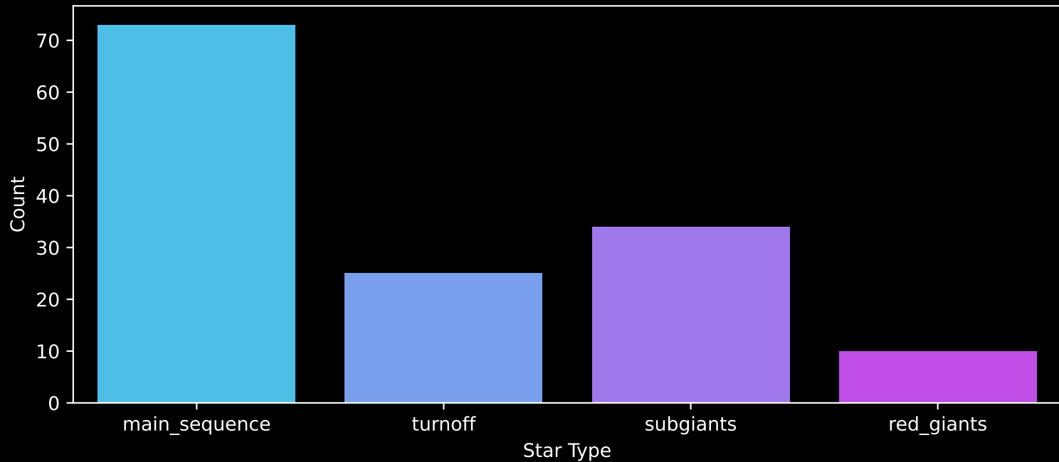
Gaia Cluster: [Trumpler_1] Count plot of Star Type
