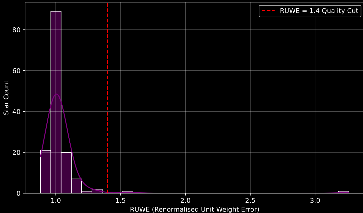
Gaia Cluster: [Trumpler_1] RUWE Distribution (n= 142)
