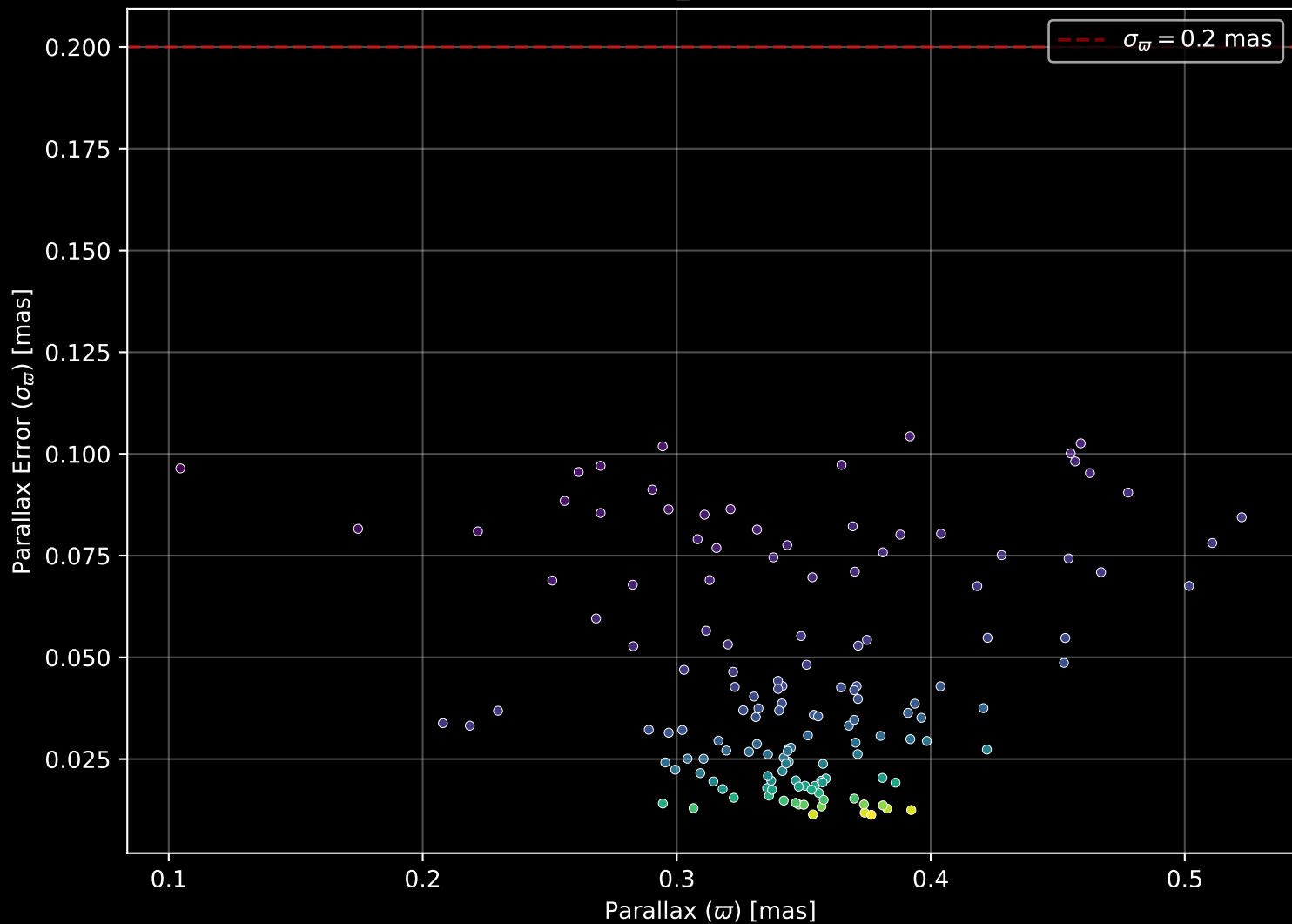
Gaia Cluster: [Trumpler_1] Parallax Quality (n= 142)
