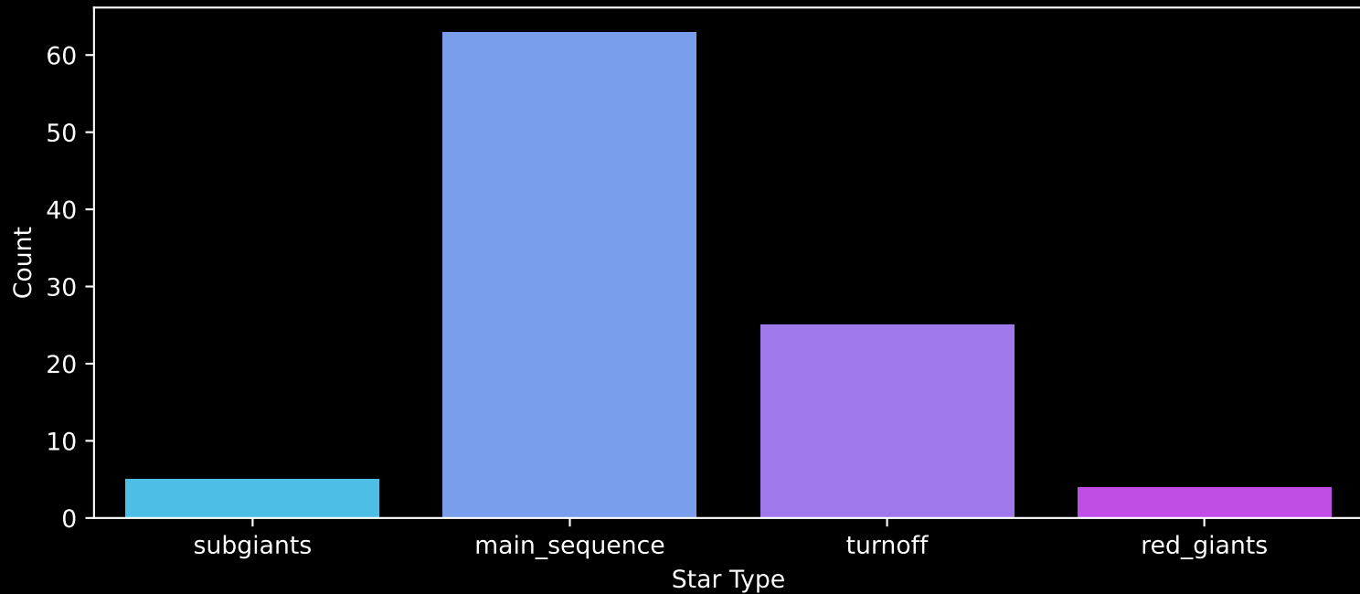
Gaia Cluster: [Trumpler_18] Count plot of Star Type
