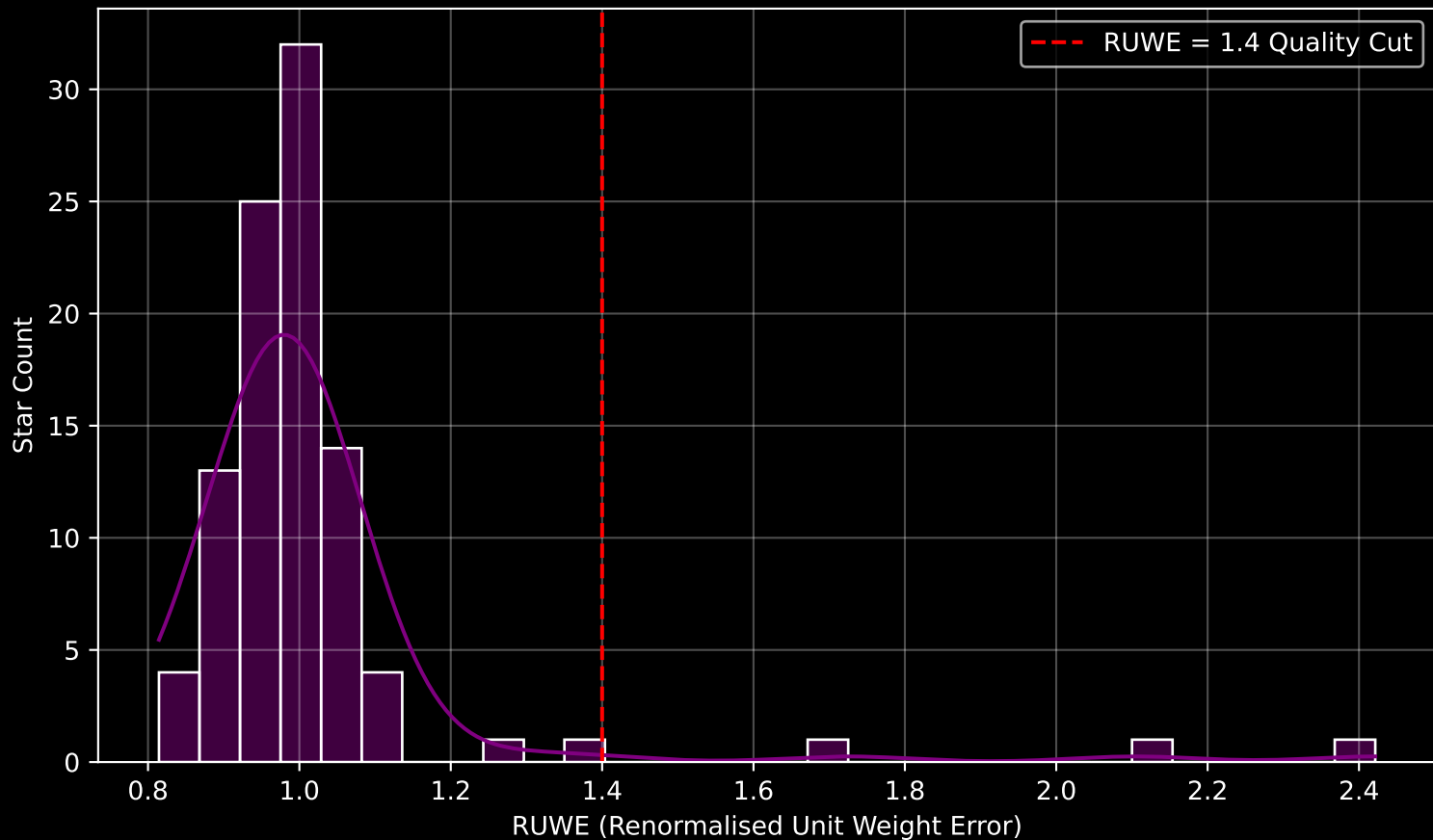
Gaia Cluster: [Trumpler_18] RUWE Distribution (n= 97)
