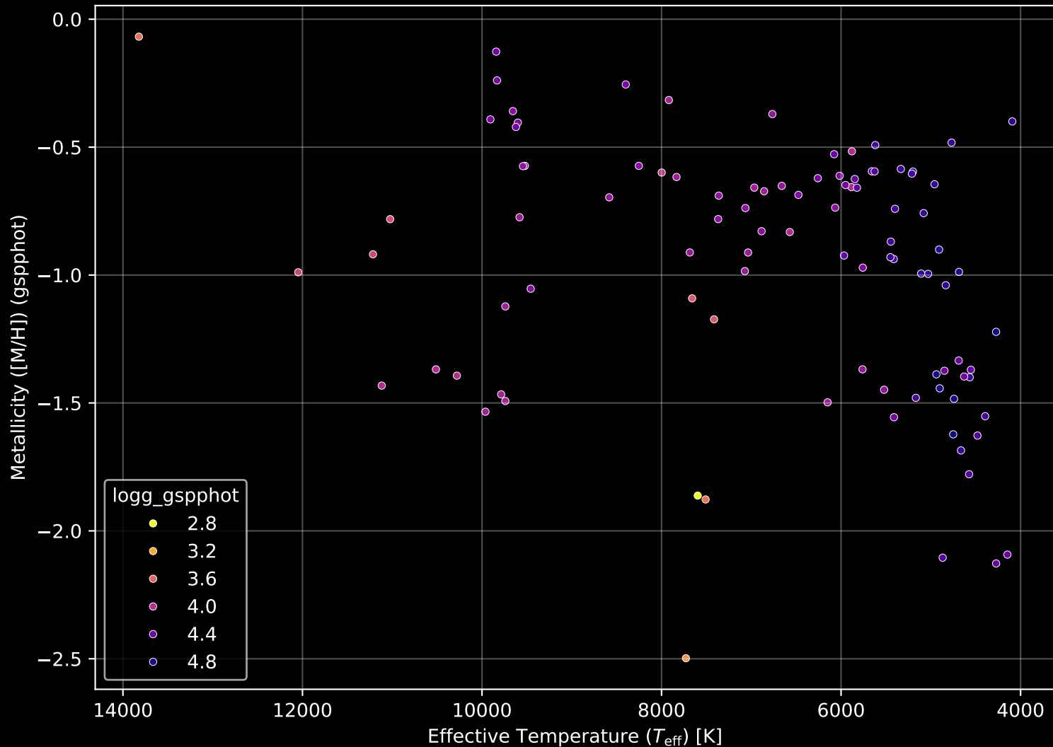
Gaia Cluster: [Trumpler_18] Stellar Population Parameters (n= 97)
