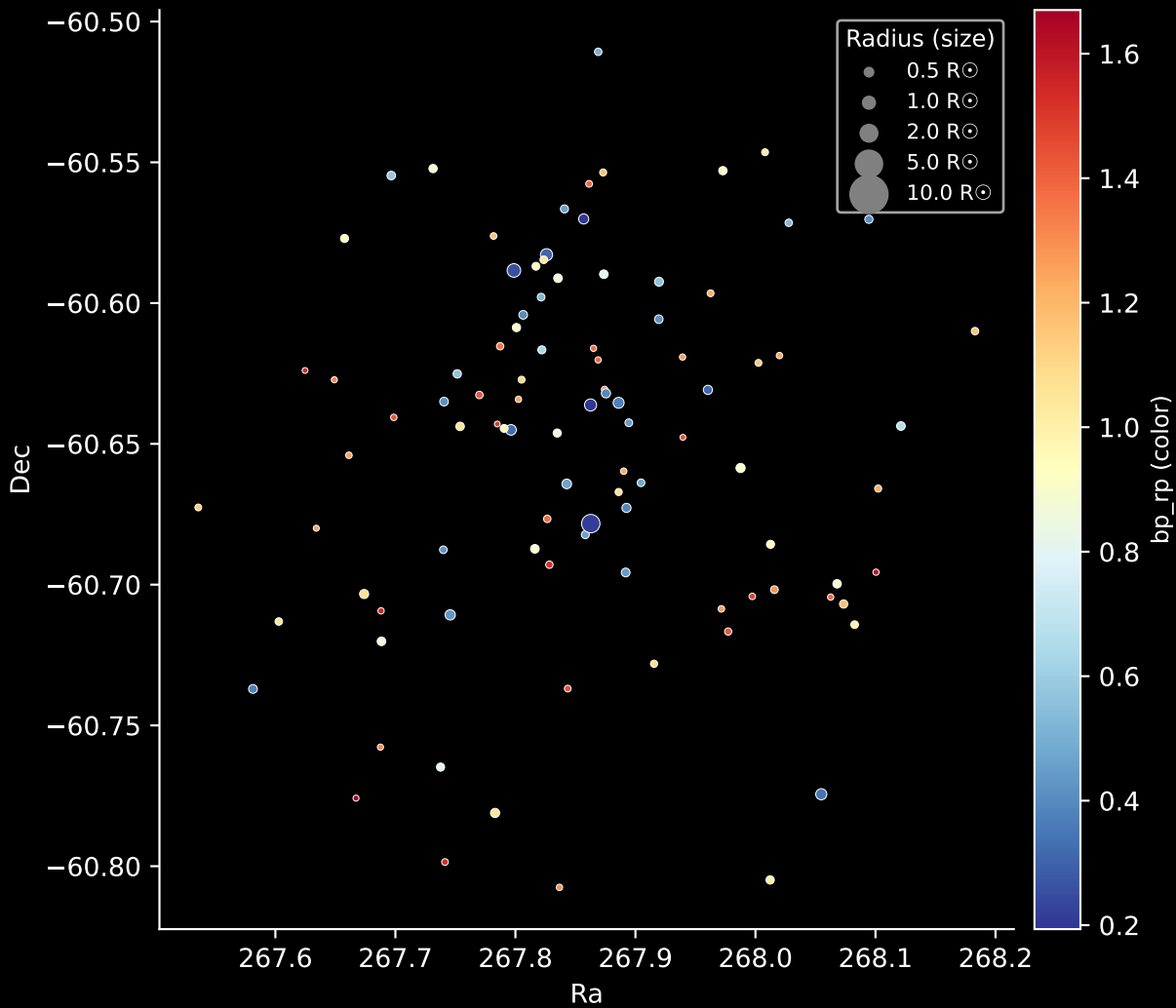
Gaia Cluster: [Trumpler_18] Stars: 97
