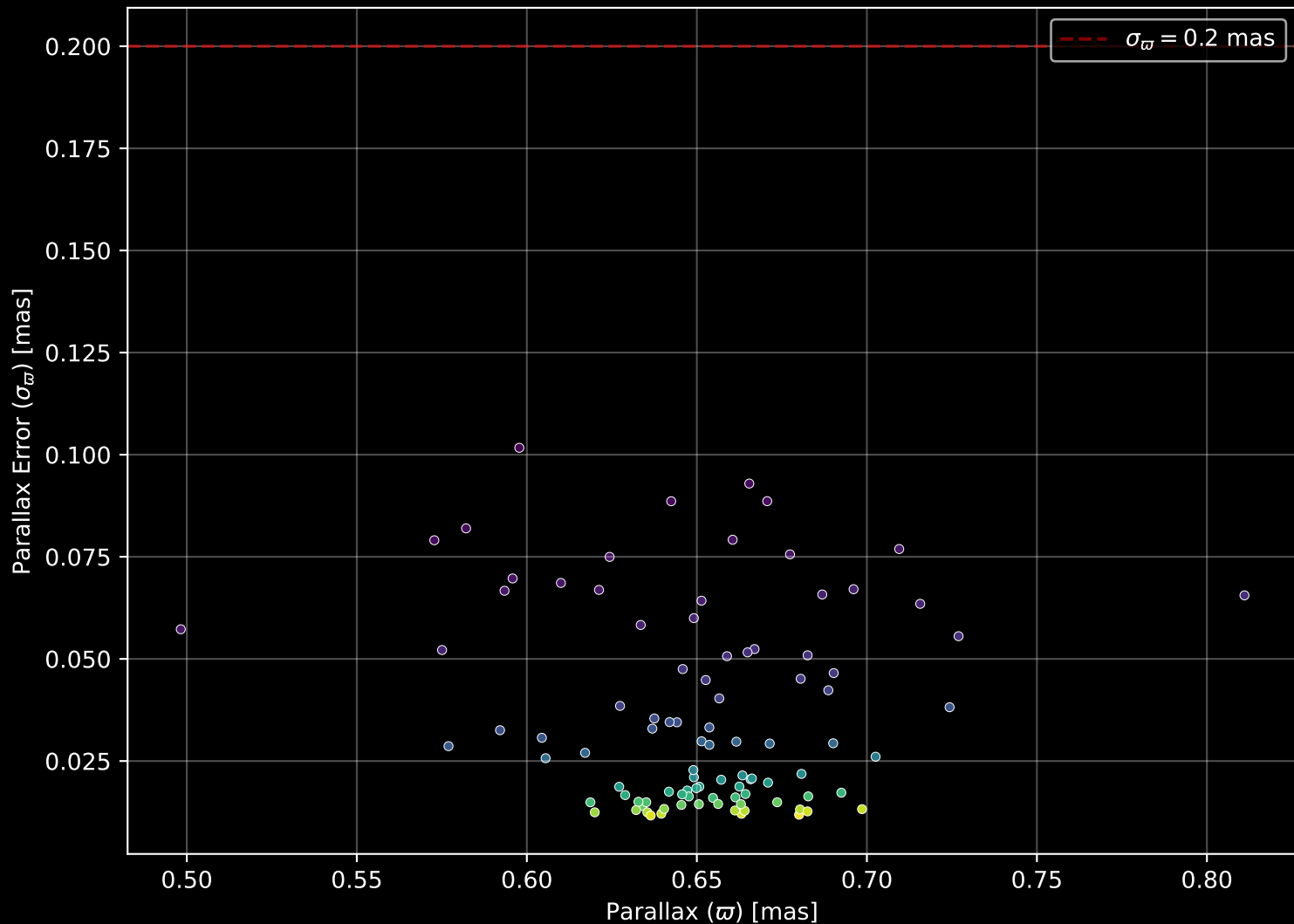
Gaia Cluster: [Trumpler_18] Parallax Quality (n= 97)
