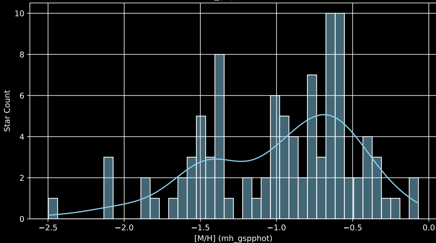
Gaia Cluster: [Trumpler_18 [M/H] (mh_gspphot) (n= 97)
