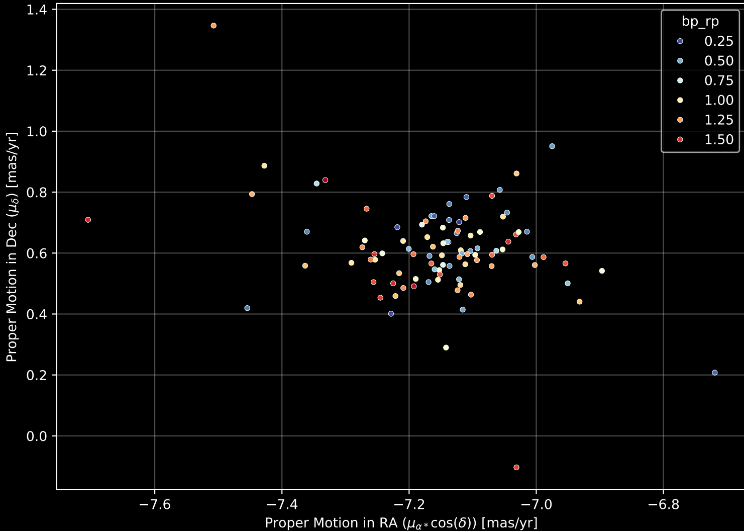
Gaia Cluster: [Trumpler_18] Proper Motion Diagram (n= 97)
