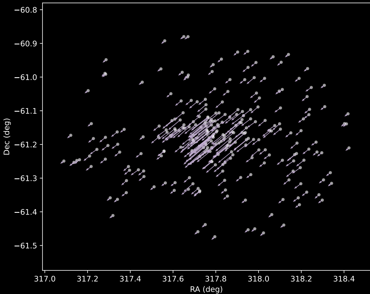
Gaia DR3 Cluster 9 Proper Motion Vectors (n=258)
