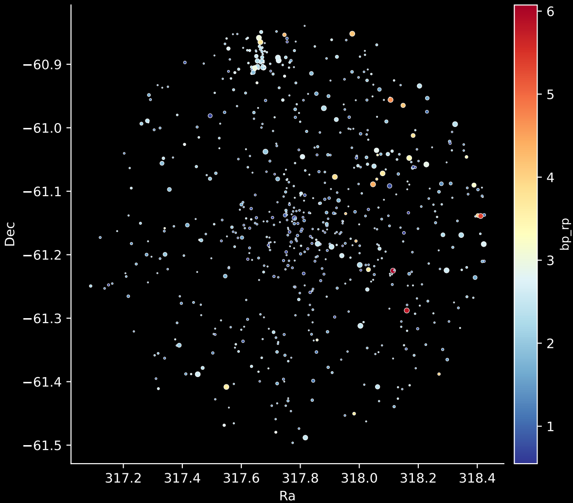
Gaia Cluster: [Trumpler_22] Stars: 692
