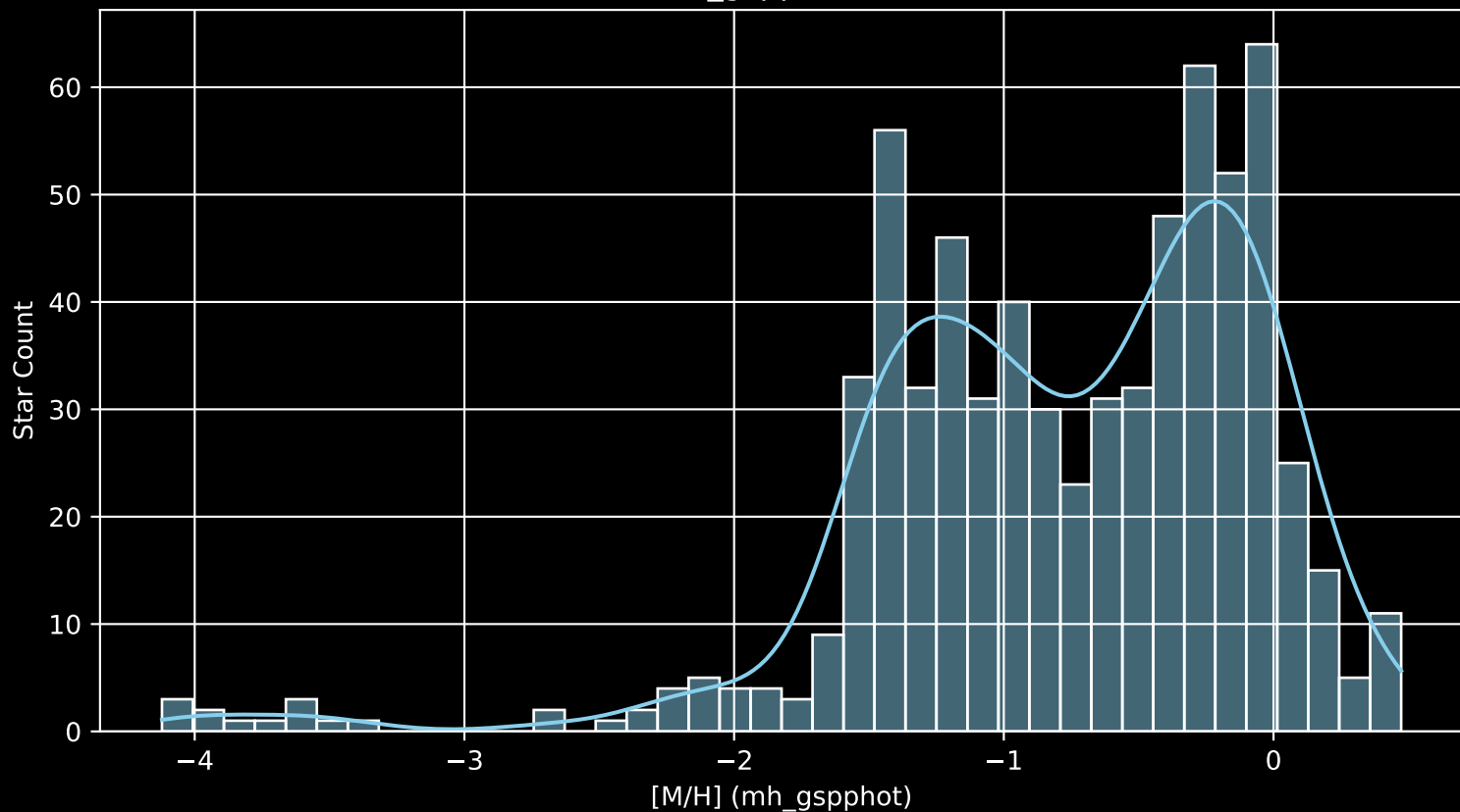
Gaia Cluster: [Trumpler_22 [M/H] (mh_gspphot) (n= 682)
