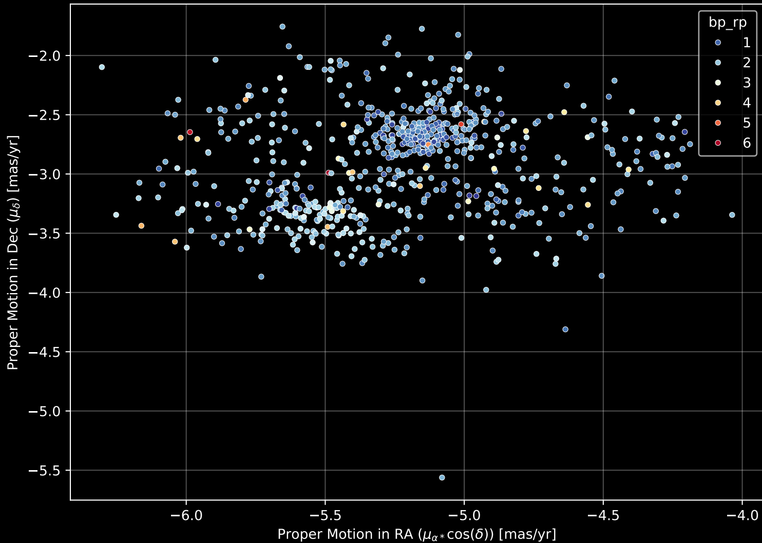
Gaia Cluster: [Trumpler_22] Proper Motion Diagram (n= 692)
