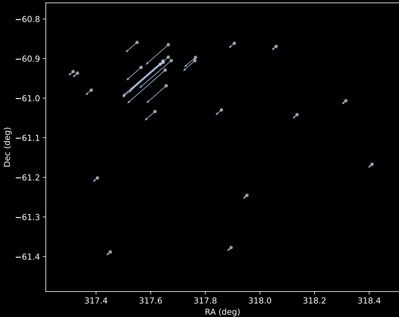
Gaia DR3 Cluster 21 Proper Motion Vectors (n=26)
