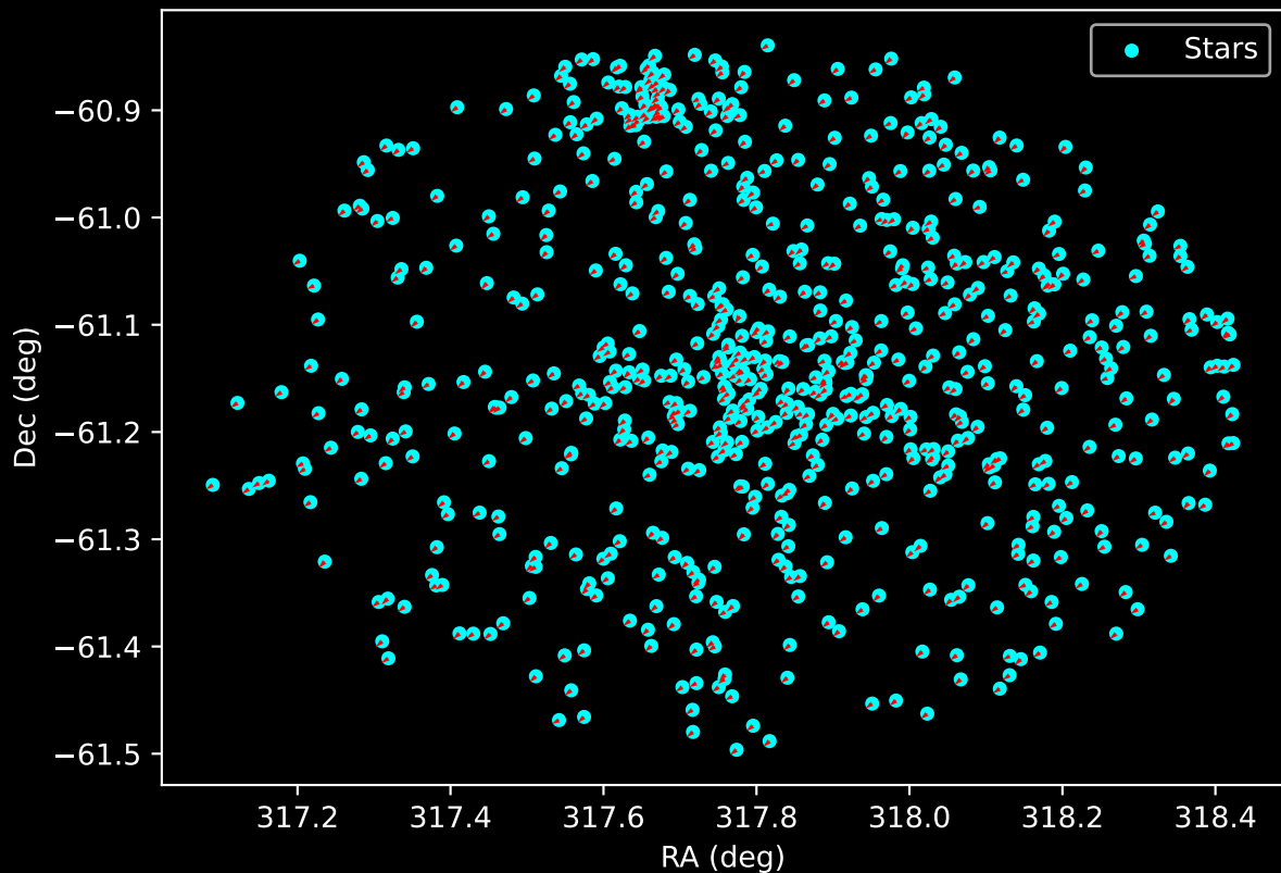
Gaia Cluster: [Trumpler_22] Proper Motion Vectors for Gaia Star Field (n= 692)
