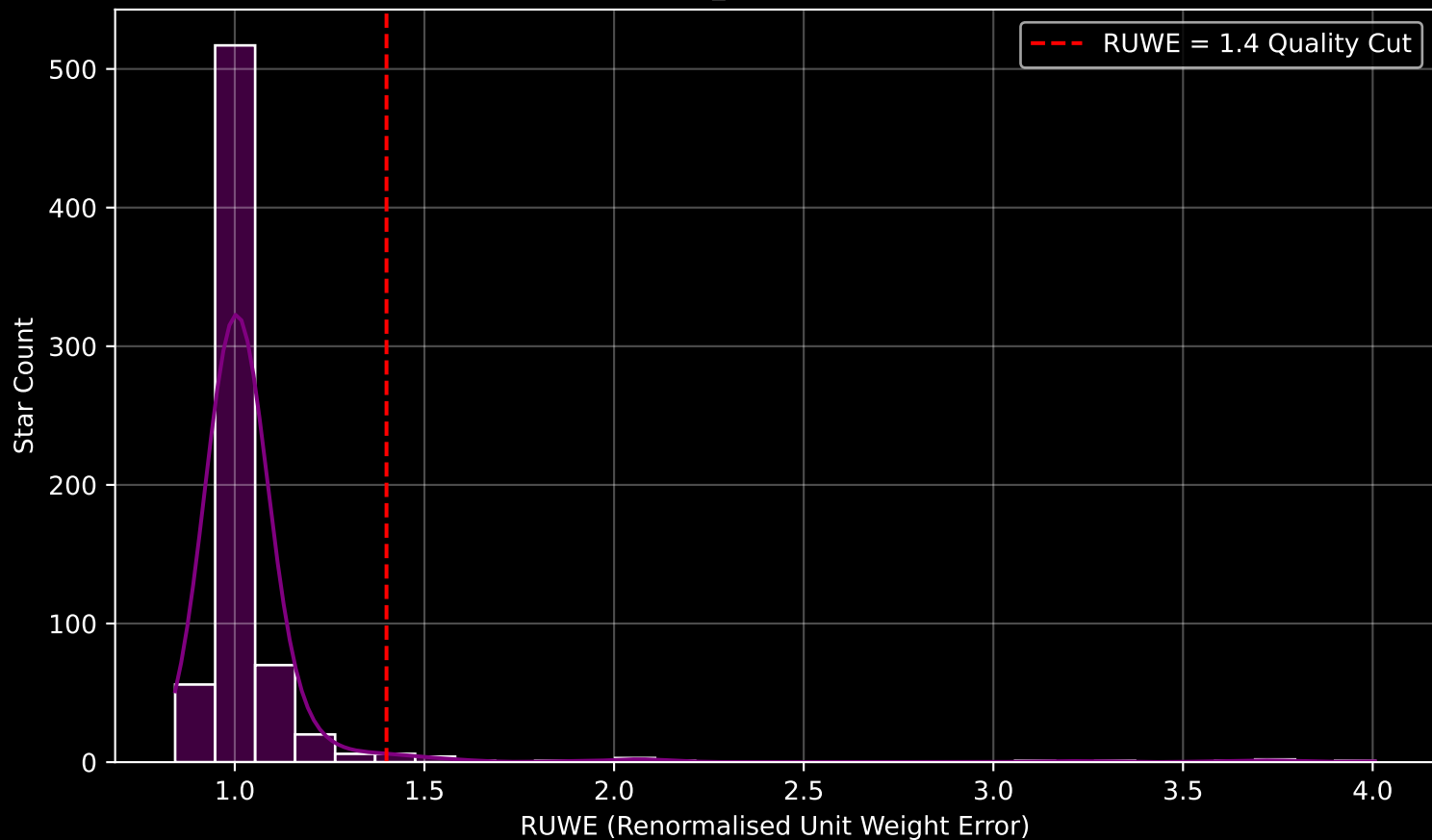
Gaia Cluster: [Trumpler_22] RUWE Distribution (n= 691)
