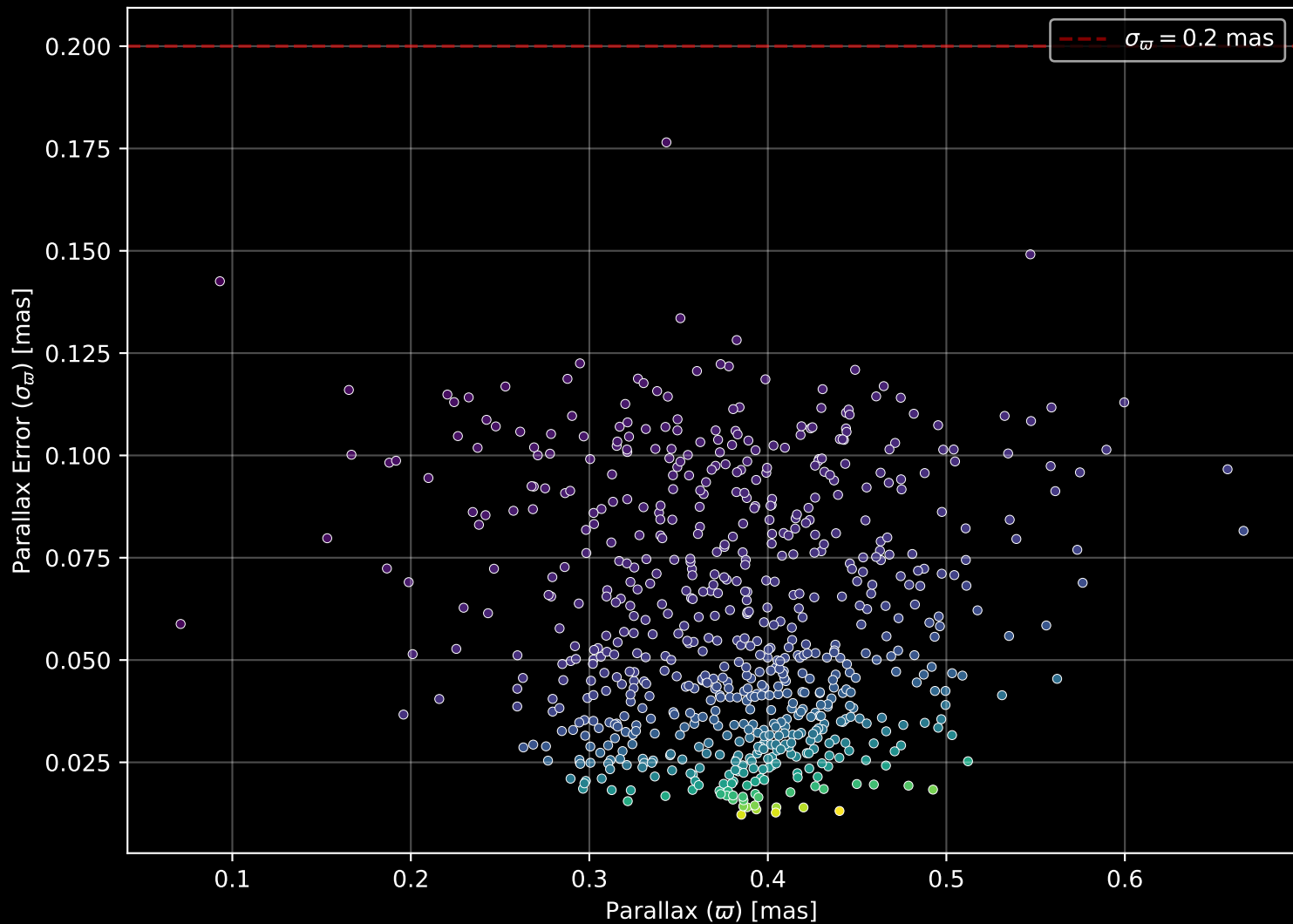
Gaia Cluster: [Trumpler_22] Parallax Quality (n= 692)
