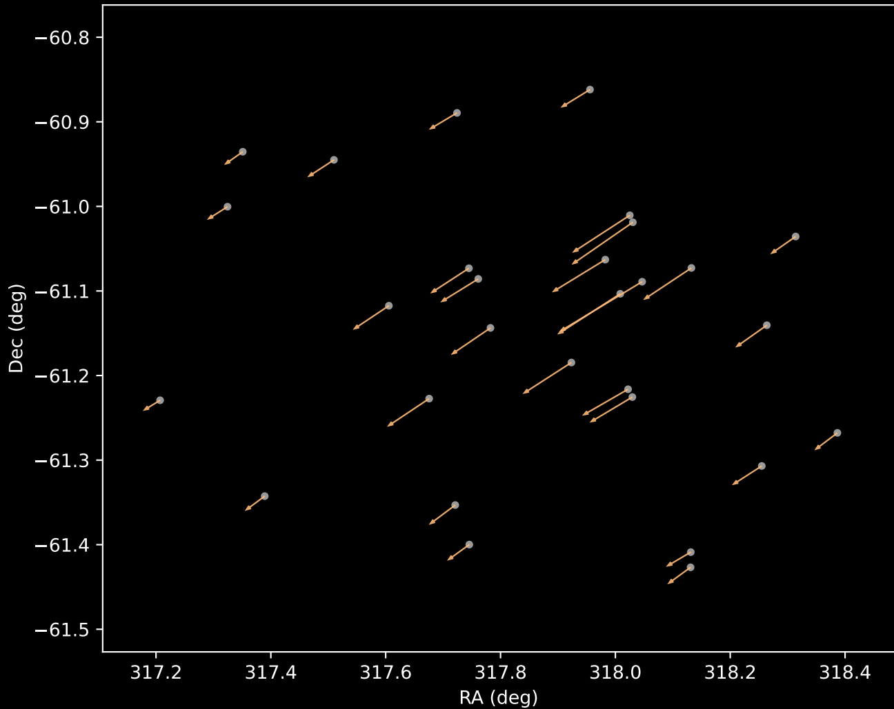
Gaia DR3 Cluster 3 Proper Motion Vectors (n=29)
