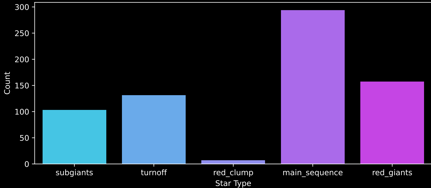
Gaia Cluster: [Trumpler_22] Count plot of Star Type
