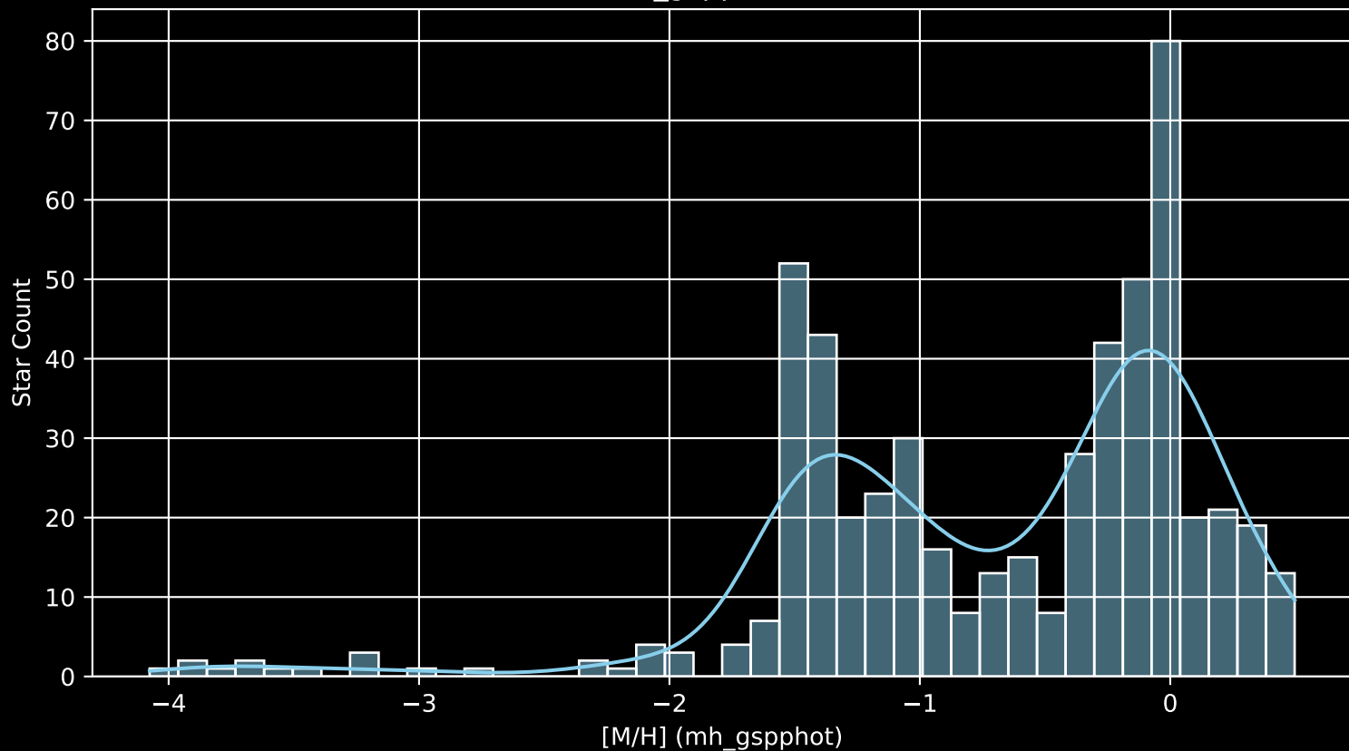
Gaia Cluster: [Trumpler_23 [M/H] (mh_gspphot) (n= 535)
