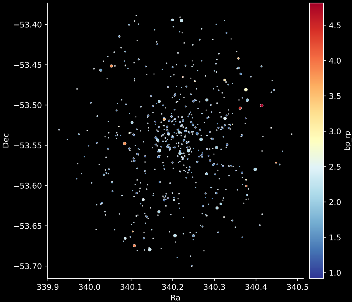
Gaia Cluster: [Trumpler_23] Stars: 554
