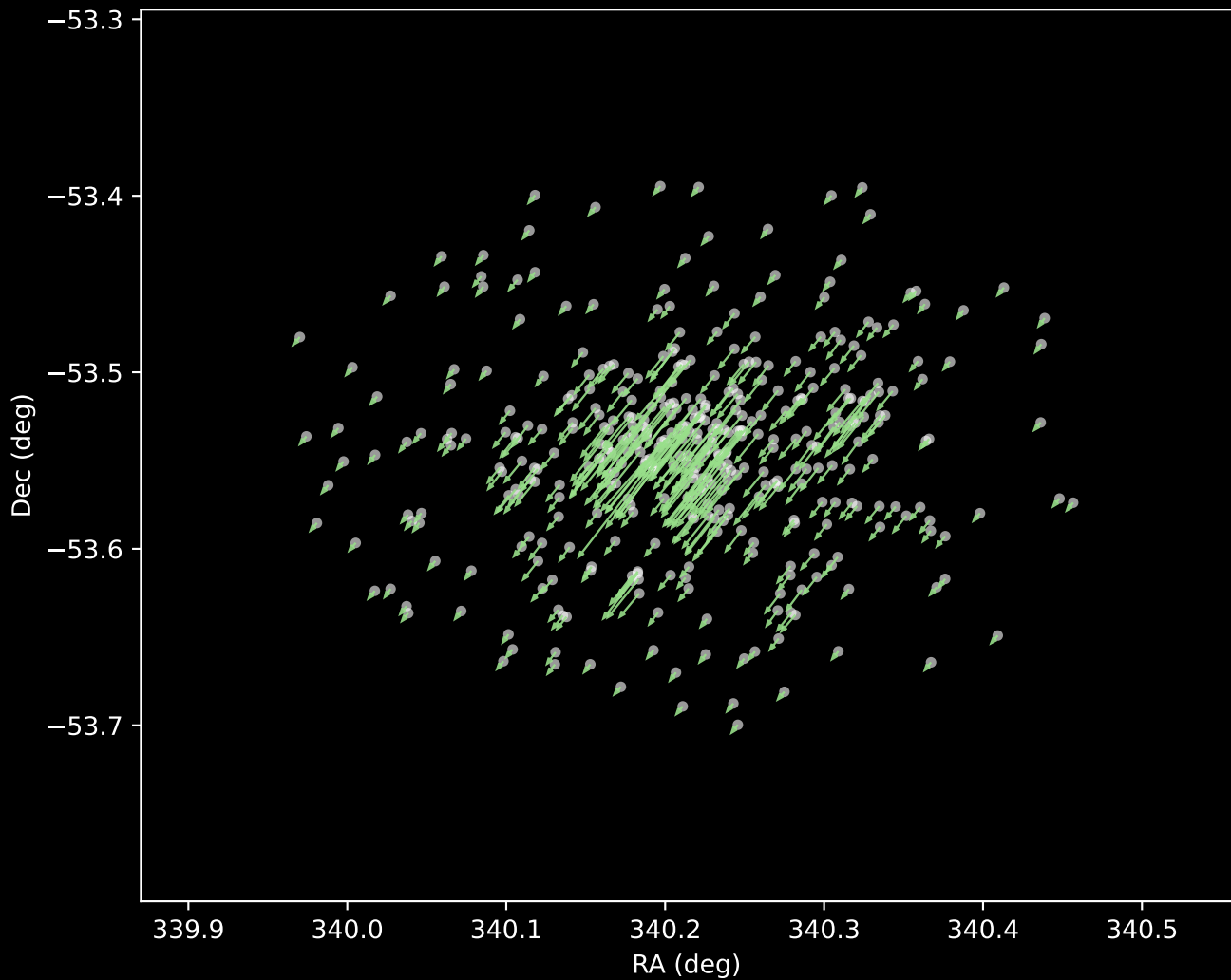
Gaia DR3 Cluster 5 Proper Motion Vectors (n=397)
