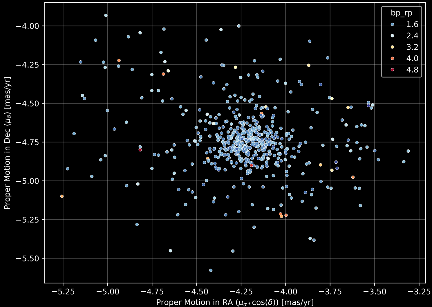
Gaia Cluster: [Trumpler_23] Proper Motion Diagram (n= 554)
