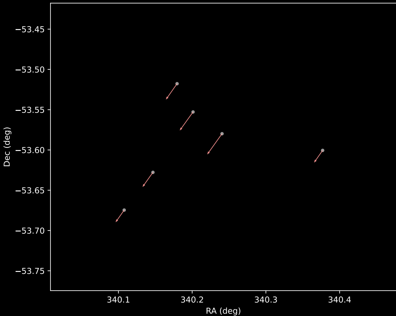
Gaia DR3 Cluster 7 Proper Motion Vectors (n=6)
