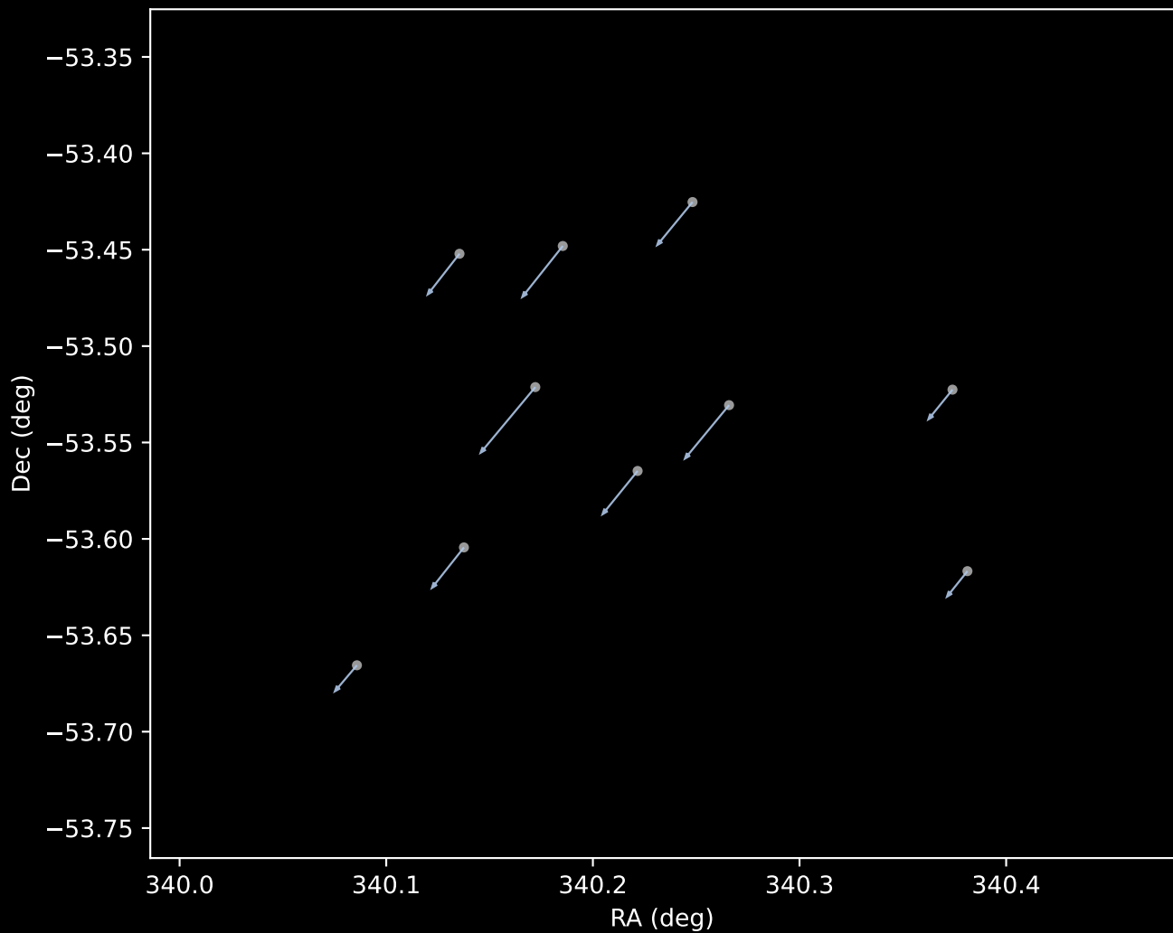
Gaia DR3 Cluster 1 Proper Motion Vectors (n=10)
