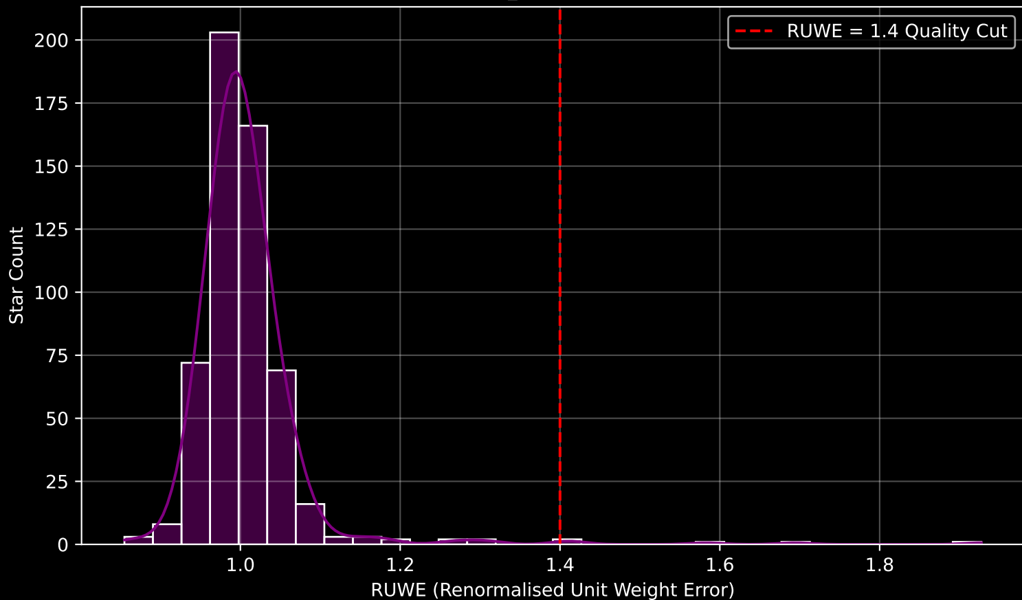
Gaia Cluster: [Trumpler_23] RUWE Distribution (n= 554)
