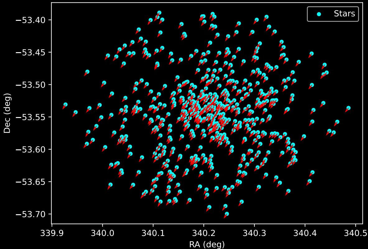
Gaia Cluster: [Trumpler_23] Proper Motion Vectors for Gaia Star Field (n= 554)
