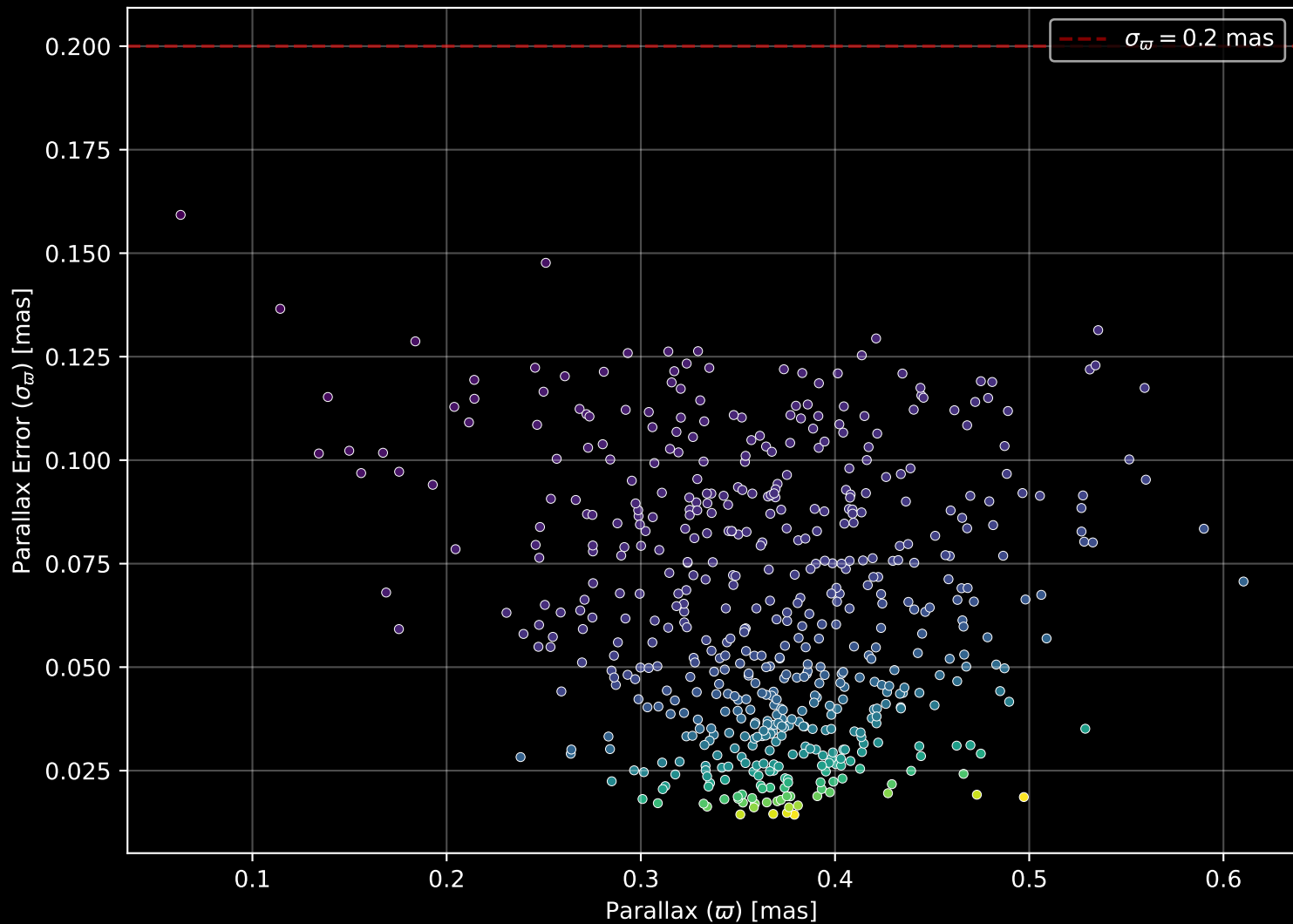
Gaia Cluster: [Trumpler_23] Parallax Quality (n= 554)
