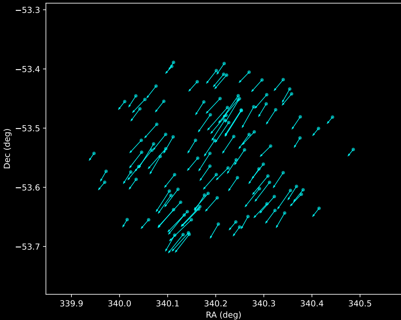
Gaia DR3 Noise Stream Proper Motion Vectors (n=107)
