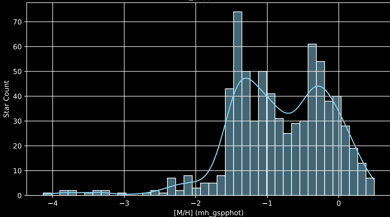
Gaia Cluster: [Trumpler_25 [M/H] (mh_gspphot) (n= 716)
