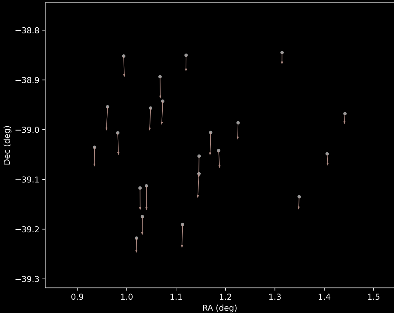
Gaia DR3 Cluster 11 Proper Motion Vectors (n=22)
