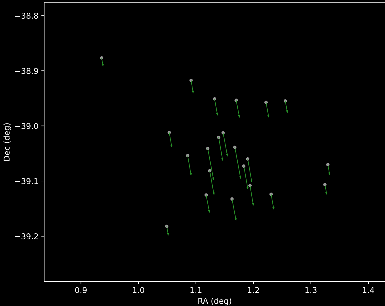
Gaia DR3 Cluster 24 Proper Motion Vectors (n=22)
