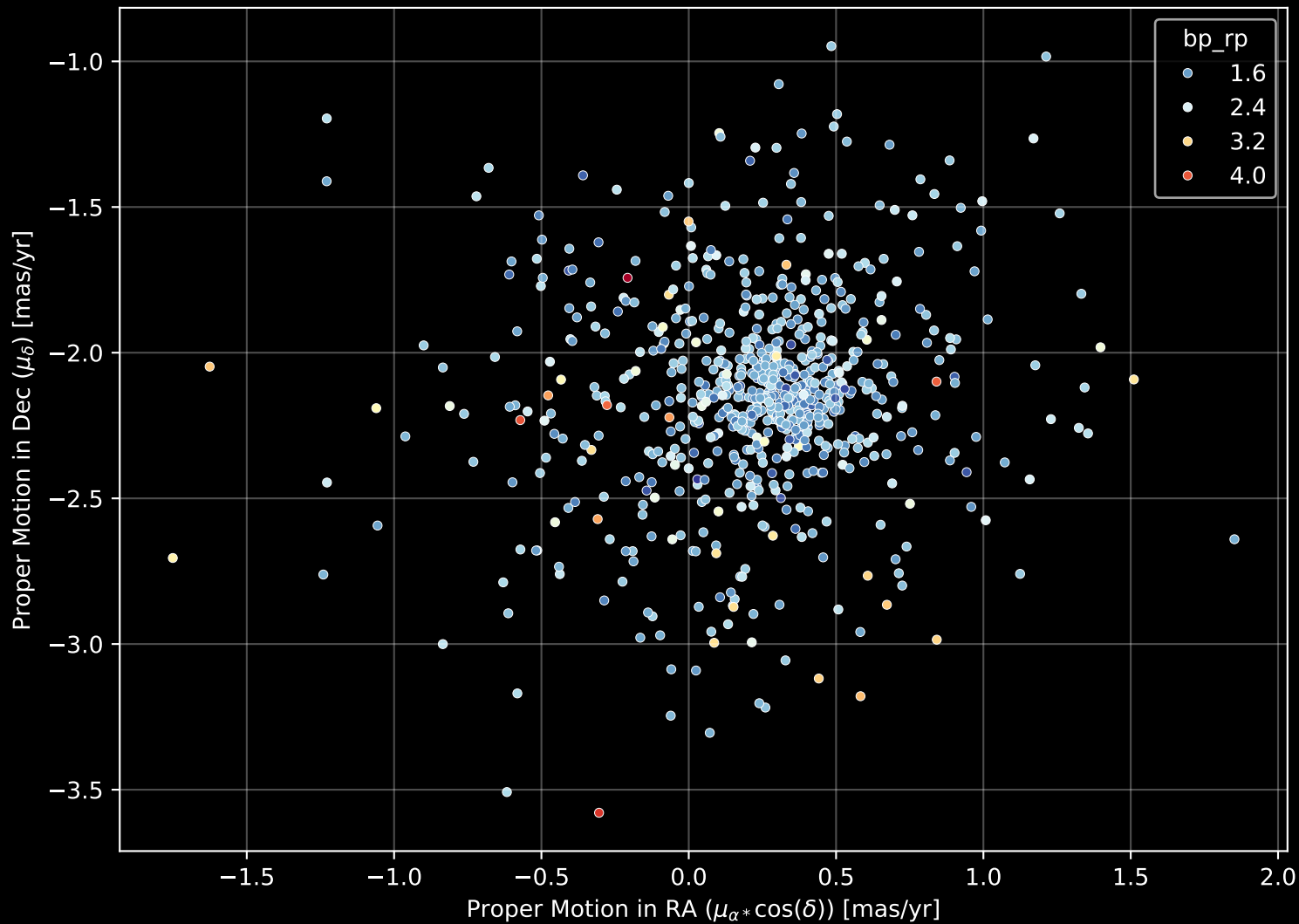
Gaia Cluster: [Trumpler_25] Proper Motion Diagram (n= 731)
