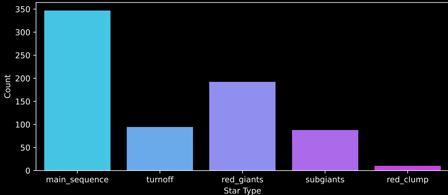
Gaia Cluster: [Trumpler_25] Count plot of Star Type
