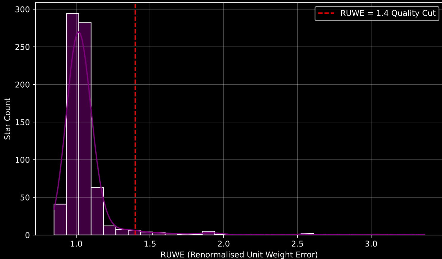
Gaia Cluster: [Trumpler_25] RUWE Distribution (n= 730)
