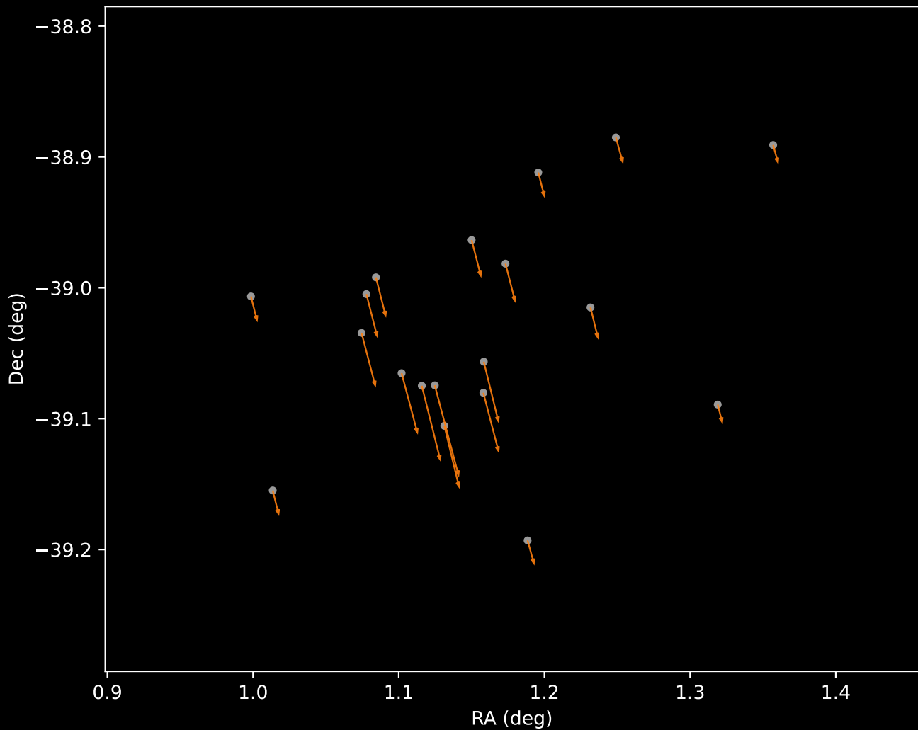
Gaia DR3 Cluster 22 Proper Motion Vectors (n=19)
