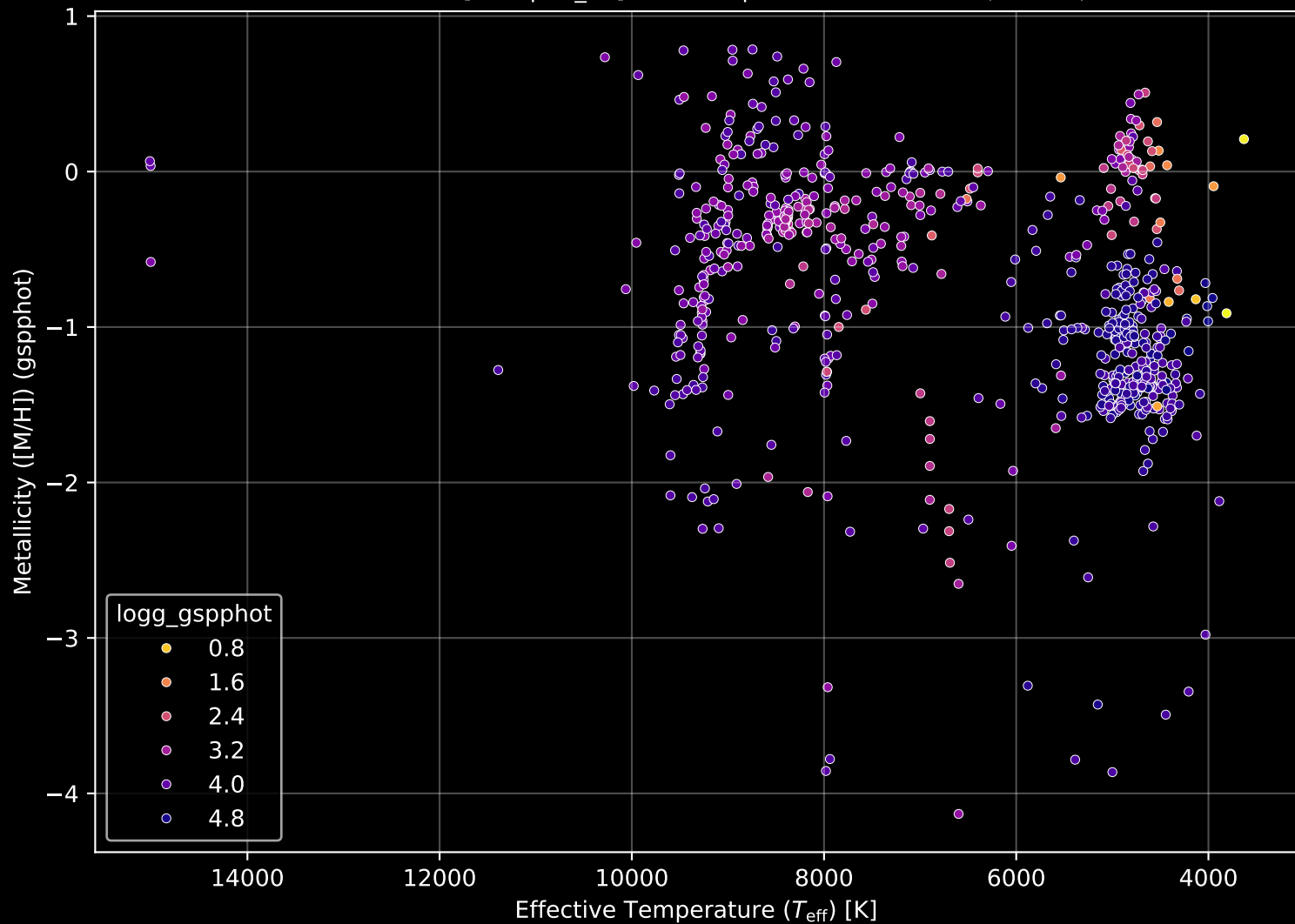
Gaia Cluster: [Trumpler_25] Stellar Population Parameters (n= 731)
