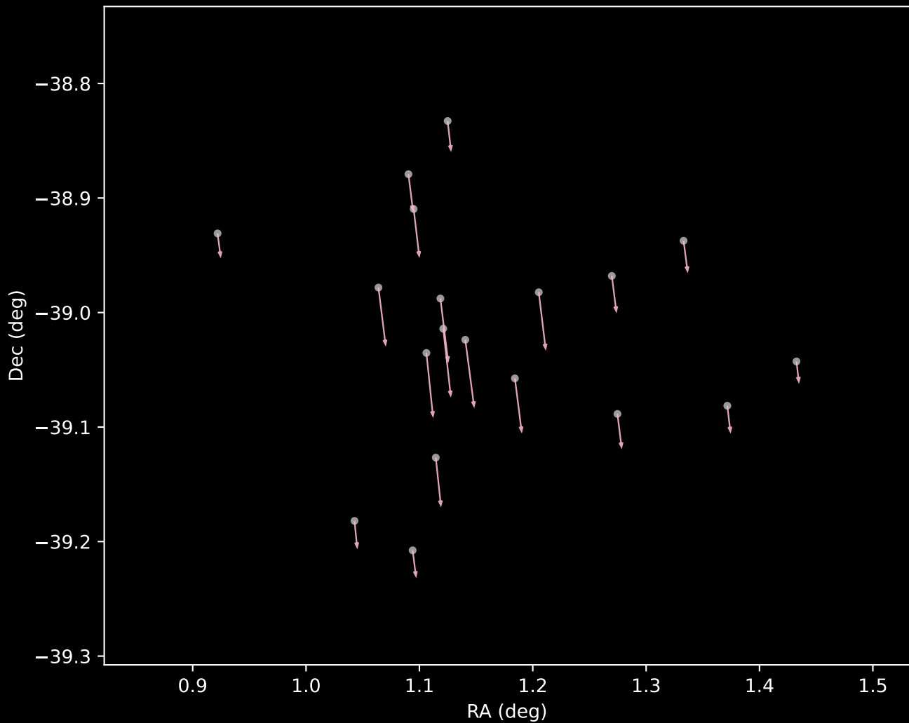
Gaia DR3 Cluster 33 Proper Motion Vectors (n=19)
