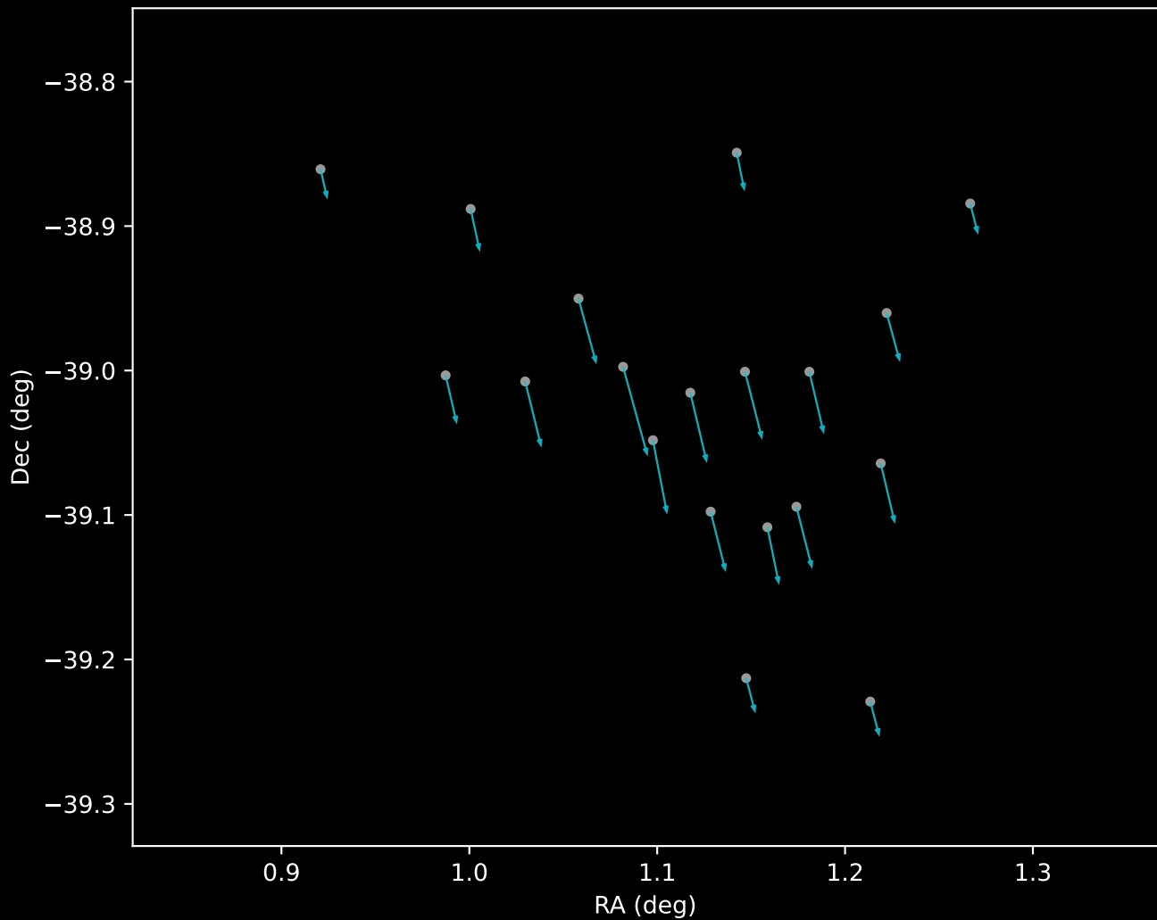
Gaia DR3 Cluster 18 Proper Motion Vectors (n=19)
