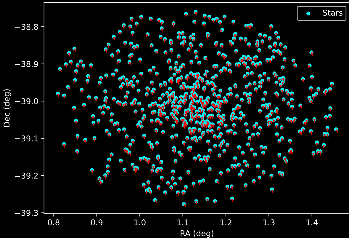
Gaia Cluster: [Trumpler_25] Proper Motion Vectors for Gaia Star Field (n= 731)
