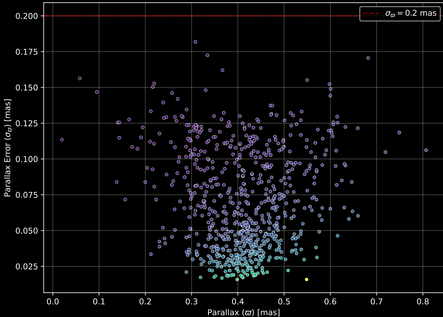
Gaia Cluster: [Trumpler_25] Parallax Quality (n= 731)
