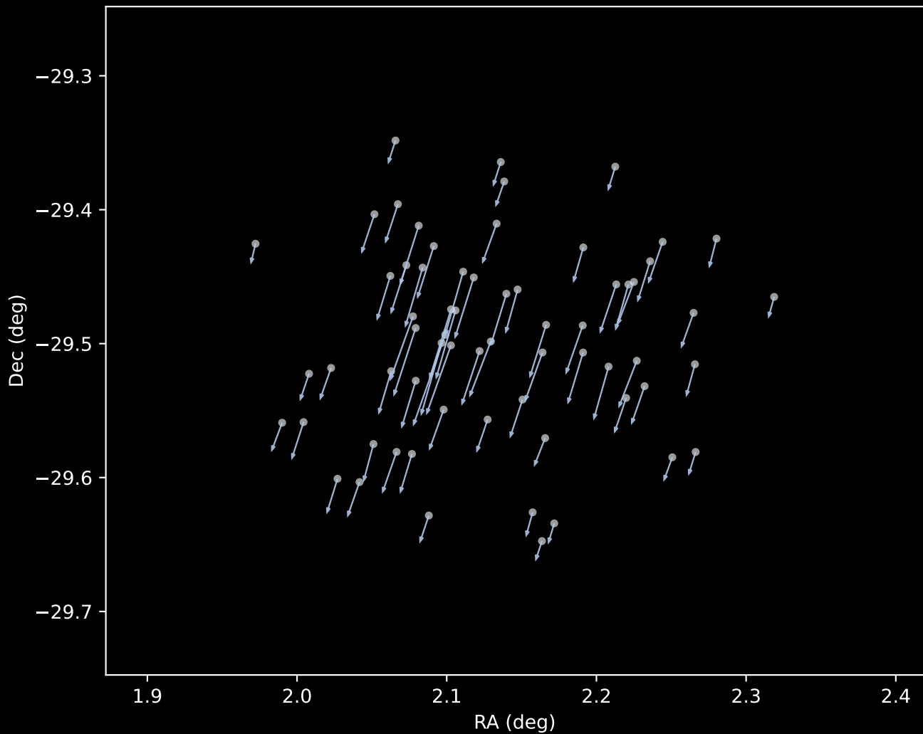
Gaia DR3 Cluster 1 Proper Motion Vectors (n=65)
