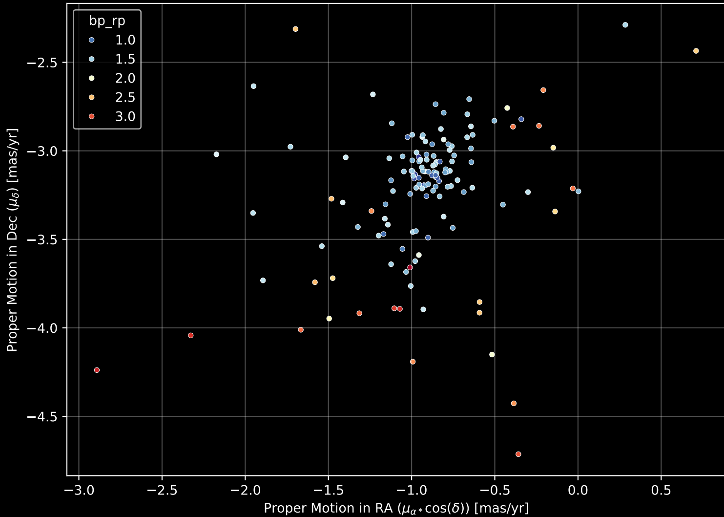
Gaia Cluster: [Trumpler_26] Proper Motion Diagram (n= 138)
