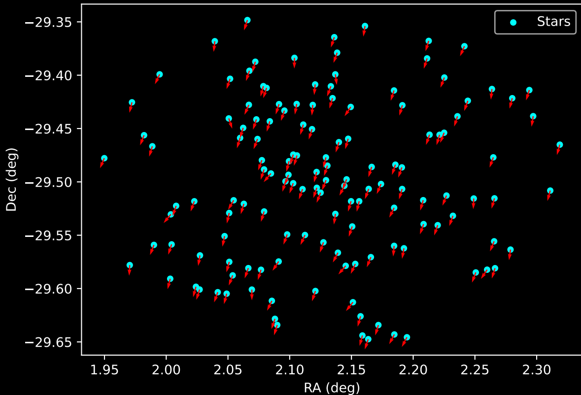
Gaia Cluster: [Trumpler_26] Proper Motion Vectors for Gaia Star Field (n= 138)
