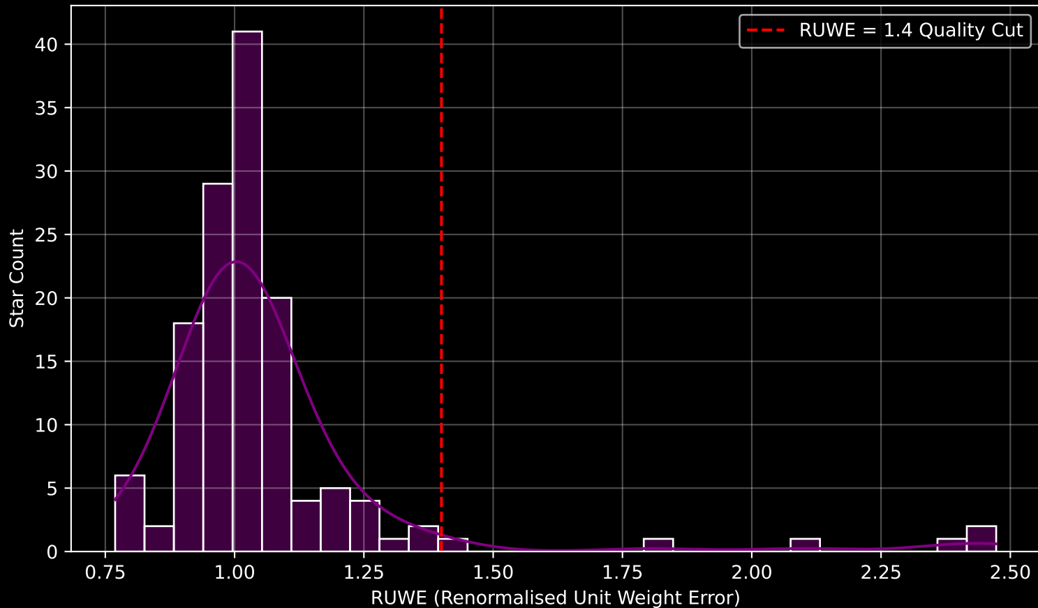
Gaia Cluster: [Trumpler_26] RUWE Distribution (n= 138)
