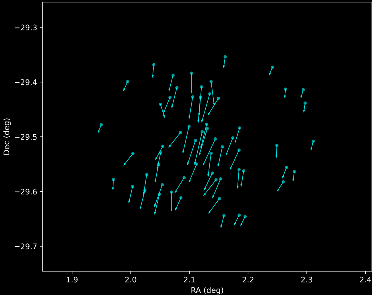
Gaia DR3 Noise Stream Proper Motion Vectors (n=59)
