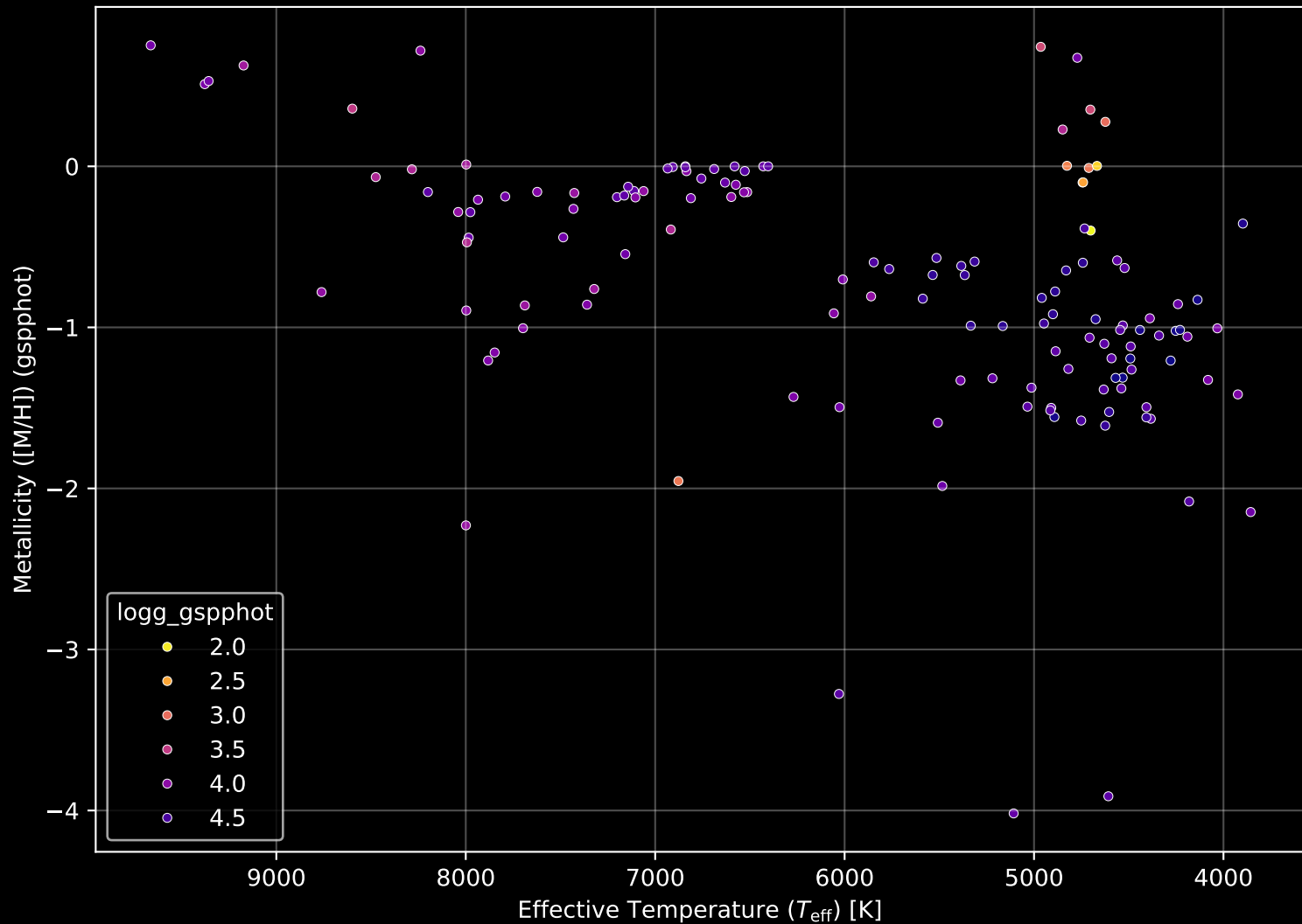
Gaia Cluster: [Trumpler_26] Stellar Population Parameters (n= 138)
