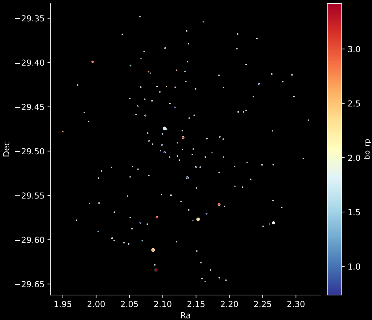
Gaia Cluster: [Trumpler_26] Stars: 138
