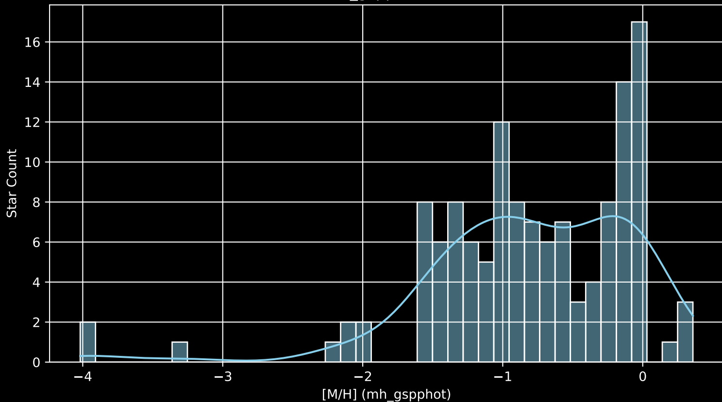
Gaia Cluster: [Trumpler_26 [M/H] (mh_gspphot) (n= 131)
