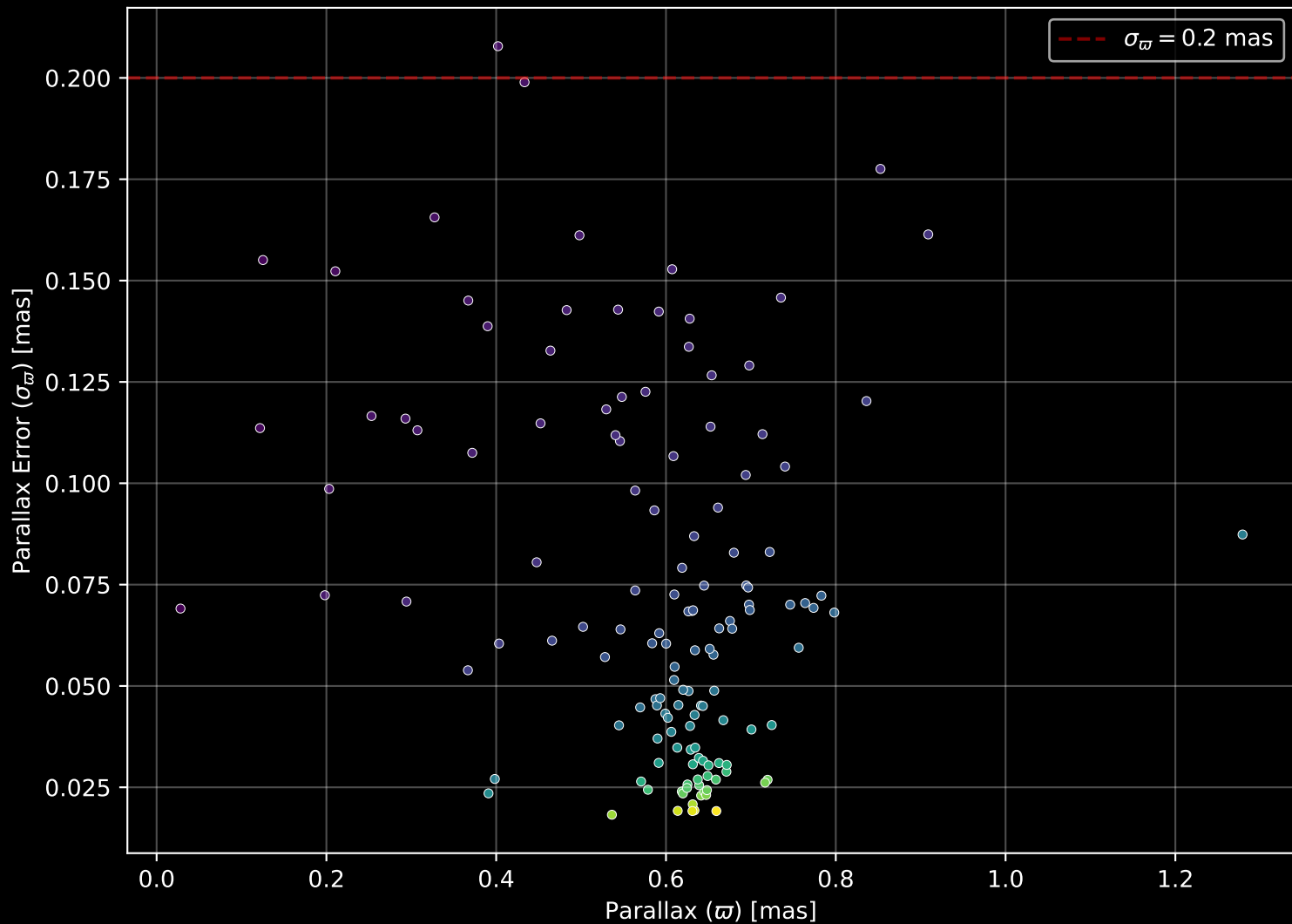
Gaia Cluster: [Trumpler_26] Parallax Quality (n= 138)
