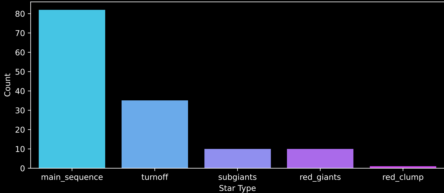
Gaia Cluster: [Trumpler_26] Count plot of Star Type
