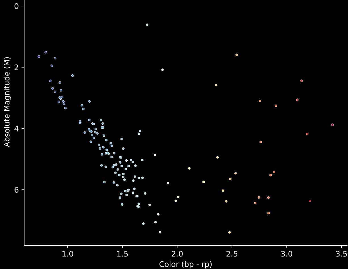
Gaia Cluster: [Trumpler_26] Stars (n= 138) Hertzsprung-Russel Diagram
