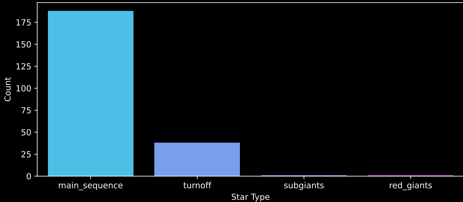
Gaia Cluster: [Trumpler_3] Count plot of Star Type
