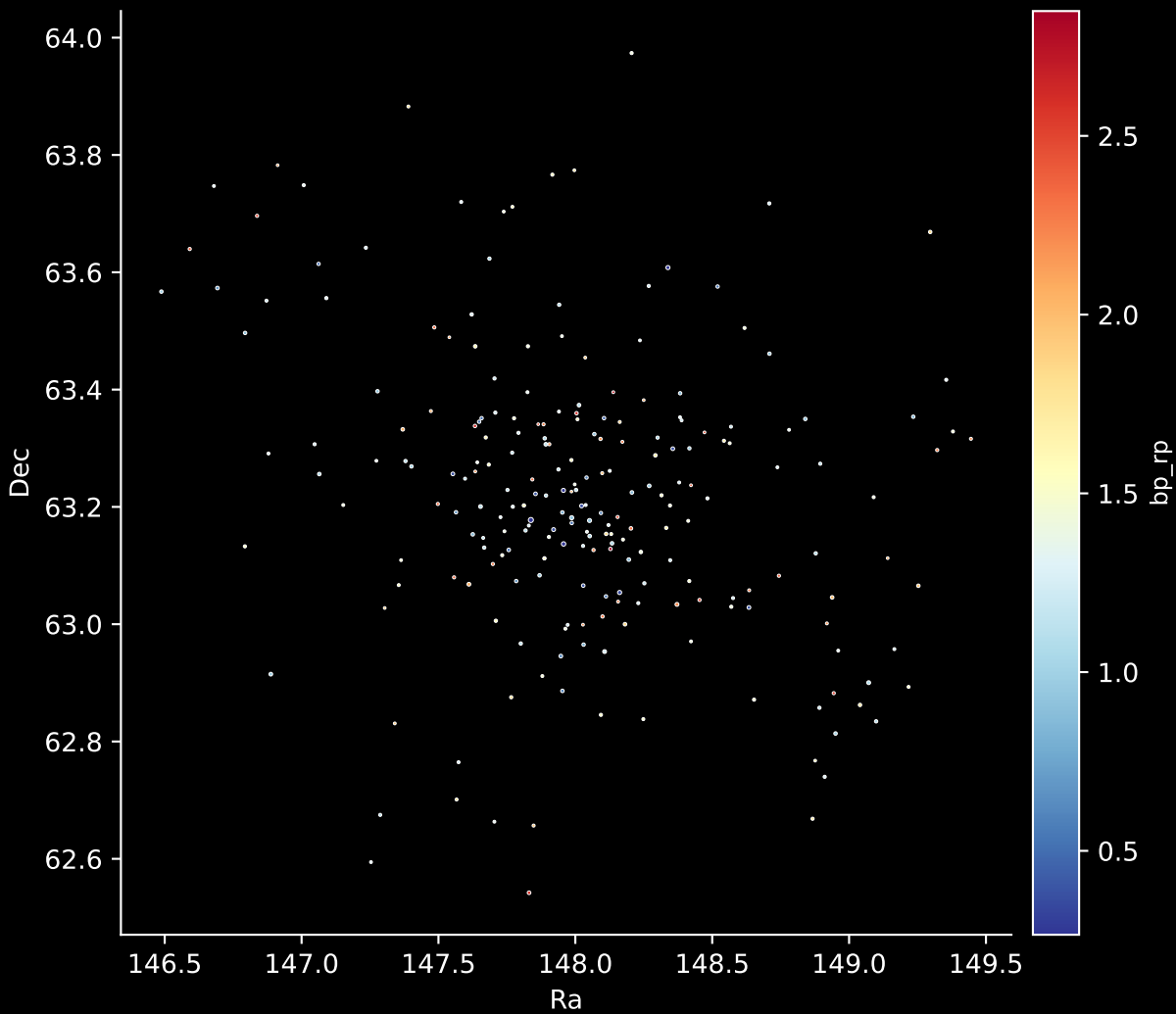
Gaia Cluster: [Trumpler_3] Stars: 228
