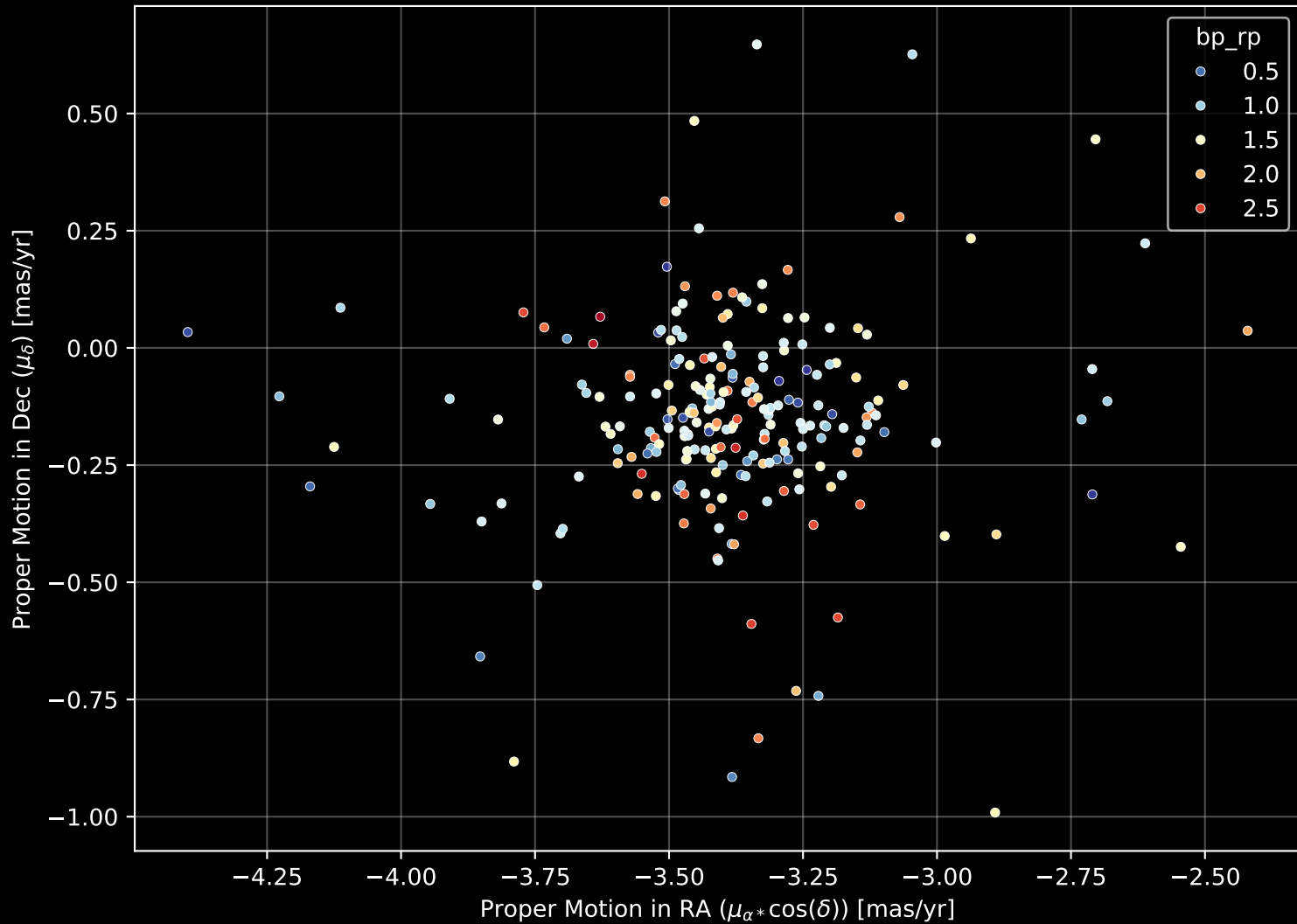
Gaia Cluster: [Trumpler_3] Proper Motion Diagram (n= 228)
