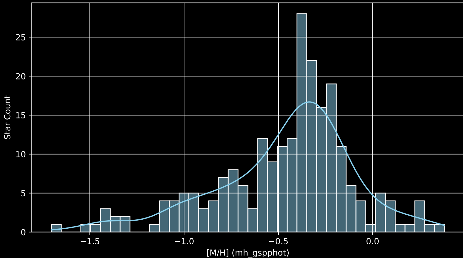
Gaia Cluster: [Trumpler_3 [M/H] (mh_gspphot) (n= 228)
