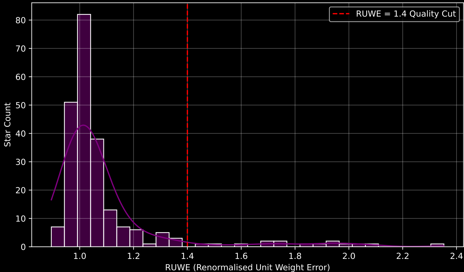
Gaia Cluster: [Trumpler_3] RUWE Distribution (n= 228)
