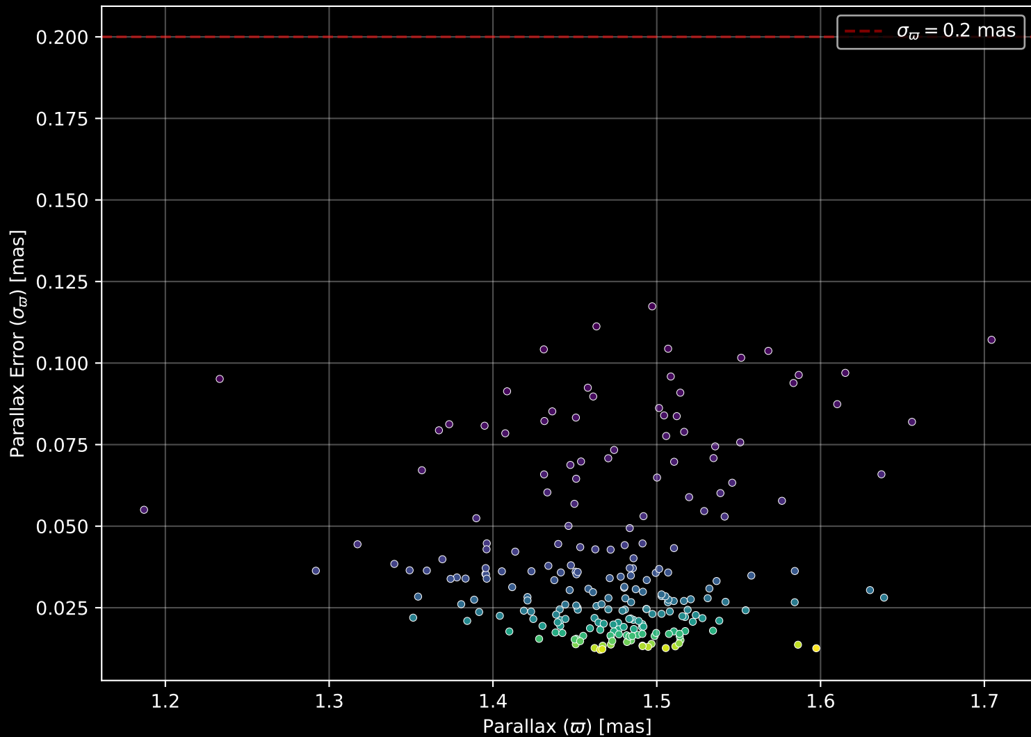
Gaia Cluster: [Trumpler_3] Parallax Quality (n= 228)
