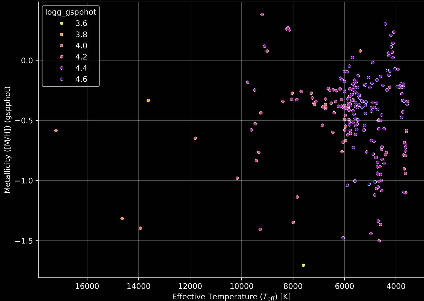
Gaia Cluster: [Trumpler_3] Stellar Population Parameters (n= 228)
