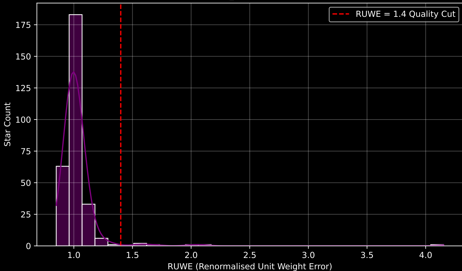
Gaia Cluster: [Trumpler_32] RUWE Distribution (n= 292)
