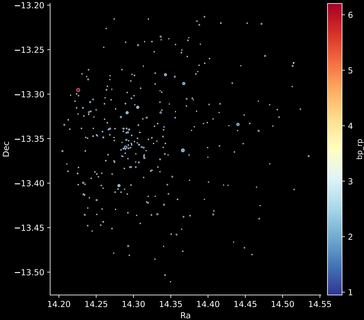
Gaia Cluster: [Trumpler_32] Stars: 292
