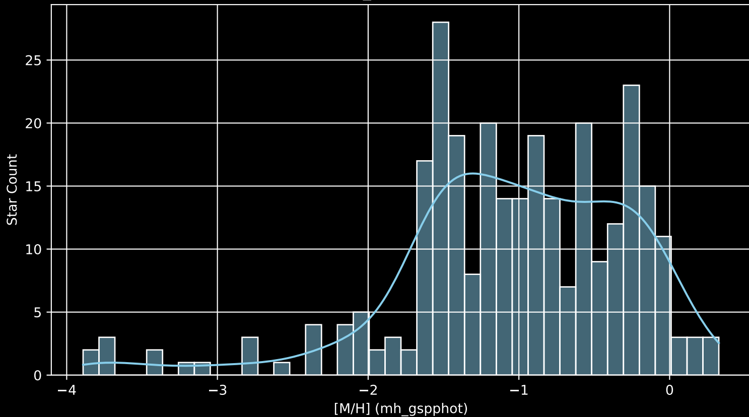
Gaia Cluster: [Trumpler_32 [M/H] (mh_gspphot) (n= 292)
