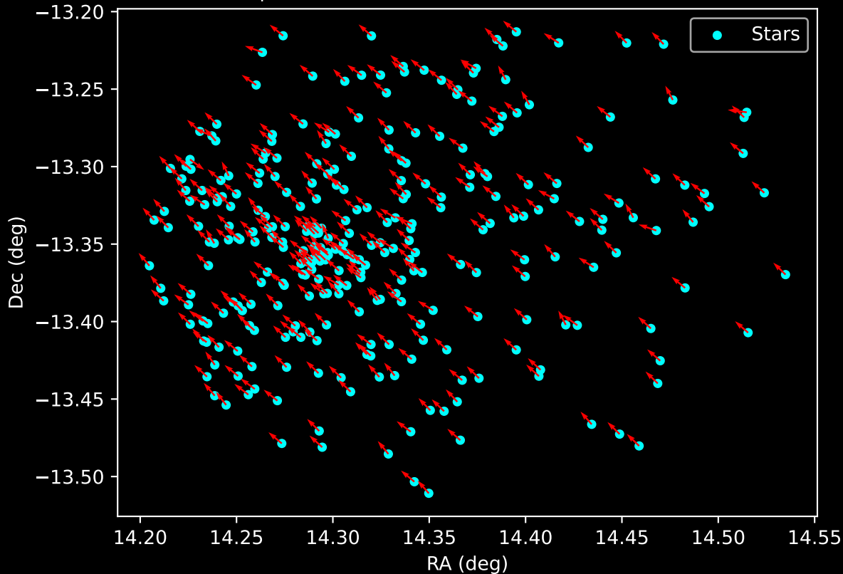
Gaia Cluster: [Trumpler_32] Proper Motion Vectors for Gaia Star Field (n= 292)
