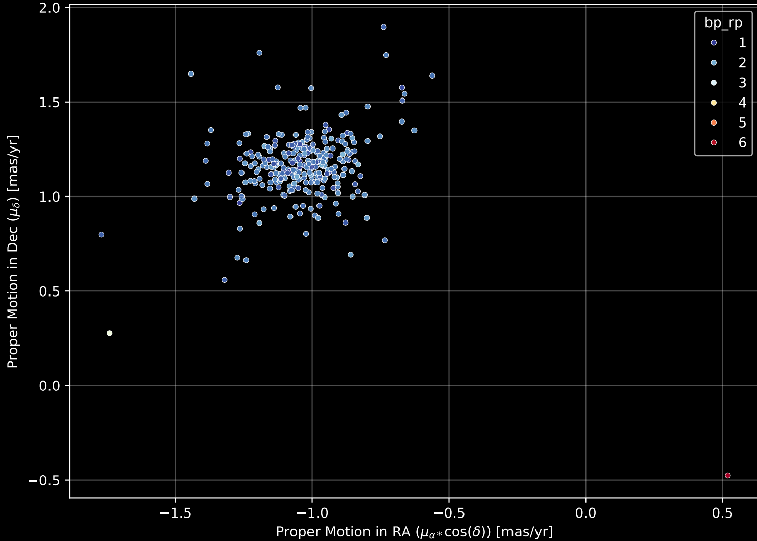
Gaia Cluster: [Trumpler_32] Proper Motion Diagram (n= 292)
