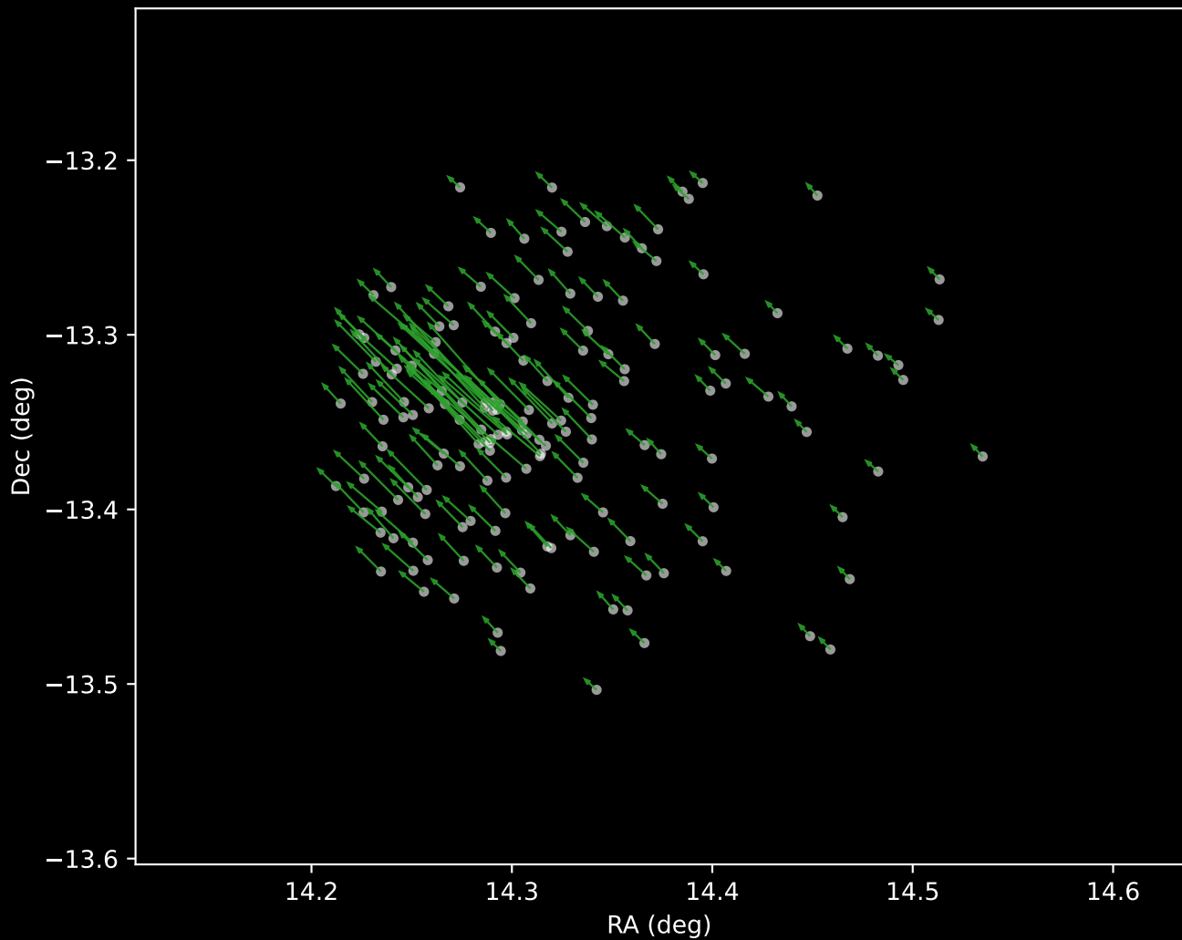
Gaia DR3 Cluster 4 Proper Motion Vectors (n=166)
