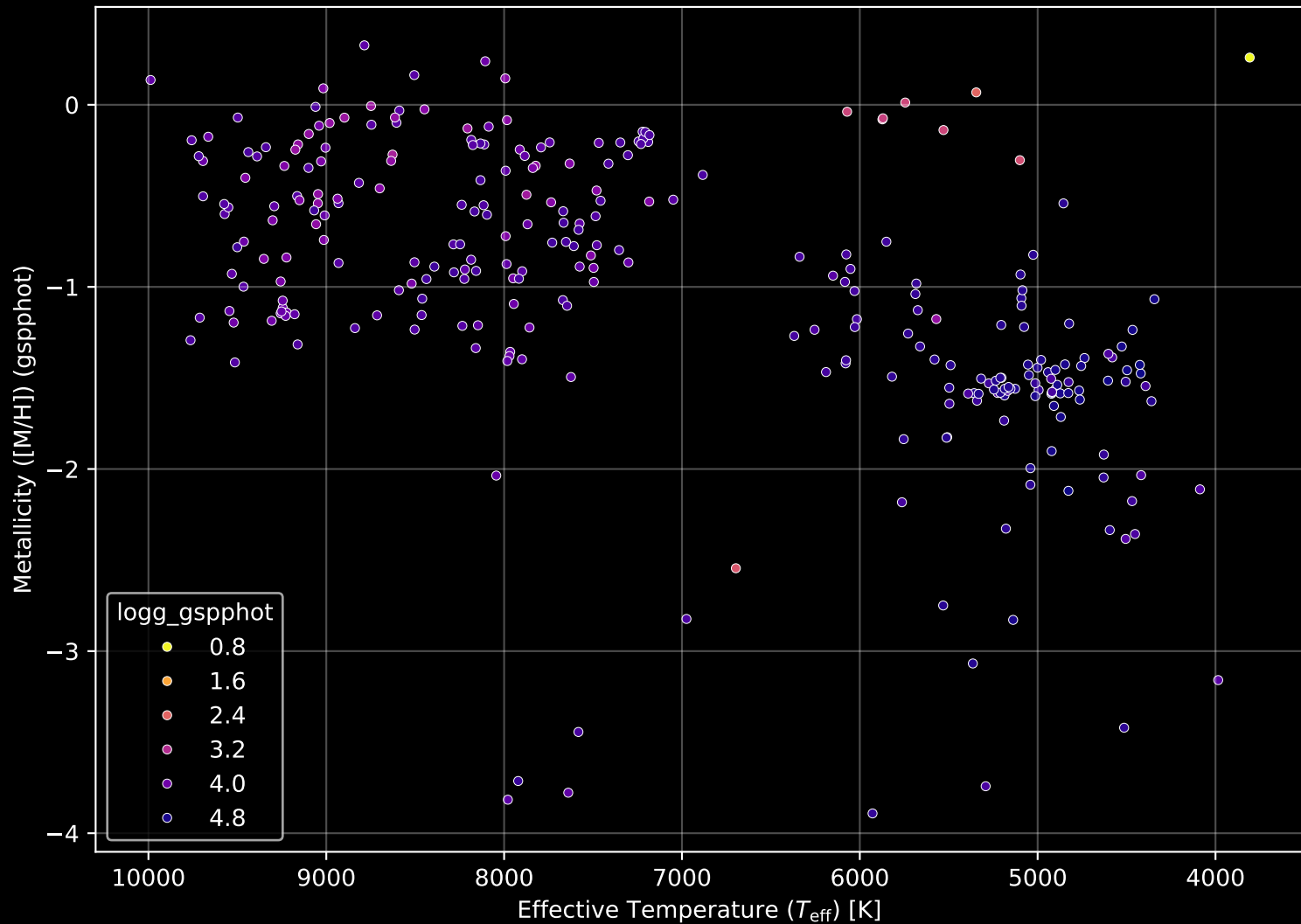
Gaia Cluster: [Trumpler_32] Stellar Population Parameters (n= 292)
