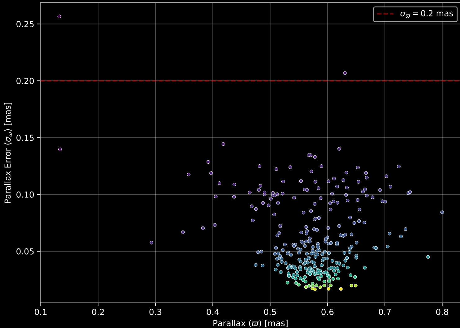
Gaia Cluster: [Trumpler_32] Parallax Quality (n= 292)
