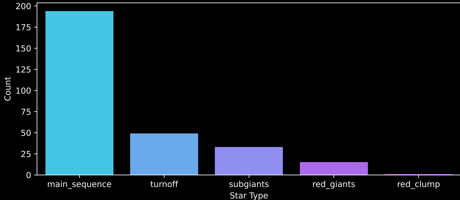
Gaia Cluster: [Trumpler_32] Count plot of Star Type
