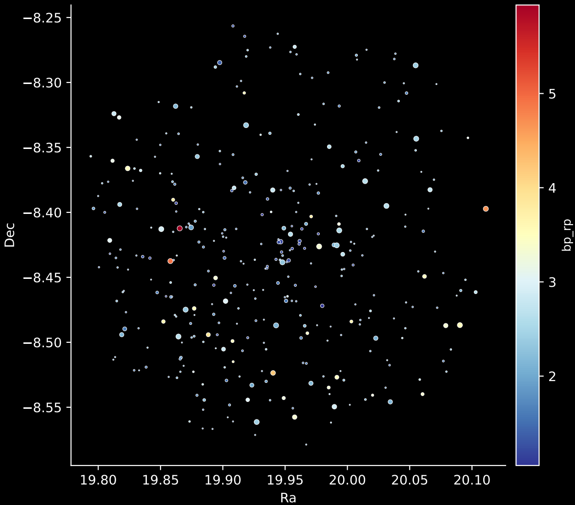
Gaia Cluster: [Trumpler_34] Stars: 354
