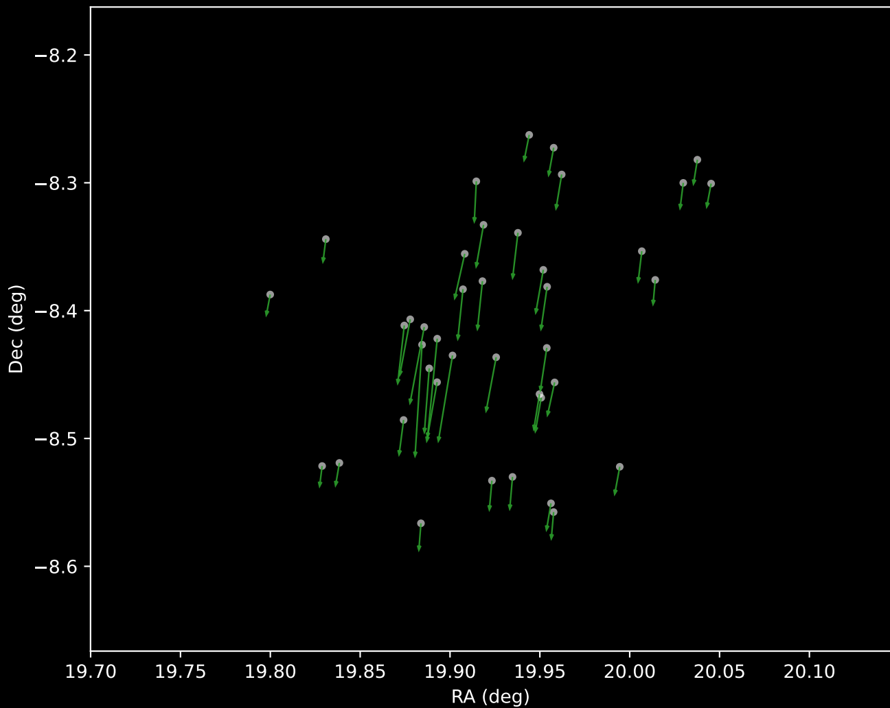
Gaia DR3 Cluster 4 Proper Motion Vectors (n=40)
