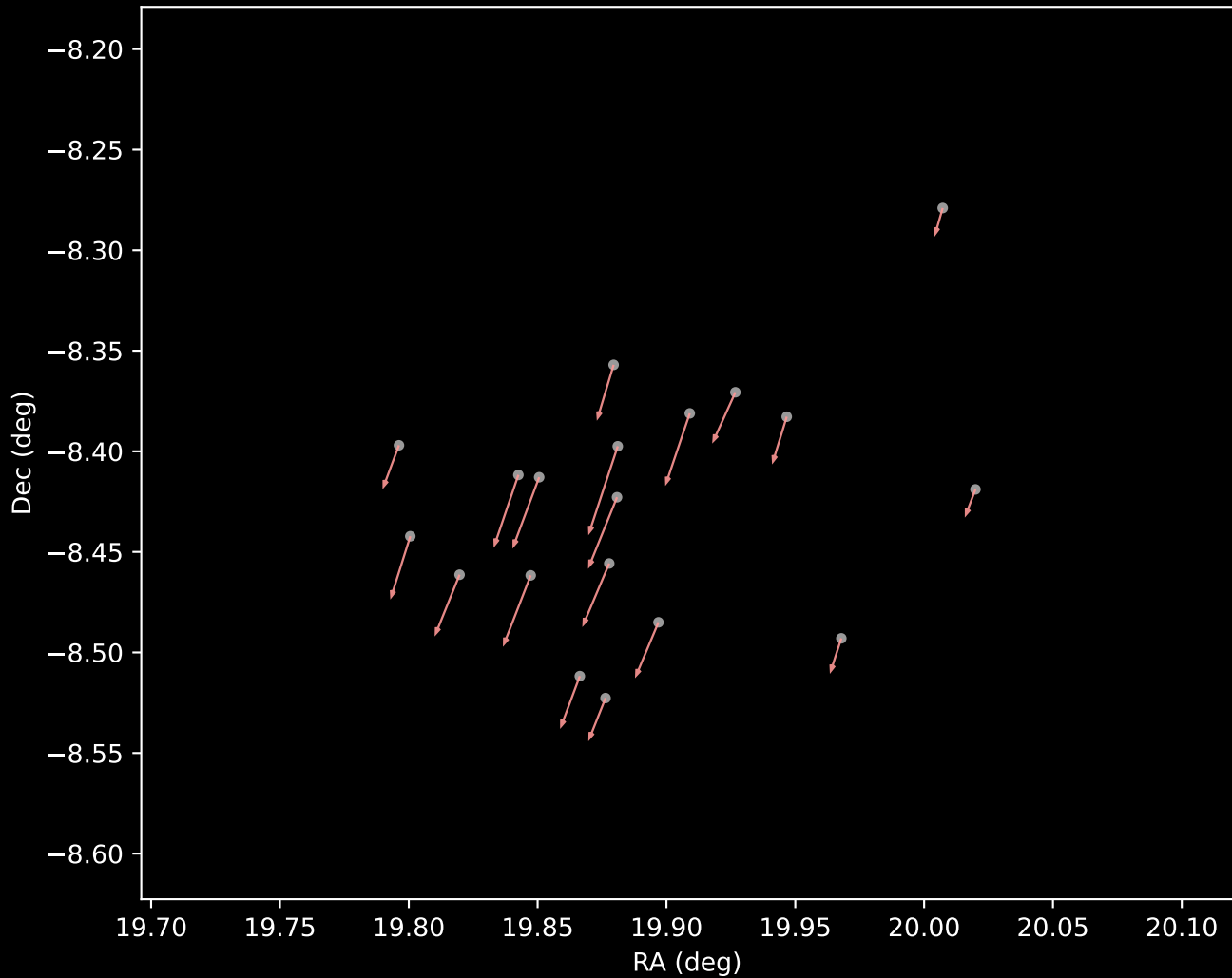
Gaia DR3 Cluster 7 Proper Motion Vectors (n=19)
