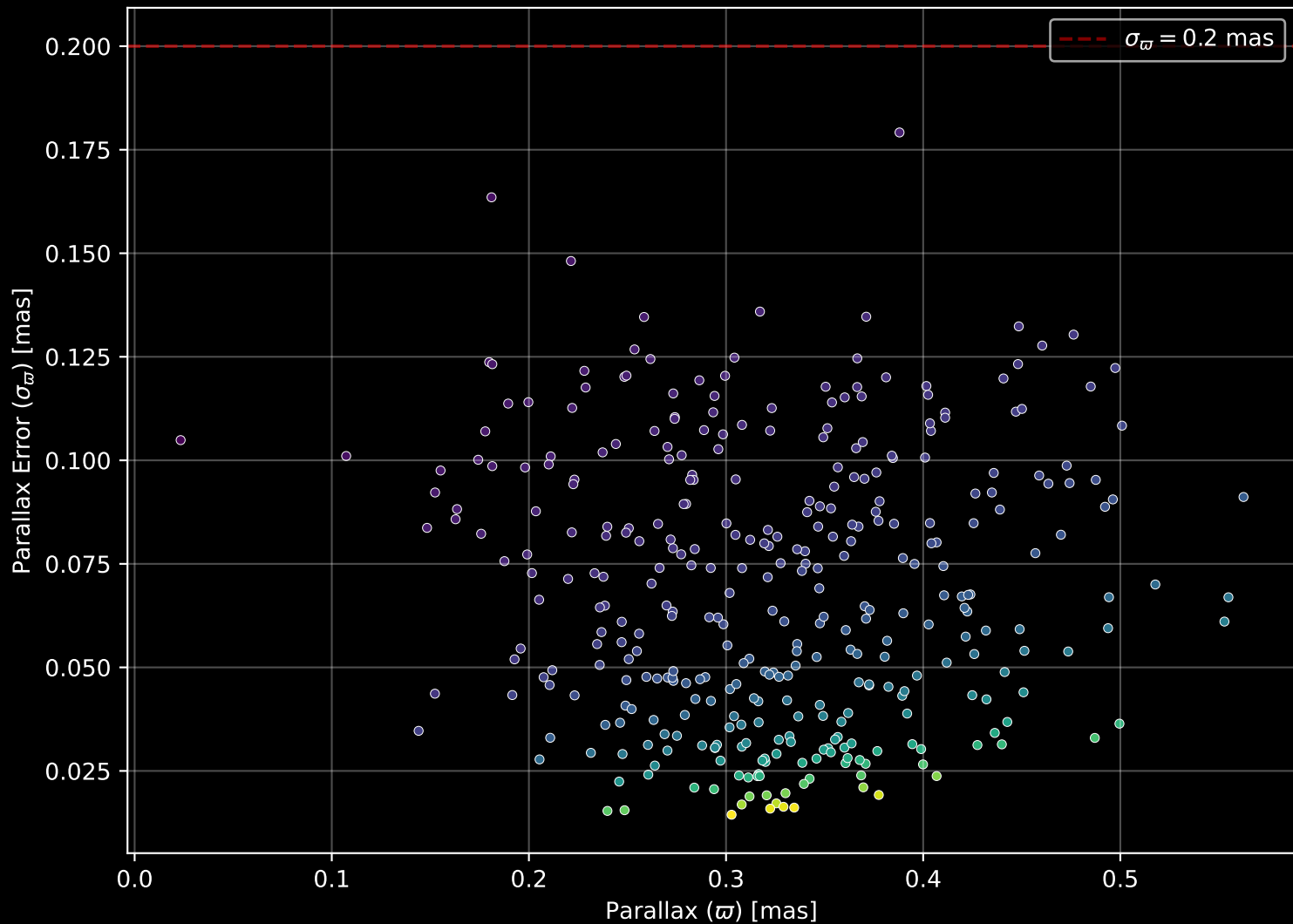
Gaia Cluster: [Trumpler_34] Parallax Quality (n= 354)
