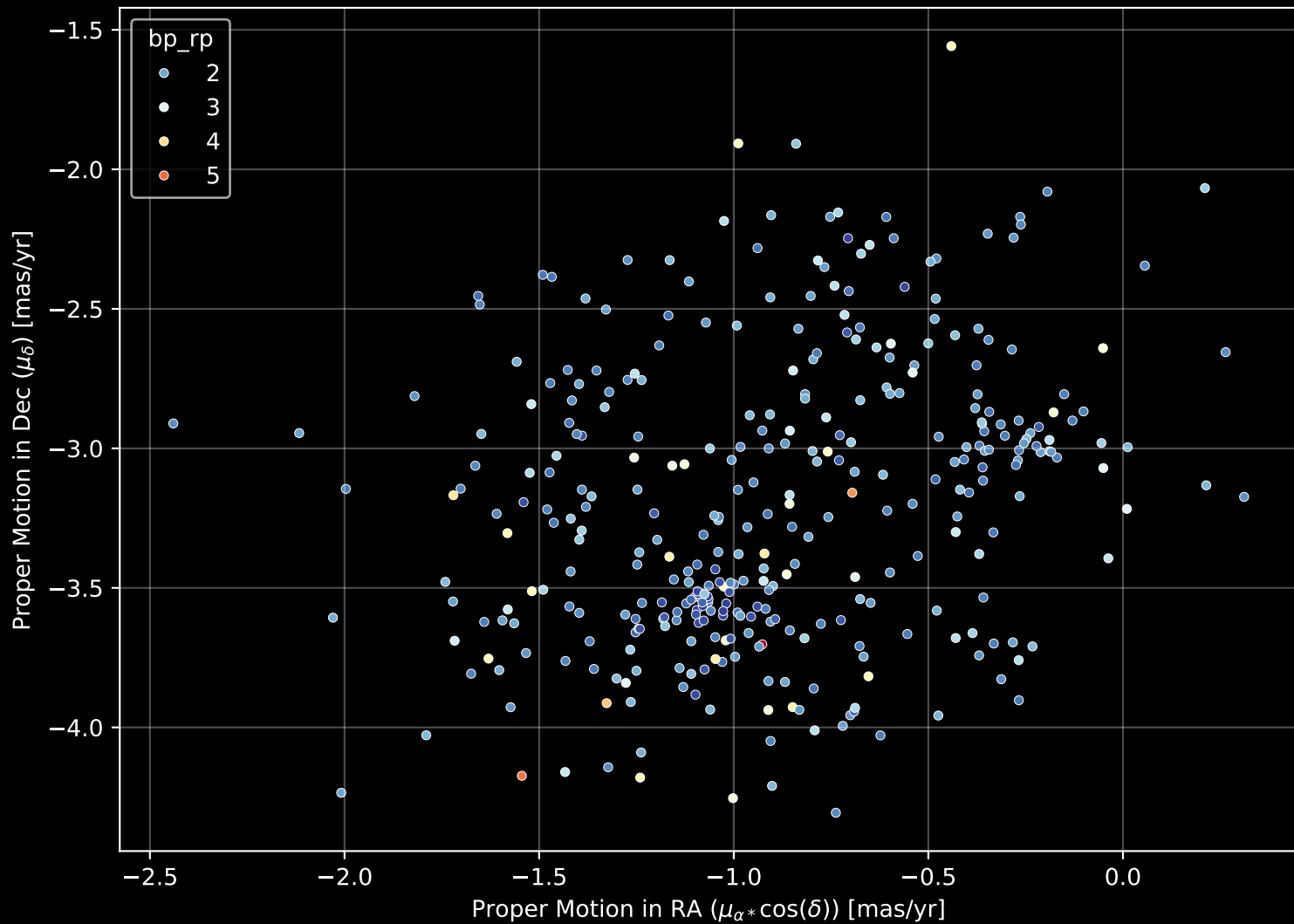
Gaia Cluster: [Trumpler_34] Proper Motion Diagram (n= 354)
