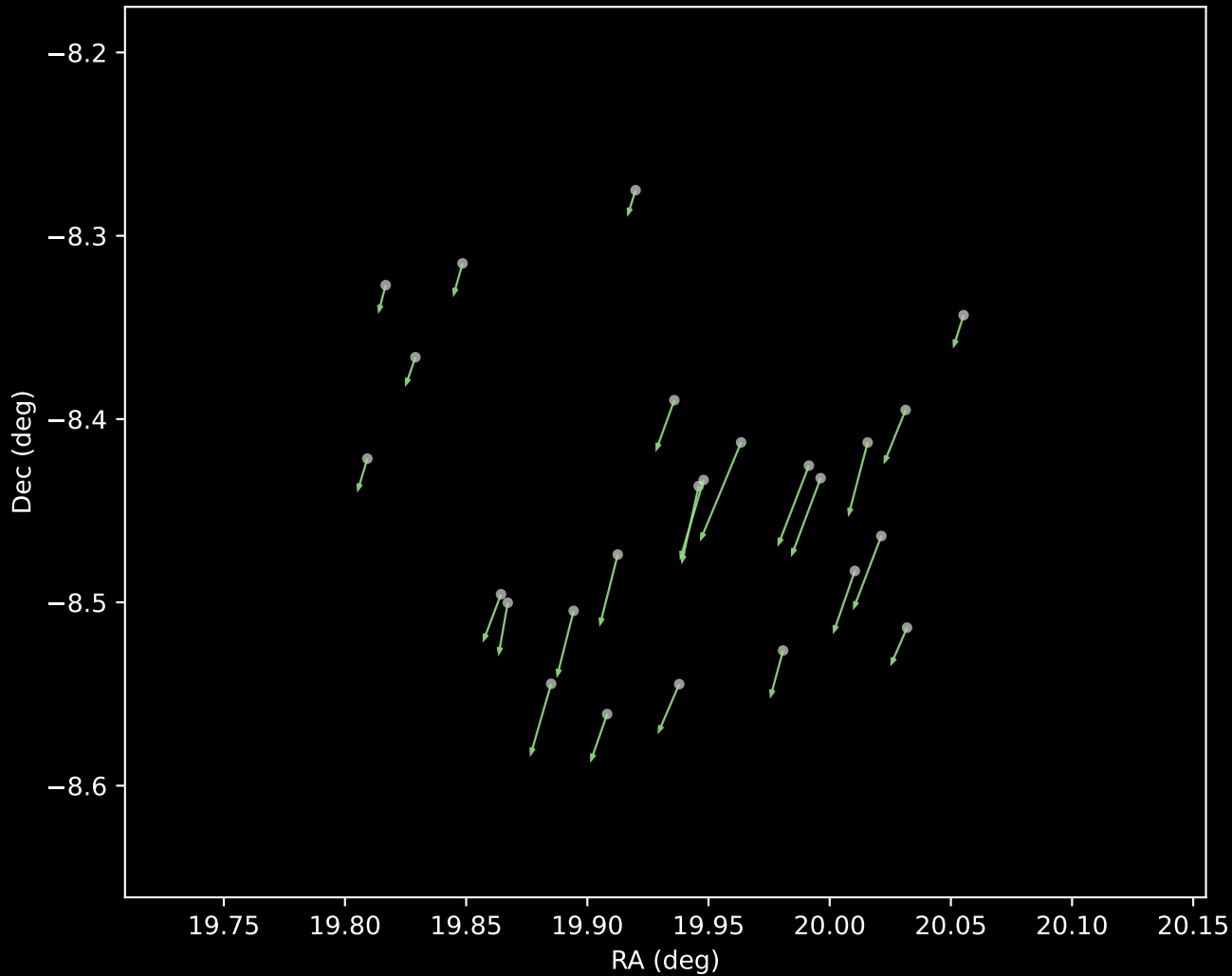
Gaia DR3 Cluster 5 Proper Motion Vectors (n=25)
