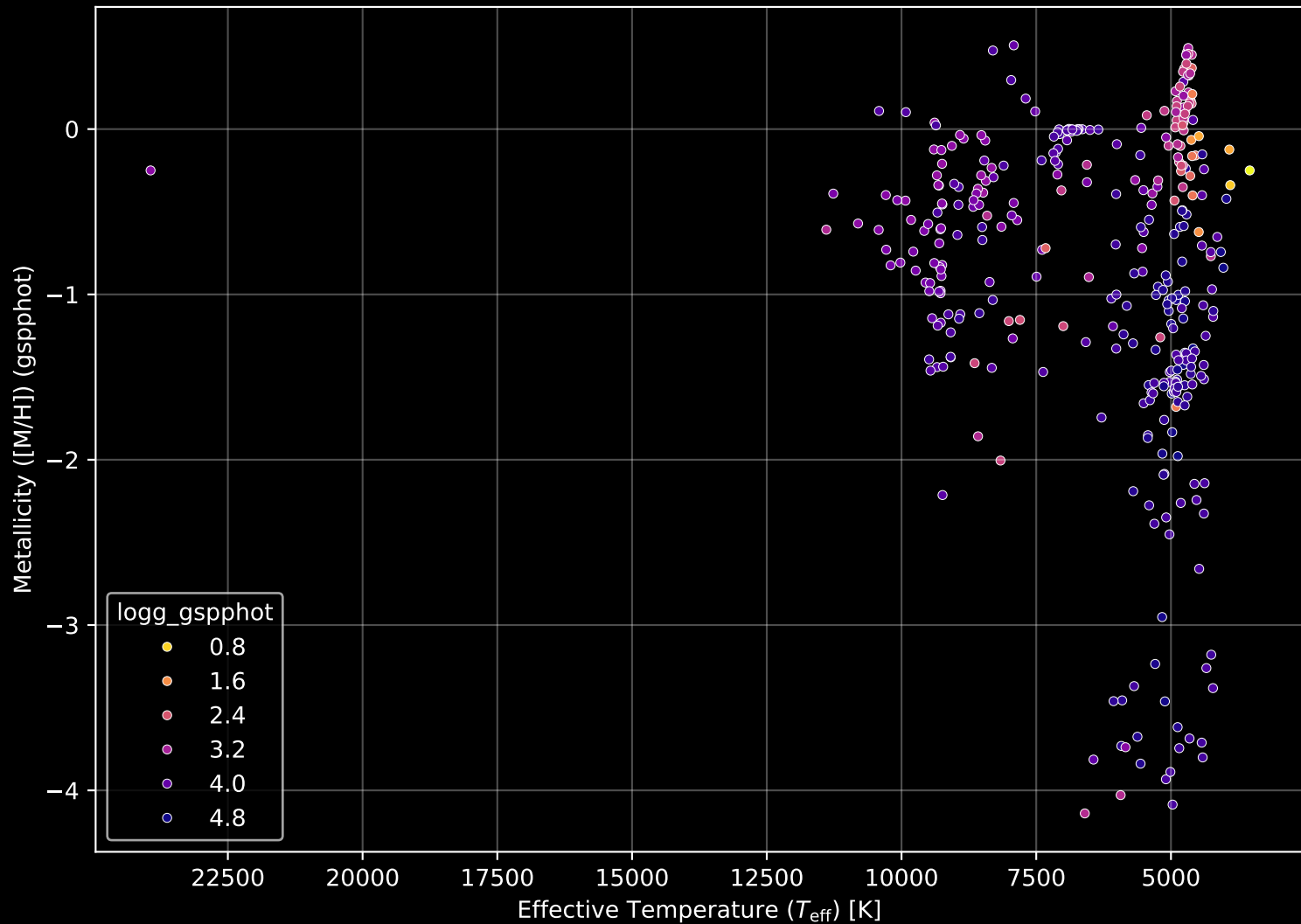
Gaia Cluster: [Trumpler_34] Stellar Population Parameters (n= 354)
