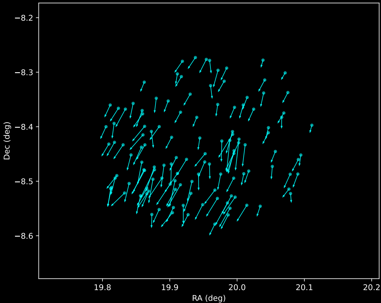
Gaia DR3 Noise Stream Proper Motion Vectors (n=121)
