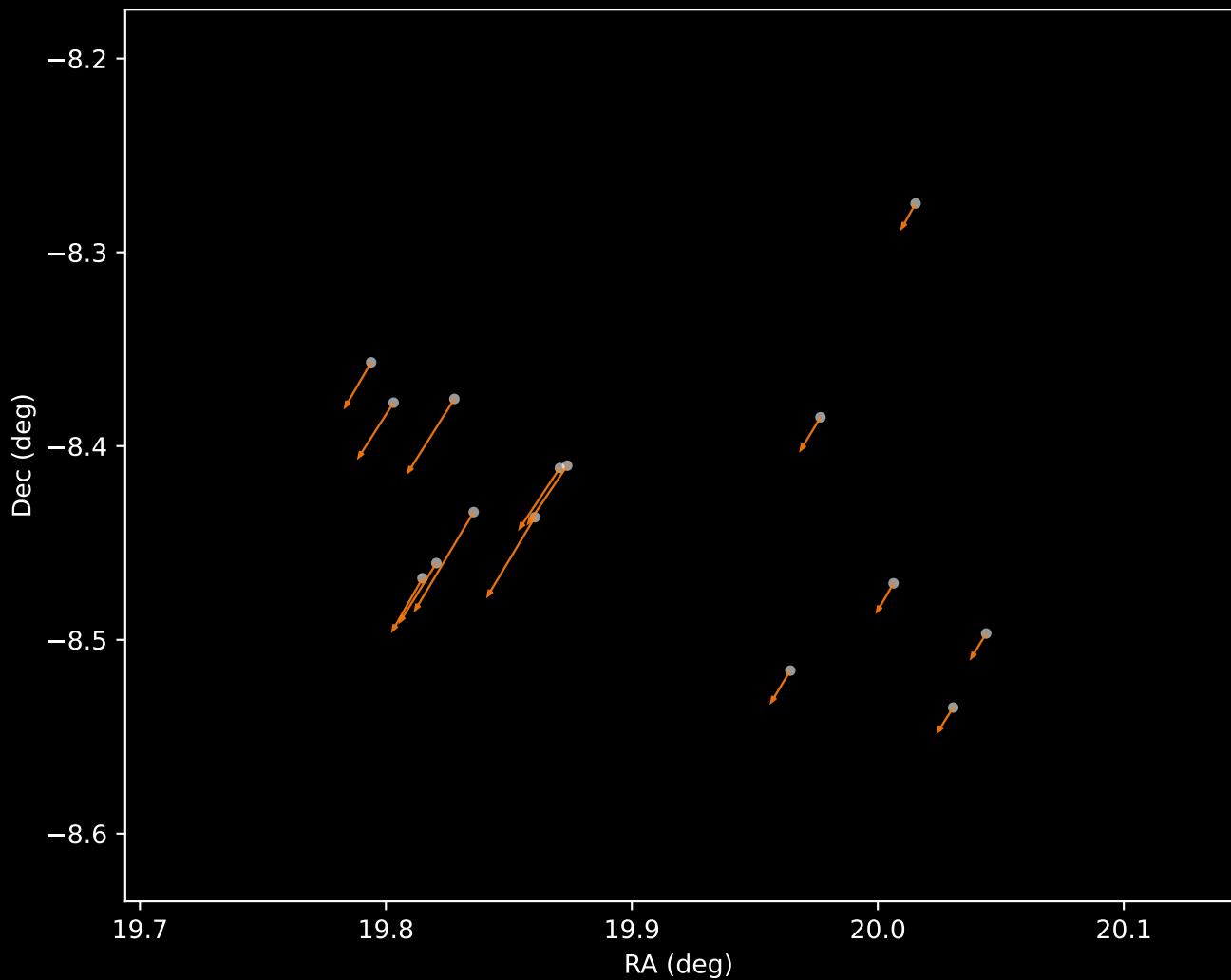
Gaia DR3 Cluster 2 Proper Motion Vectors (n=15)
