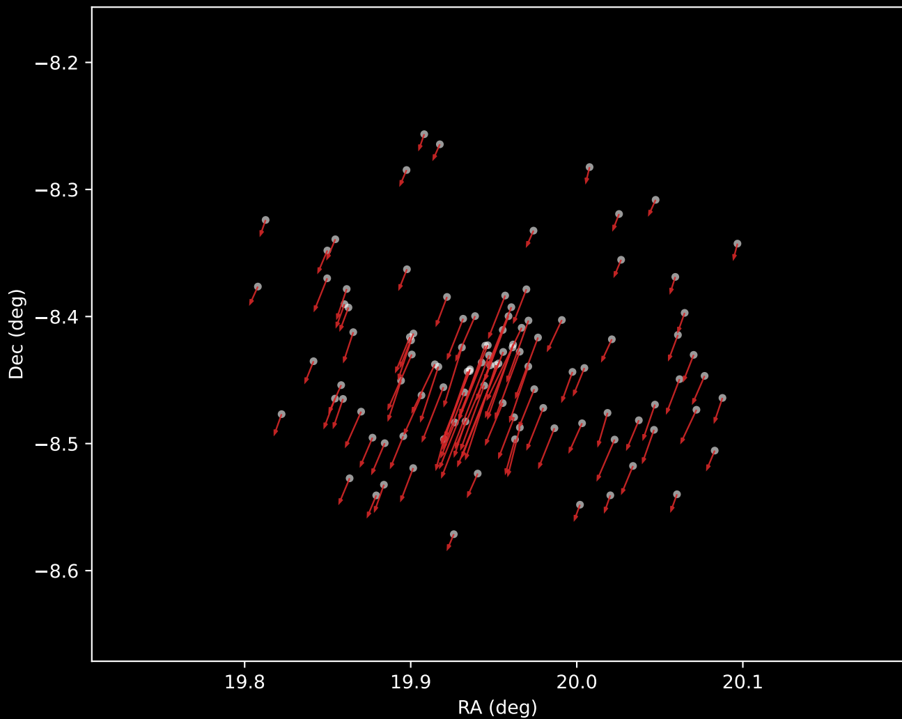
Gaia DR3 Cluster 6 Proper Motion Vectors (n=105)
