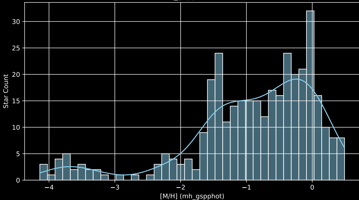
Gaia Cluster: [Trumpler_34 [M/H] (mh_gspphot) (n= 353)
