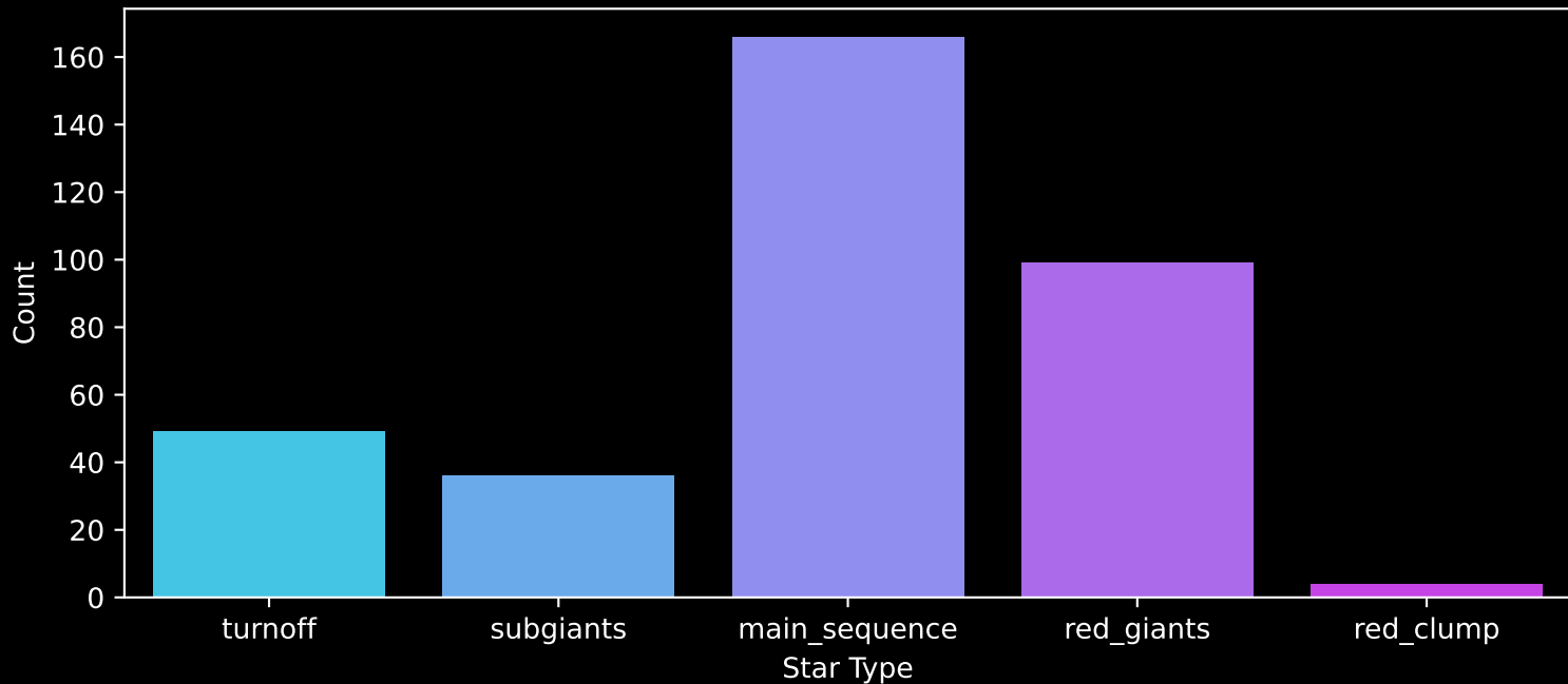
Gaia Cluster: [Trumpler_34] Count plot of Star Type
