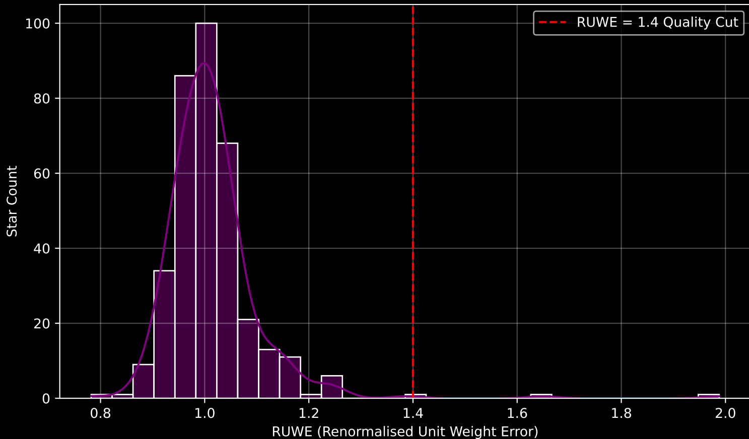
Gaia Cluster: [Trumpler_34] RUWE Distribution (n= 354)
