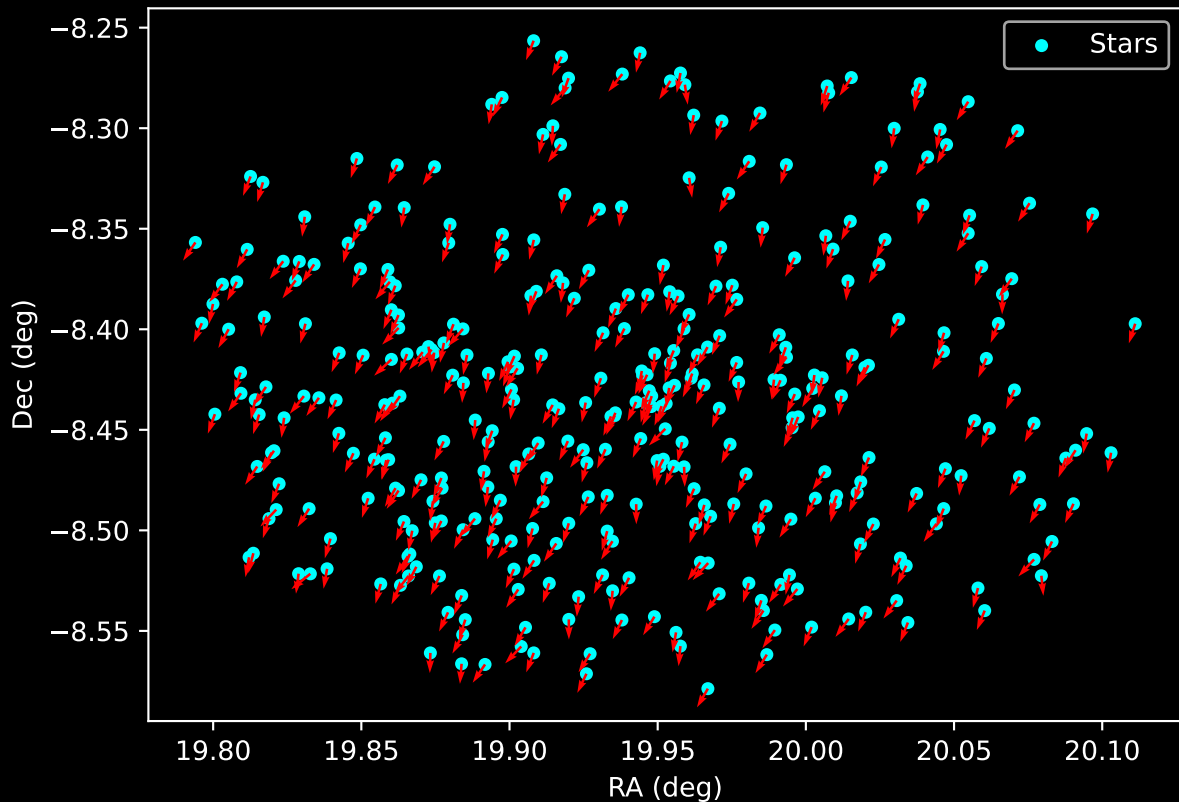
Gaia Cluster: [Trumpler_34] Proper Motion Vectors for Gaia Star Field (n= 354)
