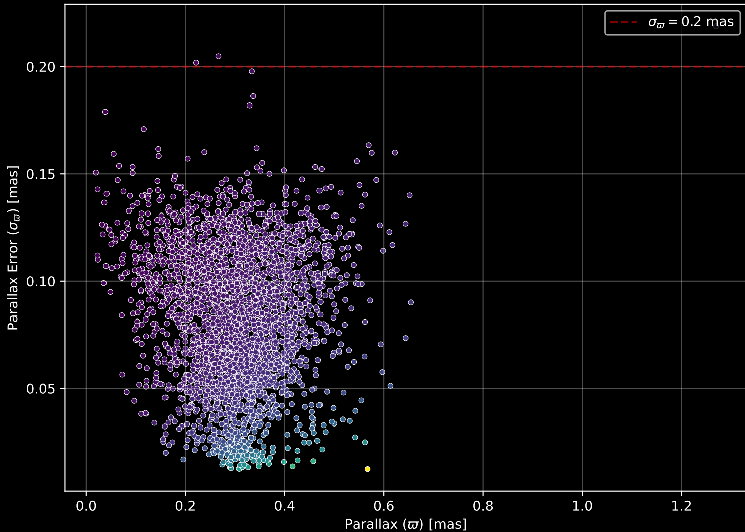
Gaia Cluster: [Trumpler_5] Parallax Quality (n= 2994)
