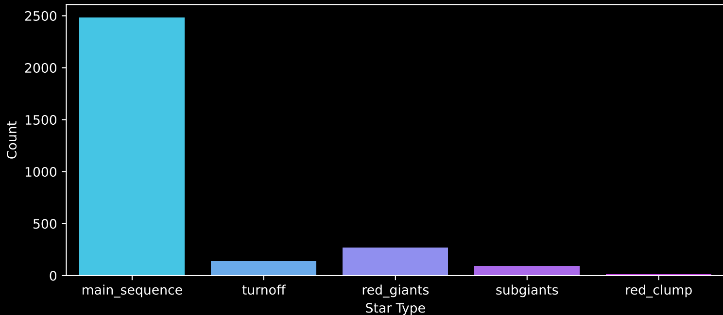
Gaia Cluster: [Trumpler_5] Count plot of Star Type
