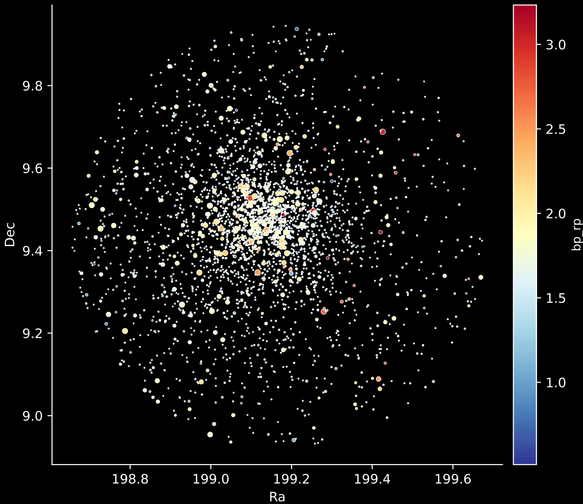
Gaia Cluster: [Trumpler_5] Stars: 2994
