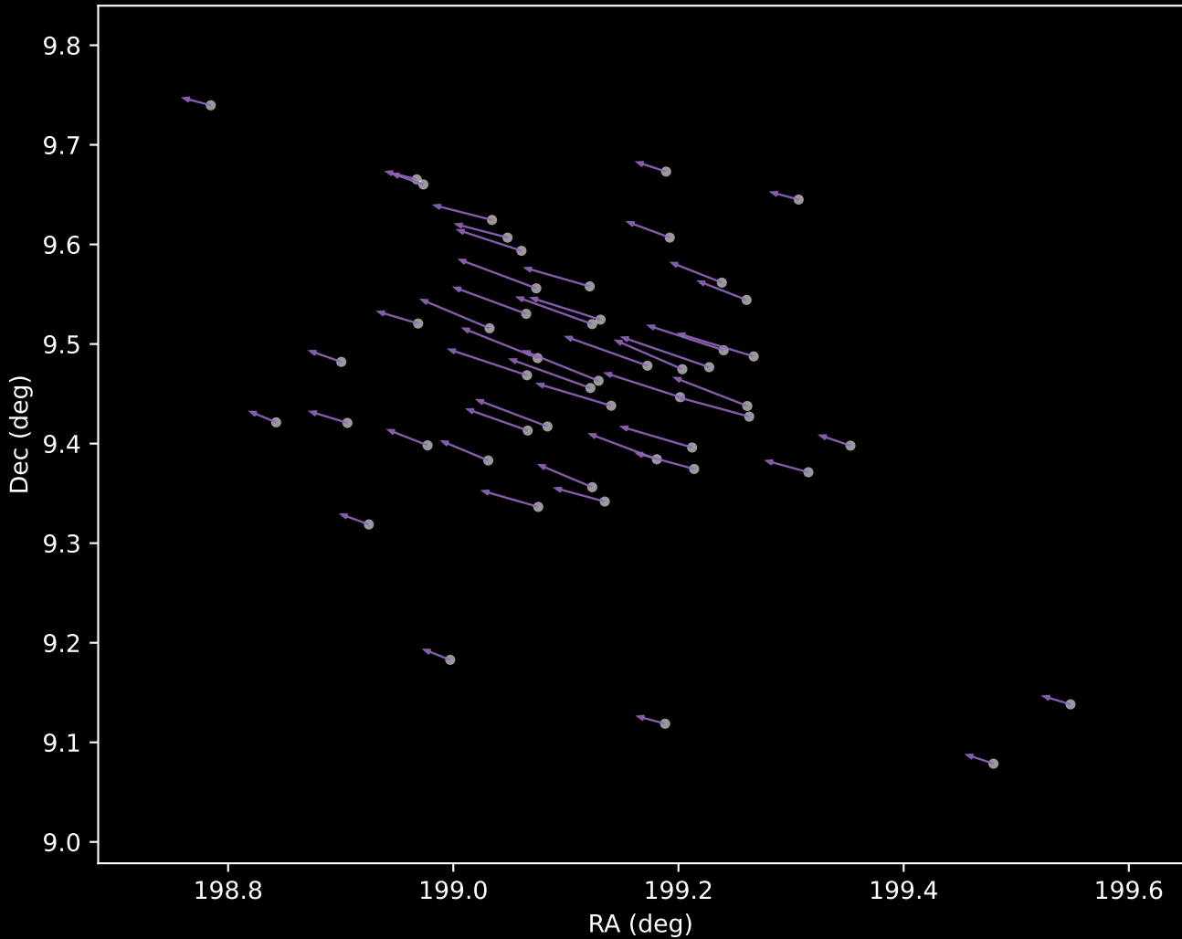
Gaia DR3 Cluster 108 Proper Motion Vectors (n=51)
