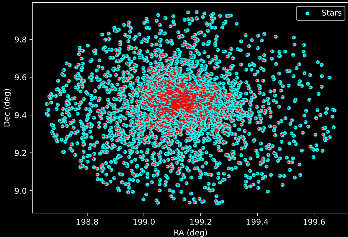
Gaia Cluster: [Trumpler_5] Proper Motion Vectors for Gaia Star Field (n= 2994)
