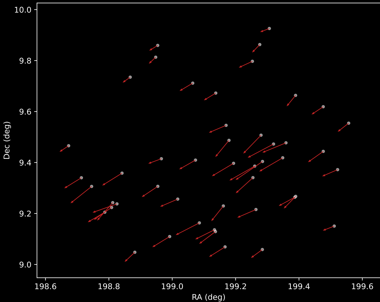
Gaia DR3 Cluster 6 Proper Motion Vectors (n=47)
