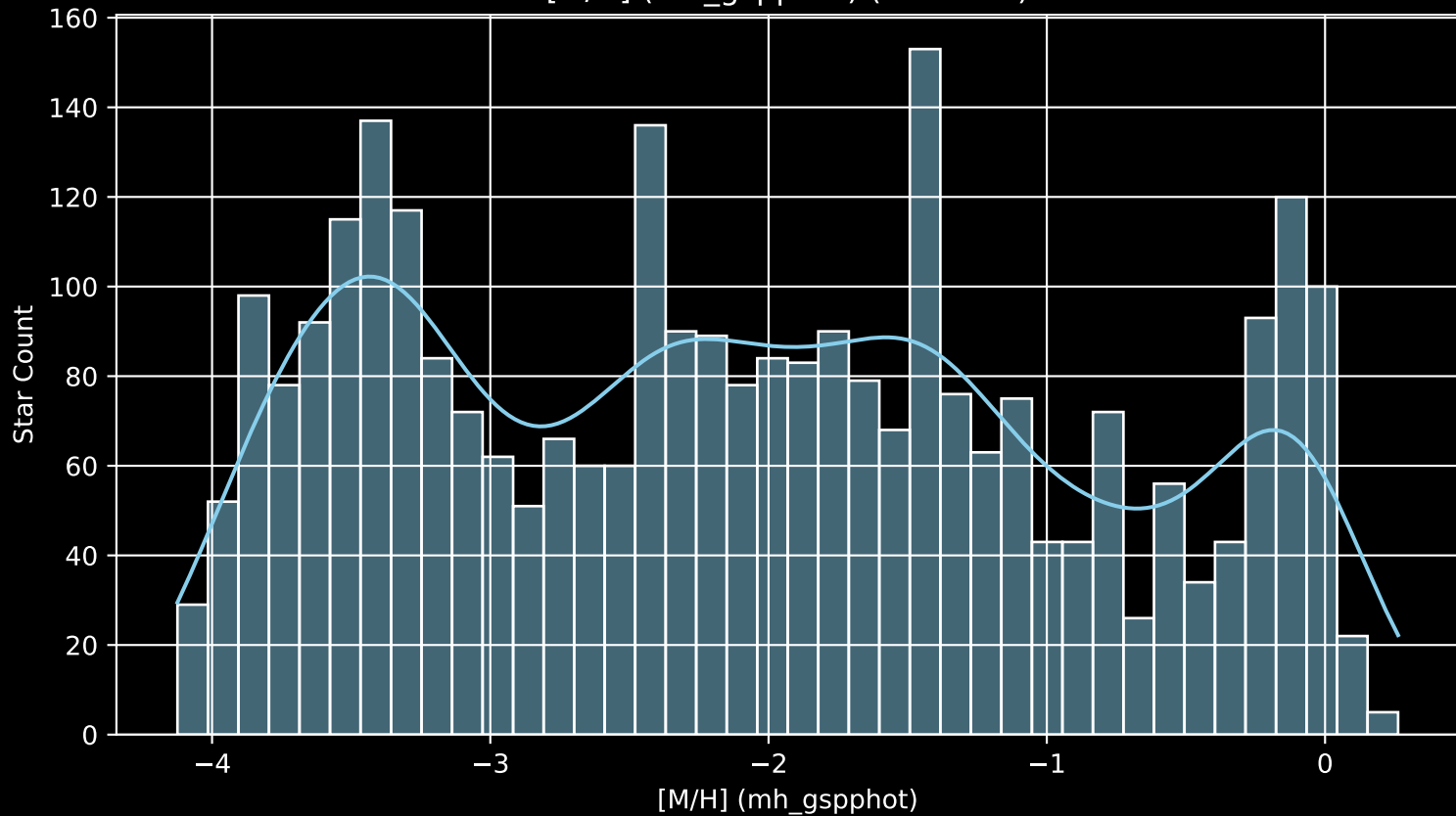
Gaia Cluster: [Trumpler_5 [M/H] (mh_gspphot) (n= 2994)
