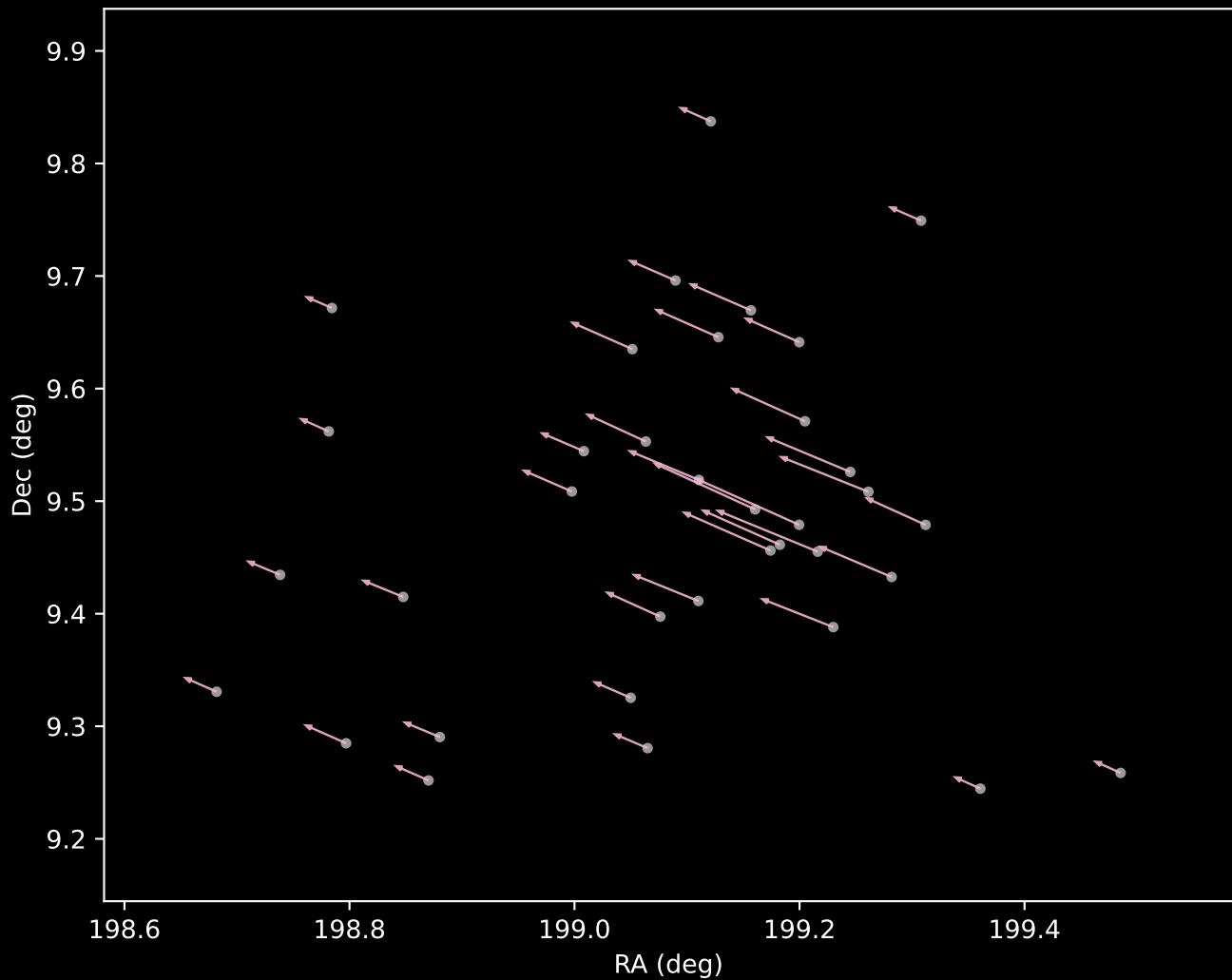
Gaia DR3 Cluster 153 Proper Motion Vectors (n=36)
