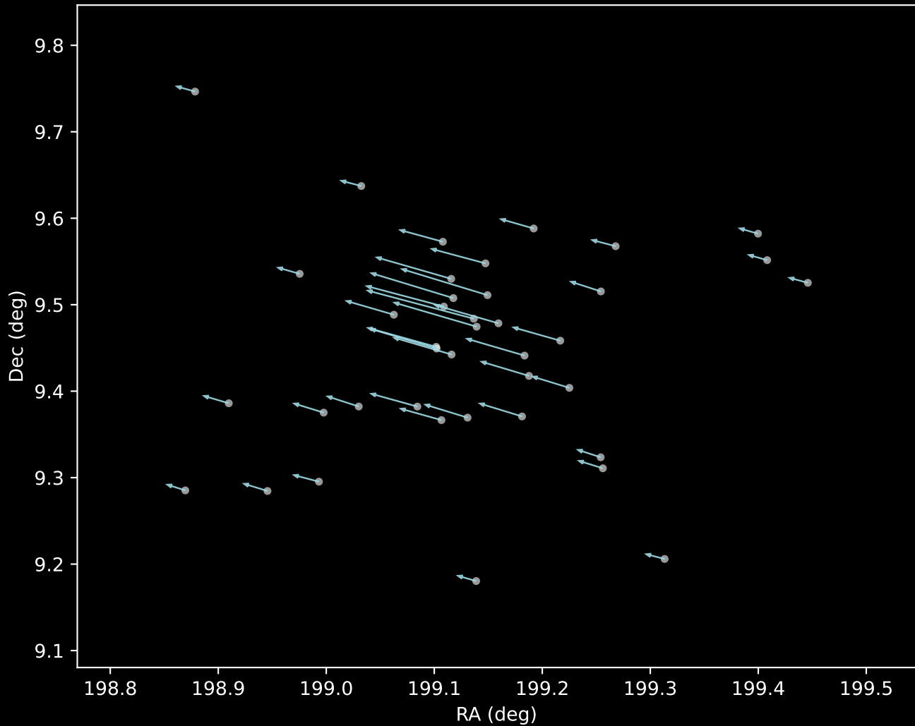
Gaia DR3 Cluster 139 Proper Motion Vectors (n=40)
