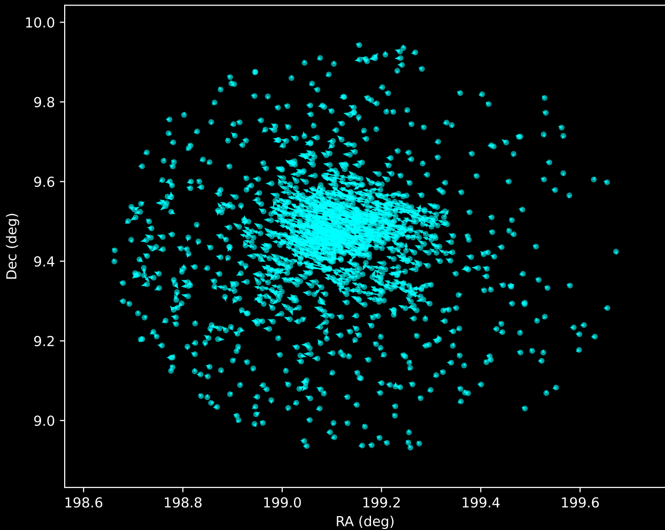
Gaia DR3 Noise Stream Proper Motion Vectors (n=1176)
