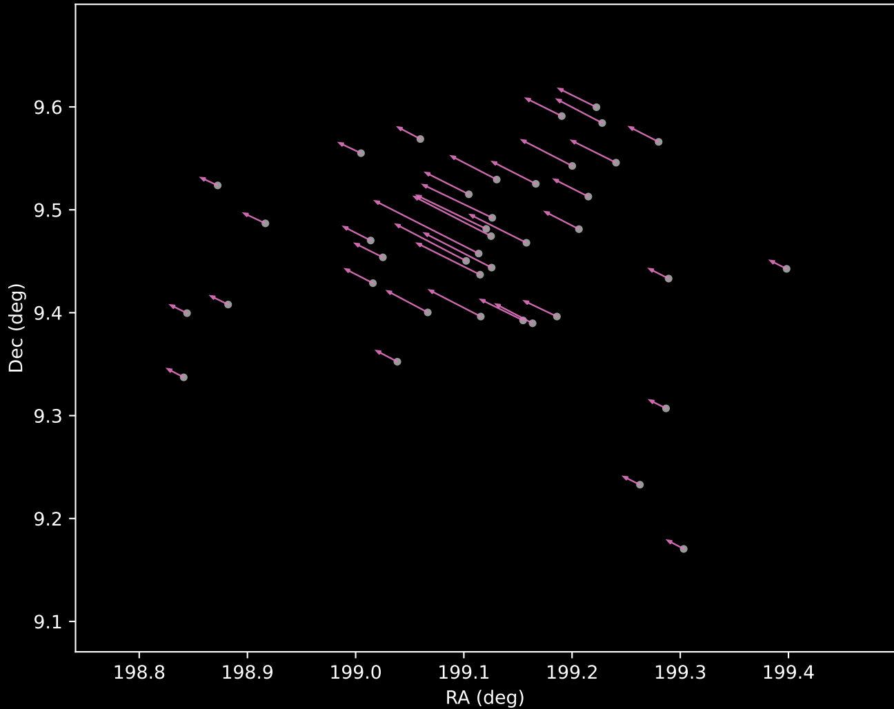
Gaia DR3 Cluster 152 Proper Motion Vectors (n=40)
