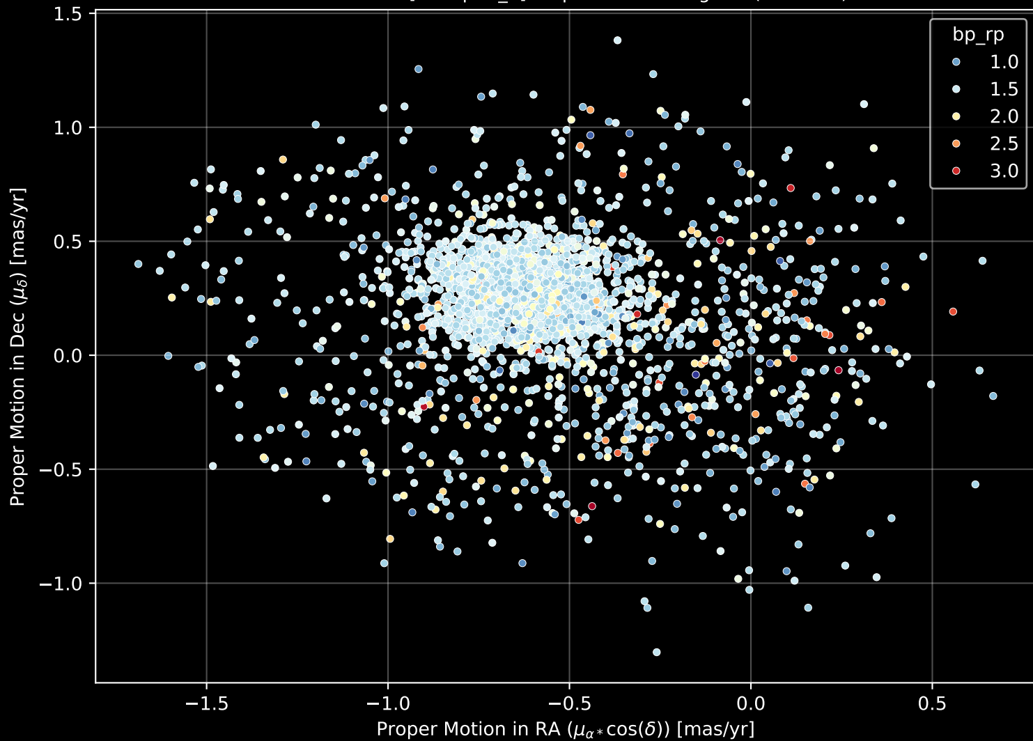
Gaia Cluster: [Trumpler_5] Proper Motion Diagram (n= 2994)
