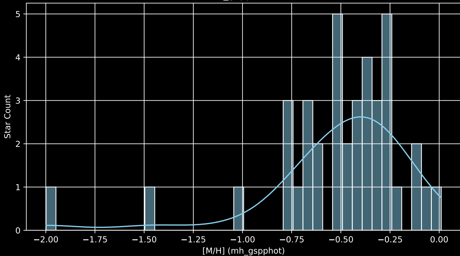
Gaia Cluster: [UBC_10a [M/H] (mh_gspphot) (n= 39)
