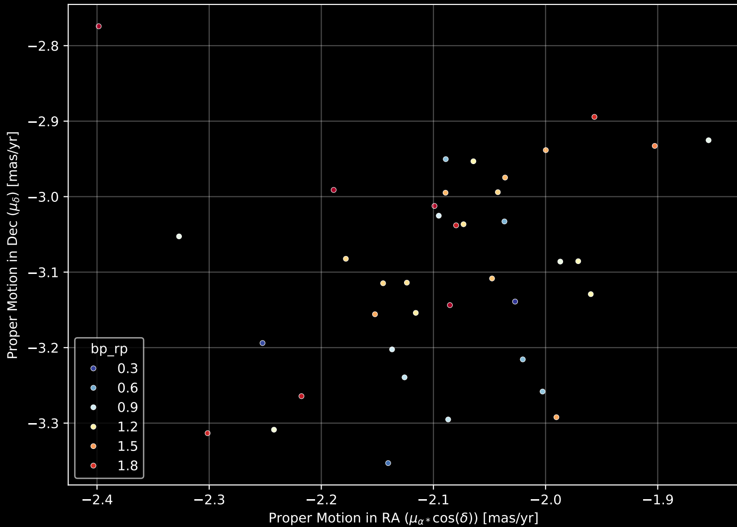
Gaia Cluster: [UBC_10a] Proper Motion Diagram (n= 39)
