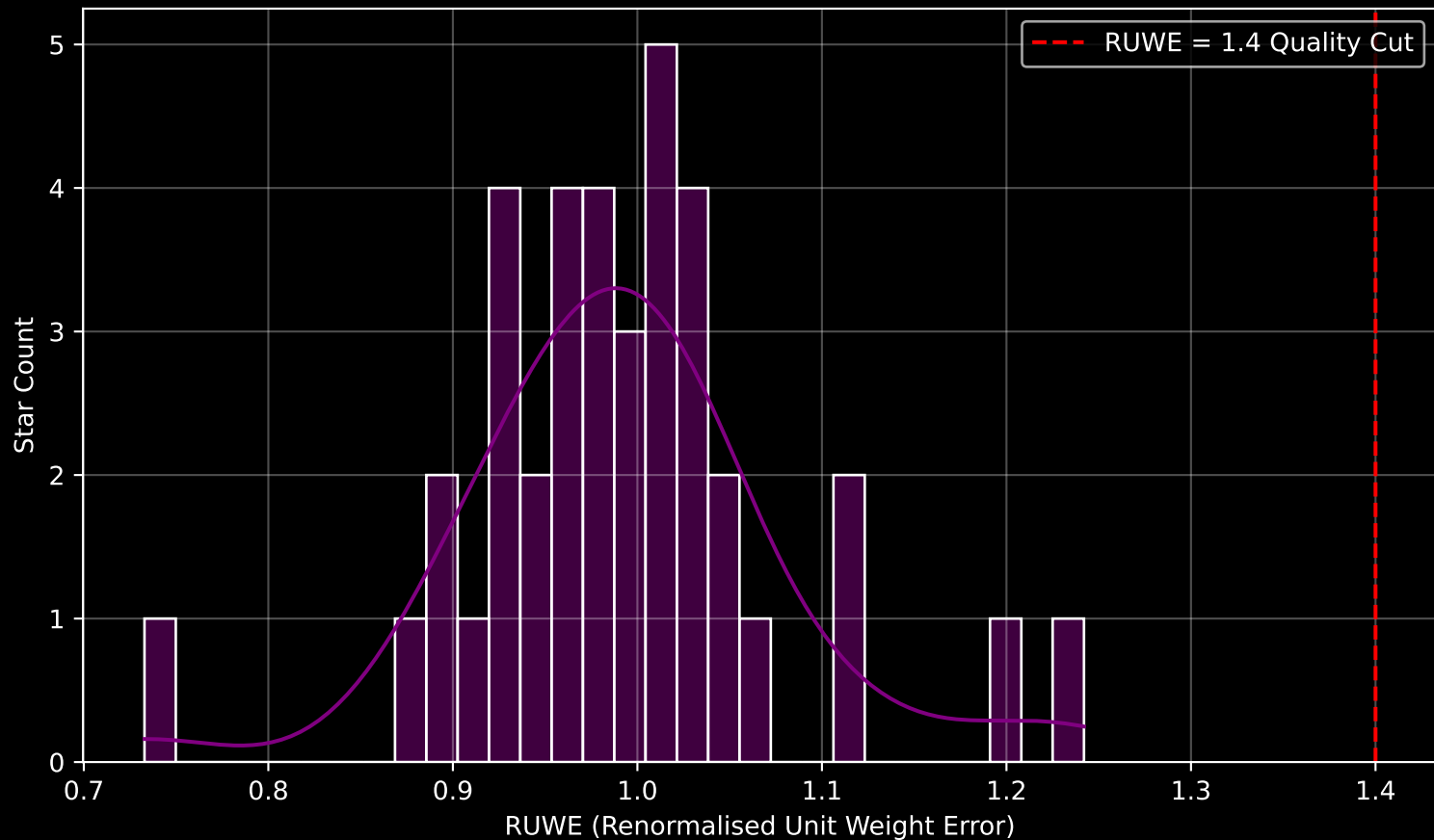
Gaia Cluster: [UBC_10a] RUWE Distribution (n= 38)
