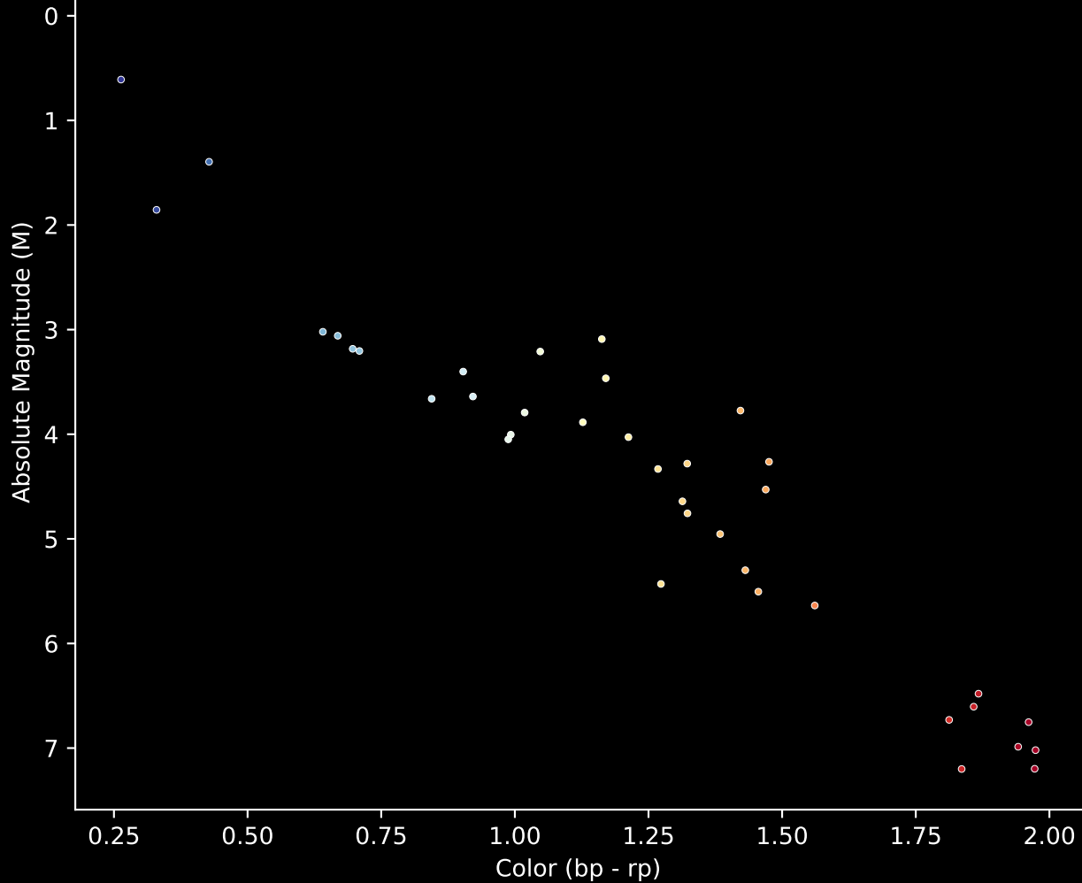
Gaia Cluster: [UBC_10a] Stars (n= 39) Hertzsprung-Russel Diagram
