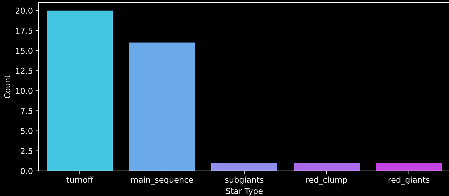
Gaia Cluster: [UBC_10a] Count plot of Star Type
