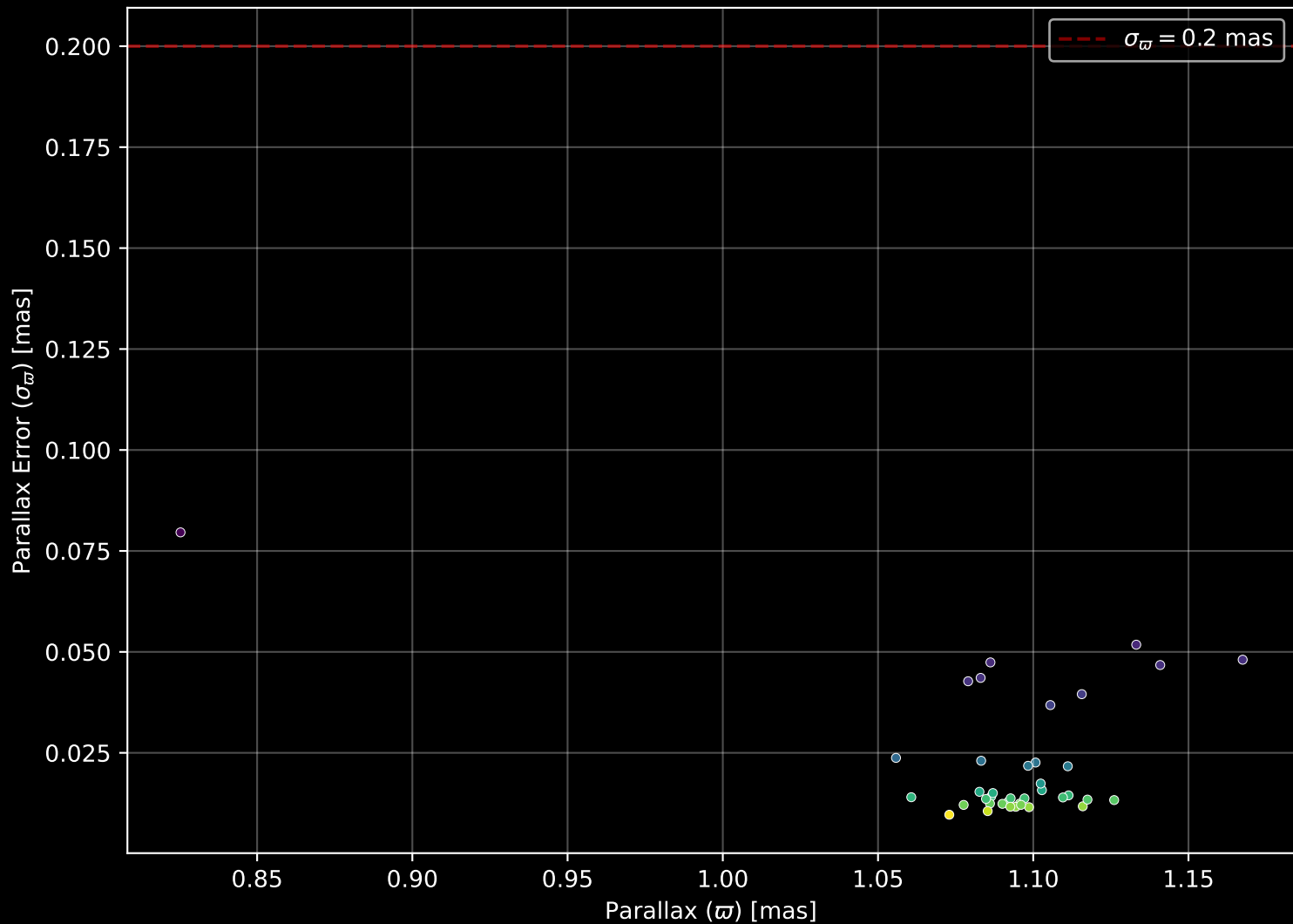
Gaia Cluster: [UBC_10a] Parallax Quality (n= 39)
