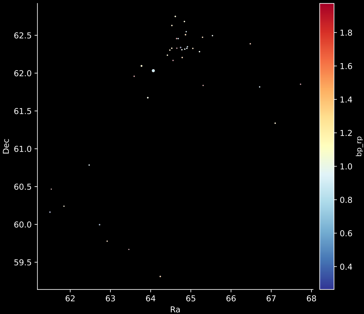
Gaia Cluster: [UBC_10a] Stars: 39
