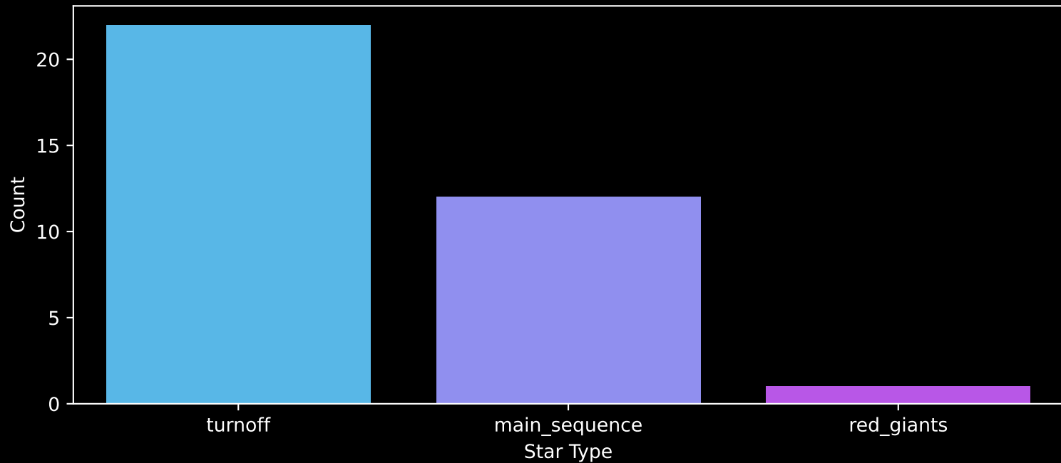
Gaia Cluster: [UBC_10b] Count plot of Star Type
