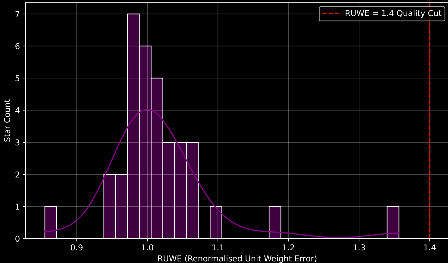
Gaia Cluster: [UBC_10b] RUWE Distribution (n= 35)
