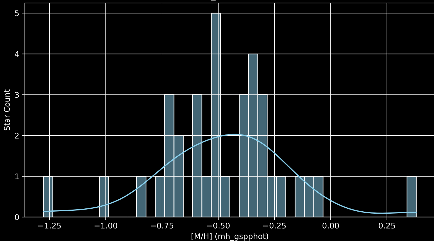
Gaia Cluster: [UBC_10b [M/H] (mh_gspphot) (n= 35)
