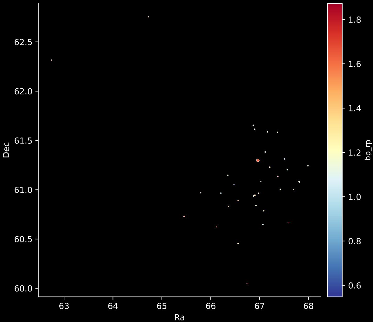
Gaia Cluster: [UBC_10b] Stars: 35
