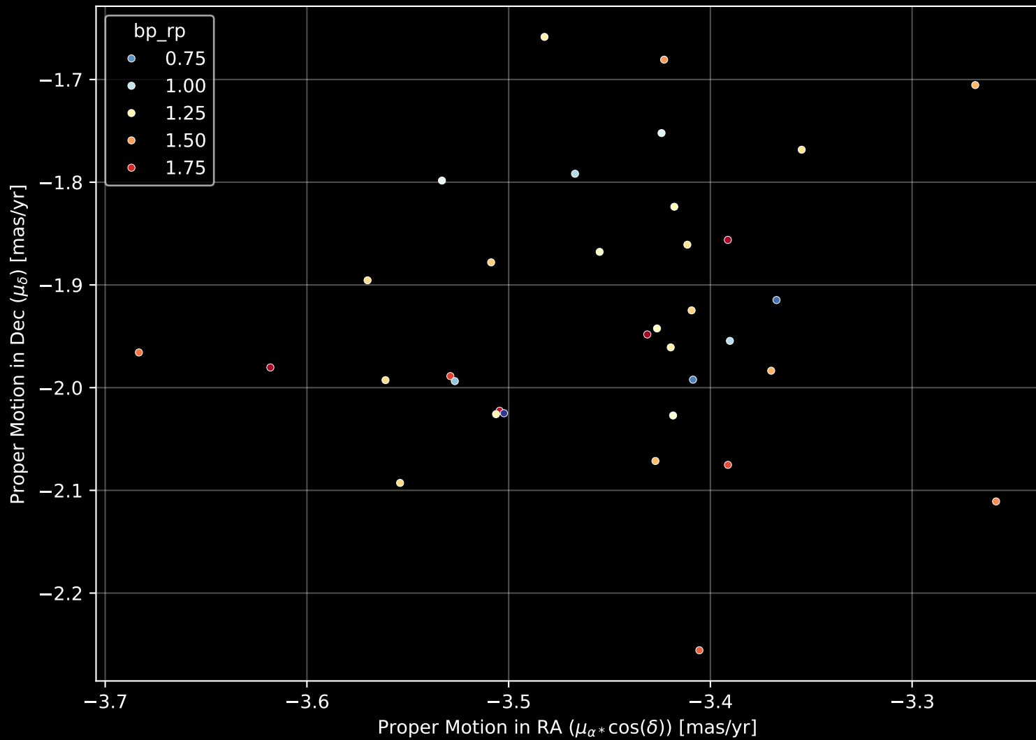
Gaia Cluster: [UBC_10b] Proper Motion Diagram (n= 35)
