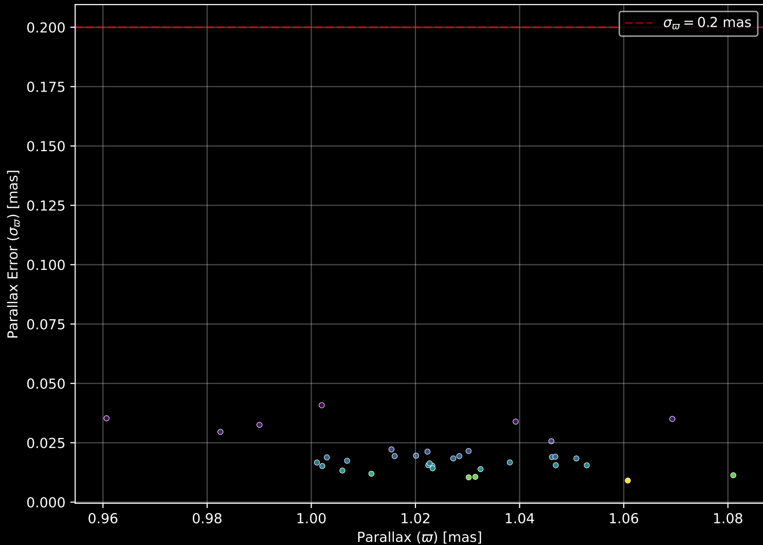
Gaia Cluster: [UBC_10b] Parallax Quality (n= 35)
