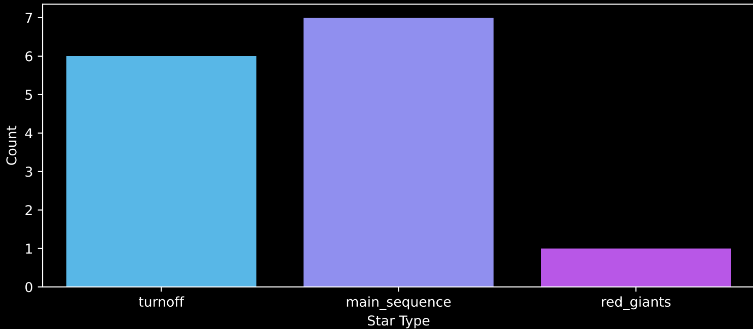
Gaia Cluster: [UBC_12] Count plot of Star Type
