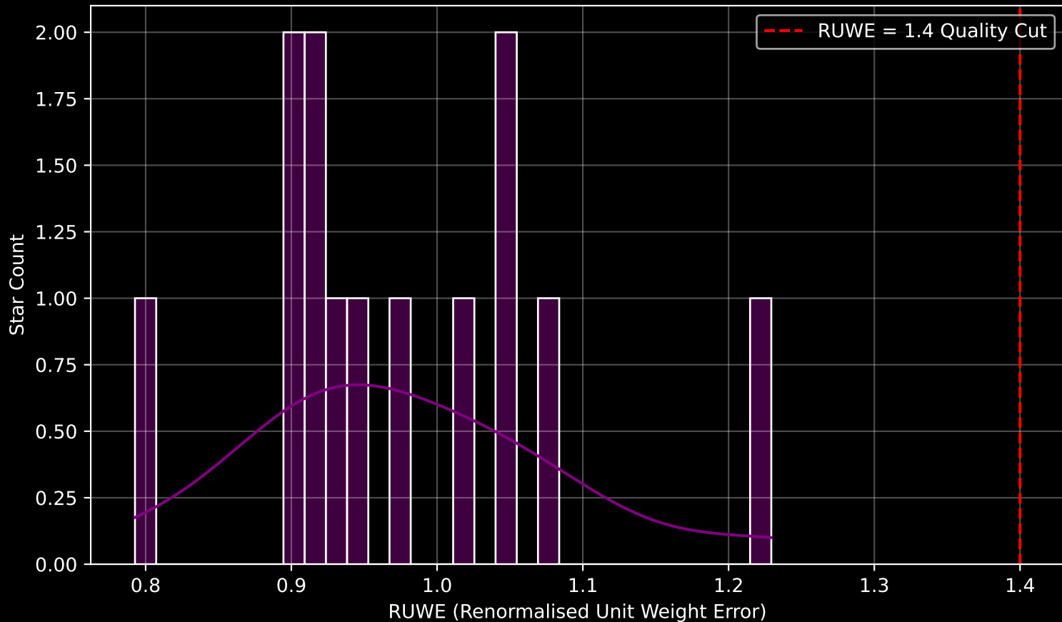
Gaia Cluster: [UBC_12] RUWE Distribution (n= 13)
