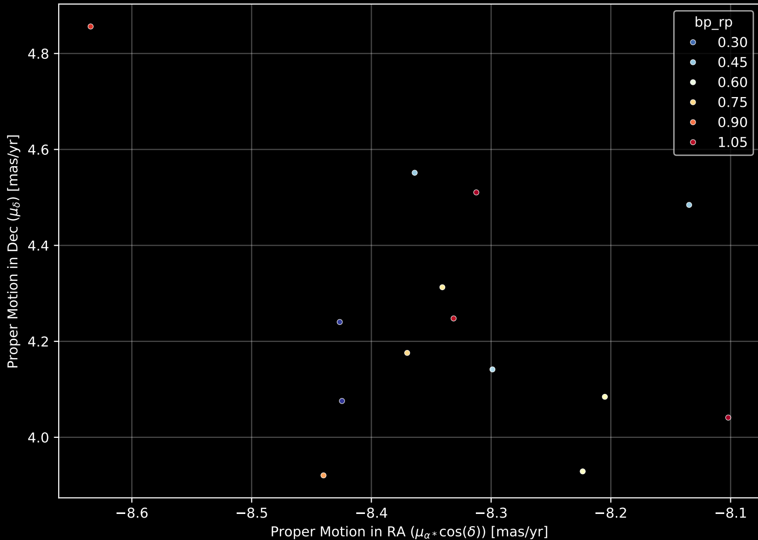
Gaia Cluster: [UBC_12] Proper Motion Diagram (n= 14)
