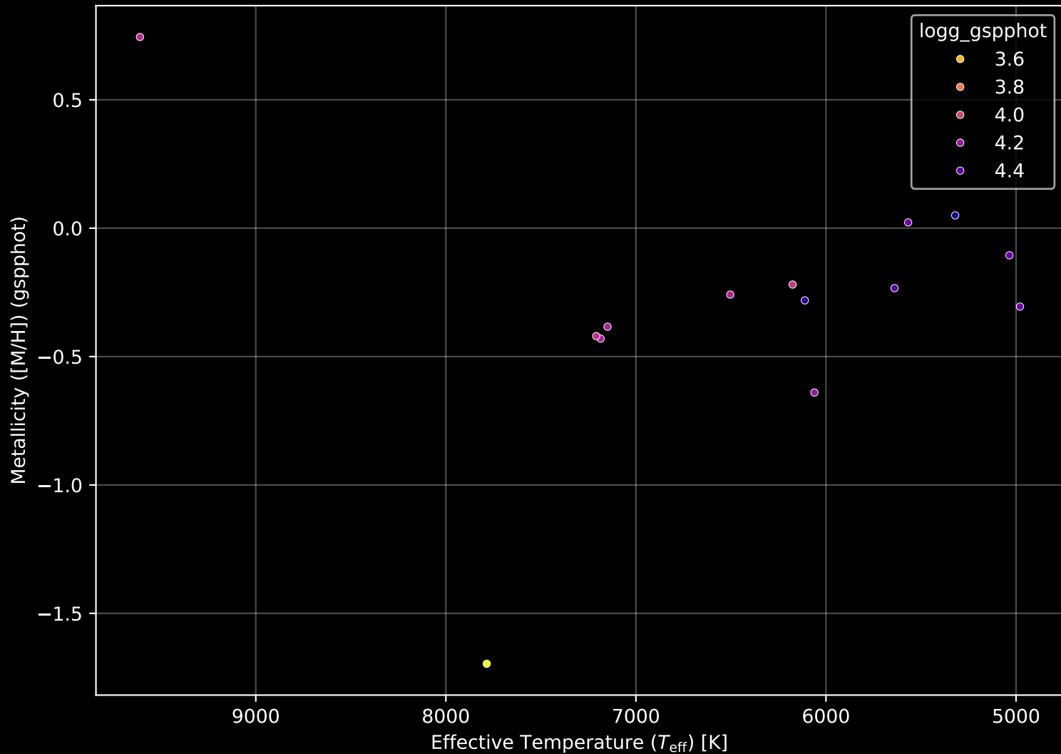
Gaia Cluster: [UBC_12] Stellar Population Parameters (n= 14)
