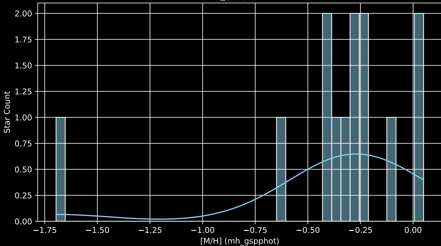
Gaia Cluster: [UBC_12 [M/H] (mh_gspphot) (n= 13)
