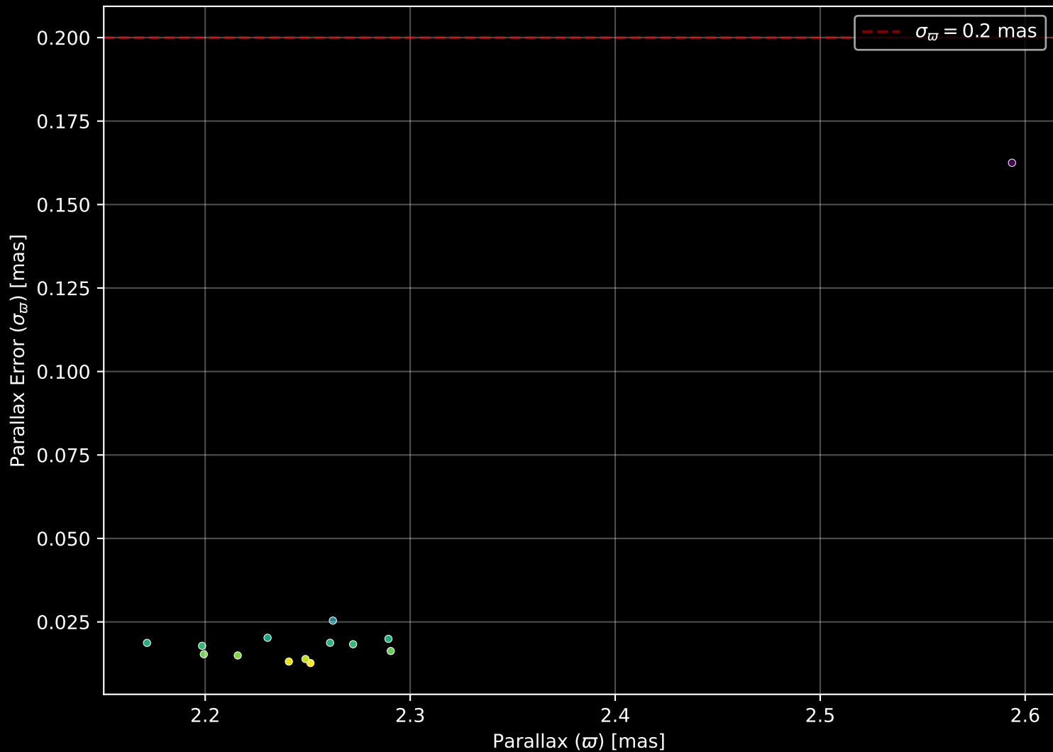
Gaia Cluster: [UBC_12] Parallax Quality (n= 14)
