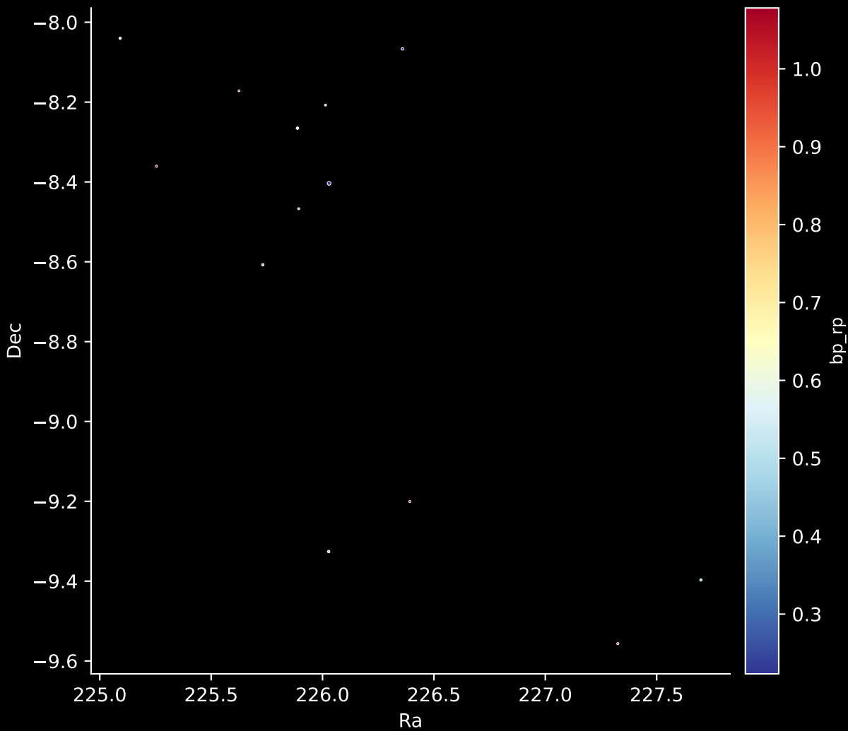
Gaia Cluster: [UBC_12] Stars: 14
