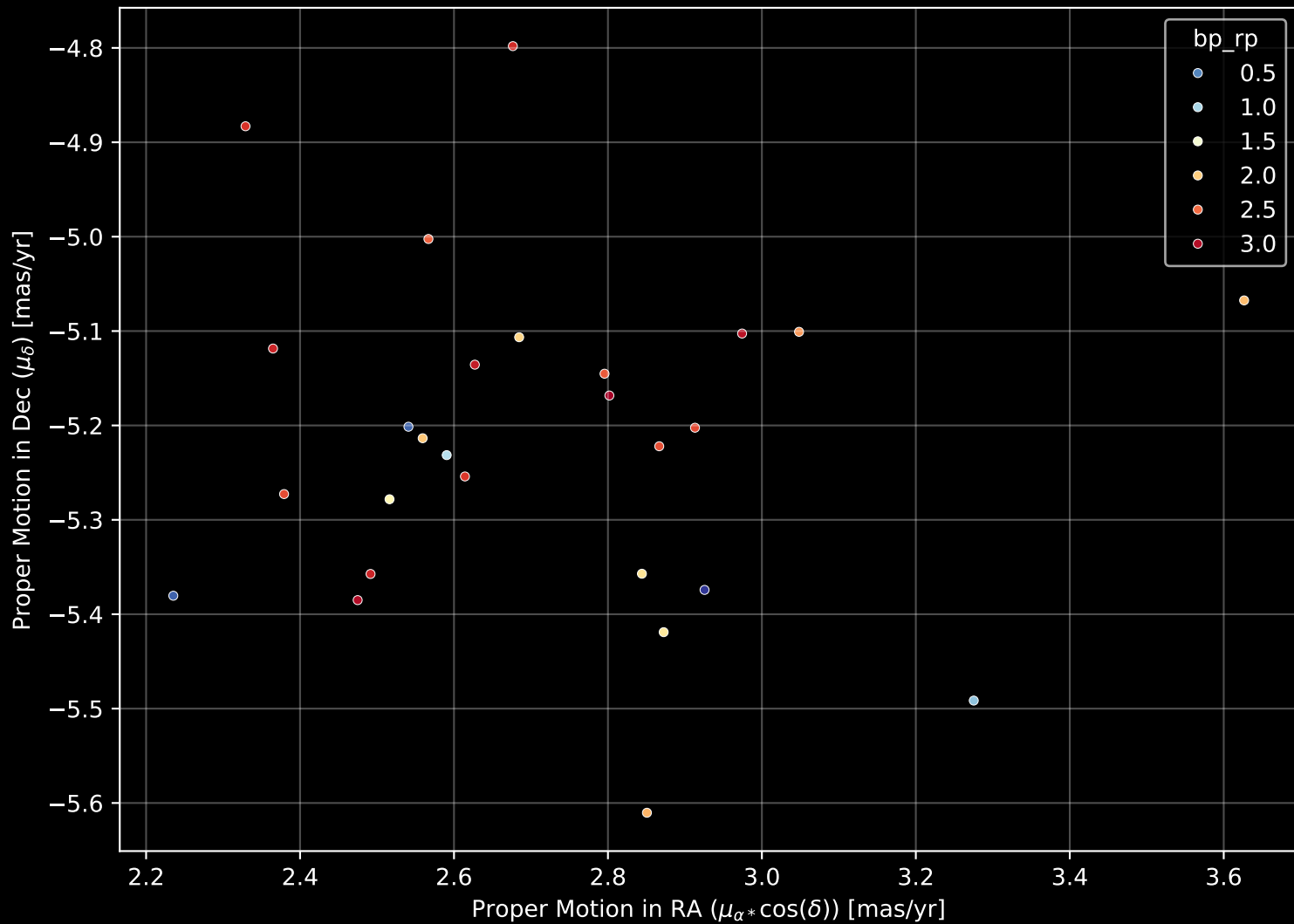
Gaia Cluster: [UBC_19] Proper Motion Diagram (n= 27)
