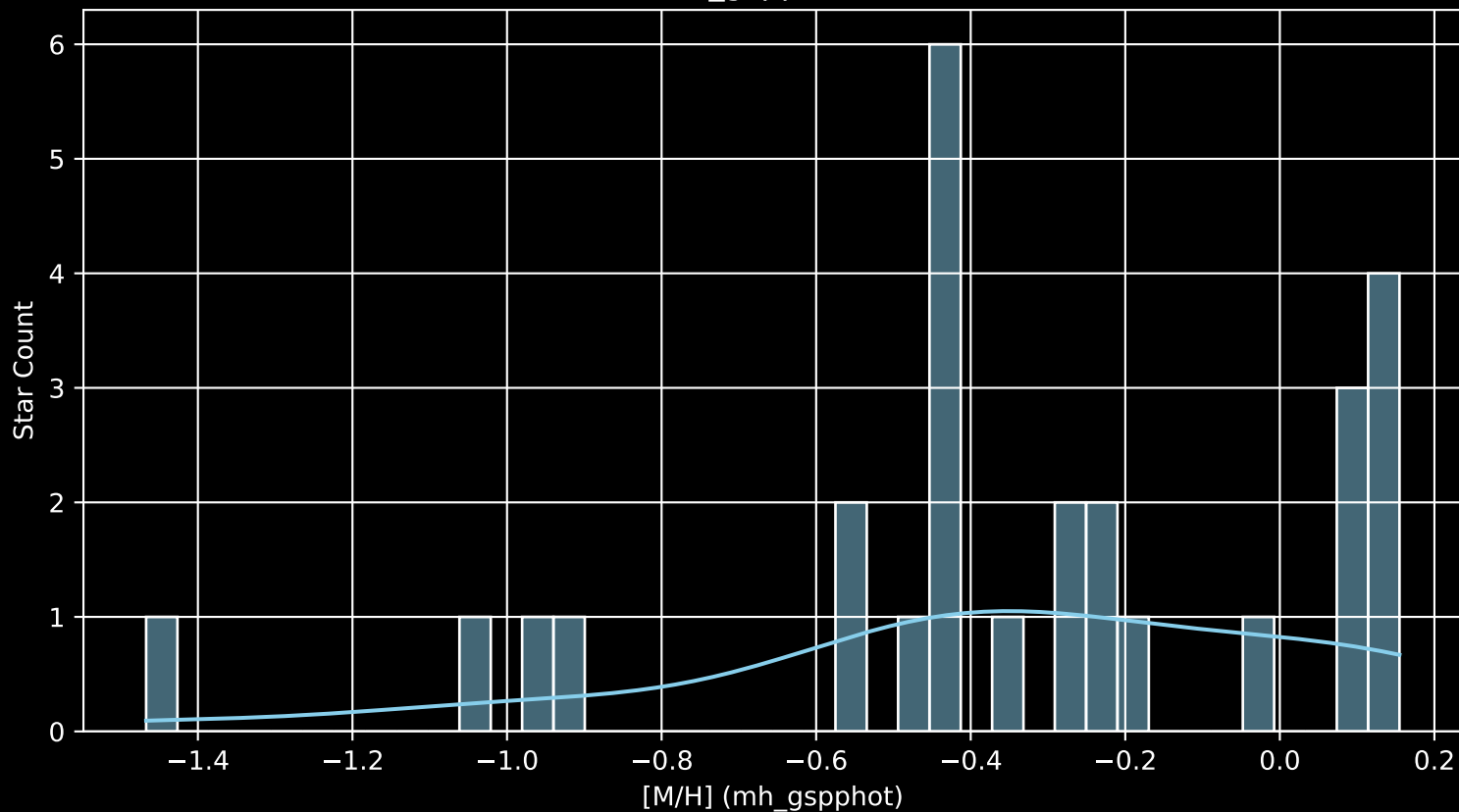
Gaia Cluster: [UBC_19 [M/H] (mh_gspphot) (n= 27)
