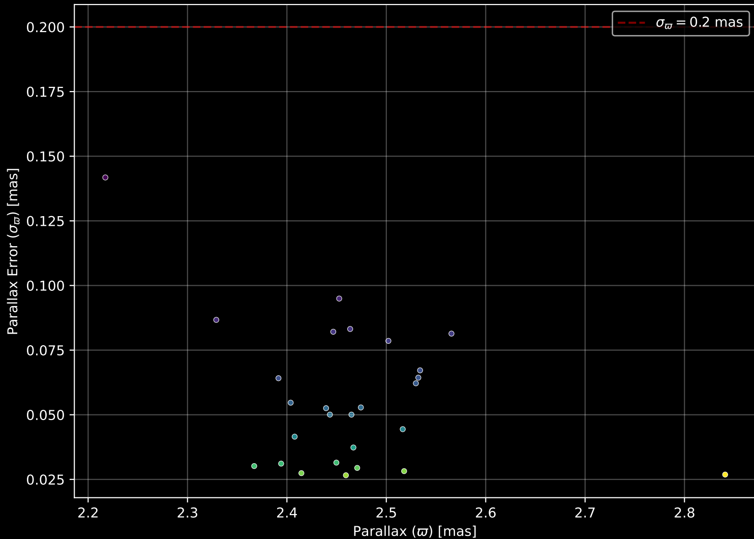
Gaia Cluster: [UBC_19] Parallax Quality (n= 27)
