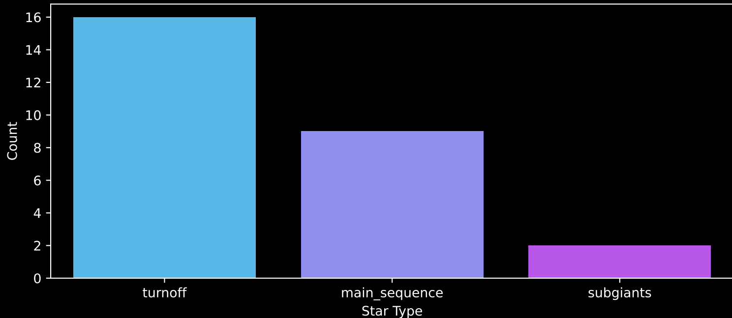
Gaia Cluster: [UBC_19] Count plot of Star Type
