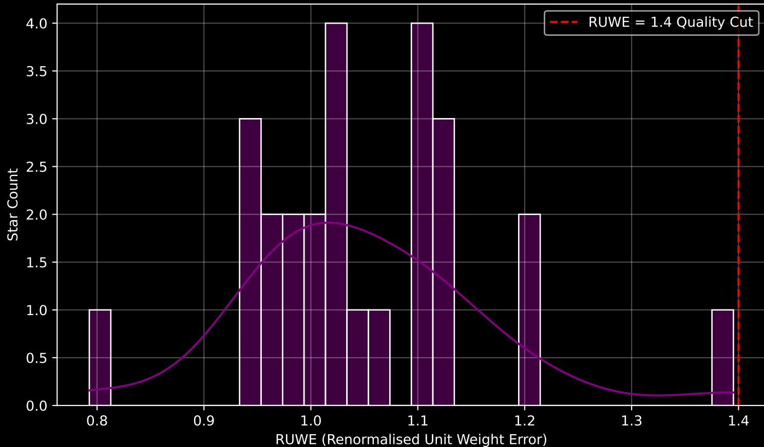
Gaia Cluster: [UBC_19] RUWE Distribution (n= 26)
