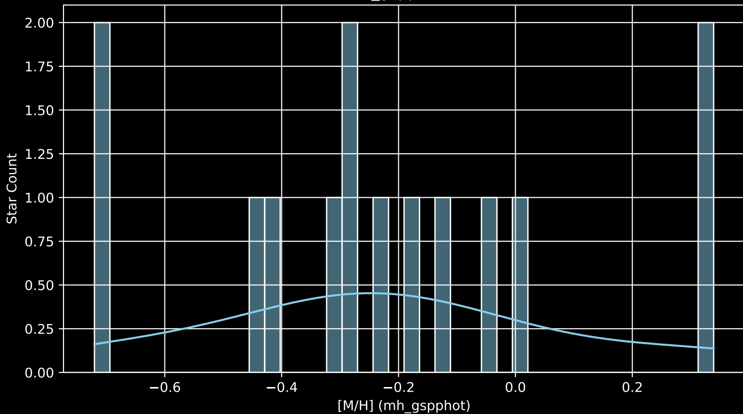
Gaia Cluster: [UBC_2 [M/H] (mh_gspphot) (n= 14)
