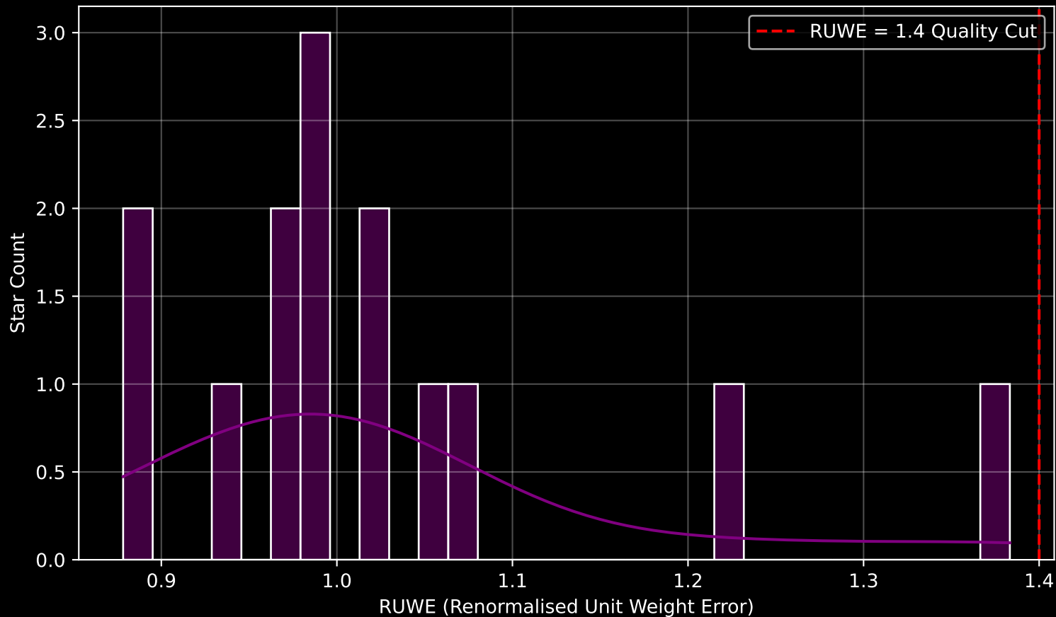
Gaia Cluster: [UBC_2] RUWE Distribution (n= 14)
