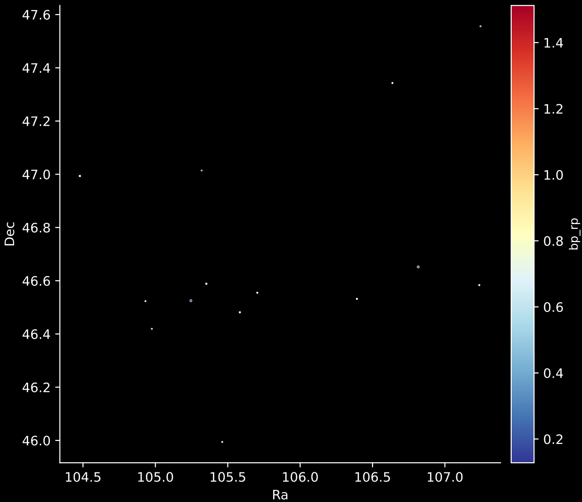
Gaia Cluster: [UBC_2] Stars: 14
