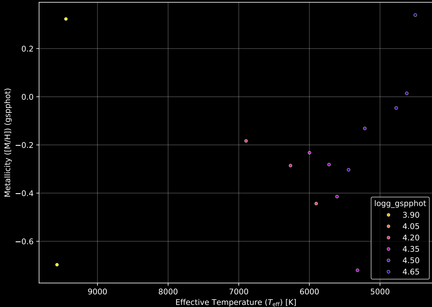
Gaia Cluster: [UBC_2] Stellar Population Parameters (n= 14)
