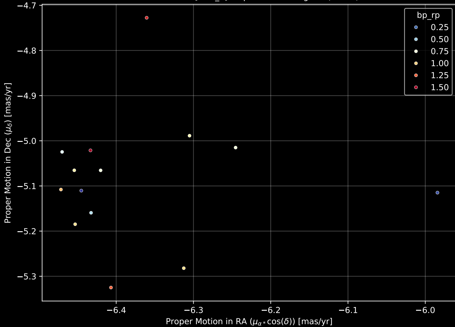
Gaia Cluster: [UBC_2] Proper Motion Diagram (n= 14)
