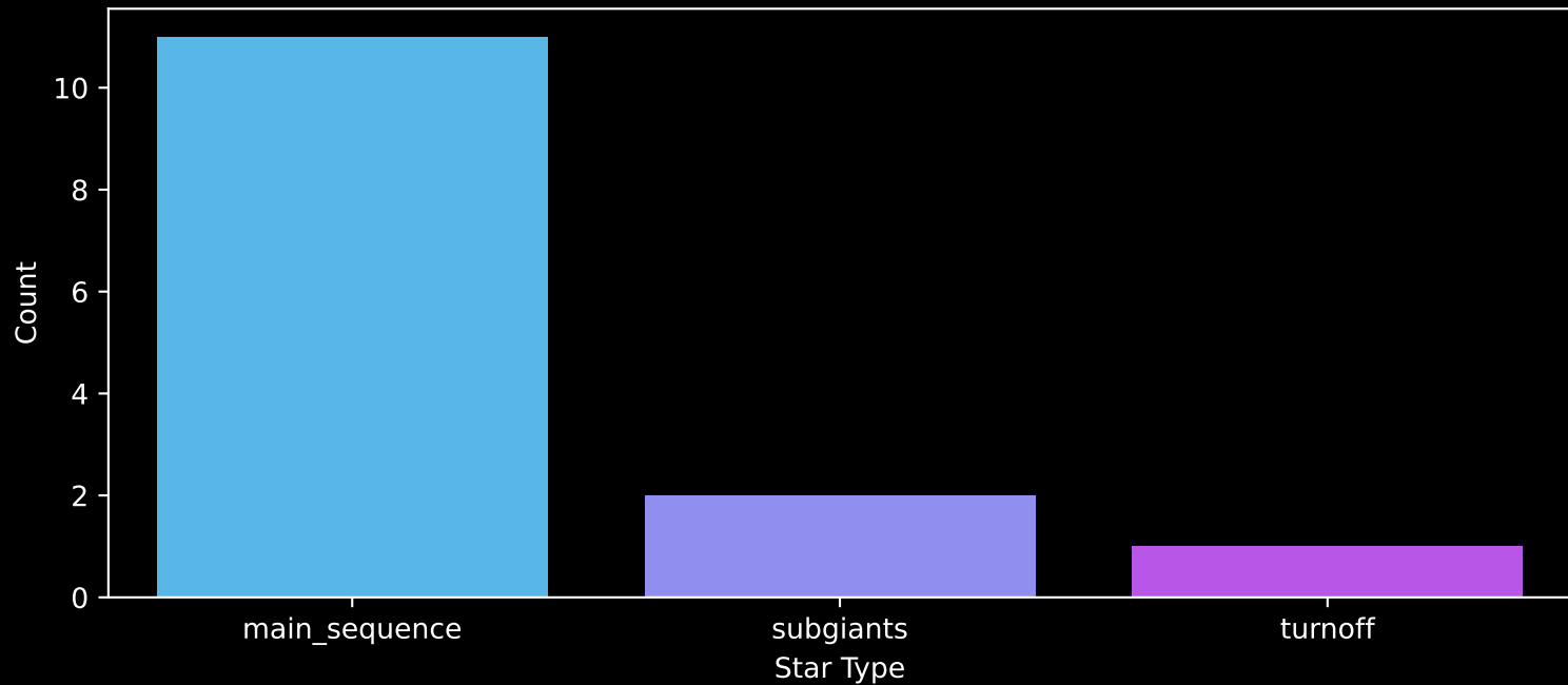
Gaia Cluster: [UBC_2] Count plot of Star Type
