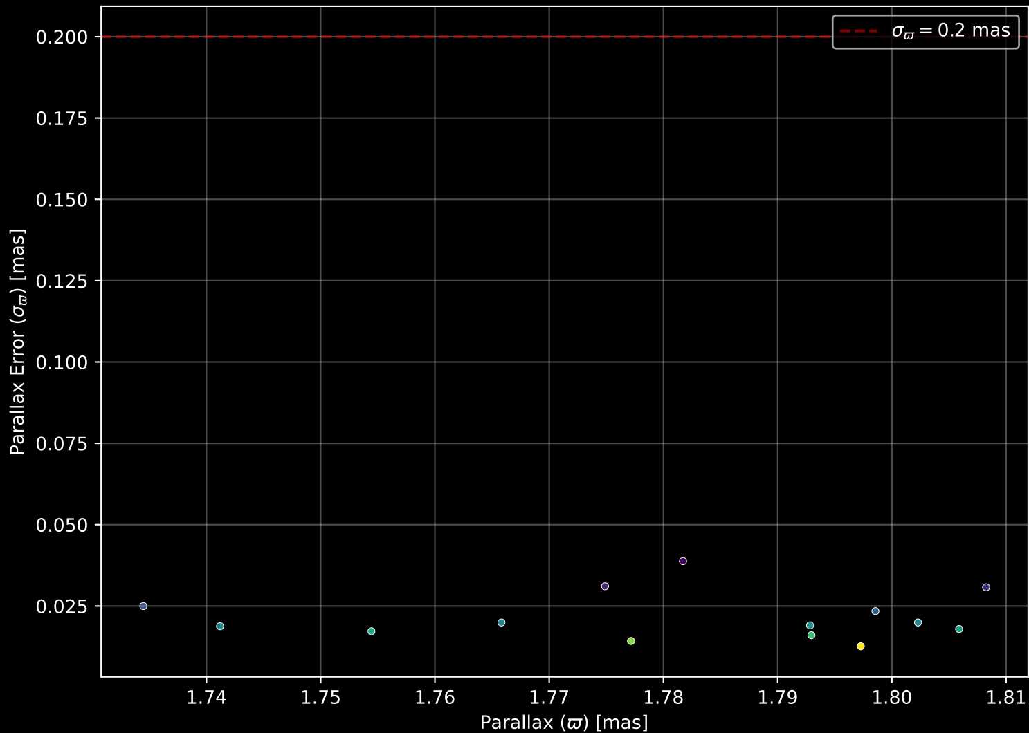
Gaia Cluster: [UBC_2] Parallax Quality (n= 14)
