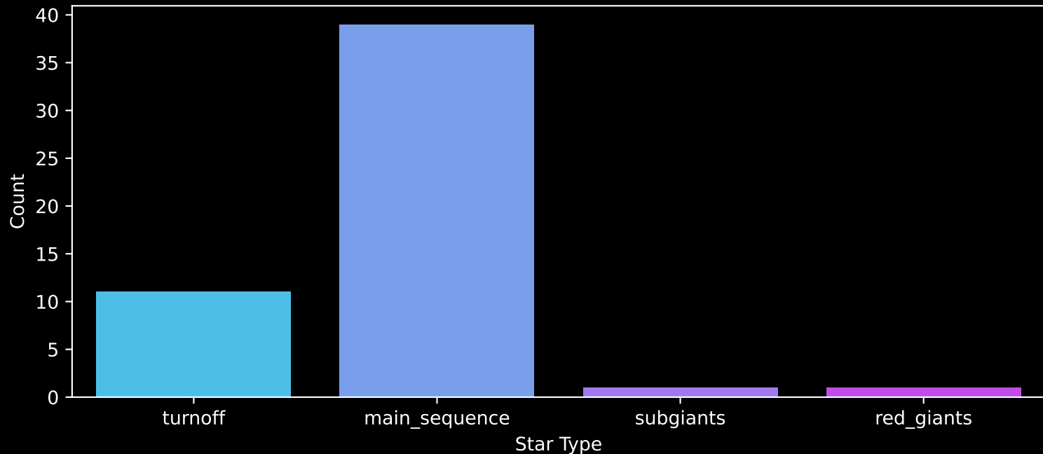
Gaia Cluster: [UBC_26] Count plot of Star Type
