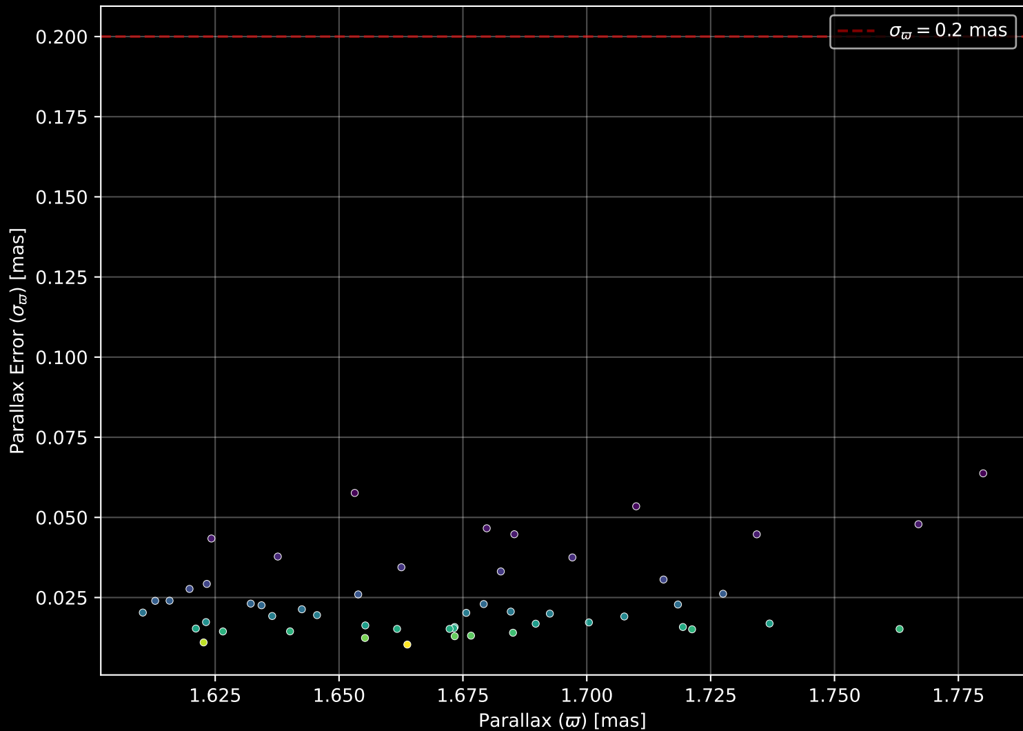
Gaia Cluster: [UBC_26] Parallax Quality (n= 52)
