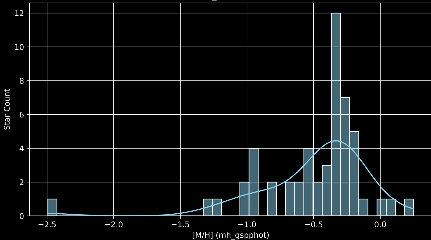
Gaia Cluster: [UBC_26 [M/H] (mh_gspphot) (n= 52)
