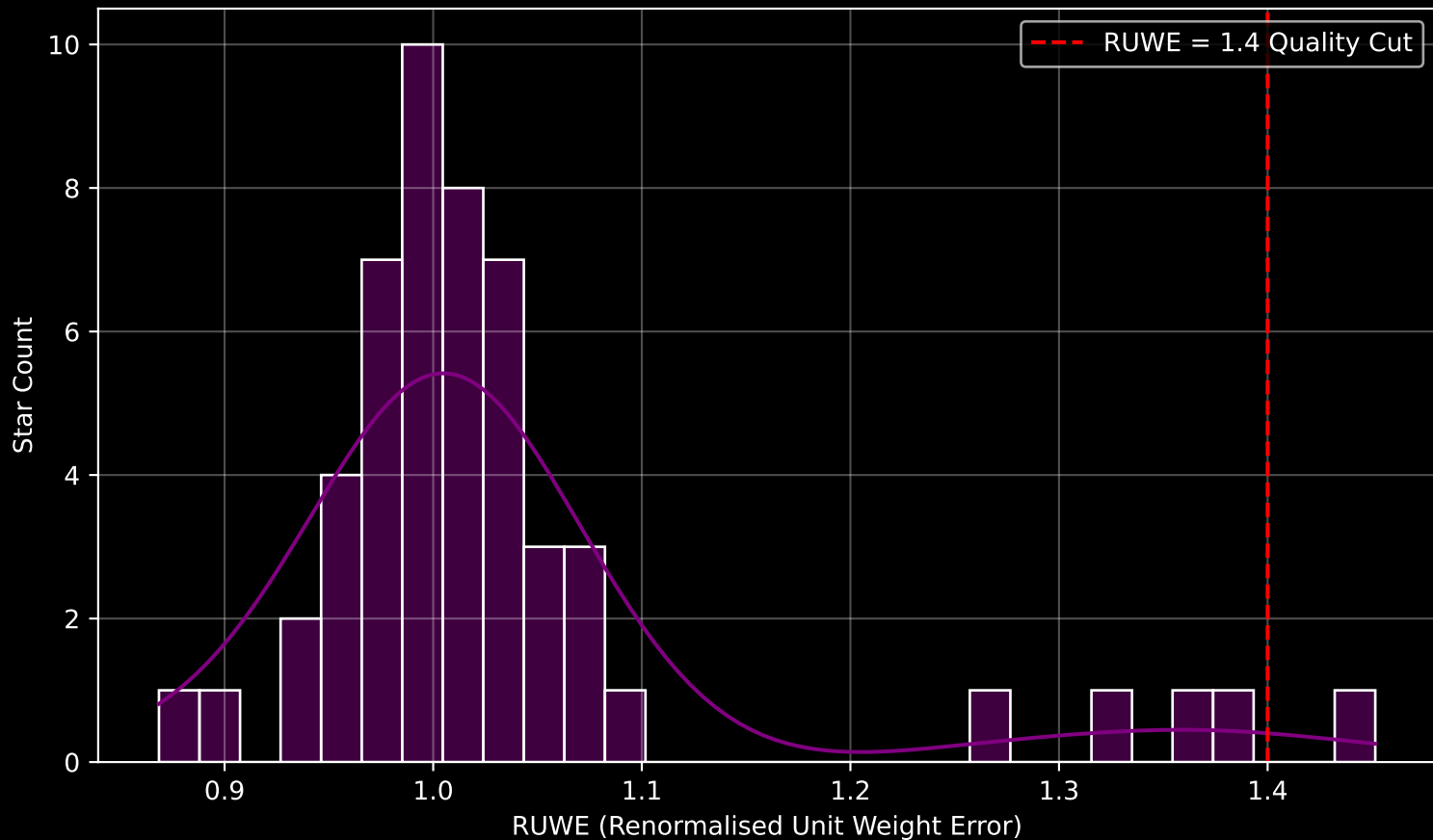
Gaia Cluster: [UBC_26] RUWE Distribution (n= 52)
