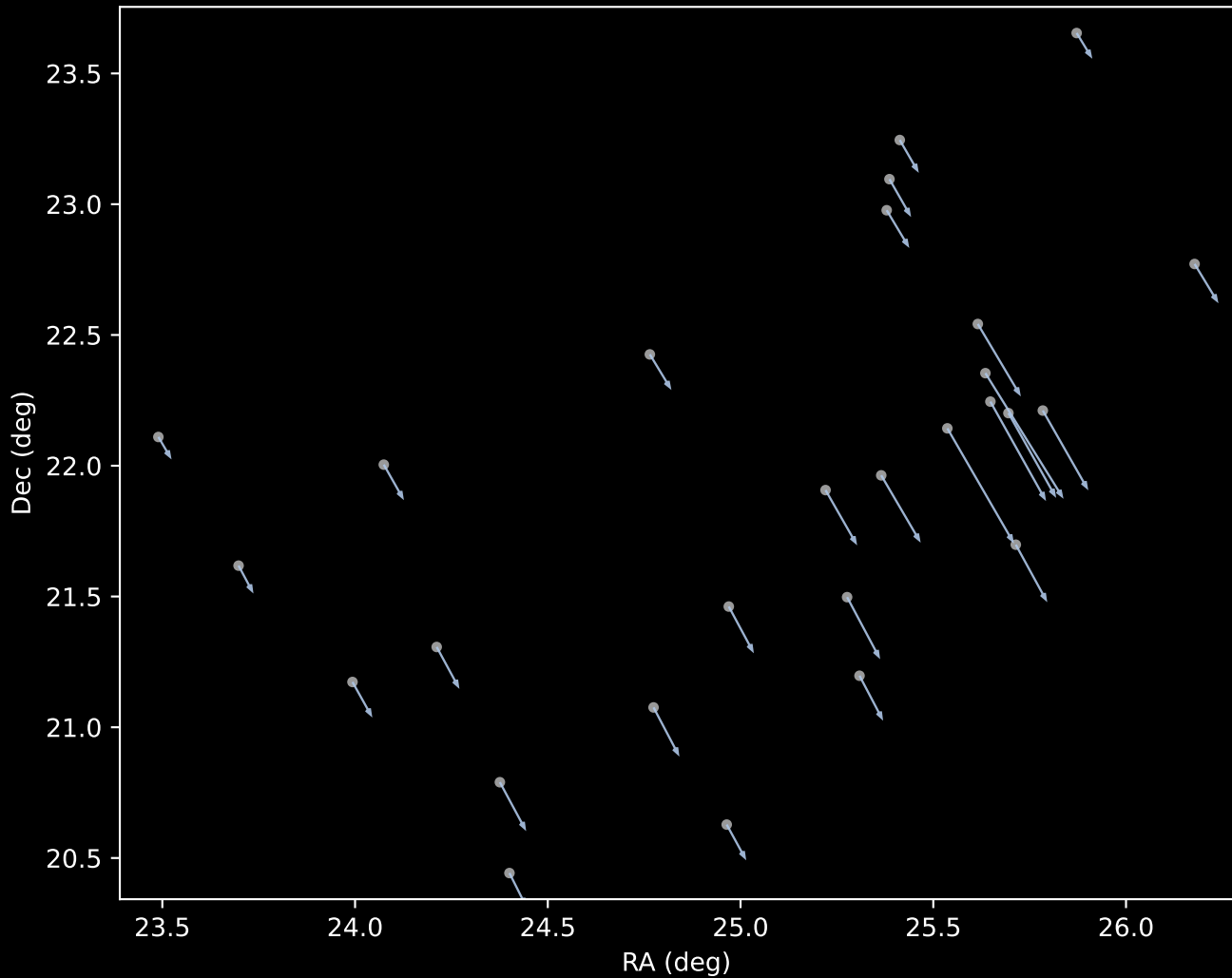
Gaia DR3 Cluster 1 Proper Motion Vectors (n=27)
