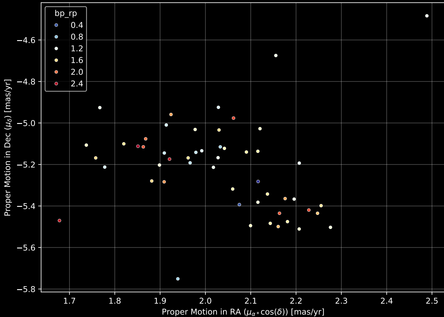
Gaia Cluster: [UBC_26] Proper Motion Diagram (n= 52)
