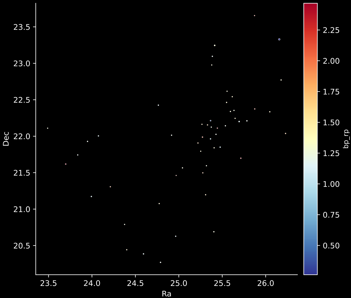
Gaia Cluster: [UBC_26] Stars: 52
