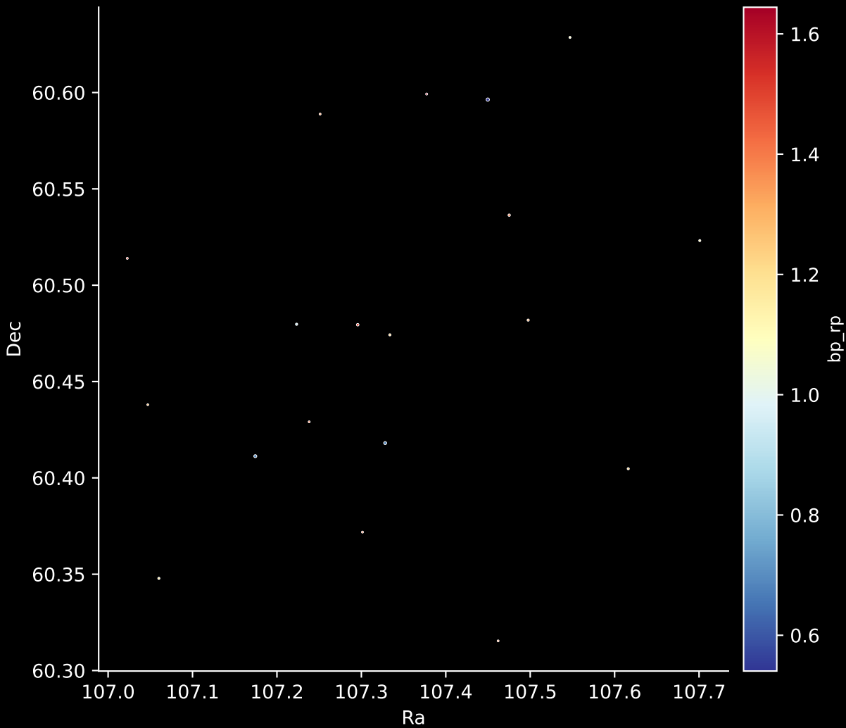
Gaia Cluster: [UBC_33] Stars: 19
