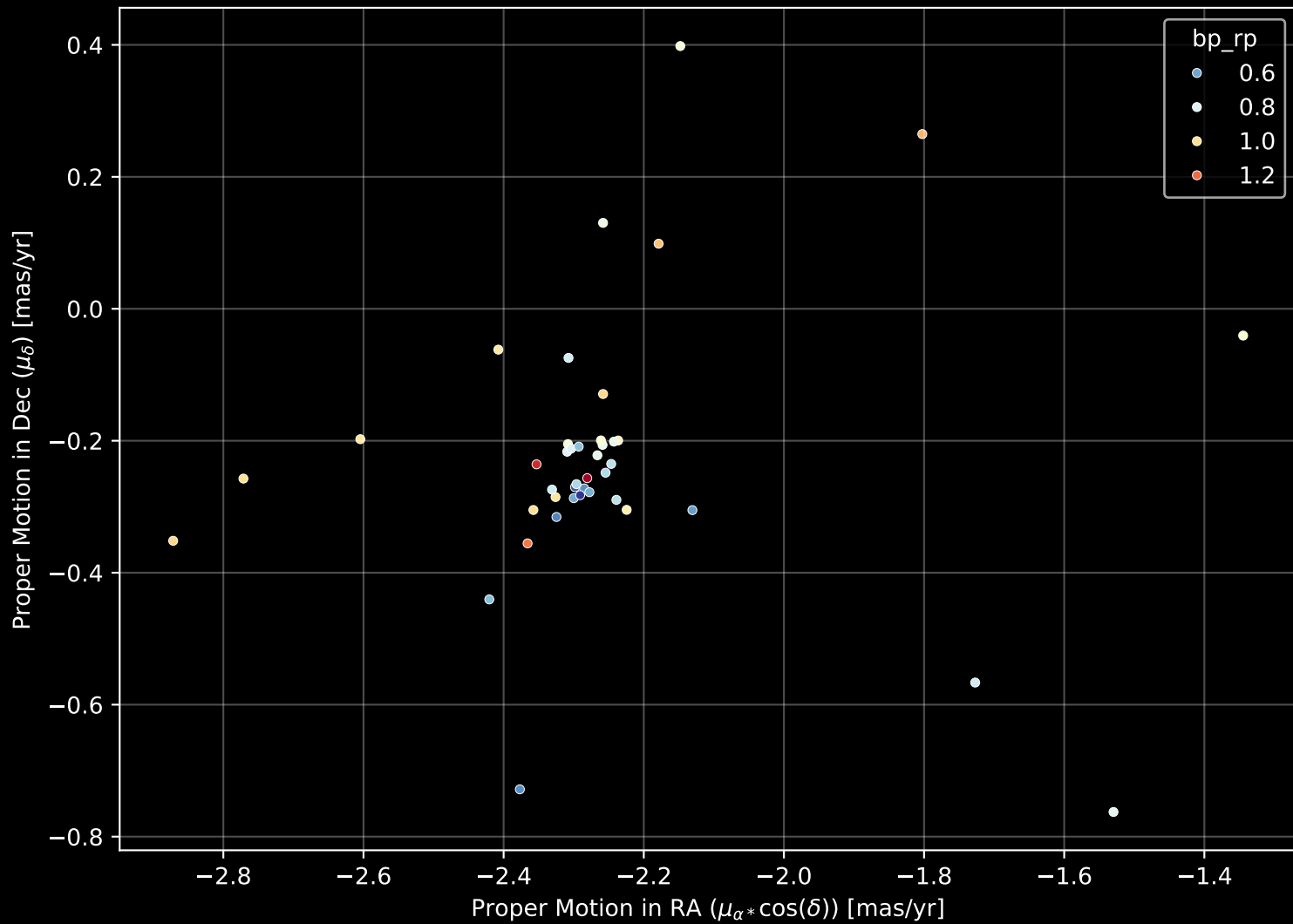
Gaia Cluster: [UBC_44] Proper Motion Diagram (n= 42)
