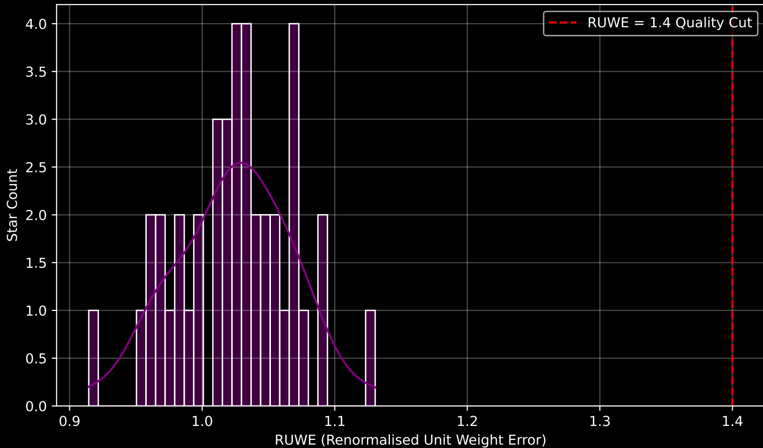
Gaia Cluster: [UBC_44] RUWE Distribution (n= 41)
