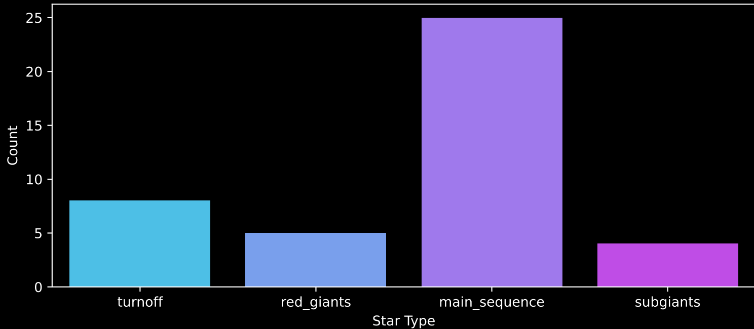
Gaia Cluster: [UBC_44] Count plot of Star Type
