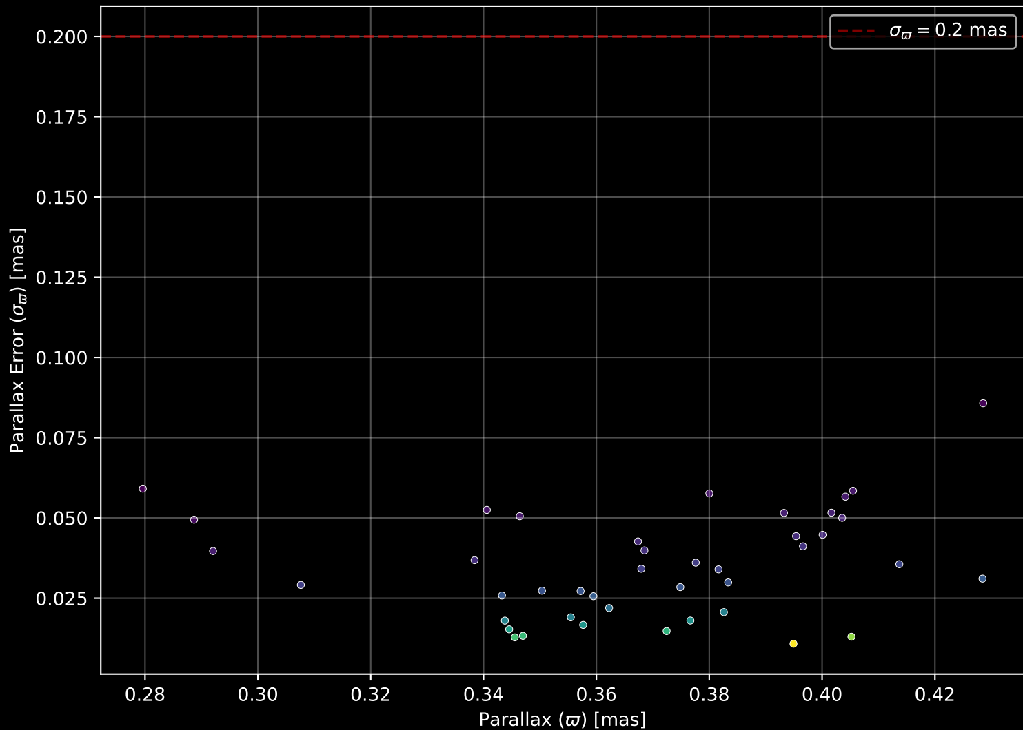
Gaia Cluster: [UBC_44] Parallax Quality (n= 42)
