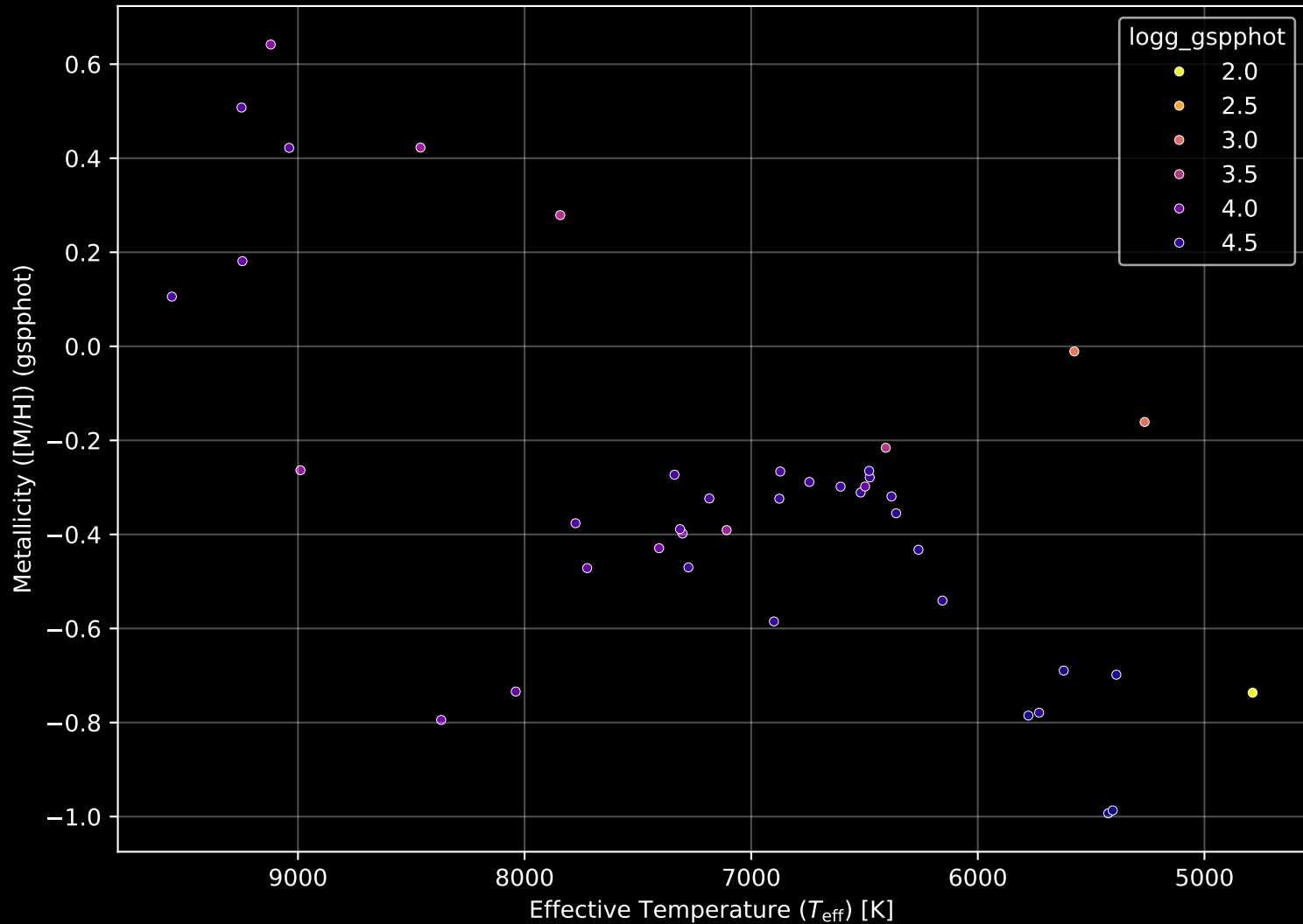
Gaia Cluster: [UBC_44] Stellar Population Parameters (n= 42)
