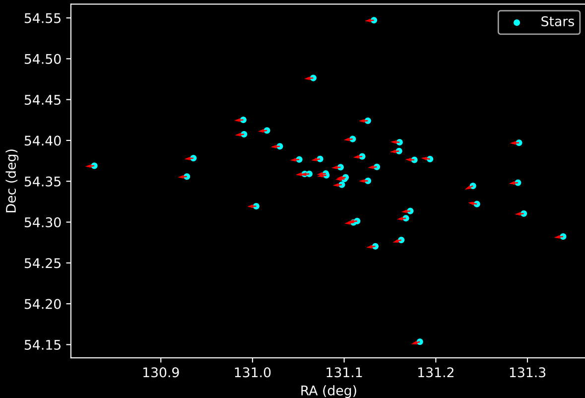
Gaia Cluster: [UBC_44] Proper Motion Vectors for Gaia Star Field (n= 42)
