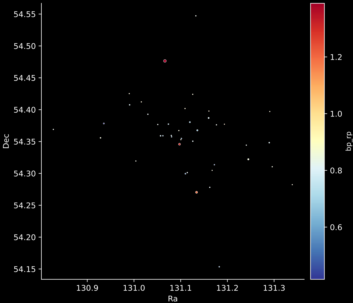
Gaia Cluster: [UBC_44] Stars: 42
