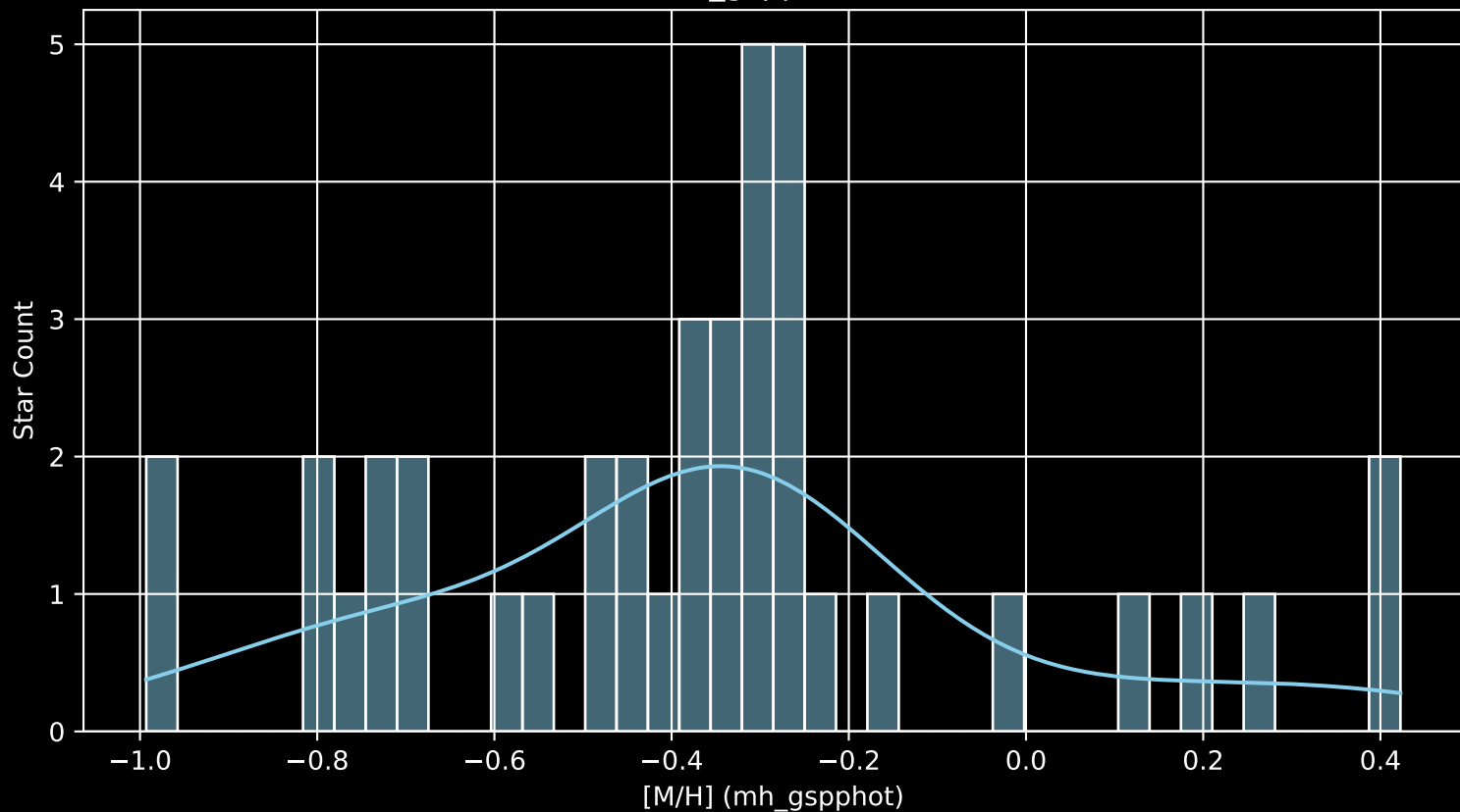
Gaia Cluster: [UBC_44 [M/H] (mh_gspphot) ( \bar{n}= 40 )
