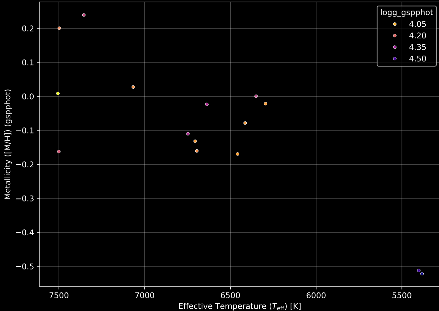
Gaia Cluster: [UBC_47] Stellar Population Parameters (n= 15)
