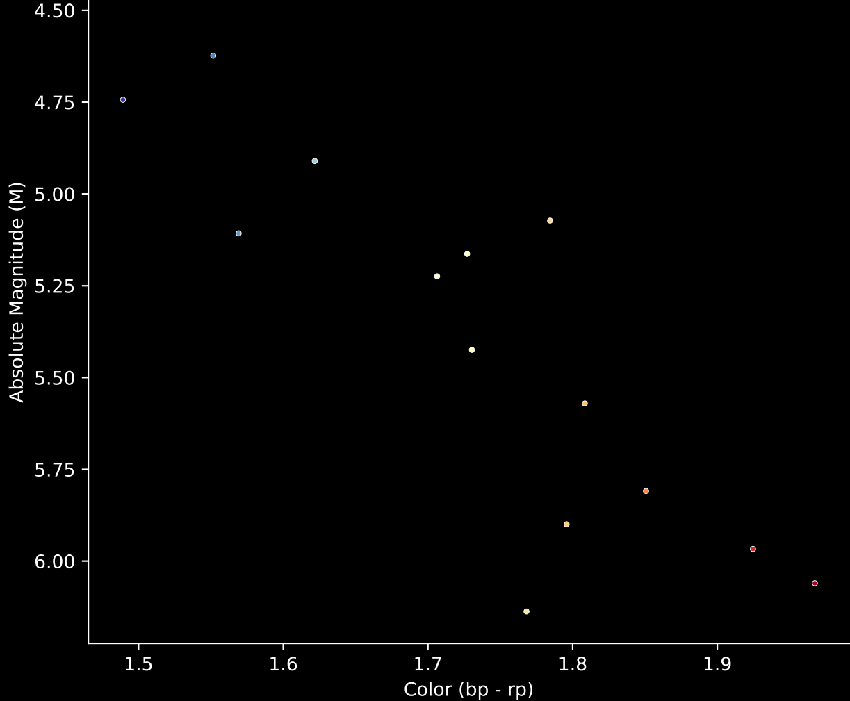
Gaia Cluster: [UBC_47] Stars (n= 15) Hertzprung-Russel Diagram
