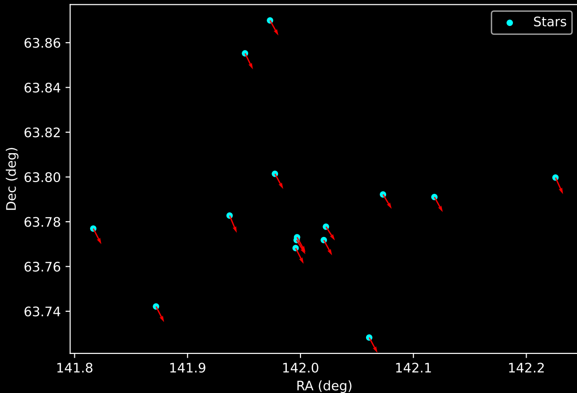
Gaia Cluster: [UBC_47] Proper Motion Vectors for Gaia Star Field (n= 15)
