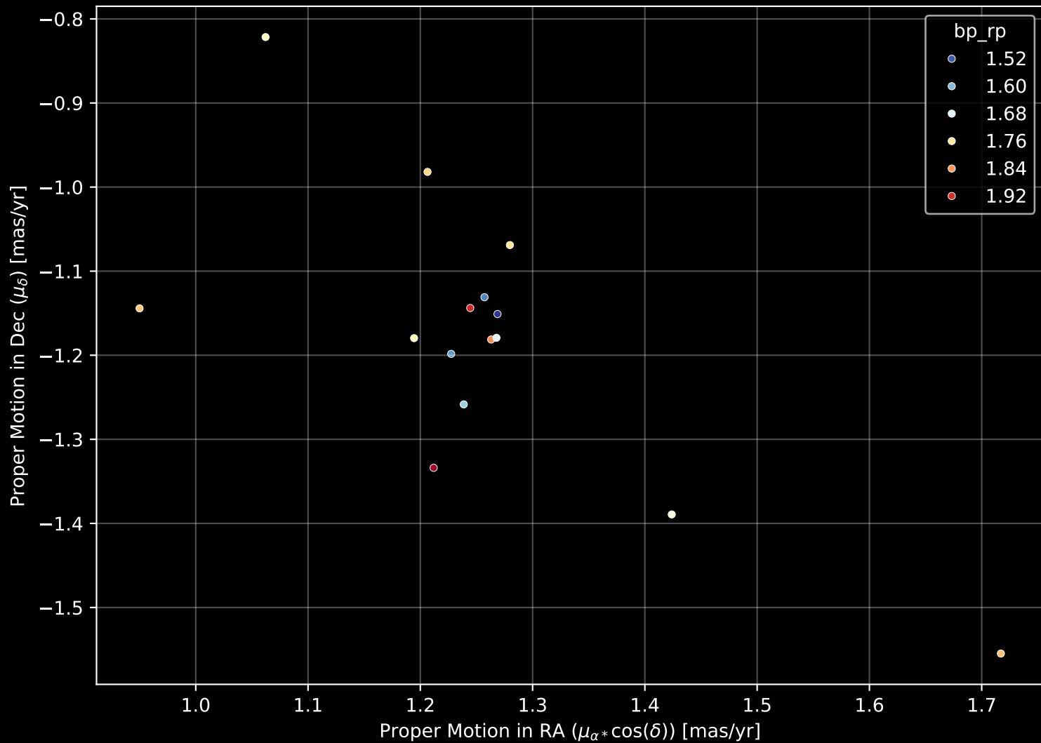
Gaia Cluster: [UBC_47] Proper Motion Diagram (n= 15)
