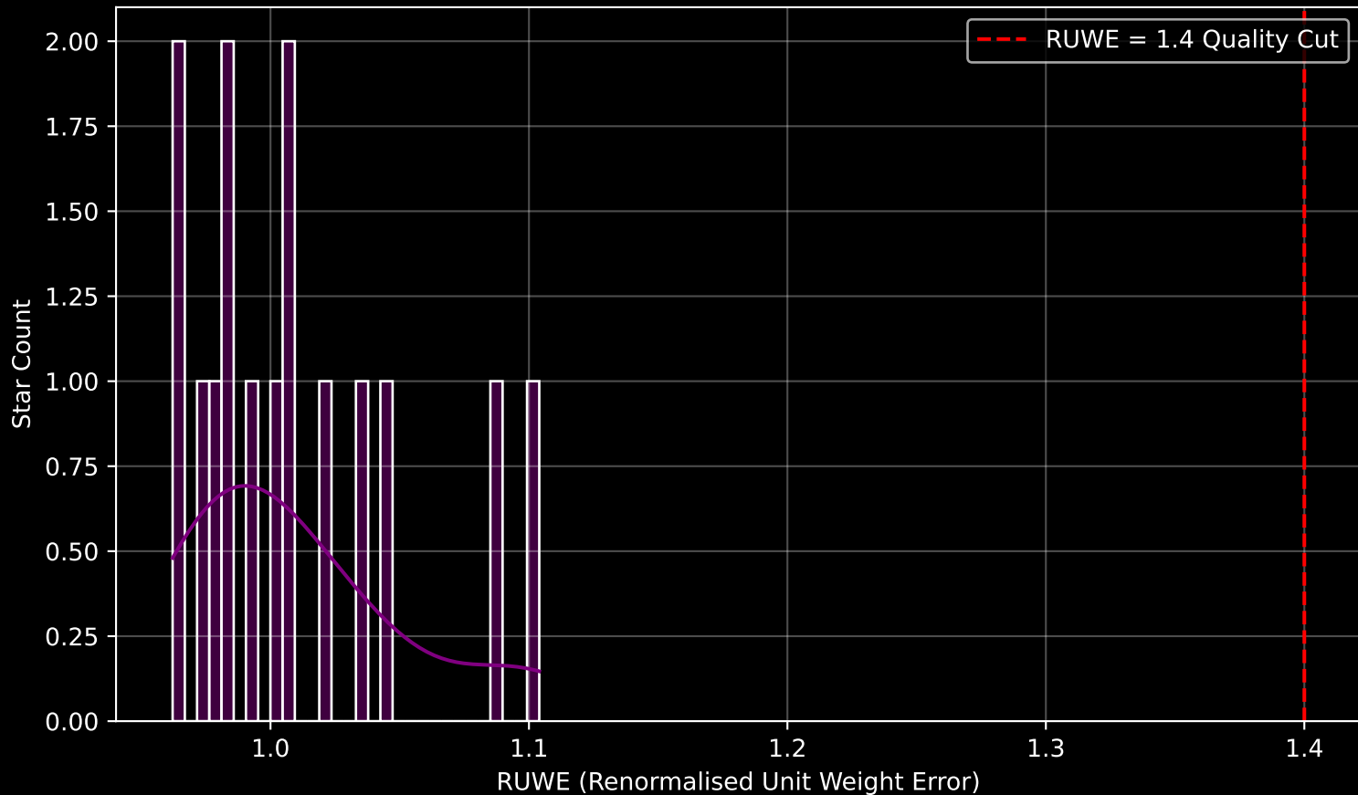
Gaia Cluster: [UBC_47] RUWE Distribution (n= 15)
