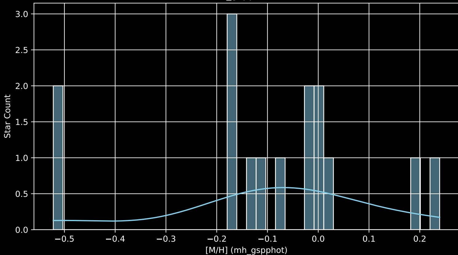
Gaia Cluster: [UBC_47 [M/H] (mh_gspphot) ( n = 15 )
