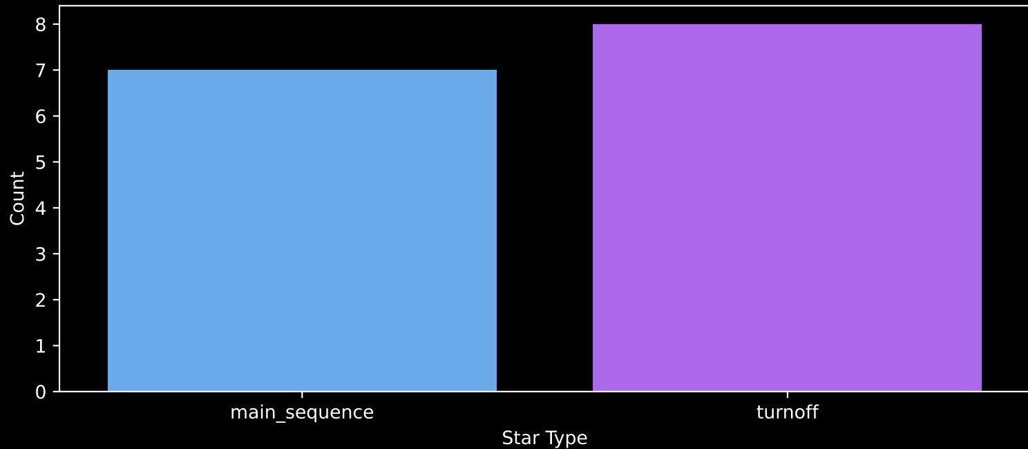
Gaia Cluster: [UBC_47] Count plot of Star Type
