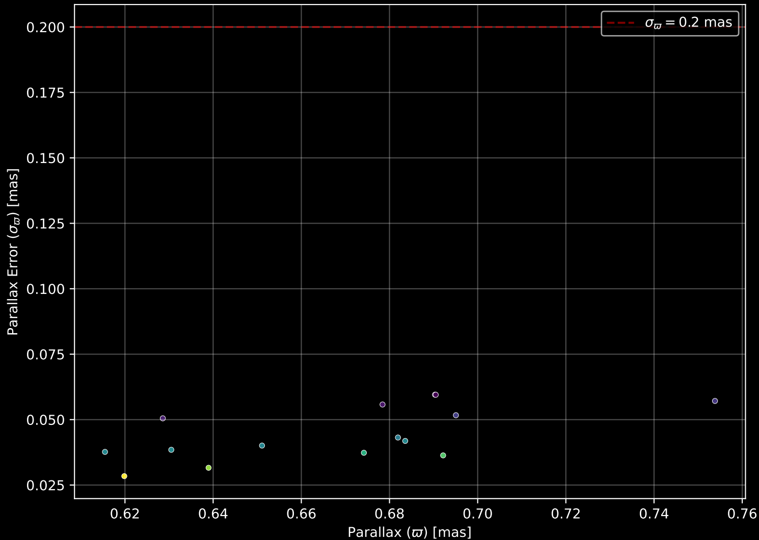
Gaia Cluster: [UBC_47] Parallax Quality (n= 15)
