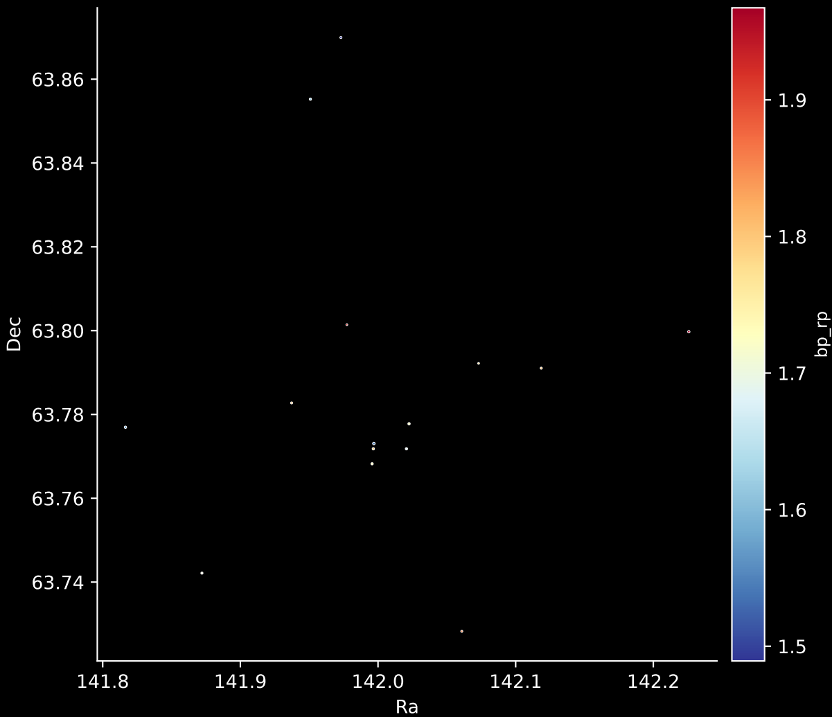
Gaia Cluster: [UBC_47] Stars: 15
