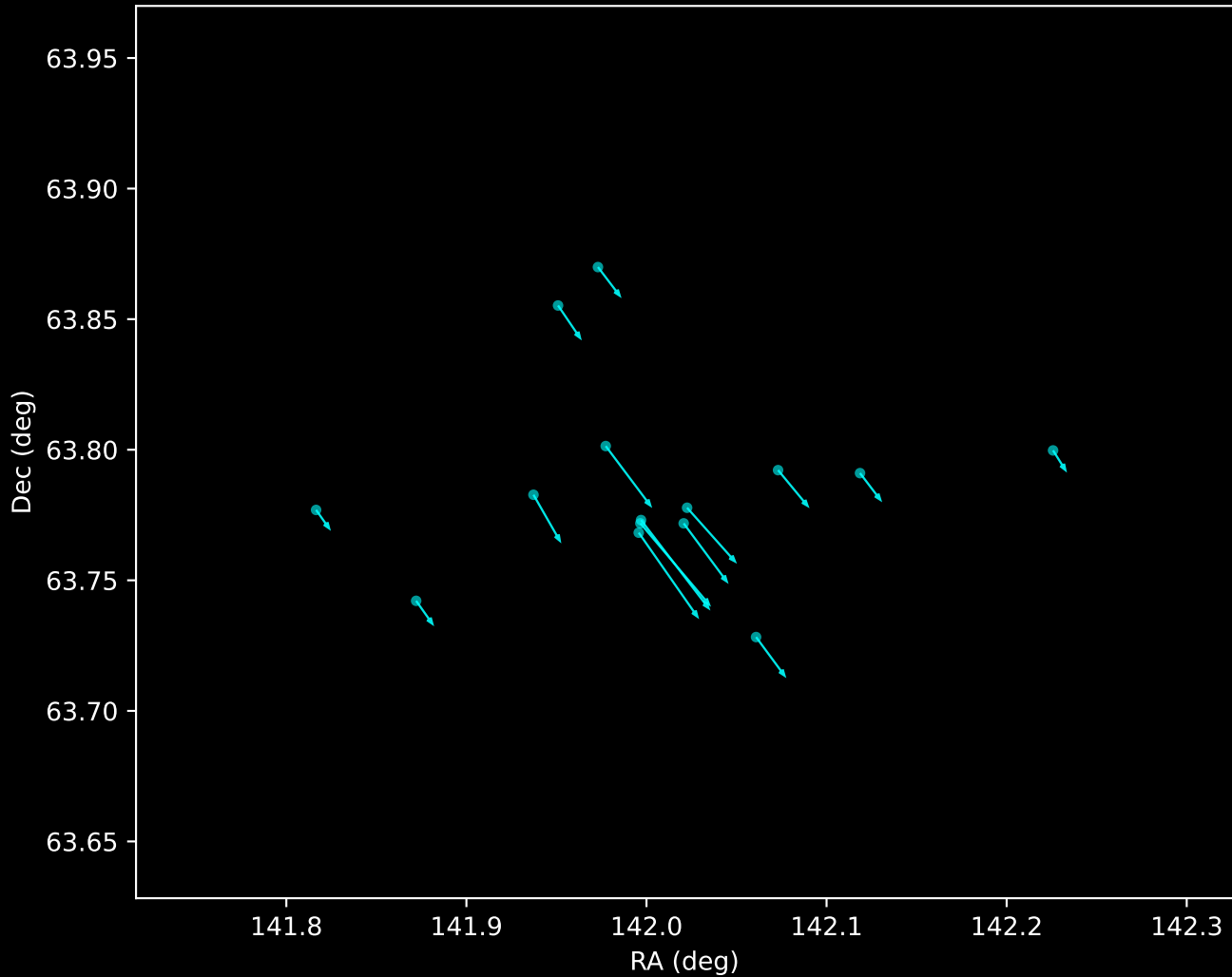
Gaia DR3 Noise Stream Proper Motion Vectors (n=15)
