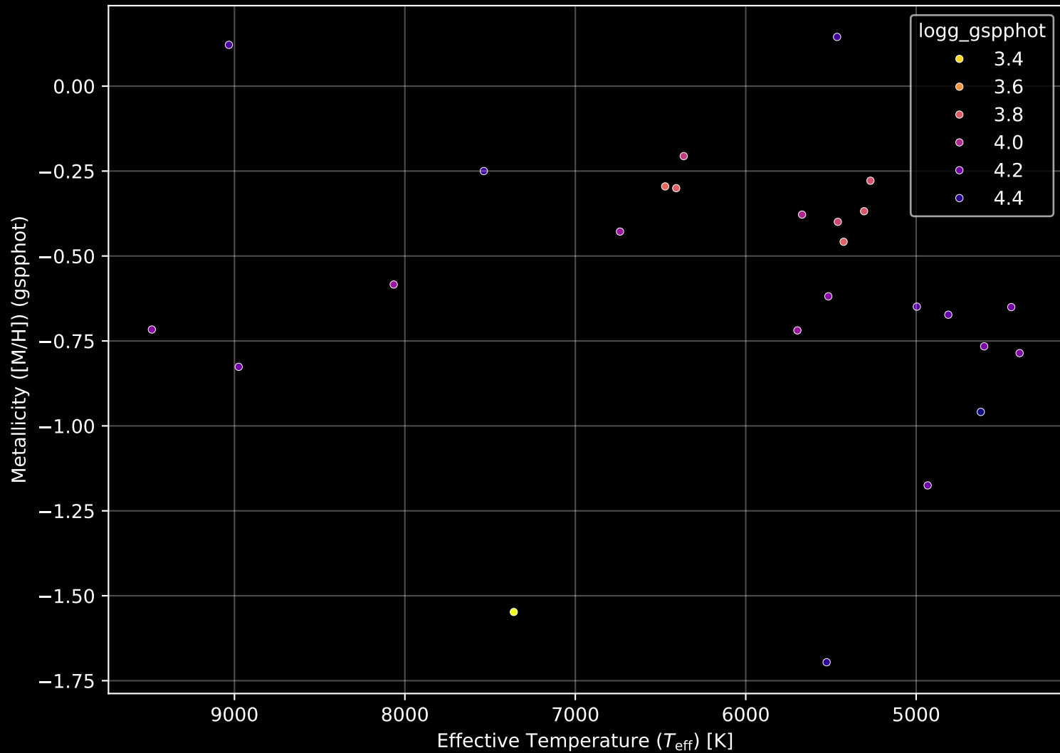
Gaia Cluster: [UBC_51] Stellar Population Parameters (n= 26)
