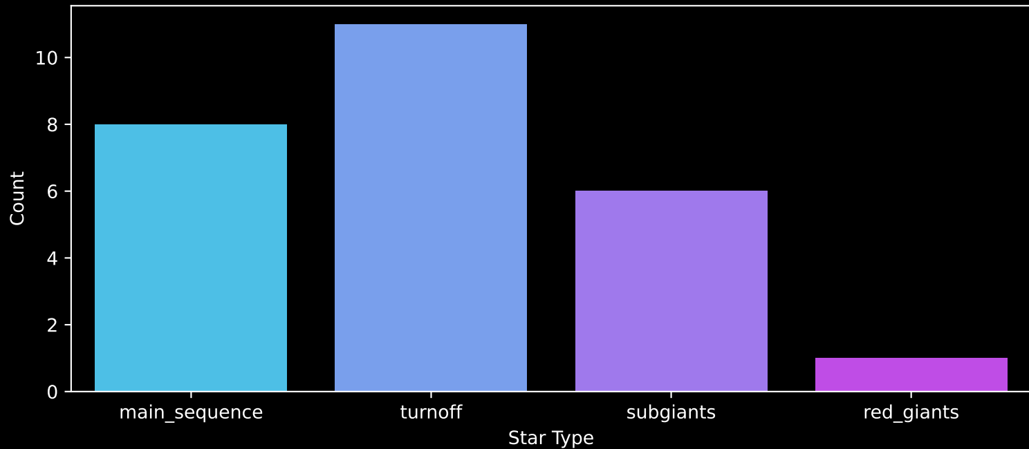
Gaia Cluster: [UBC_51] Count plot of Star Type
