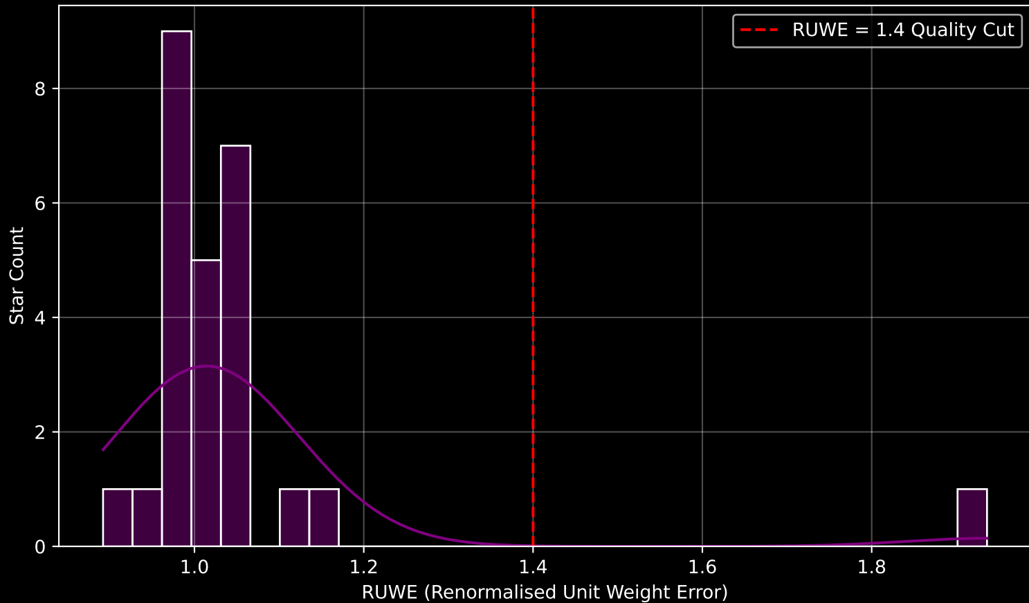
Gaia Cluster: [UBC_51] RUWE Distribution (n= 26)
