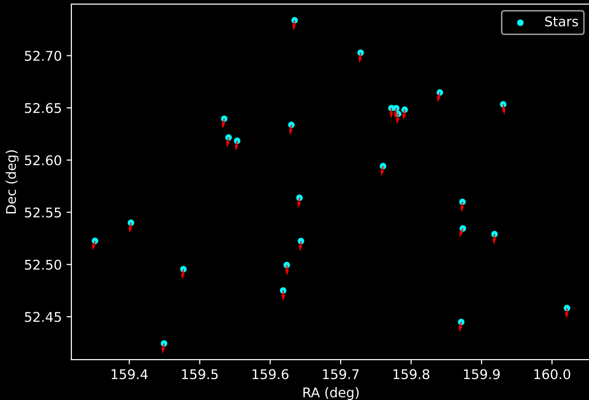
Gaia Cluster: [UBC_51] Proper Motion Vectors for Gaia Star Field (n= 26)
