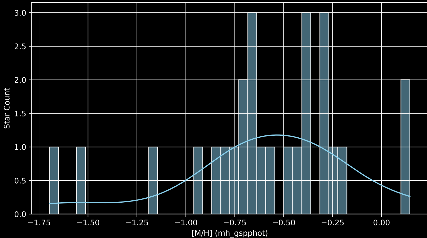
Gaia Cluster: [UBC_51 [M/H] (mh_gspphot) (n= 26)
