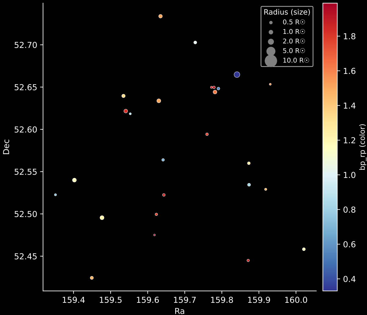
Gaia Cluster: [UBC_51] Stars: 26
