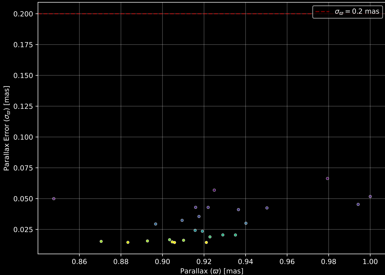
Gaia Cluster: [UBC_51] Parallax Quality (n= 26)
