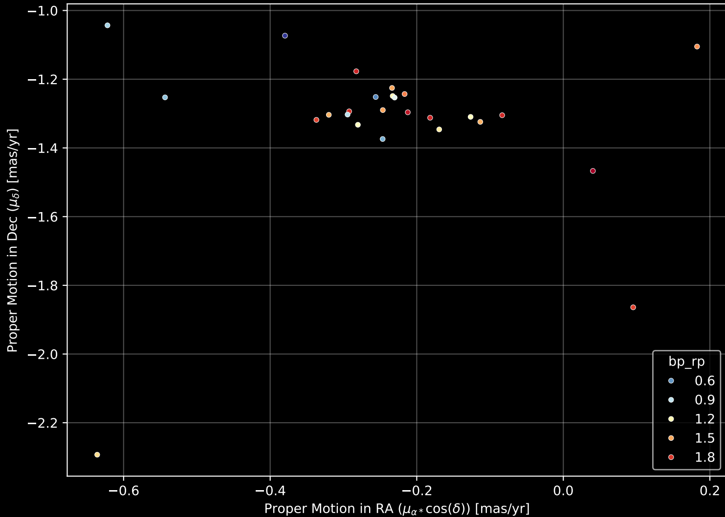
Gaia Cluster: [UBC_51] Proper Motion Diagram (n= 26)
