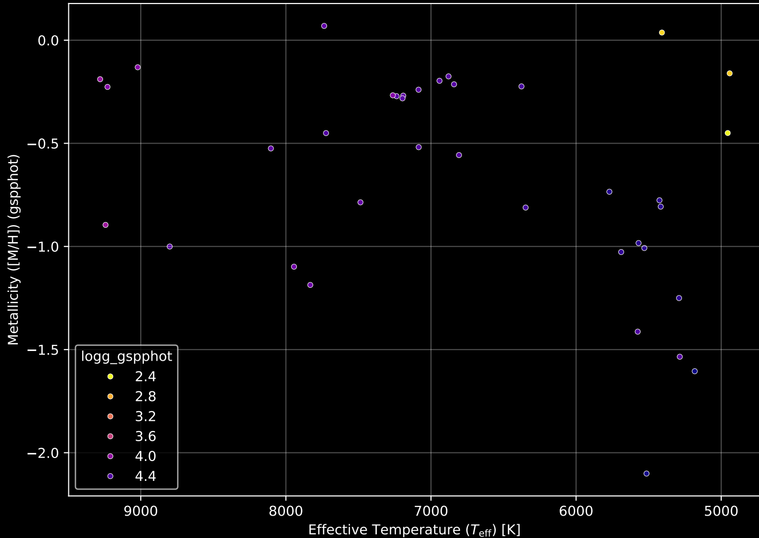
Gaia Cluster: [UBC_53] Stellar Population Parameters (n= 37)
