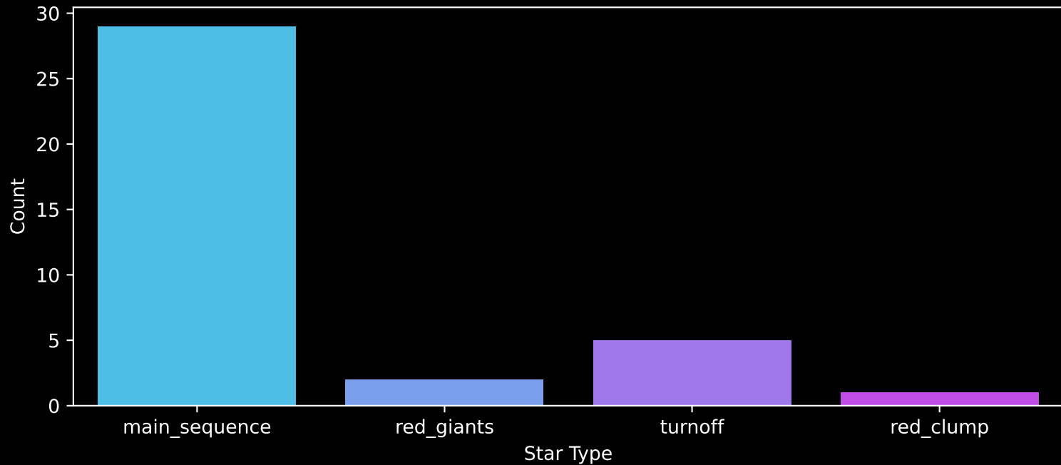
Gaia Cluster: [UBC_53] Count plot of Star Type
