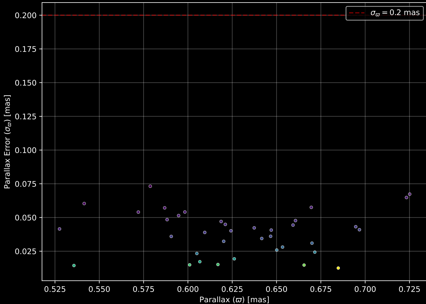
Gaia Cluster: [UBC_53] Parallax Quality (n= 37)
