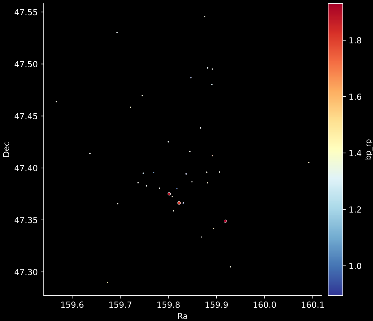
Gaia Cluster: [UBC_53] Stars: 37
