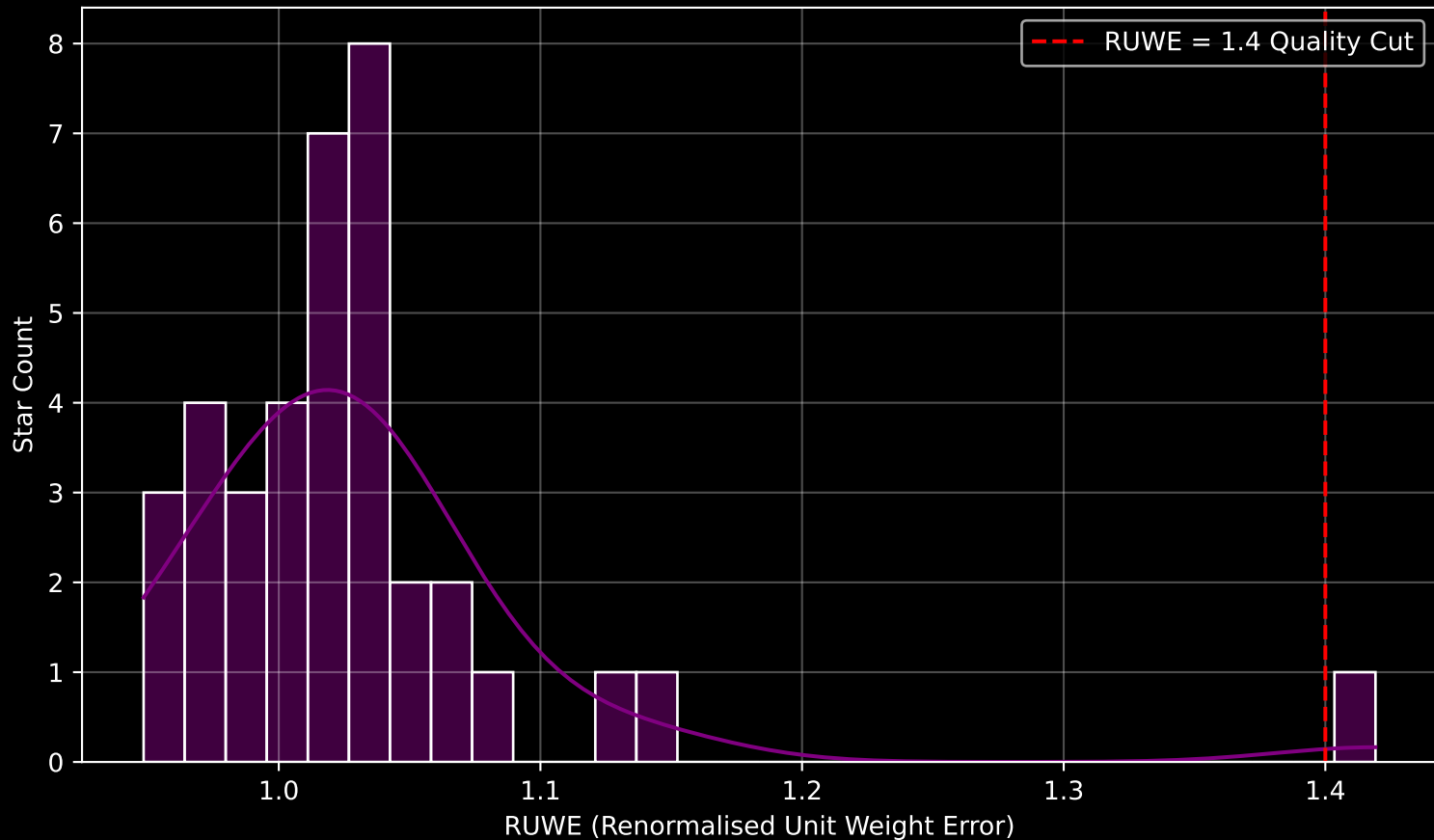
Gaia Cluster: [UBC_53] RUWE Distribution (n= 37)
