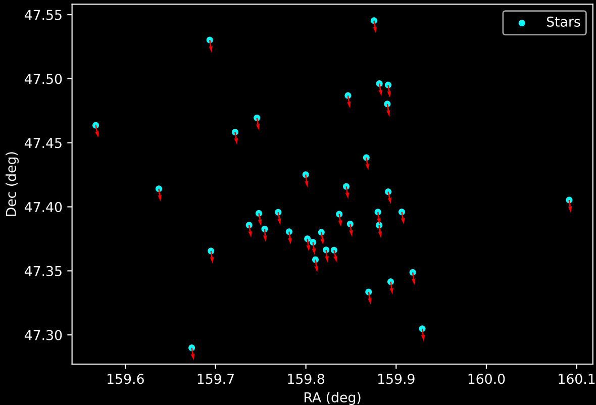
Gaia Cluster: [UBC_53] Proper Motion Vectors for Gaia Star Field (n= 37)
