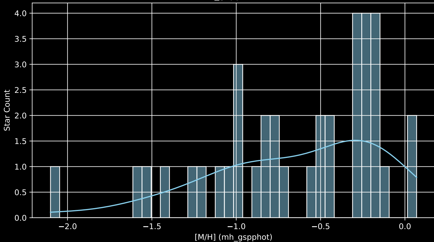
Gaia Cluster: [UBC_53 [M/H] (mh_gspphot) (n= 37)
