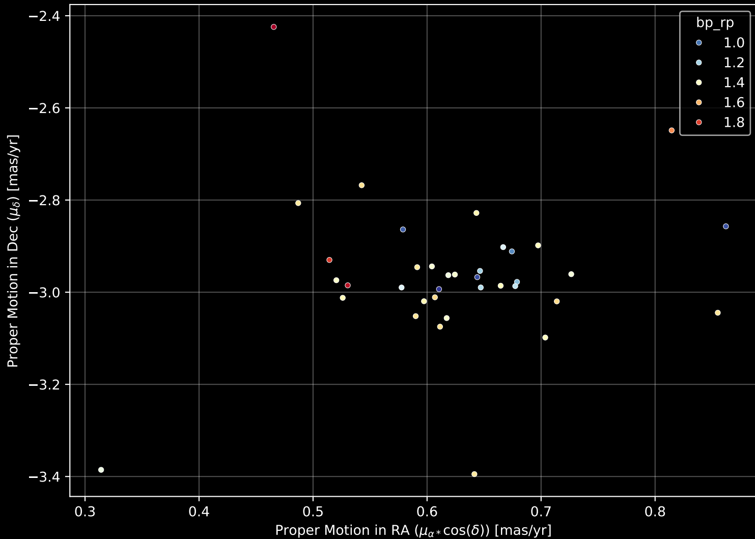
Gaia Cluster: [UBC_53] Proper Motion Diagram (n= 37)
