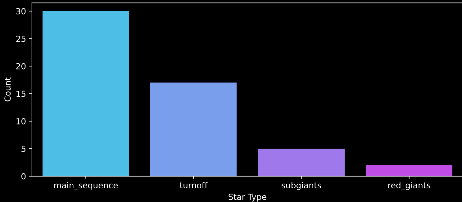
Gaia Cluster: [UBC_55] Count plot of Star Type
