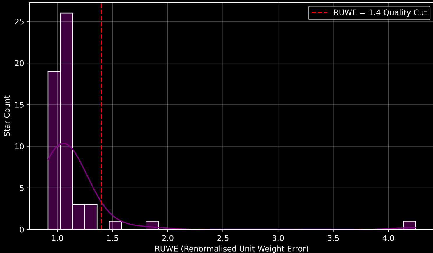
Gaia Cluster: [UBC_55] RUWE Distribution (n= 54)
