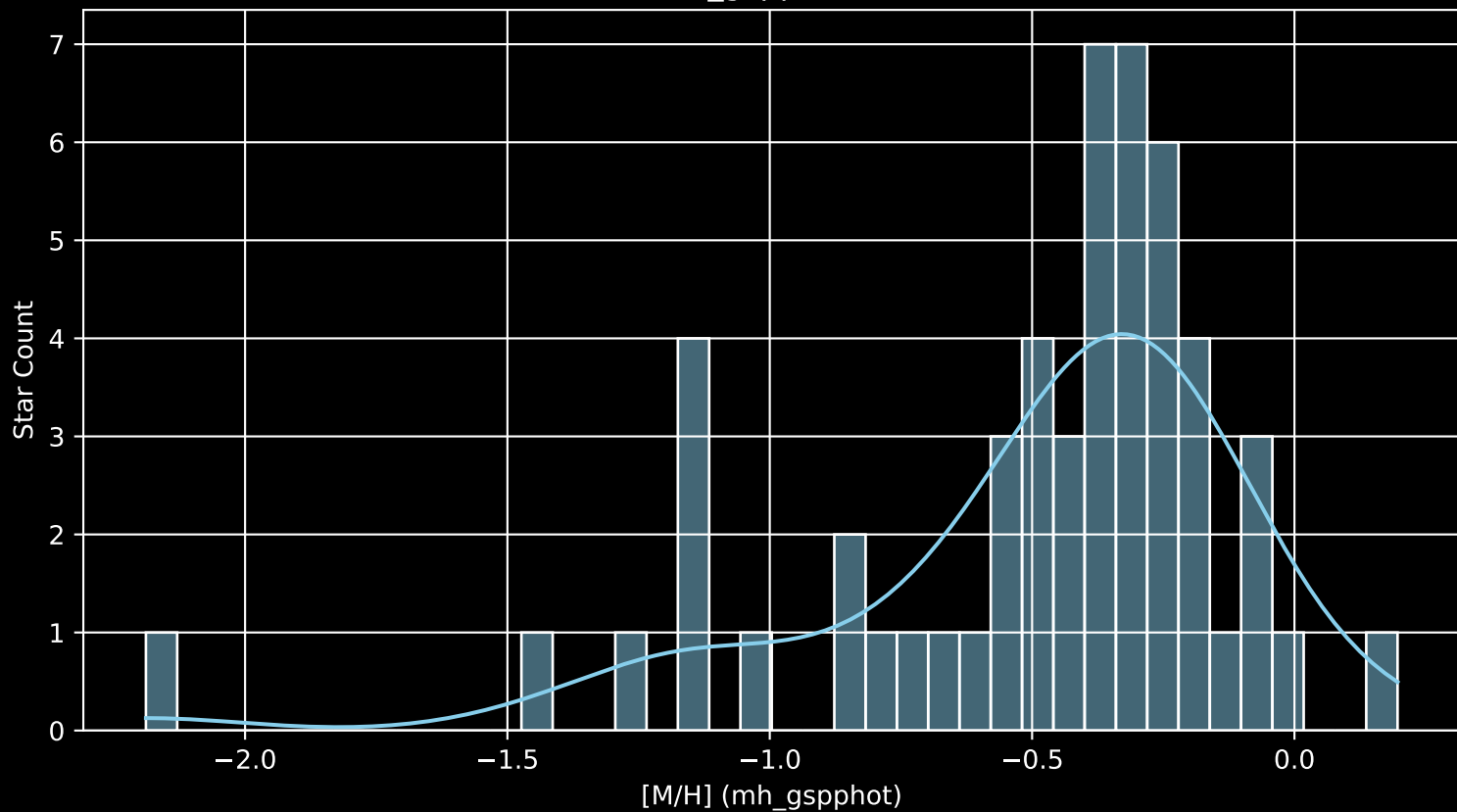
Gaia Cluster: [UBC_55 [M/H] (mh_gspphot) (n= 54)
