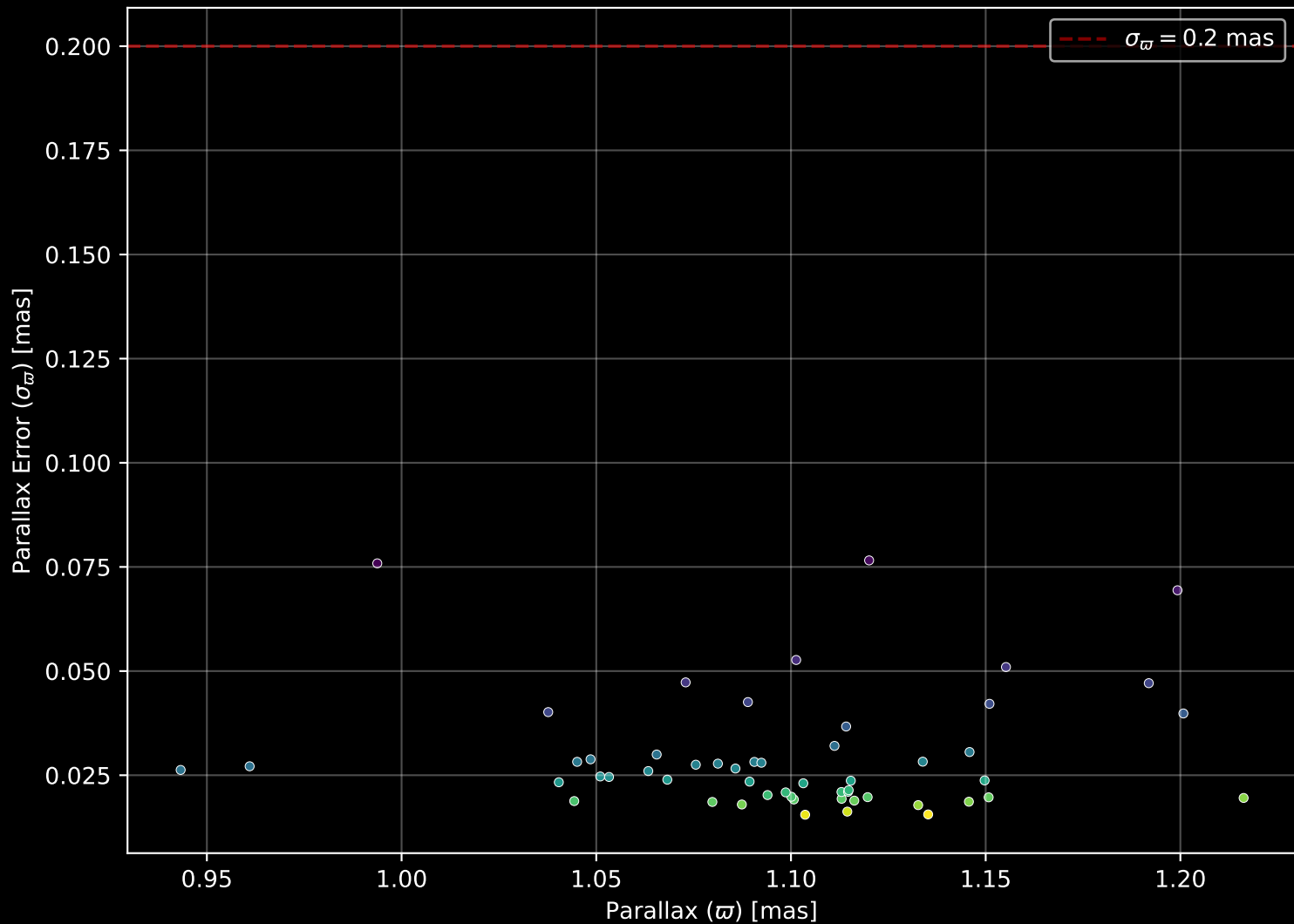
Gaia Cluster: [UBC_55] Parallax Quality (n= 54)
