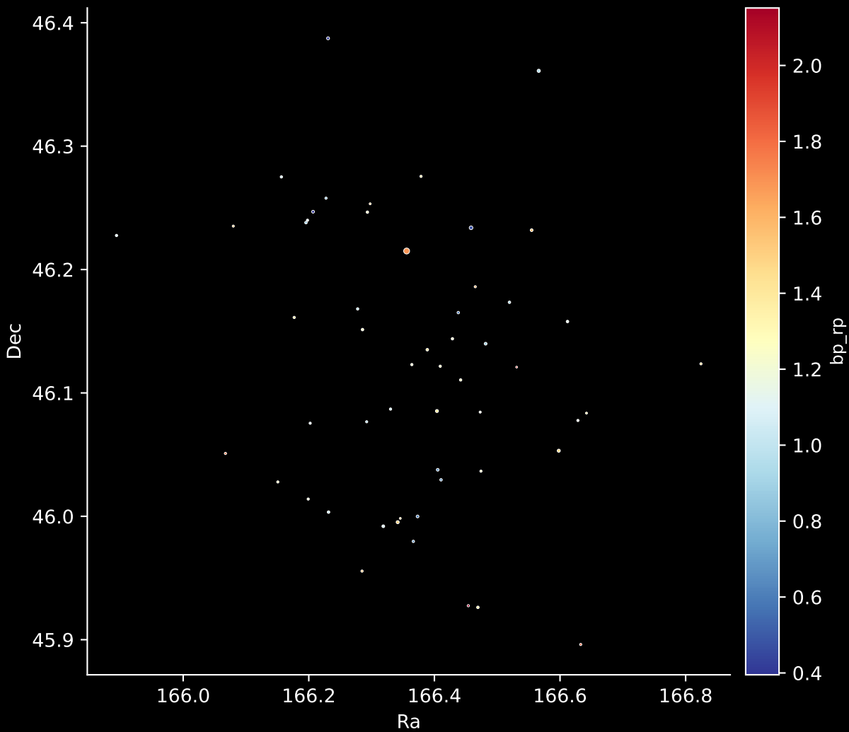
Gaia Cluster: [UBC_55] Stars: 54
