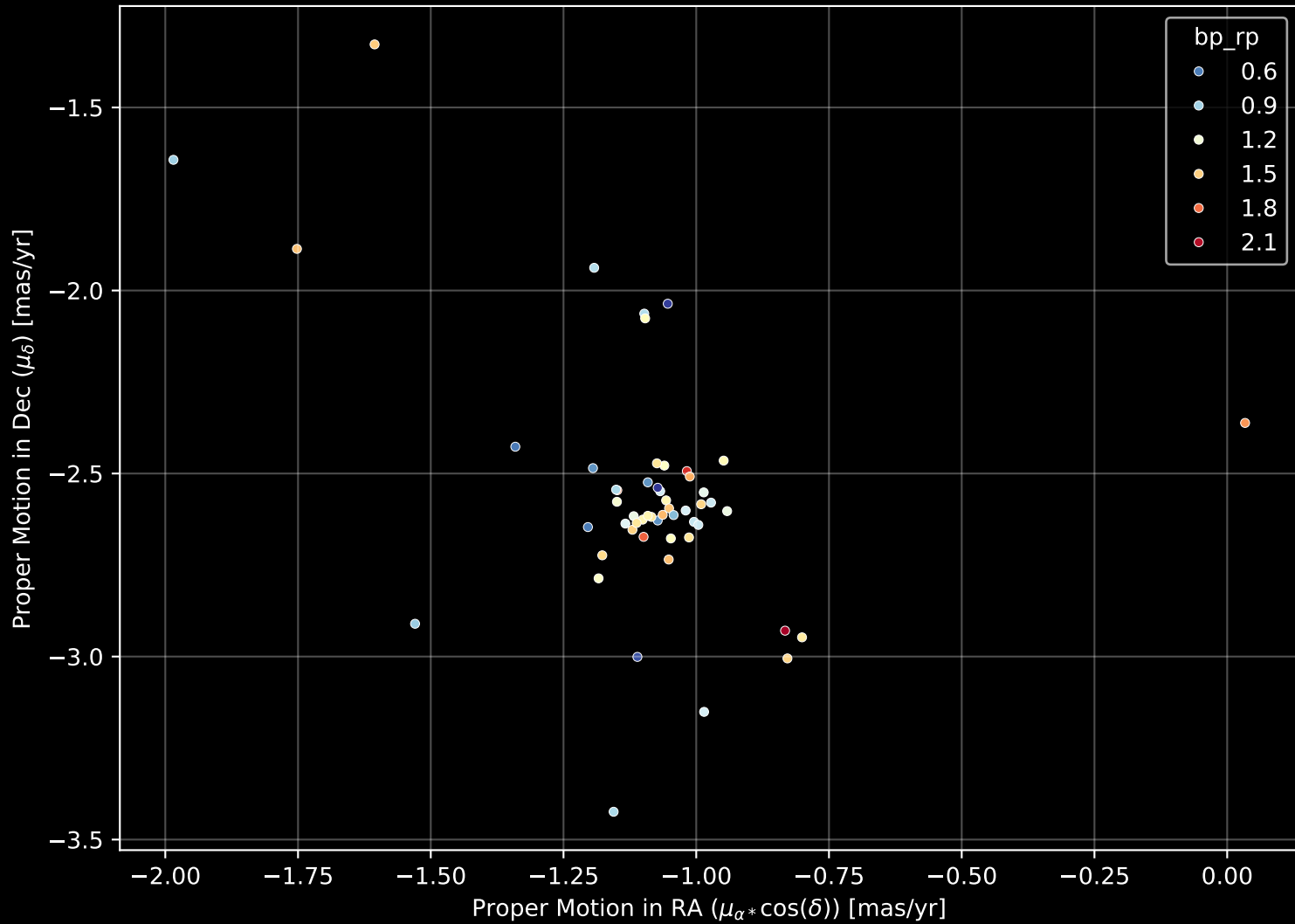
Gaia Cluster: [UBC_55] Proper Motion Diagram (n= 54)
