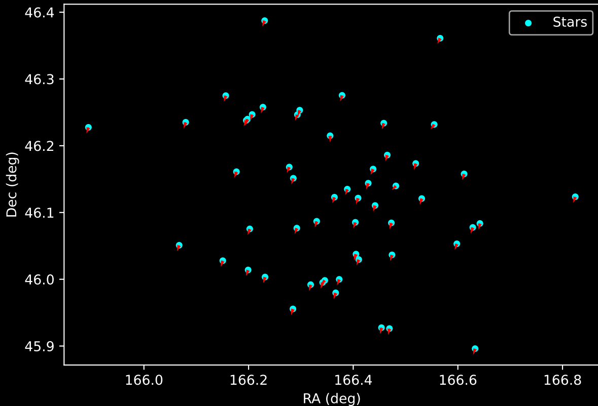
Gaia Cluster: [UBC_55] Proper Motion Vectors for Gaia Star Field (n= 54)
