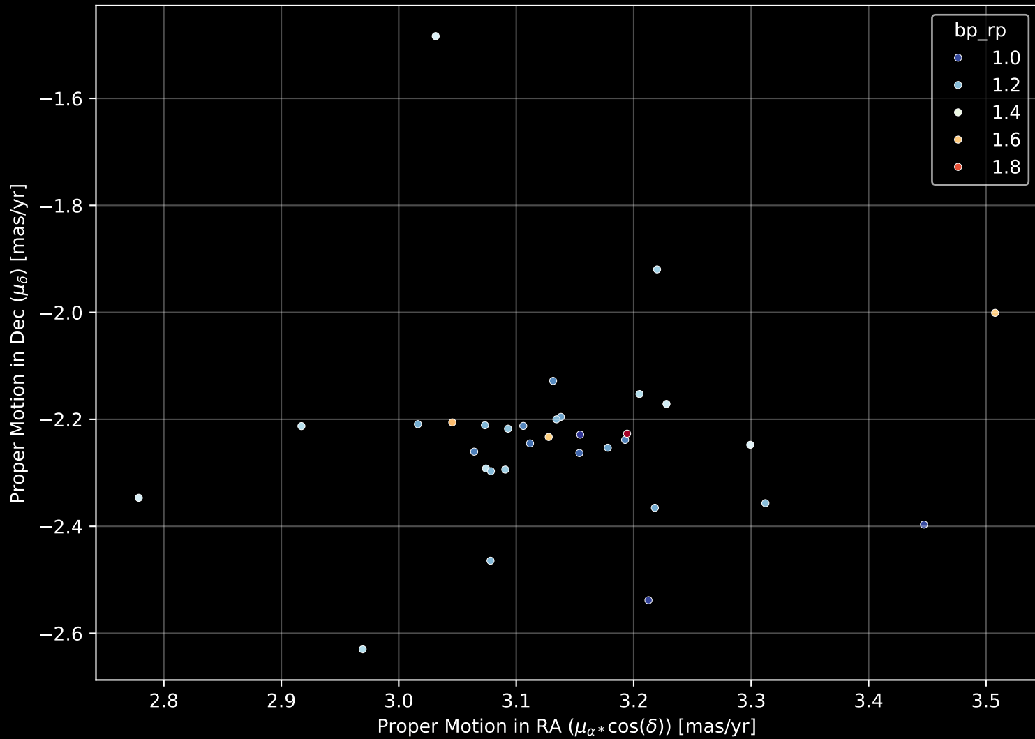
Gaia Cluster: [UBC_57] Proper Motion Diagram (n= 33)
