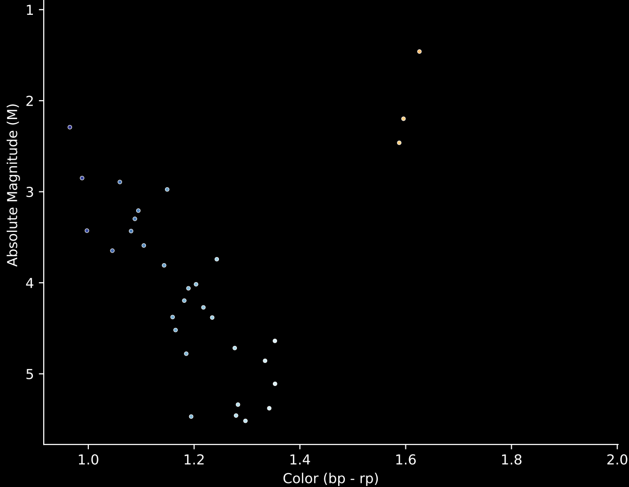
Gaia Cluster: [UBC_57] Stars (n= 33) Hertzsprung-Russel Diagram
