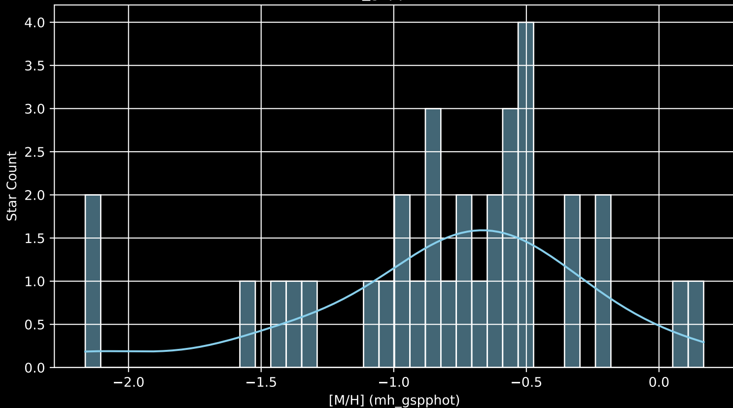
Gaia Cluster: [UBC_57 [M/H] (mh_gspphot) (n= 33)
