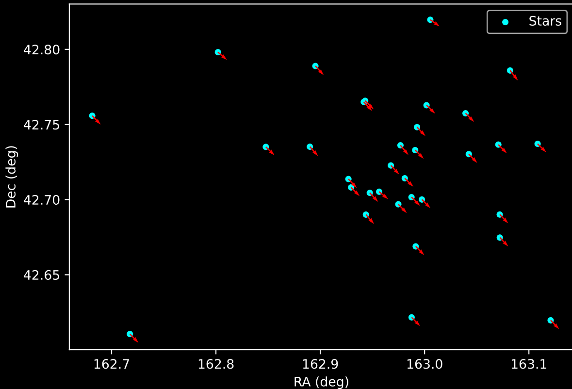
Gaia Cluster: [UBC_57] Proper Motion Vectors for Gaia Star Field (n= 33)
