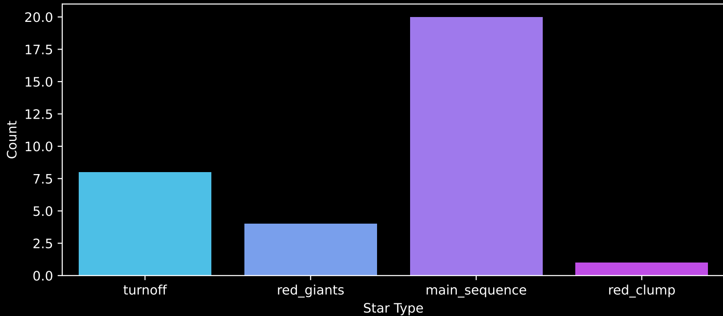
Gaia Cluster: [UBC_57] Count plot of Star Type
