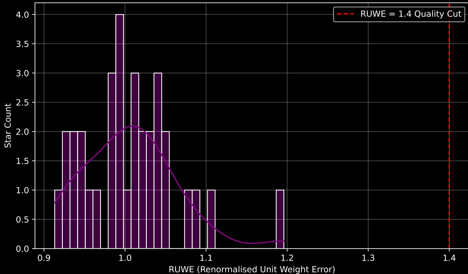
Gaia Cluster: [UBC_57] RUWE Distribution (n= 33)
