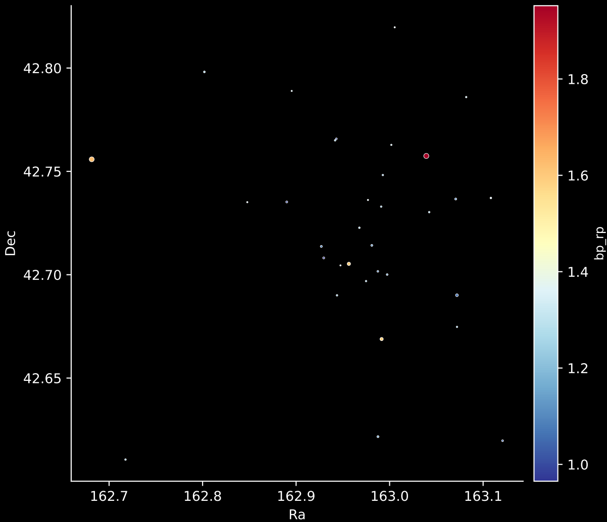
Gaia Cluster: [UBC_57] Stars: 33
