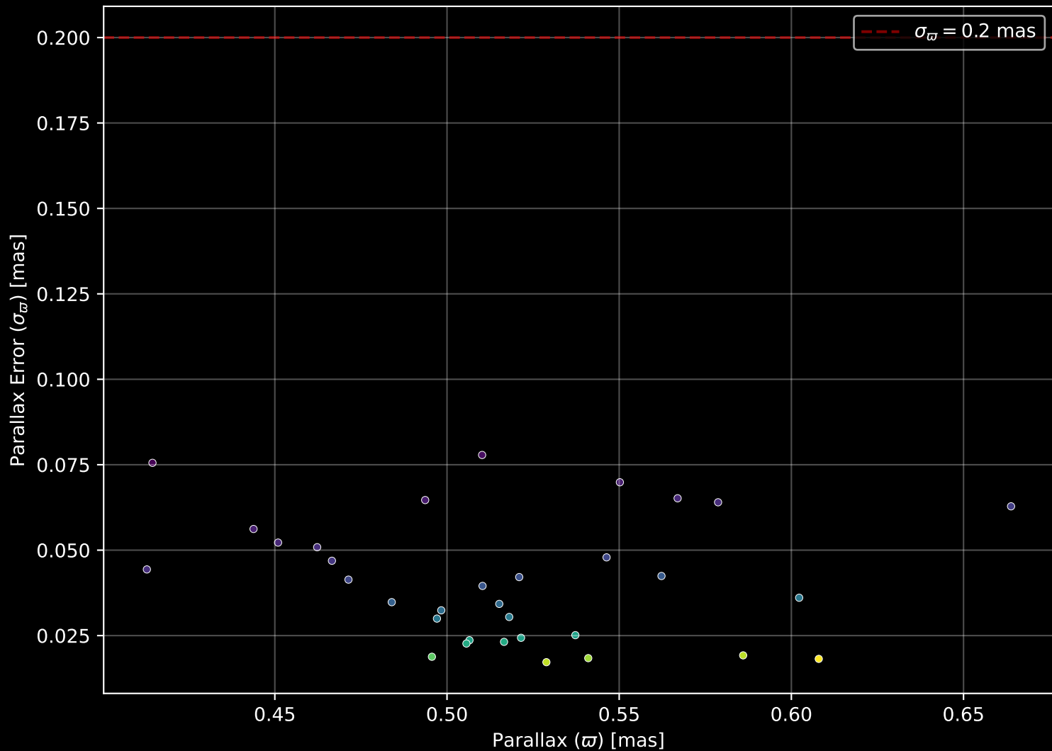
Gaia Cluster: [UBC_57] Parallax Quality (n= 33)
