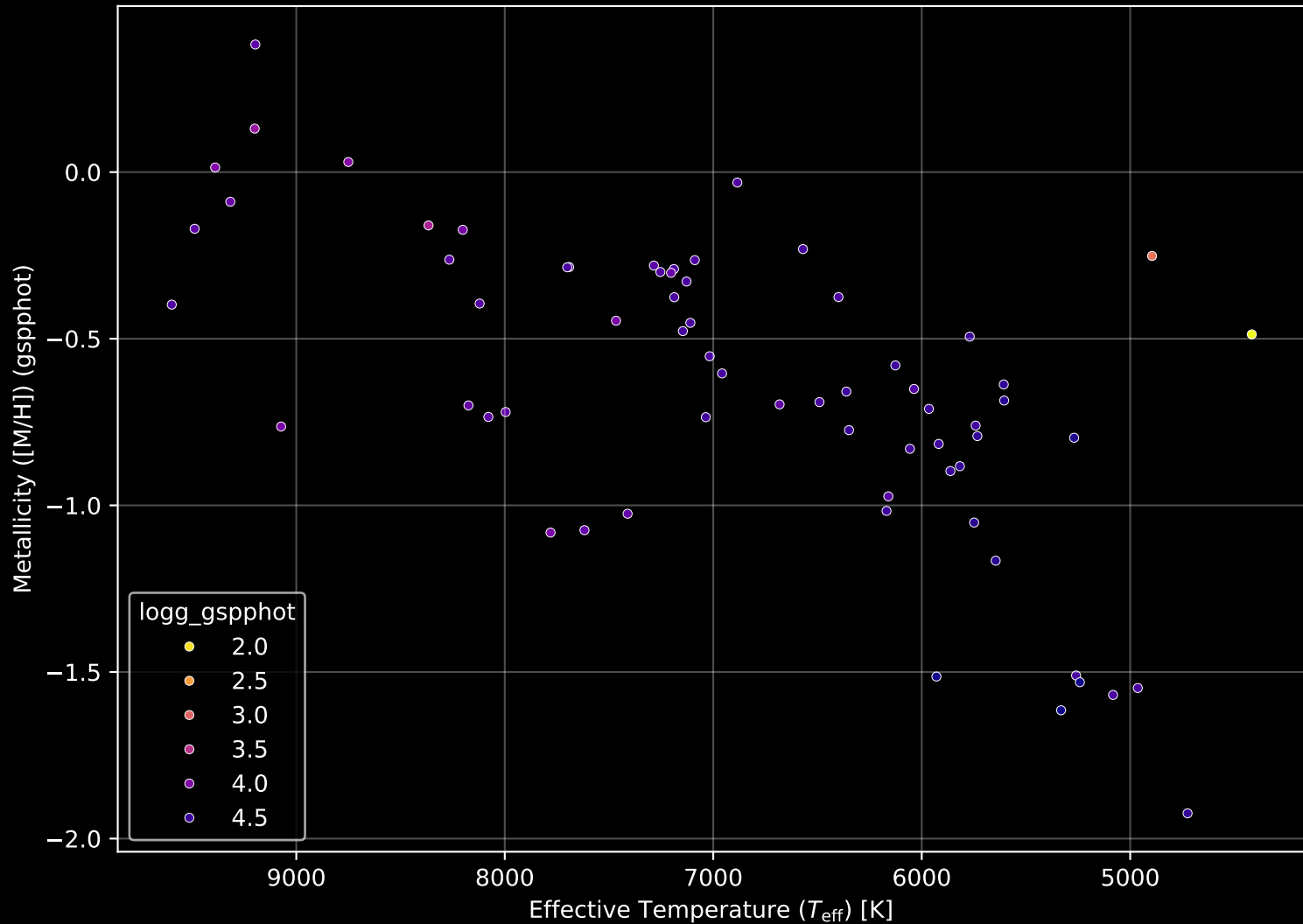
Gaia Cluster: [UBC_59] Stellar Population Parameters (n= 66)
