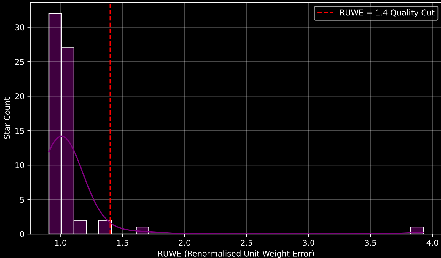
Gaia Cluster: [UBC_59] RUWE Distribution (n= 65)
