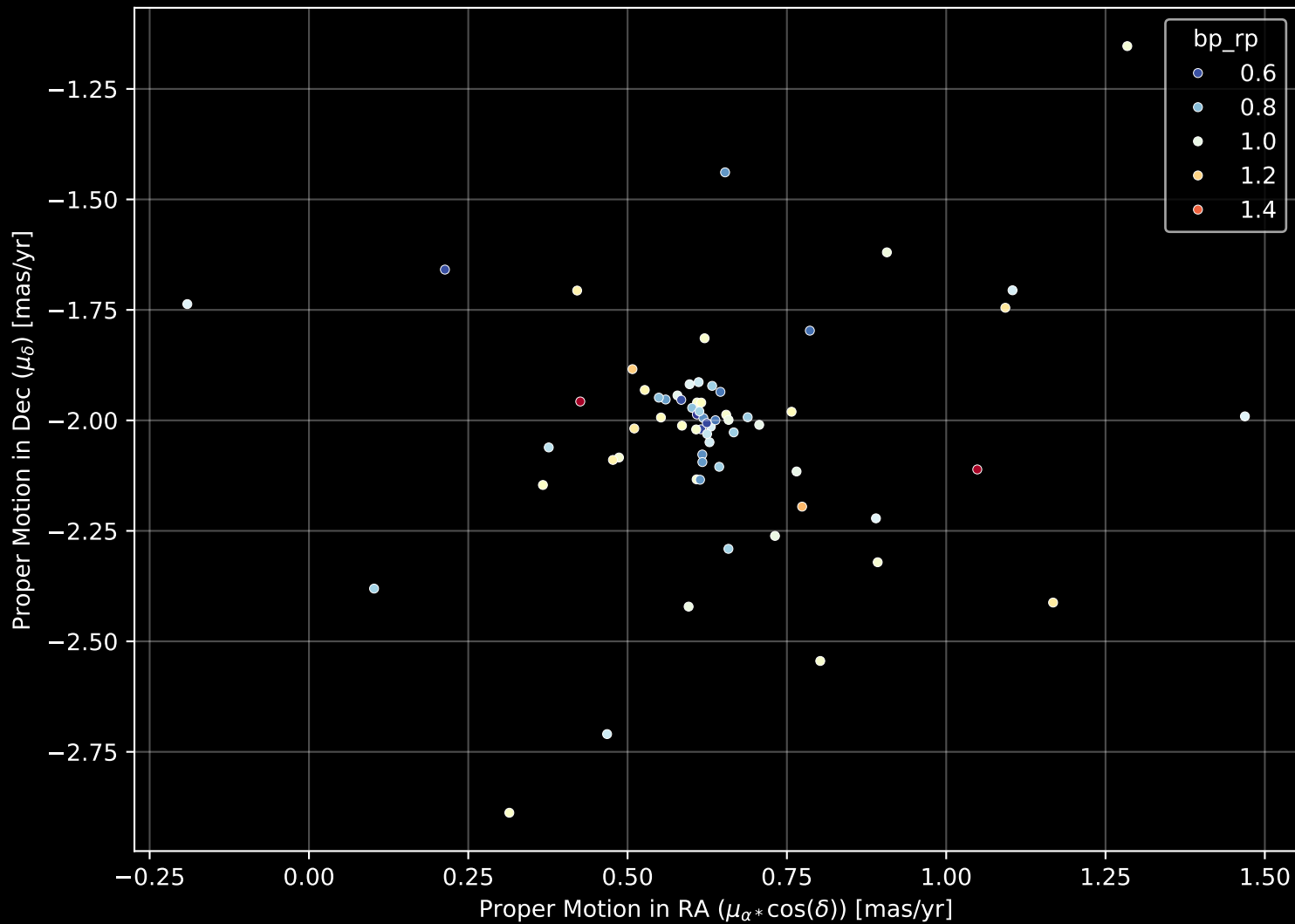
Gaia Cluster: [UBC_59] Proper Motion Diagram (n= 66)
