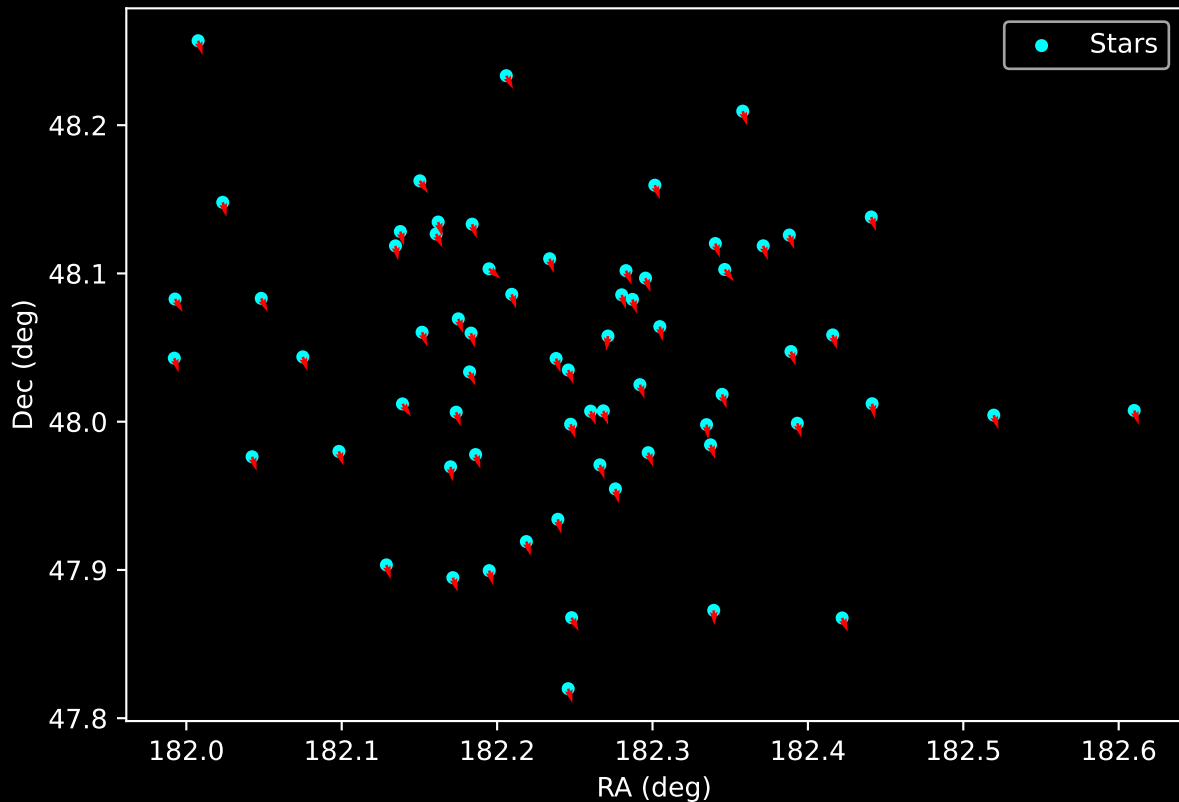
Gaia Cluster: [UBC_59] Proper Motion Vectors for Gaia Star Field (n= 66)
