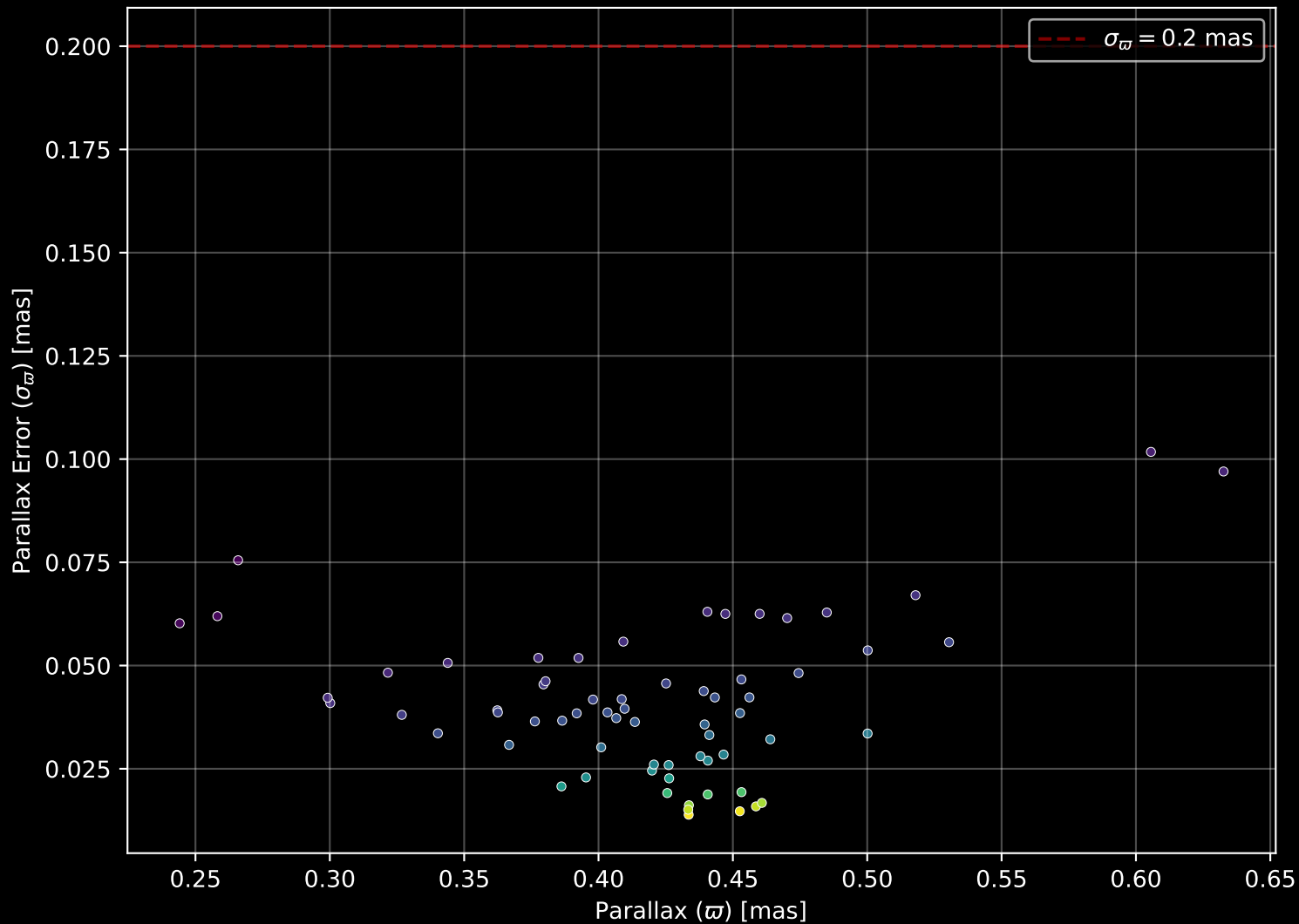
Gaia Cluster: [UBC_59] Parallax Quality (n= 66)
