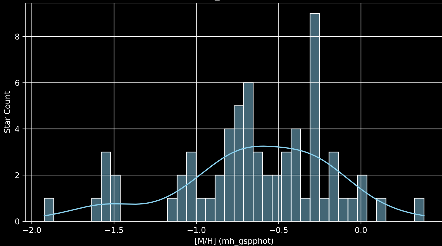
Gaia Cluster: [UBC_59 [M/H] (mh_gspphot) (n= 66)
