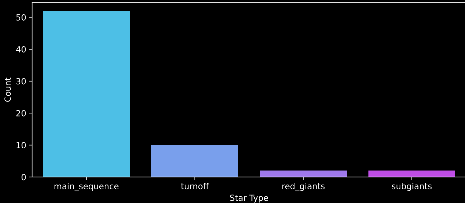
Gaia Cluster: [UBC_59] Count plot of Star Type
