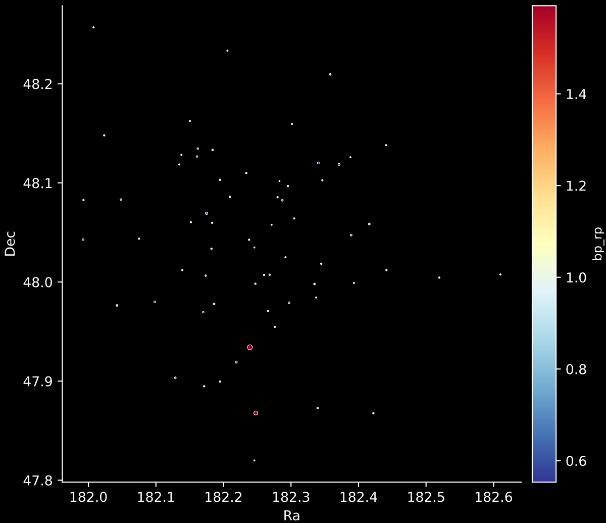
Gaia Cluster: [UBC_59] Stars: 66
