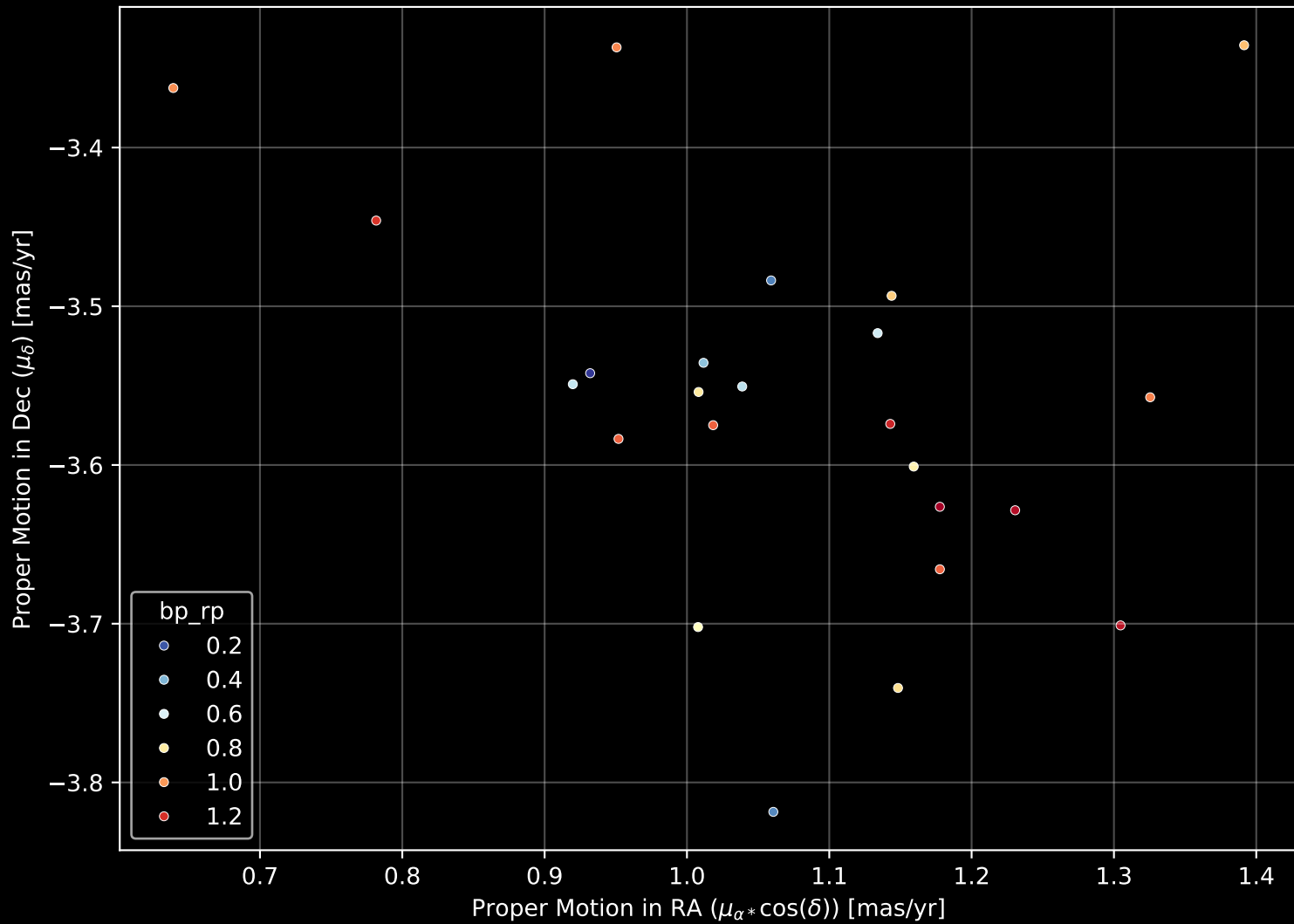
Gaia Cluster: [UBC_63] Proper Motion Diagram (n= 24)
