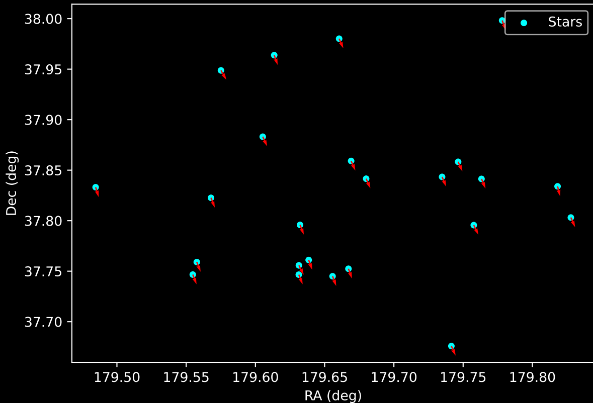
Gaia Cluster: [UBC_63] Proper Motion Vectors for Gaia Star Field (n= 24)
