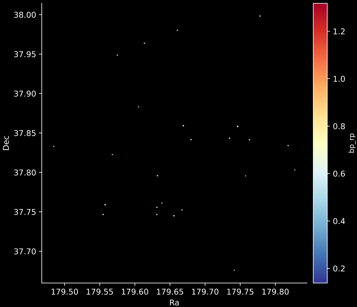
Gaia Cluster: [UBC_63] Stars: 24
