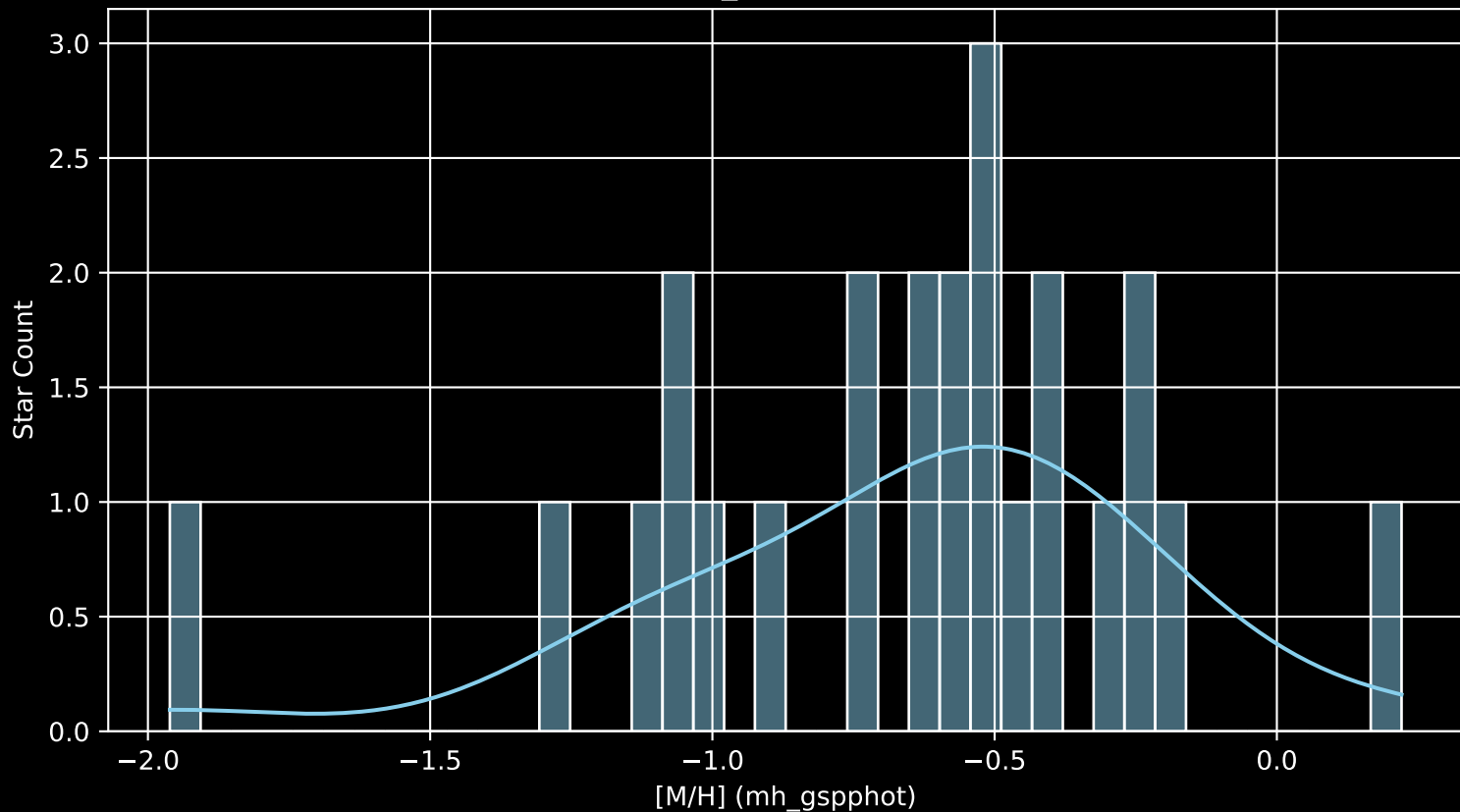
Gaia Cluster: [UBC_63 [M/H] (mh_gspphot) (n= 24)
