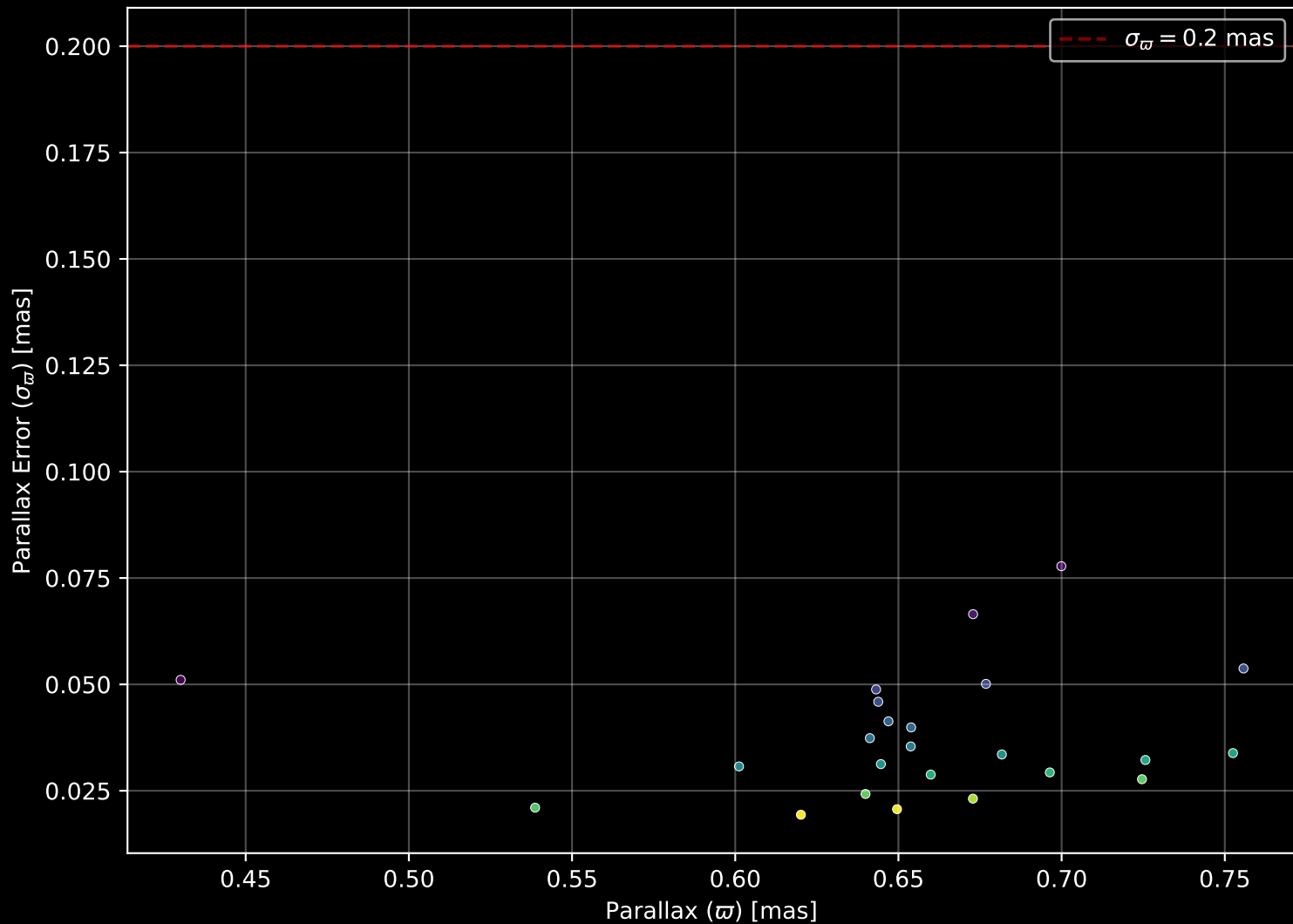
Gaia Cluster: [UBC_63] Parallax Quality (n= 24)
