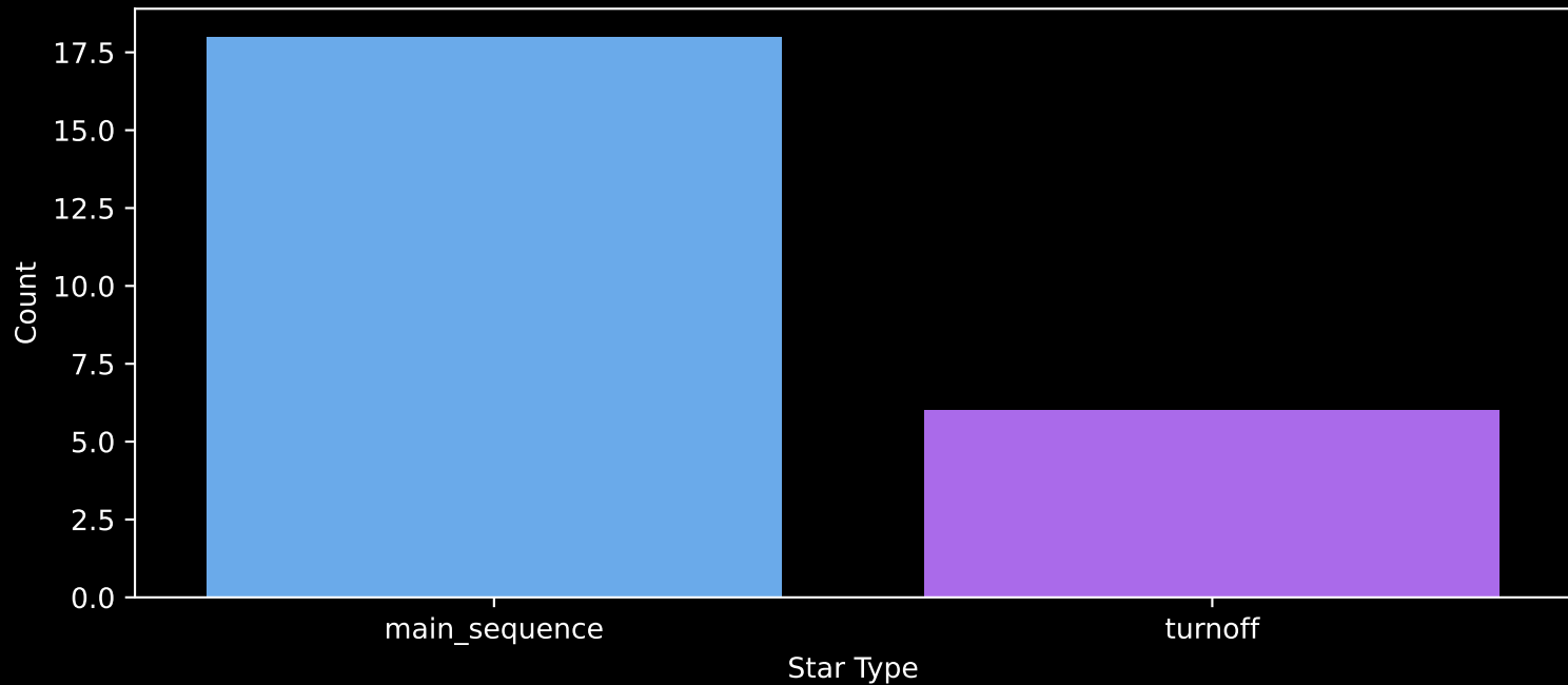
Gaia Cluster: [UBC_63] Count plot of Star Type
