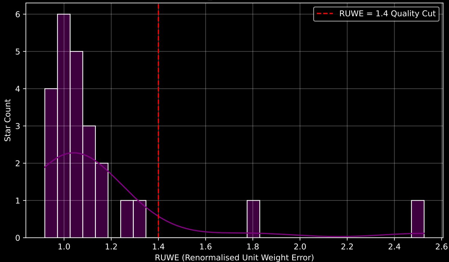
Gaia Cluster: [UBC_63] RUWE Distribution (n= 24)
