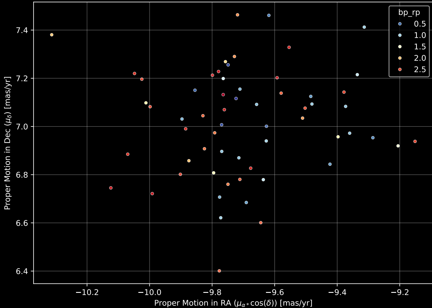
Gaia Cluster: [UBC_7] Proper Motion Diagram (n= 61)
