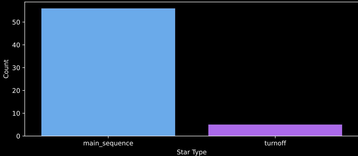
Gaia Cluster: [UBC_7] Count plot of Star Type
