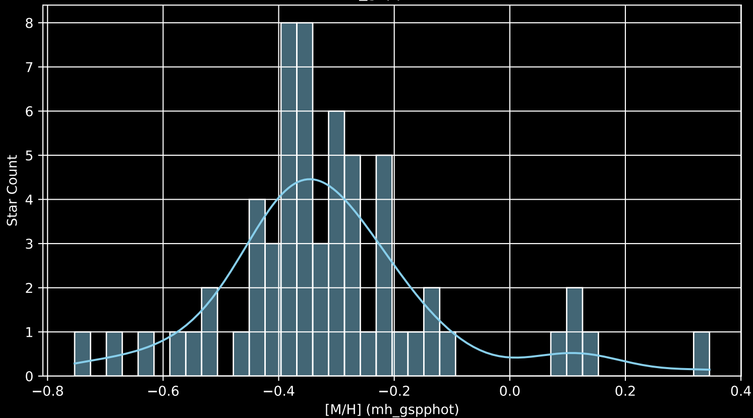
Gaia Cluster: [UBC_7 [M/H] (mh_gspphot) (n= 61)
