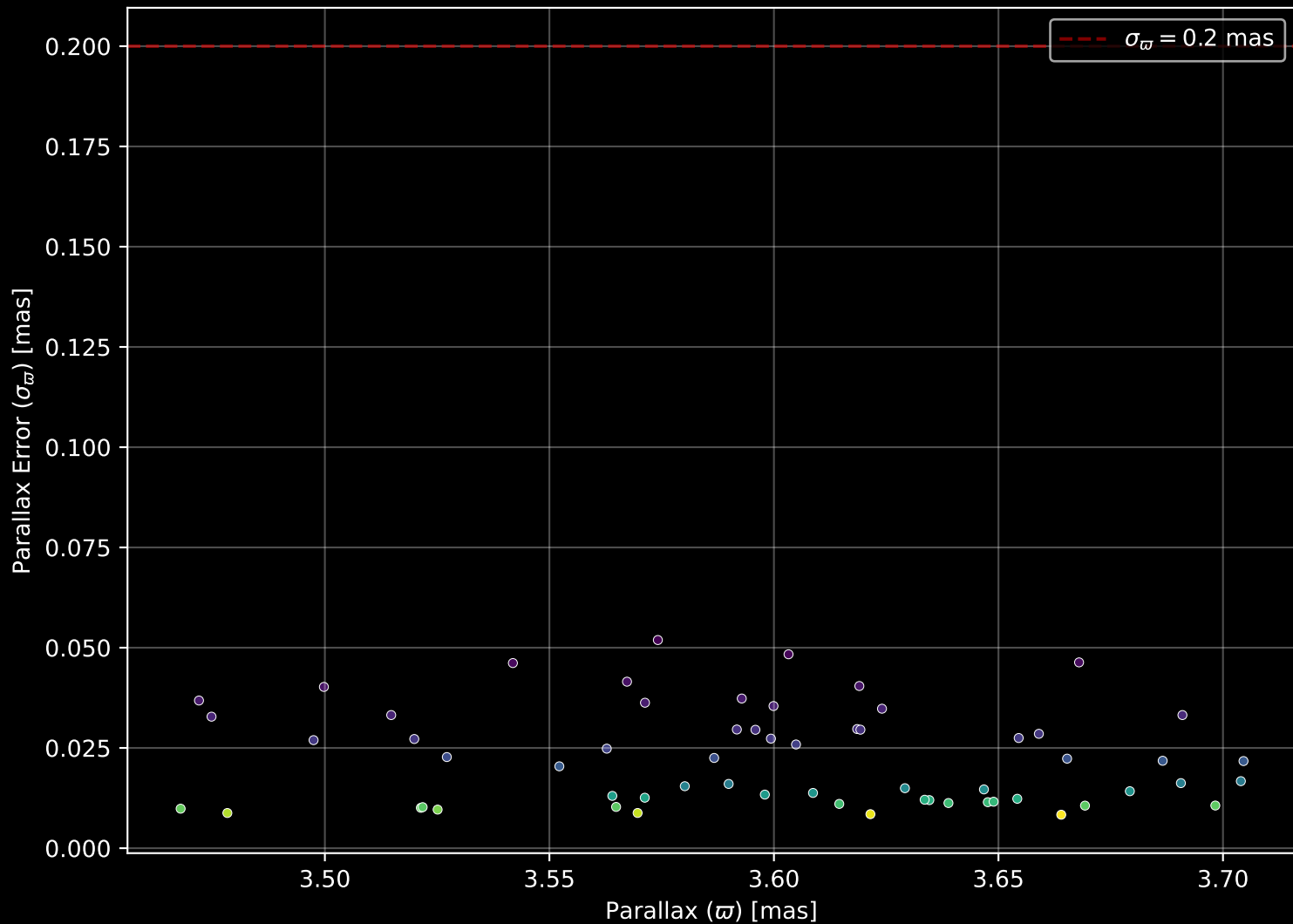
Gaia Cluster: [UBC_7] Parallax Quality (n= 61)
