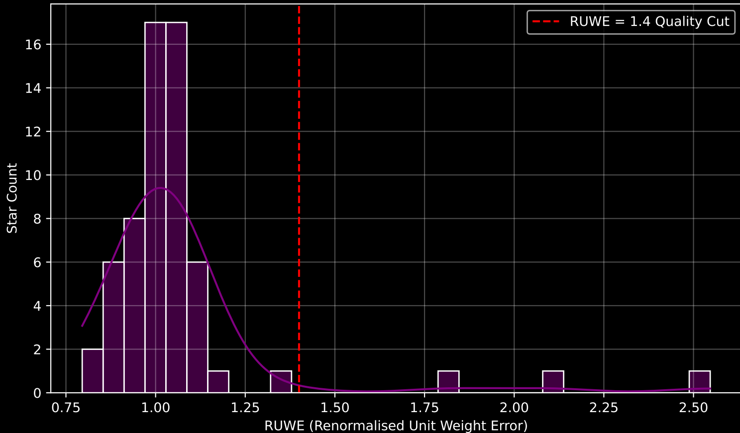
Gaia Cluster: [UBC_7] RUWE Distribution (n= 61)
