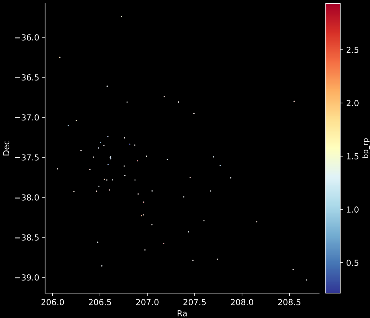
Gaia Cluster: [UBC_7] Stars: 61
