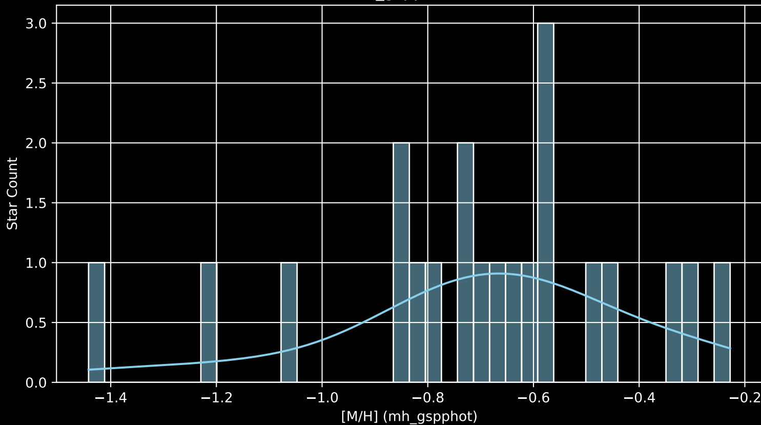
Gaia Cluster: [UBC_76 [M/H] (mh_gspphot) (n= 21)
