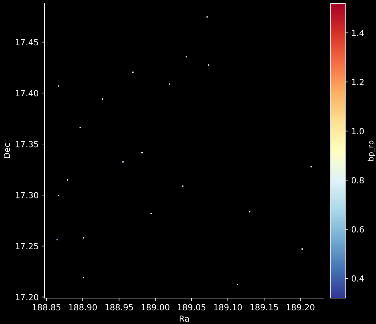
Gaia Cluster: [UBC_76] Stars: 21
