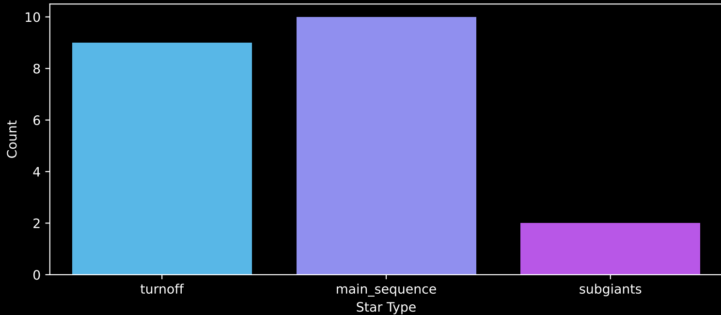
Gaia Cluster: [UBC_76] Count plot of Star Type
