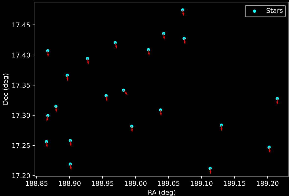
Gaia Cluster: [UBC_76] Proper Motion Vectors for Gaia Star Field (n= 21)
