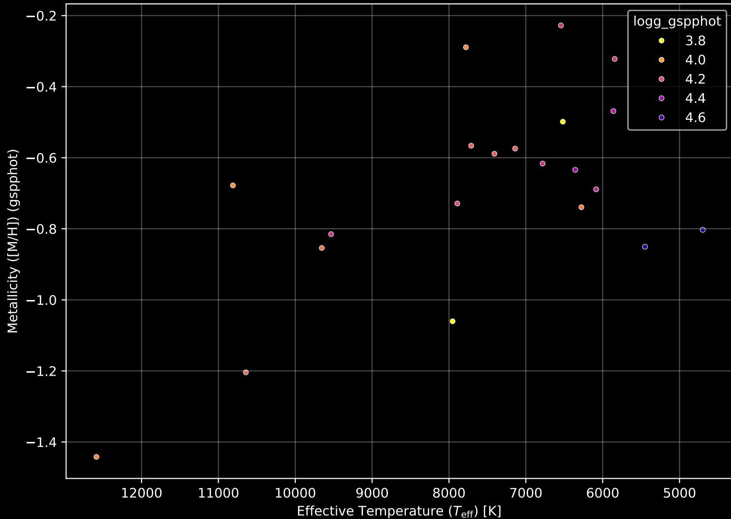
Gaia Cluster: [UBC_76] Stellar Population Parameters (n= 21)
