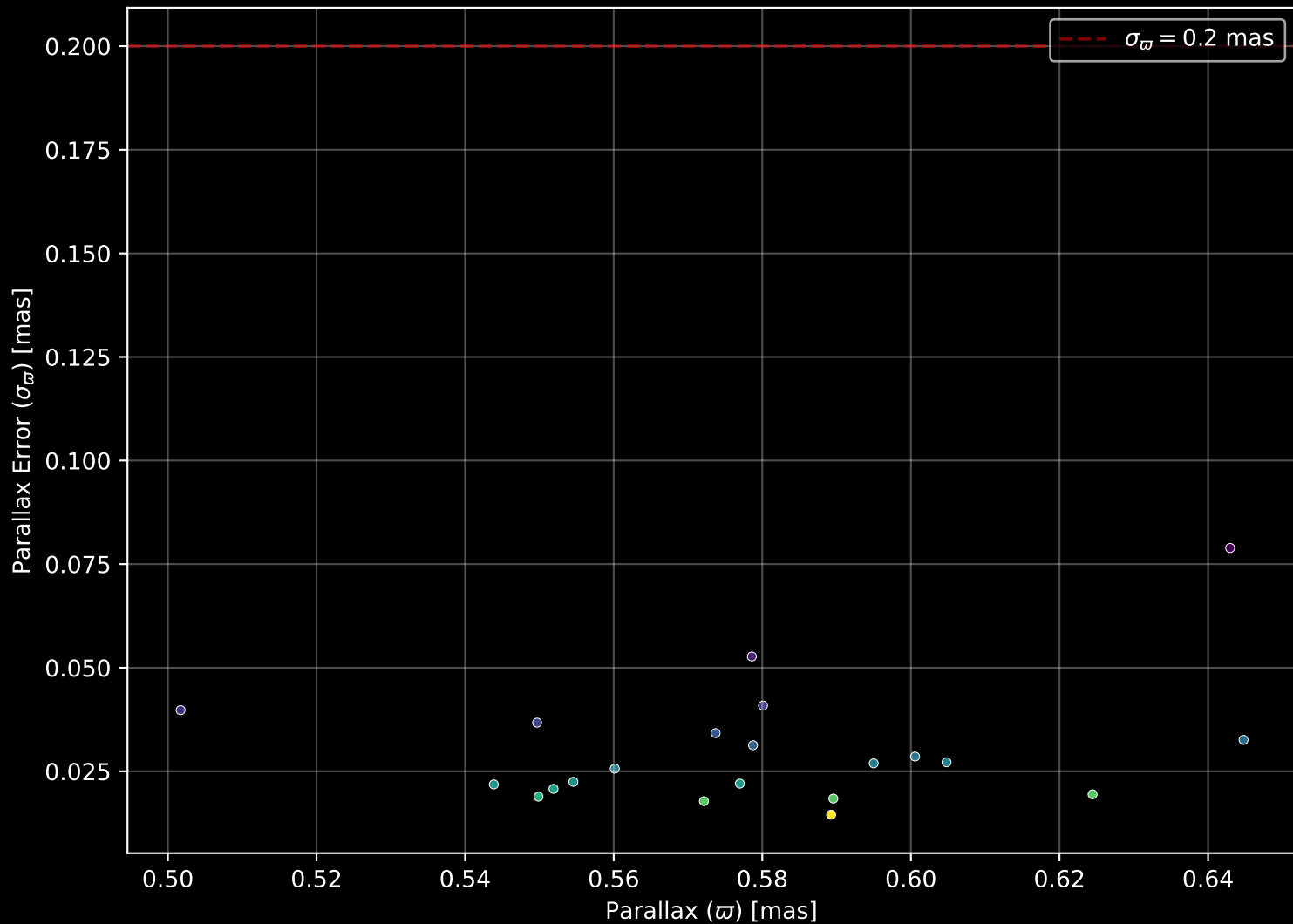
Gaia Cluster: [UBC_76] Parallax Quality (n= 21)
