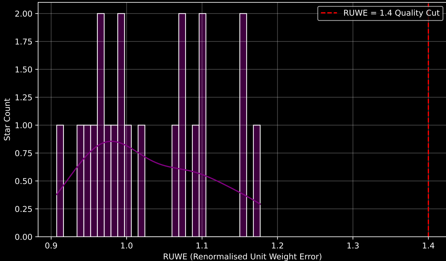
Gaia Cluster: [UBC_76] RUWE Distribution (n= 21)
