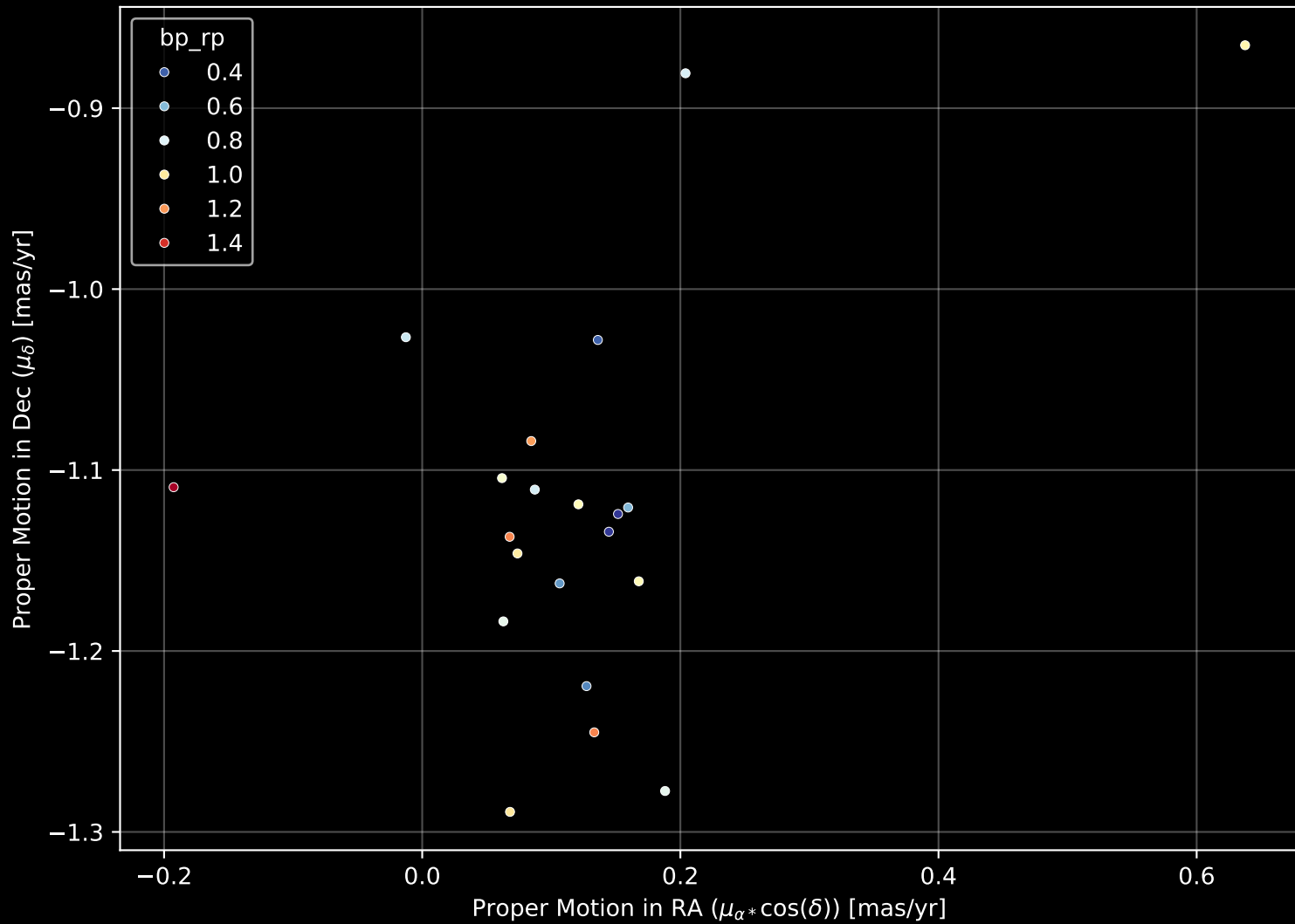
Gaia Cluster: [UBC_76] Proper Motion Diagram (n= 21)
