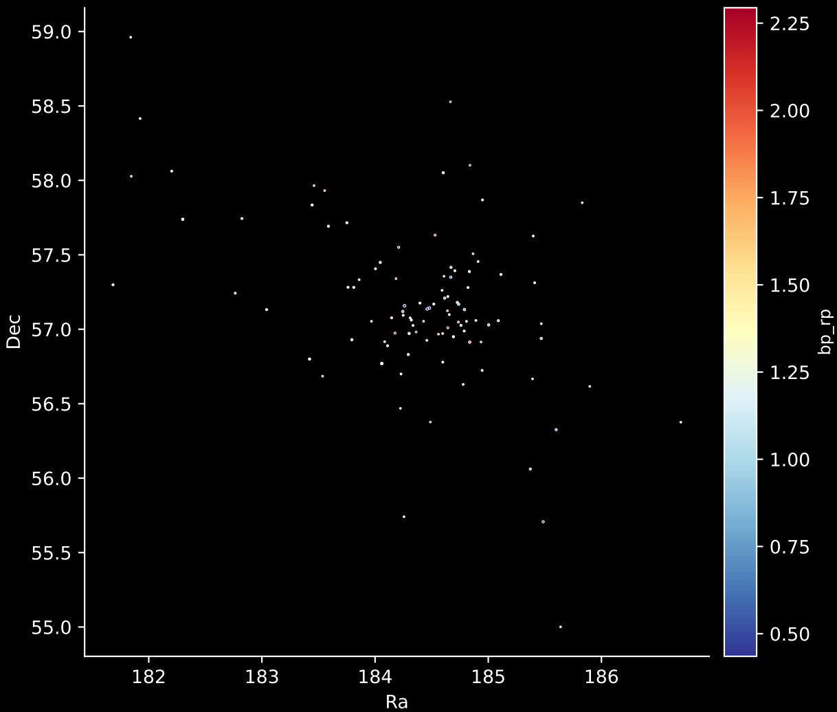
Gaia Cluster: [UBC_8] Stars: 99
