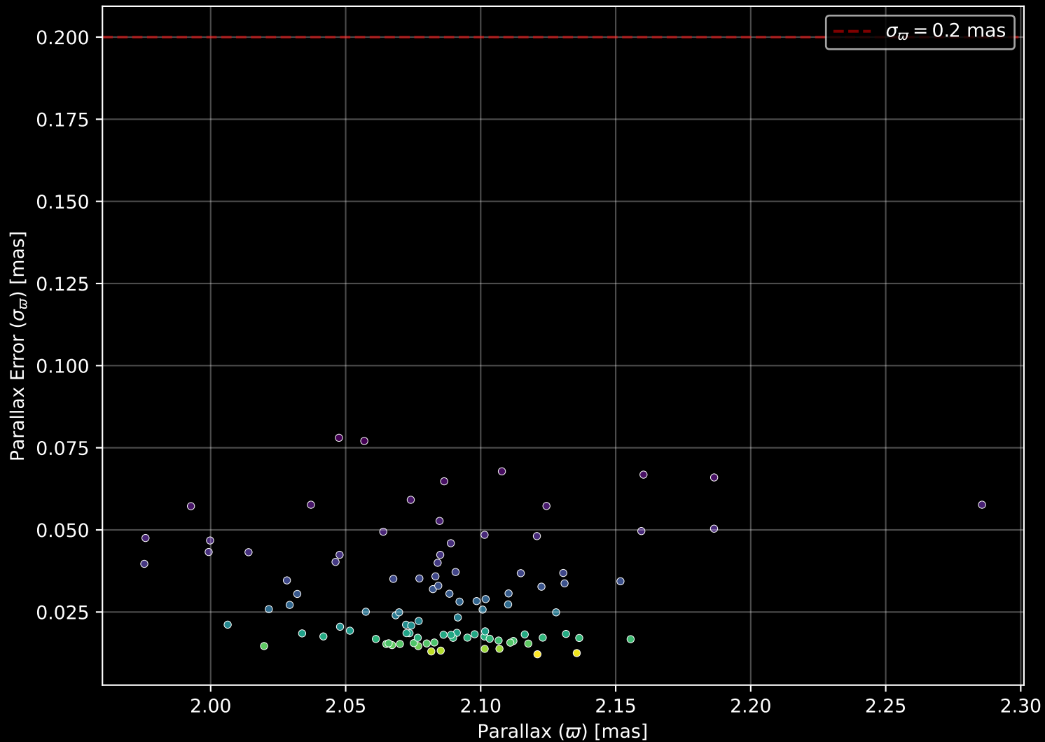
Gaia Cluster: [UBC_8] Parallax Quality (n= 99)
