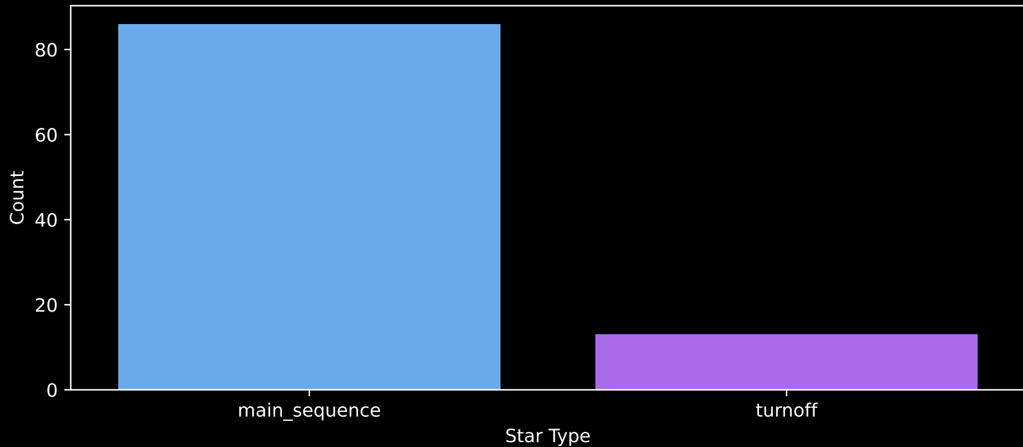
Gaia Cluster: [UBC_8] Count plot of Star Type
