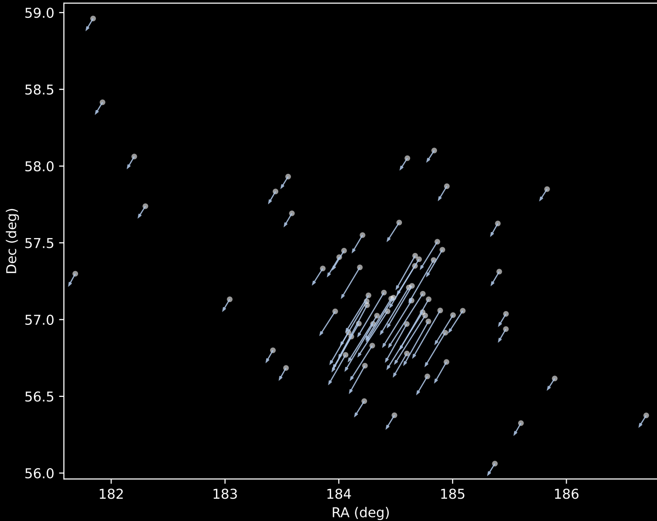
Gaia DR3 Cluster 1 Proper Motion Vectors (n=69)
