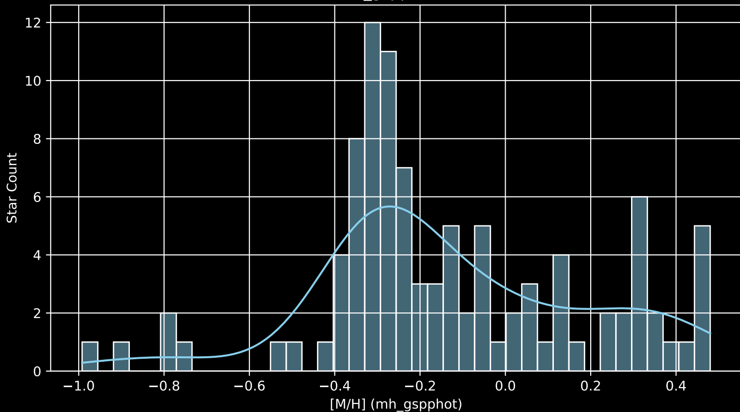
Gaia Cluster: [UBC_8 [M/H] (mh_gspphot) (n= 99)
