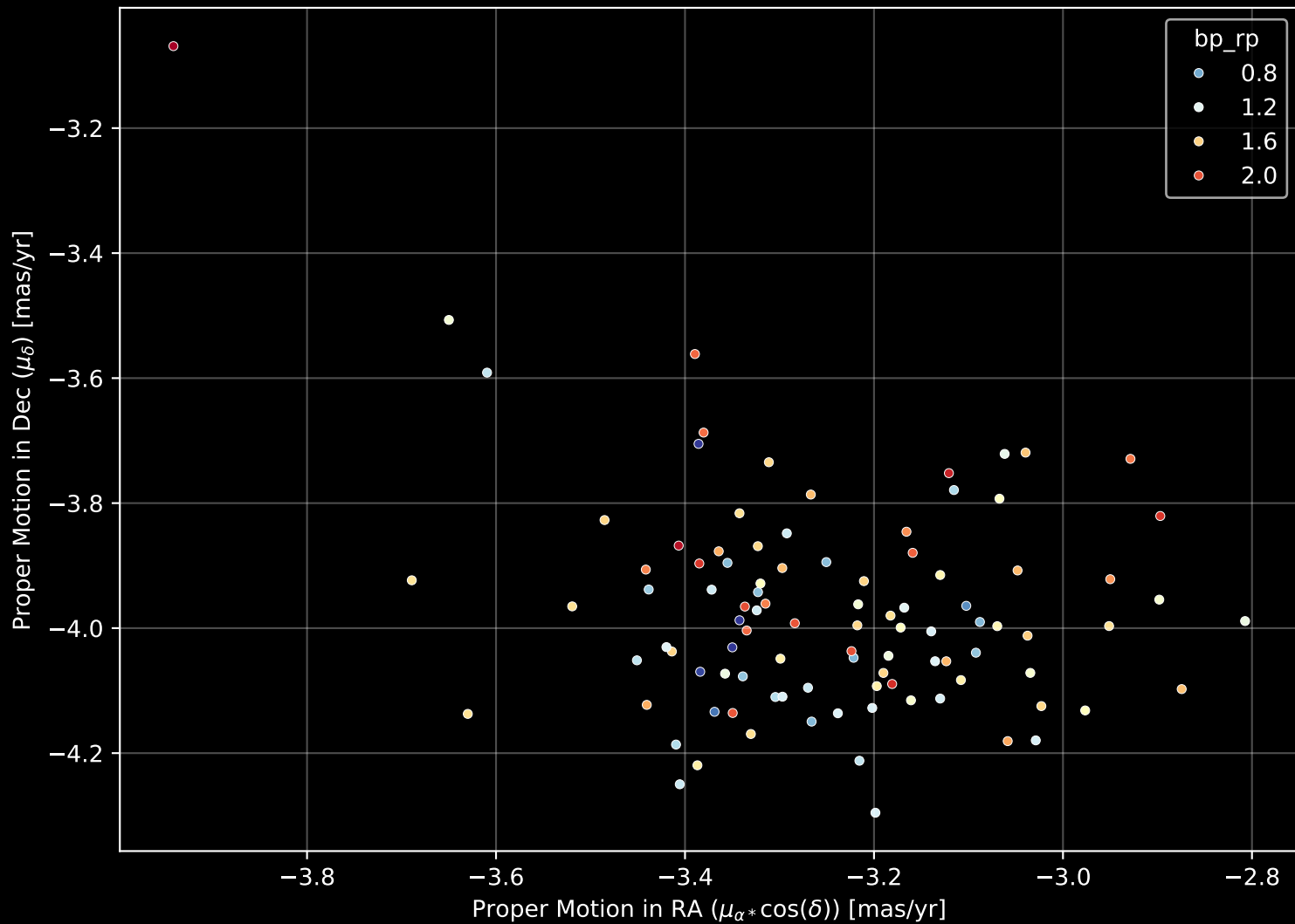
Gaia Cluster: [UBC_8] Proper Motion Diagram (n= 99)
