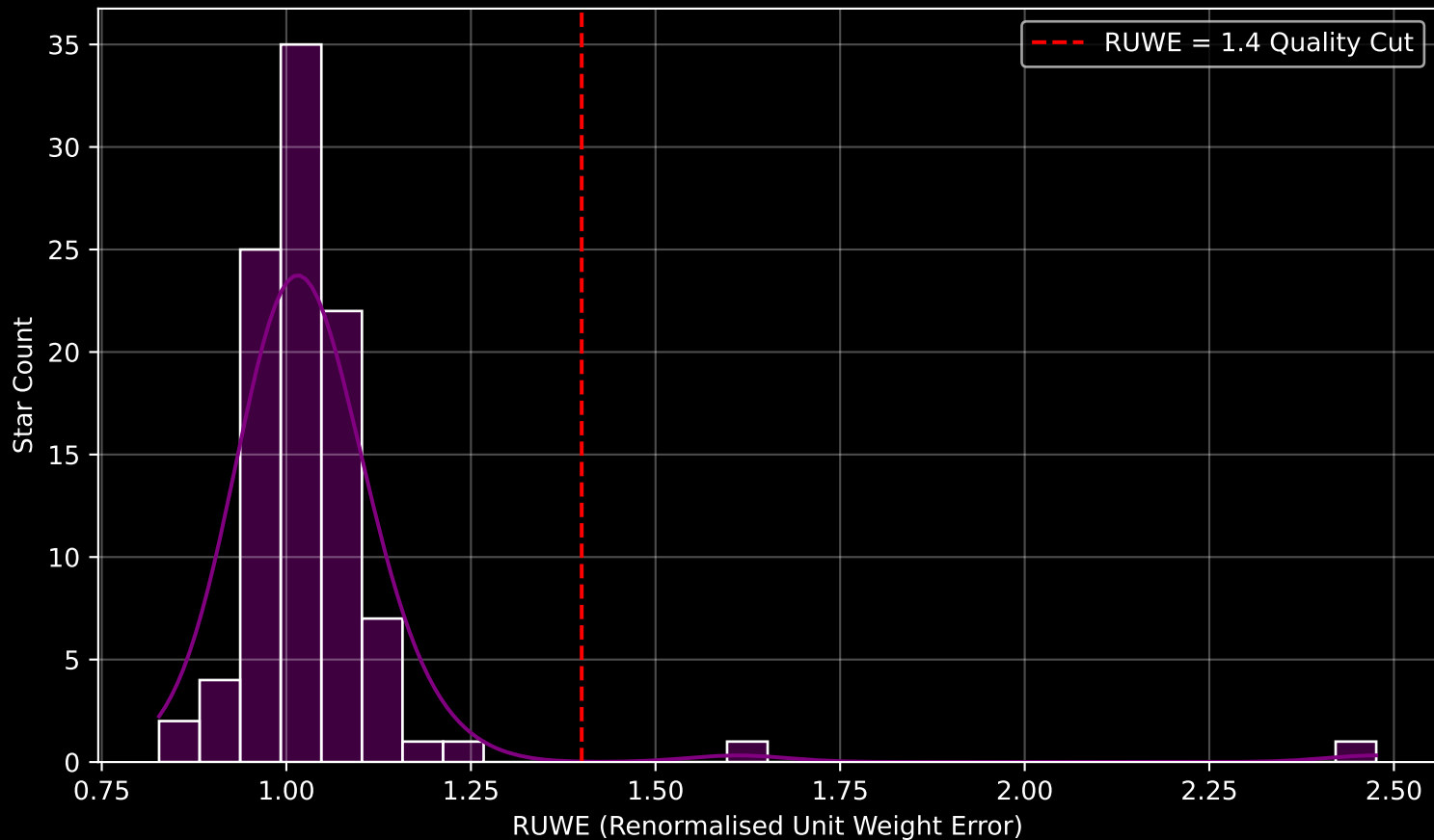
Gaia Cluster: [UBC_8] RUWE Distribution (n= 99)
