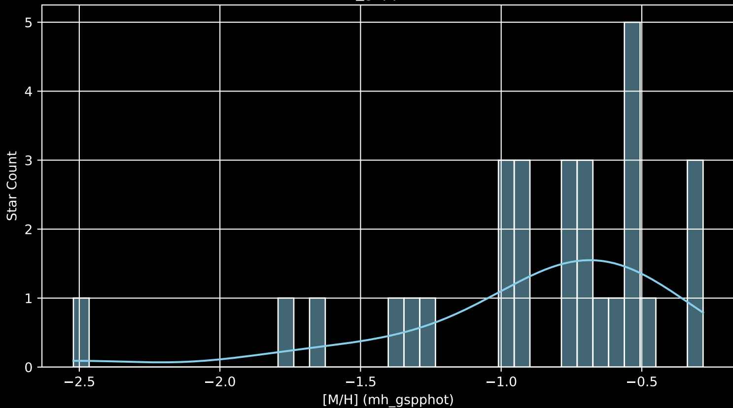
Gaia Cluster: [UBC_80 [M/H] (mh_gspphot) ( \bar{n}= 29 )
