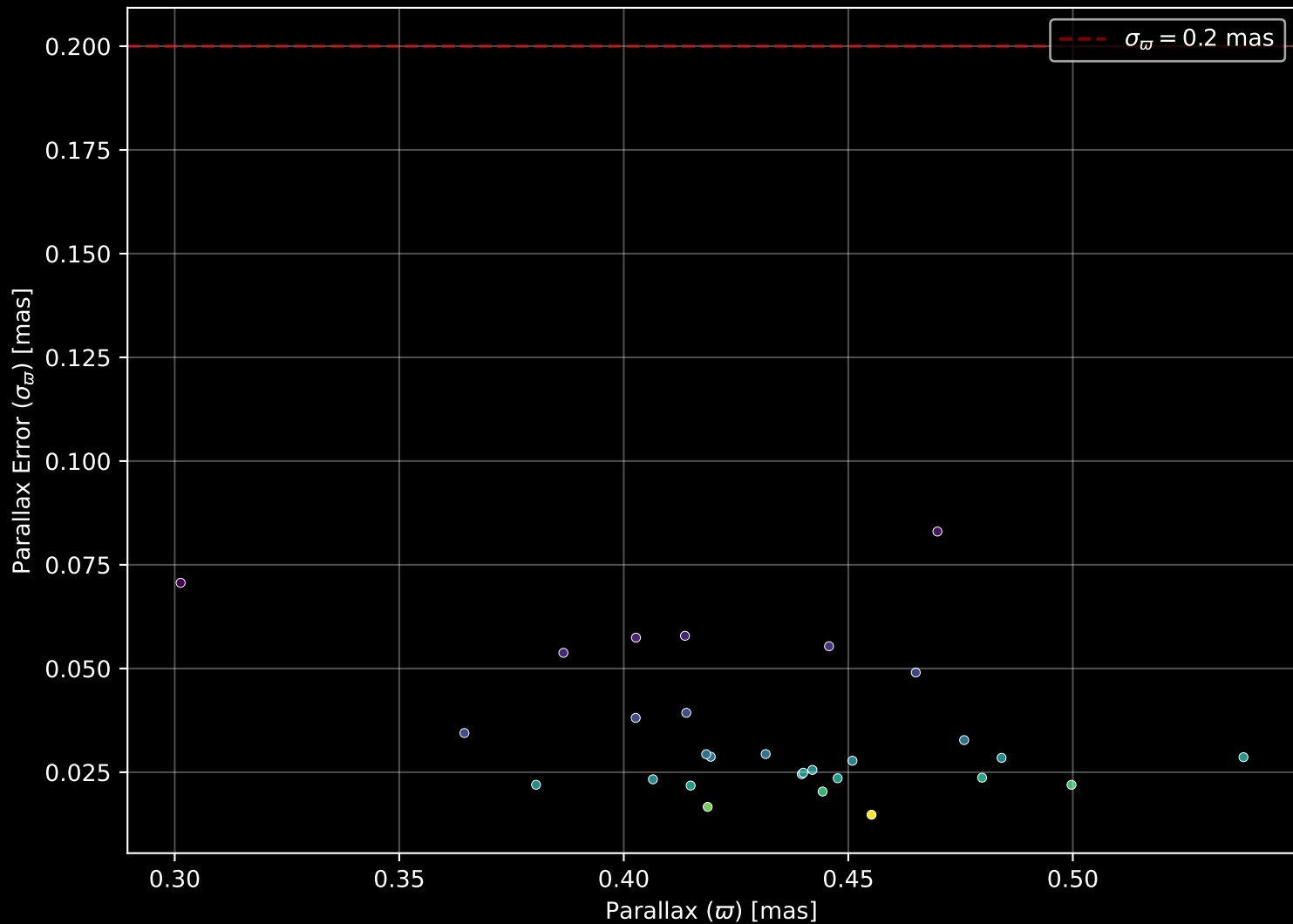
Gaia Cluster: [UBC_80] Parallax Quality (n= 29)
