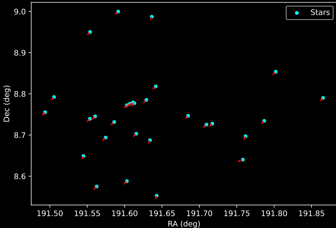
Gaia Cluster: [UBC_80] Proper Motion Vectors for Gaia Star Field (n= 29)
