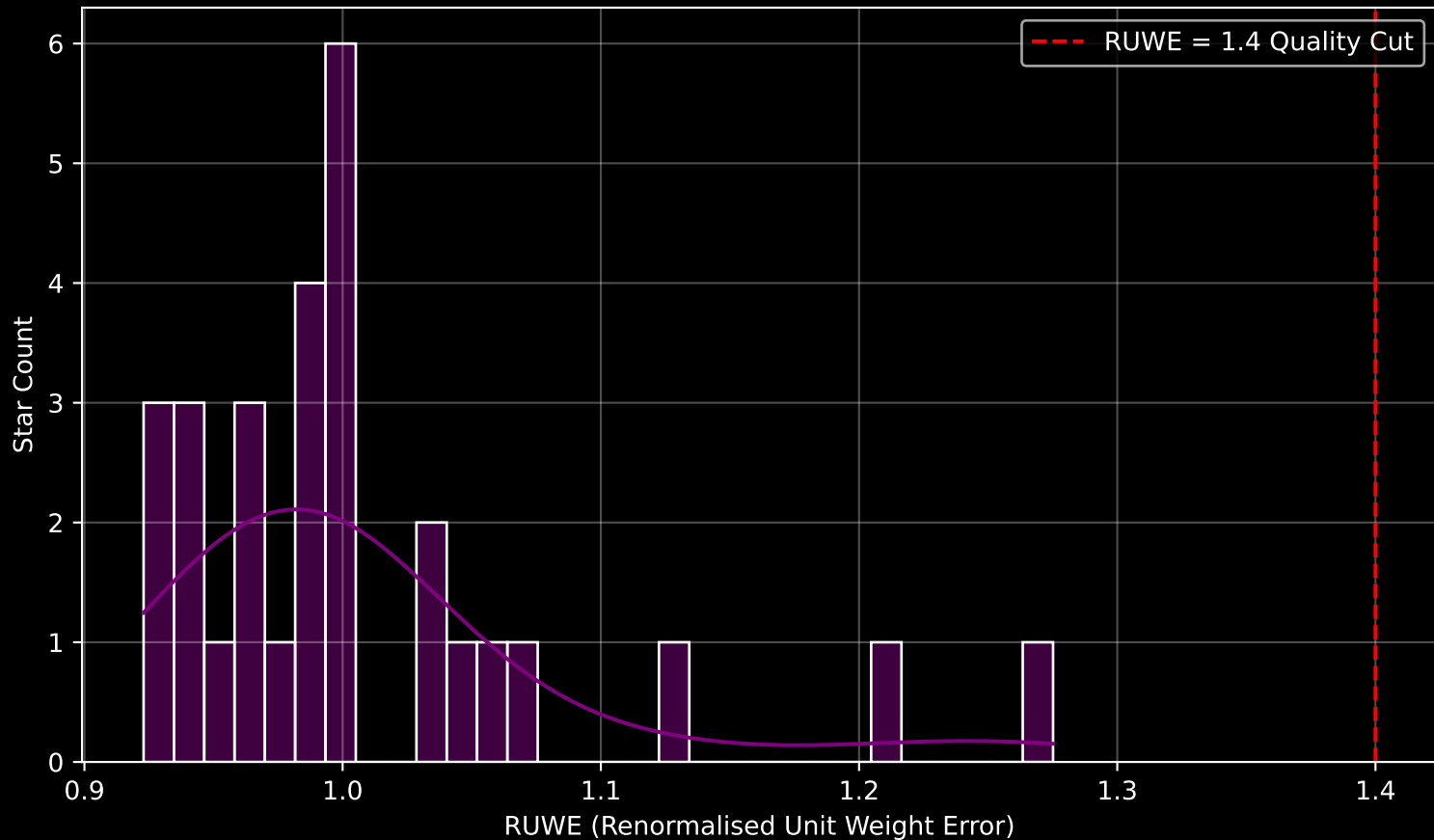
Gaia Cluster: [UBC_80] RUWE Distribution (n= 29)
