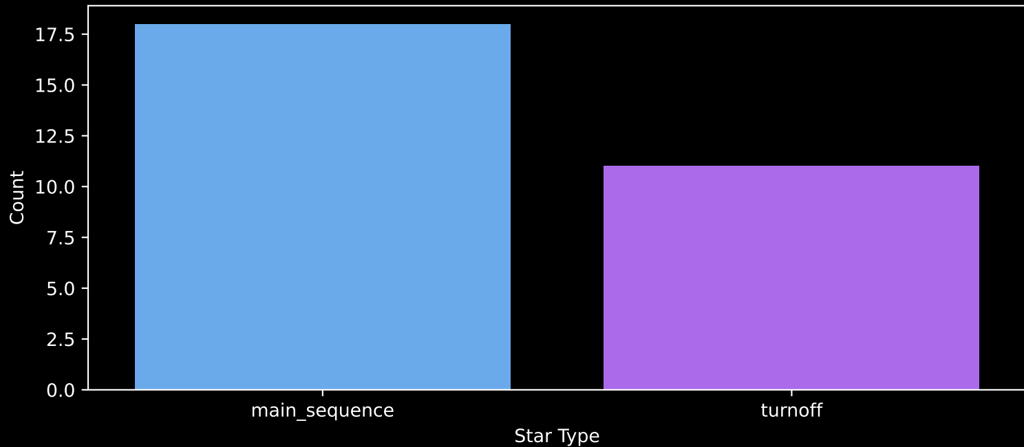
Gaia Cluster: [UBC_80] Count plot of Star Type
