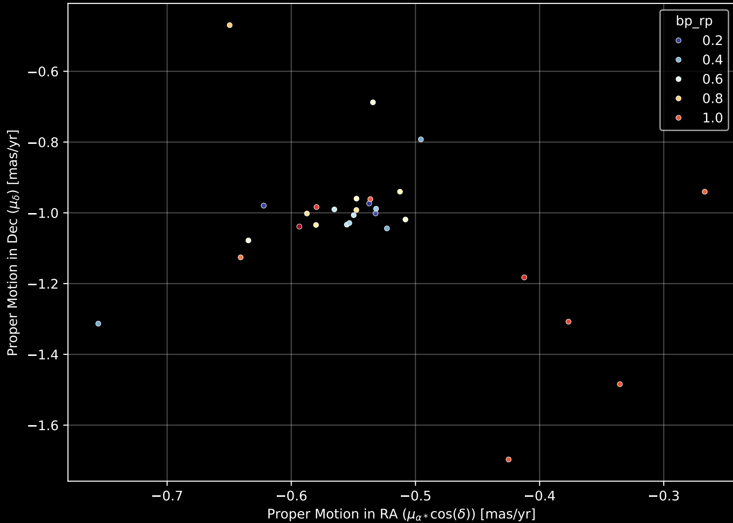
Gaia Cluster: [UBC_80] Proper Motion Diagram (n= 29)
