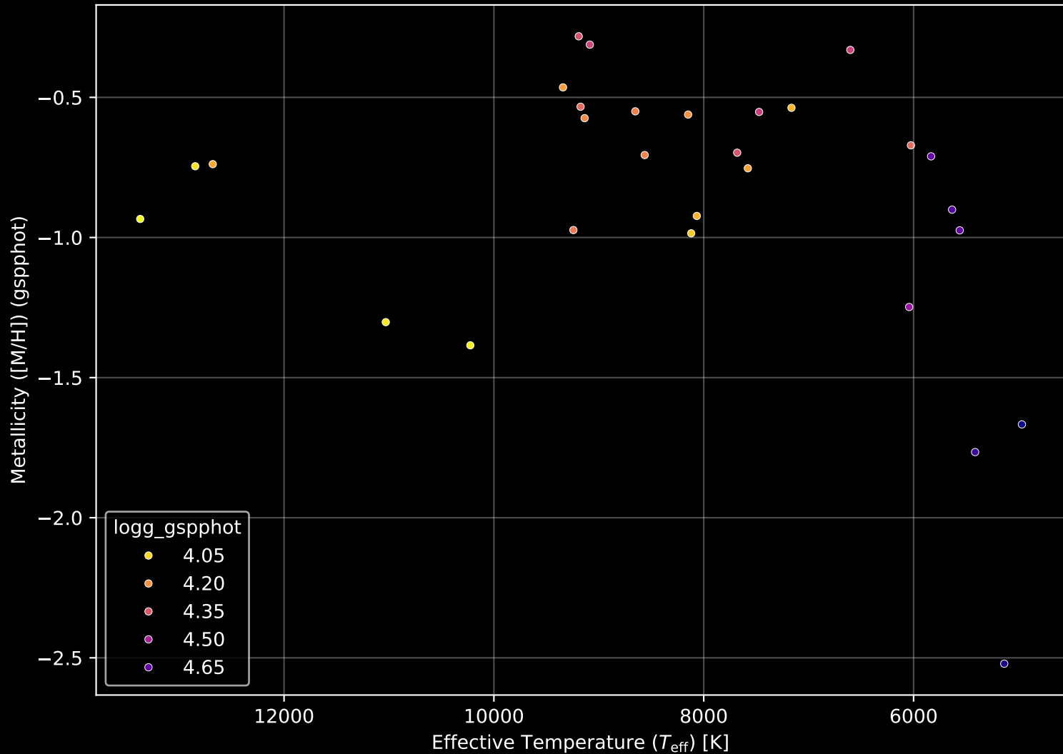
Gaia Cluster: [UBC_80] Stellar Population Parameters (n= 29)
