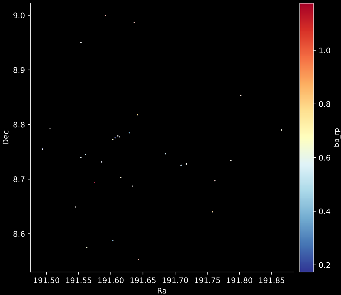
Gaia Cluster: [UBC_80] Stars: 29
