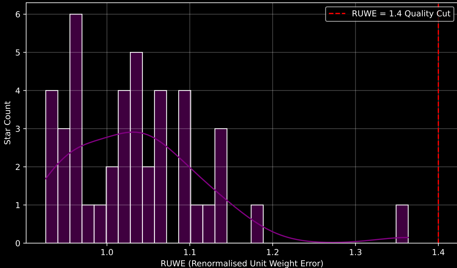
Gaia Cluster: [UBC_83] RUWE Distribution (n= 43)
