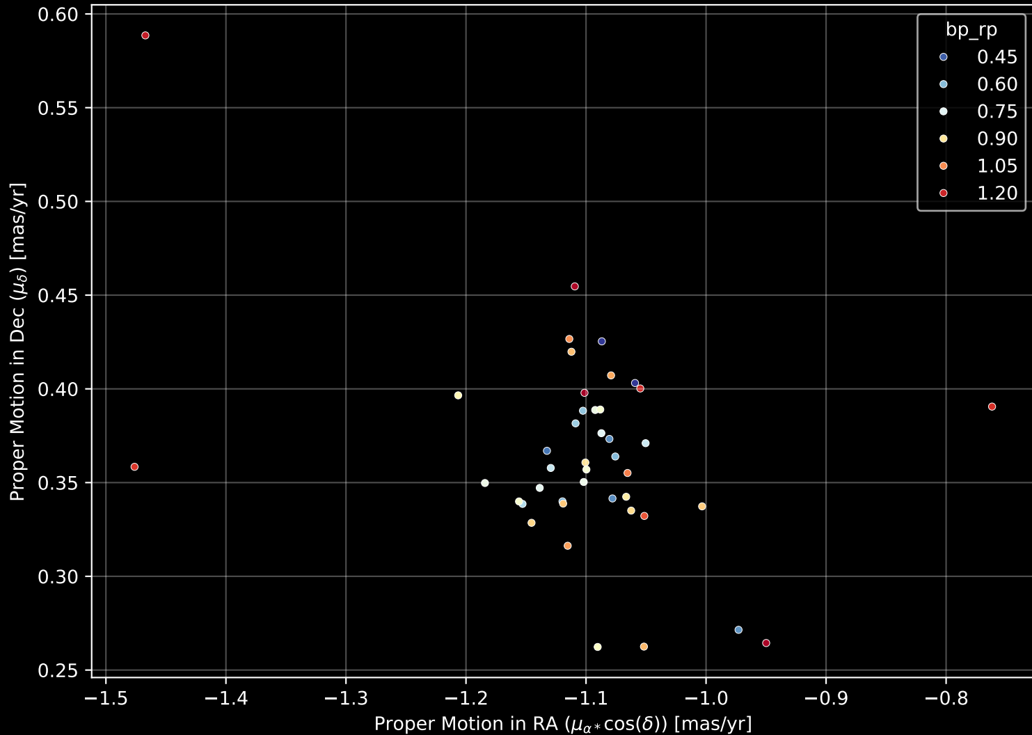
Gaia Cluster: [UBC_83] Proper Motion Diagram (n= 43)
