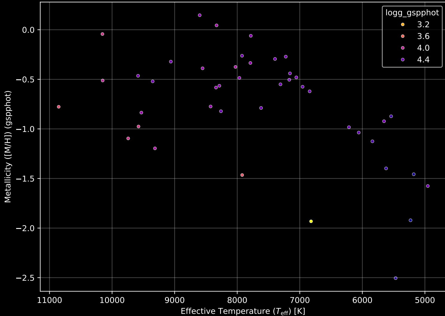
Gaia Cluster: [UBC_83] Stellar Population Parameters (n= 43)
