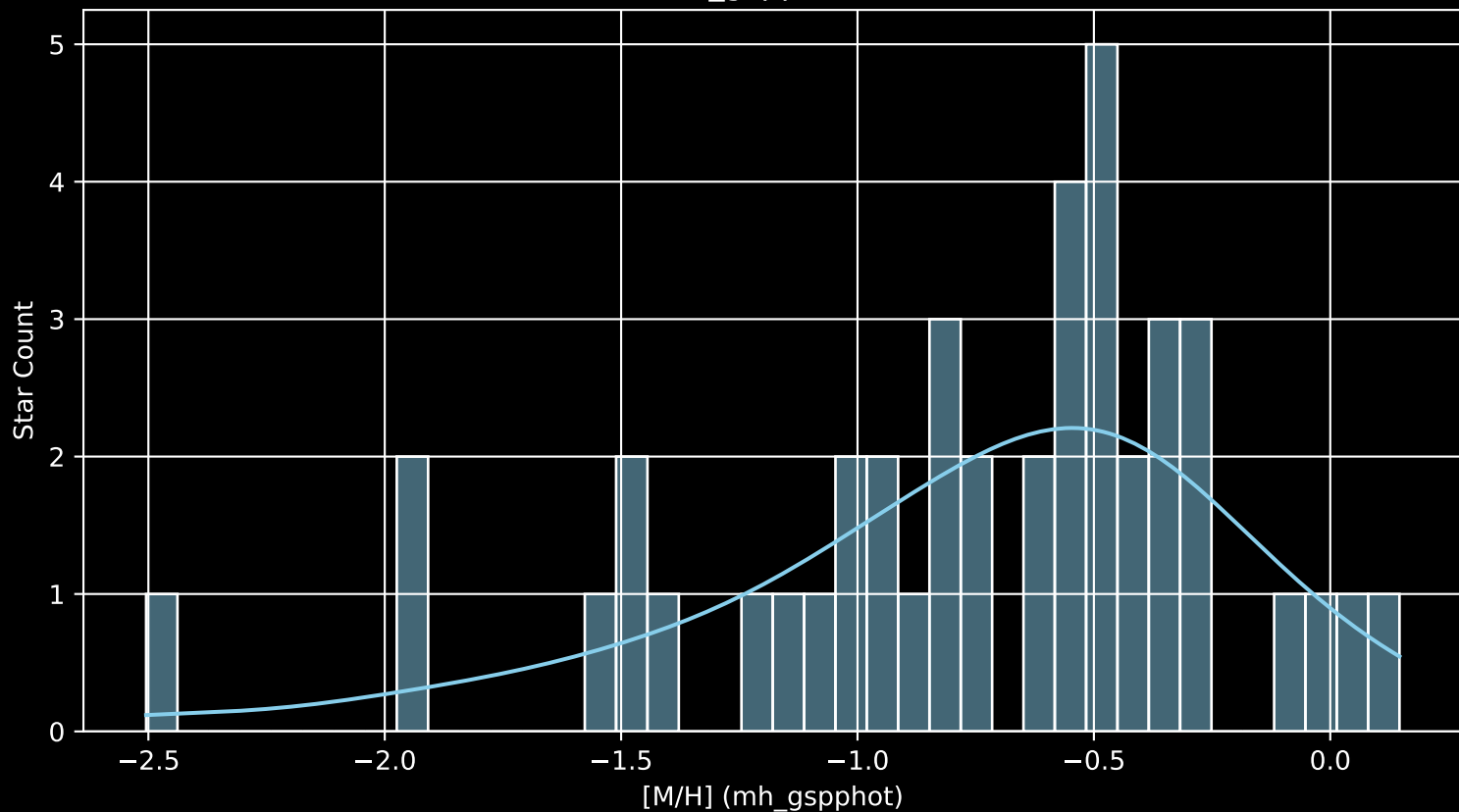
Gaia Cluster: [UBC_83 [M/H] (mh_gspphot) ( \bar{n}= 43 )
