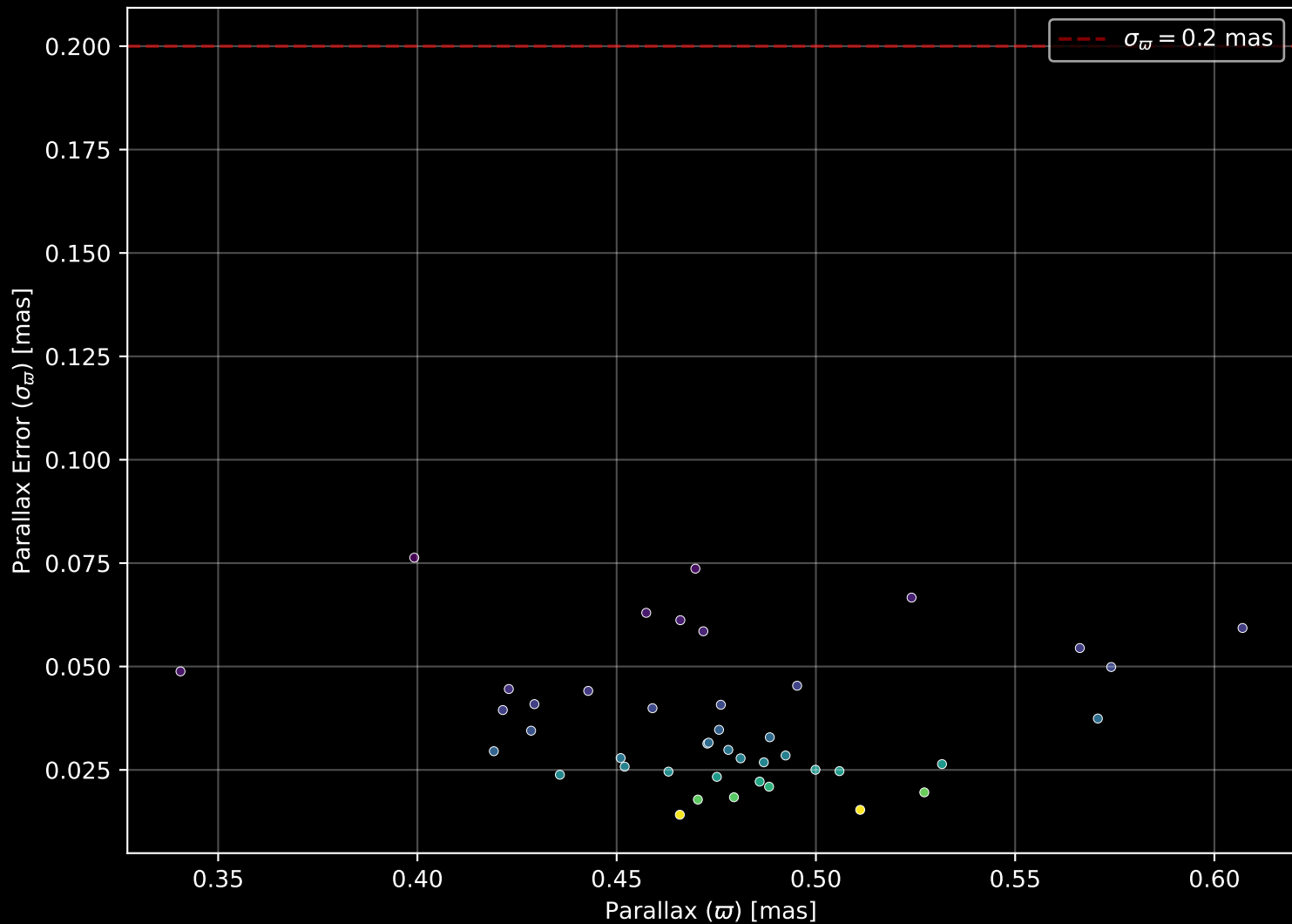
Gaia Cluster: [UBC_83] Parallax Quality (n= 43)
