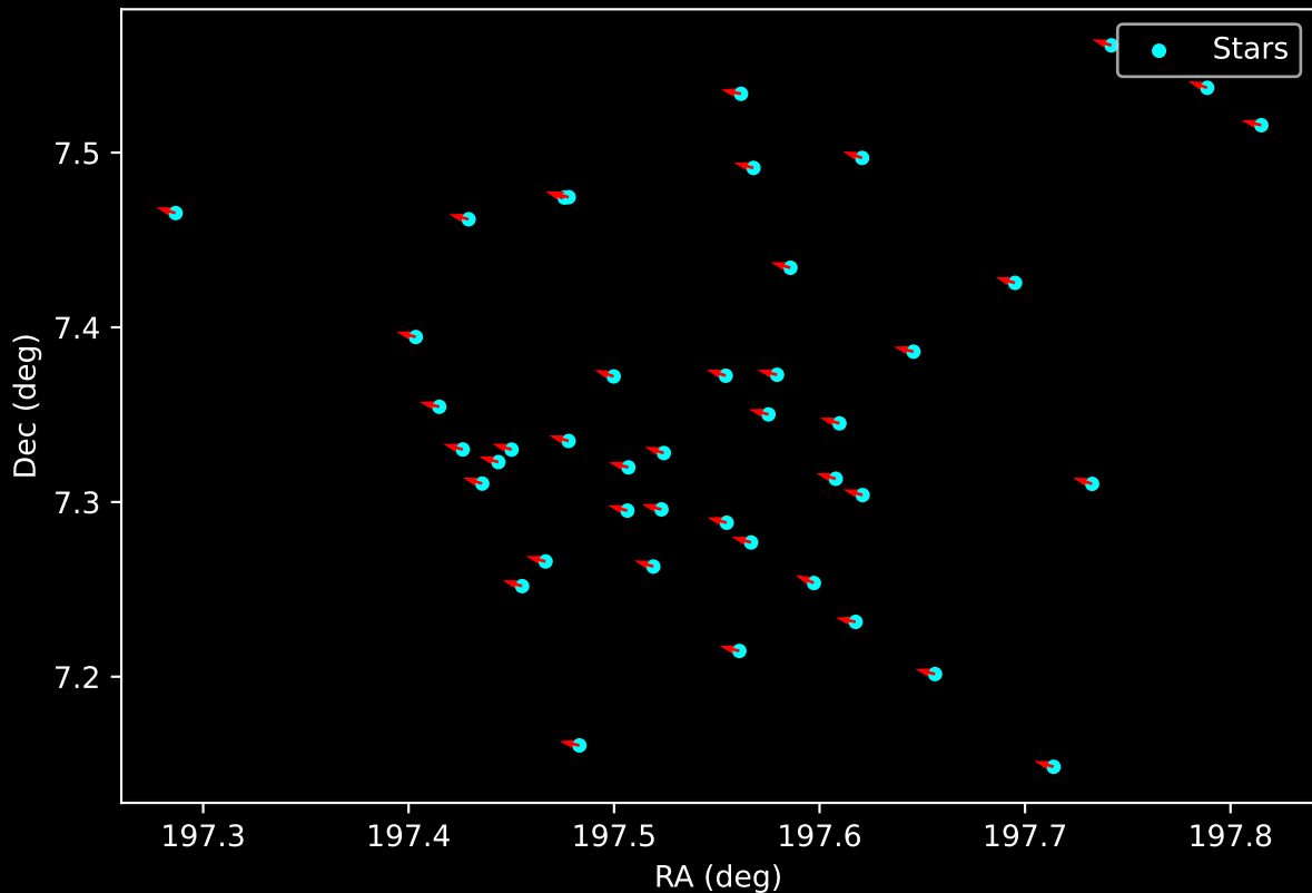
Gaia Cluster: [UBC_83] Proper Motion Vectors for Gaia Star Field (n= 43)
