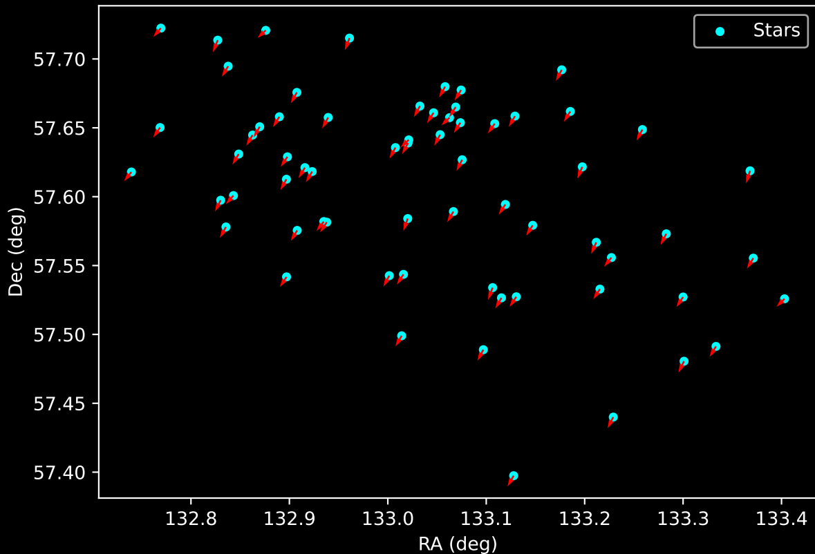
Gaia Cluster: [UBC_86] Proper Motion Vectors for Gaia Star Field (n= 65)
