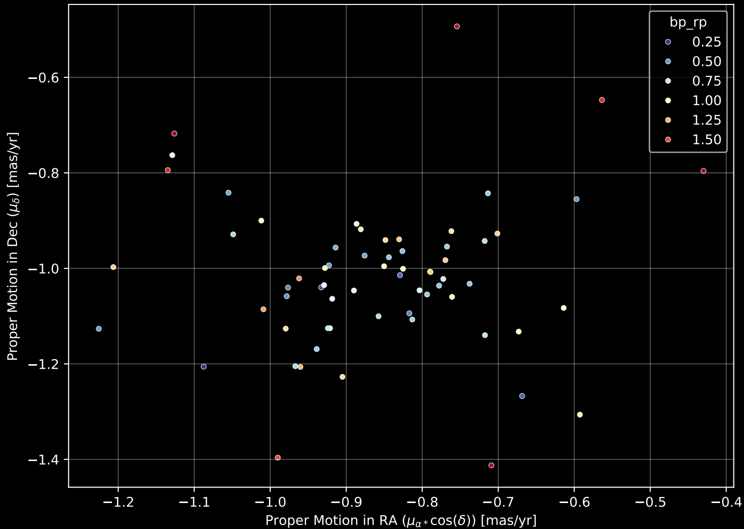
Gaia Cluster: [UBC_86] Proper Motion Diagram (n= 65)
