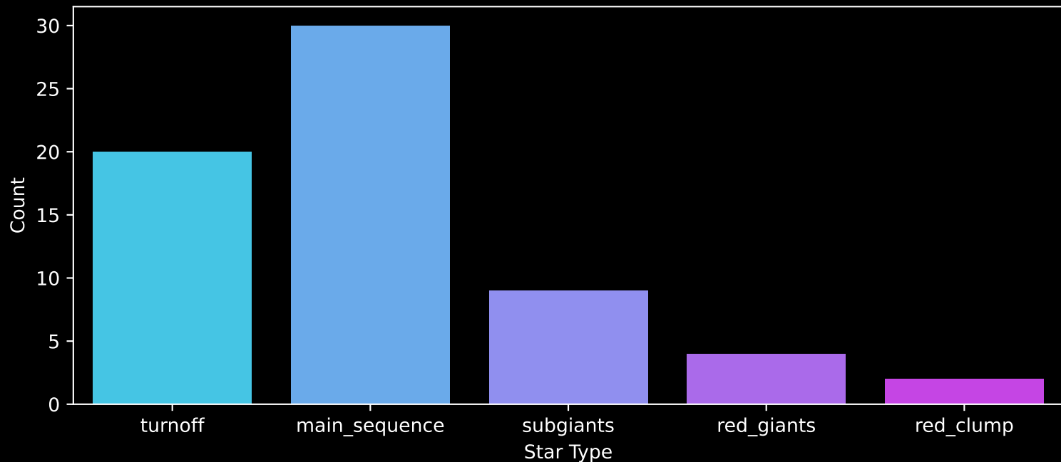
Gaia Cluster: [UBC_86] Count plot of Star Type
