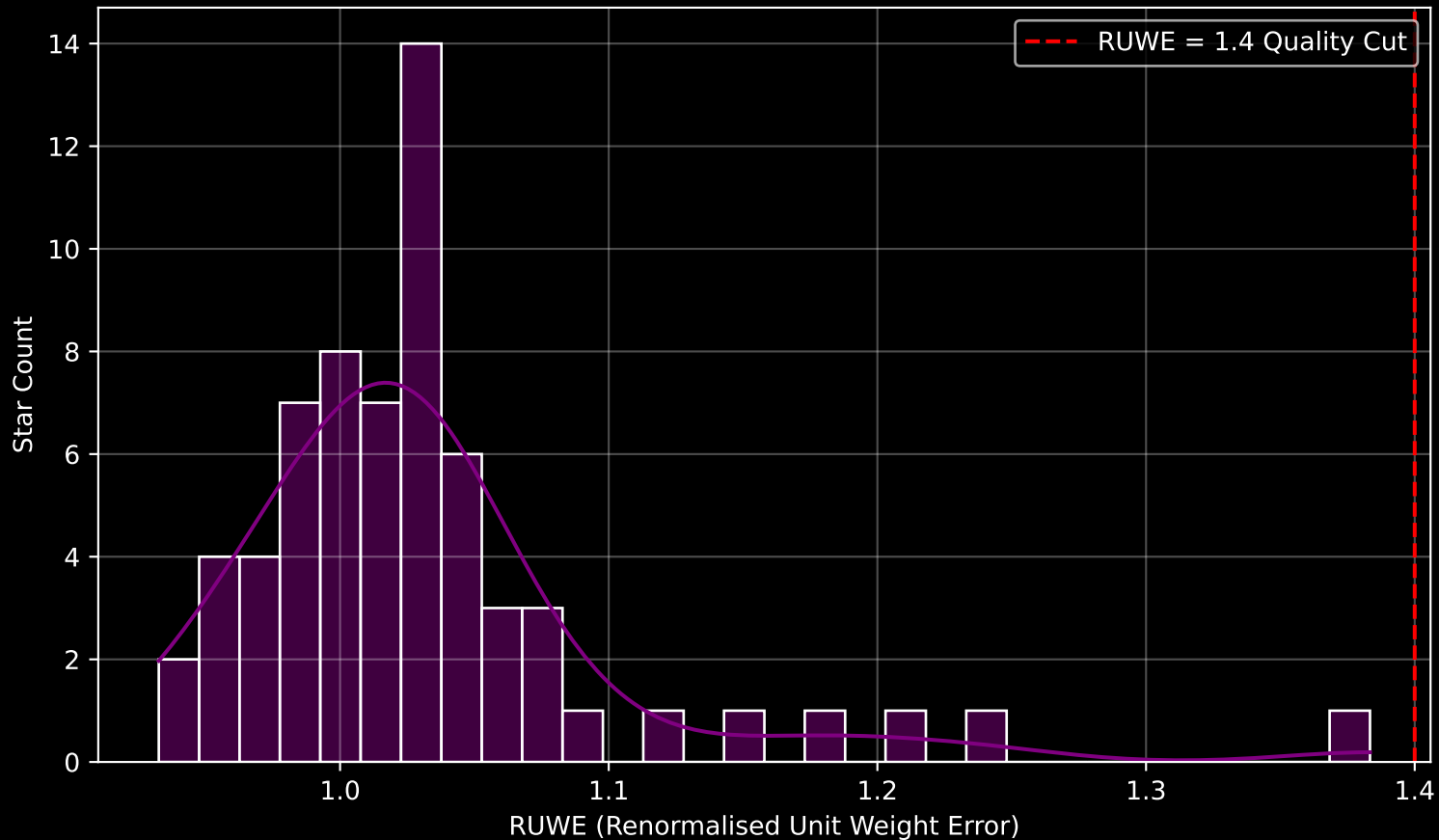
Gaia Cluster: [UBC_86] RUWE Distribution (n= 65)
