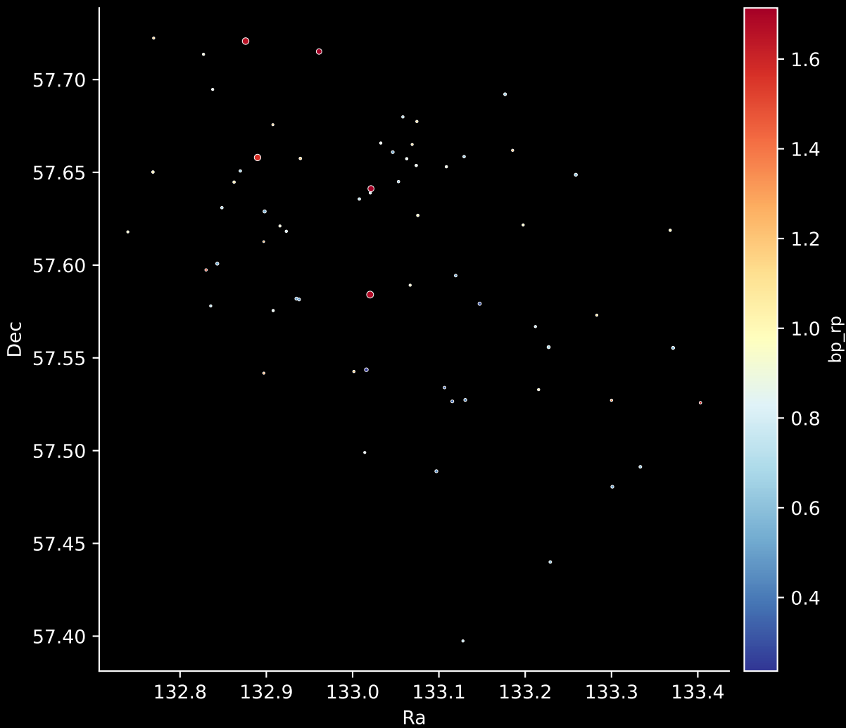
Gaia Cluster: [UBC_86] Stars: 65
