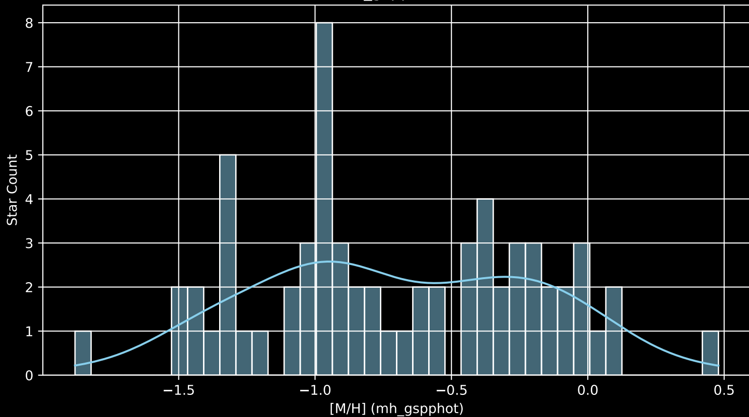
Gaia Cluster: [UBC_86 [M/H] (mh_gspphot) (n= 65)
