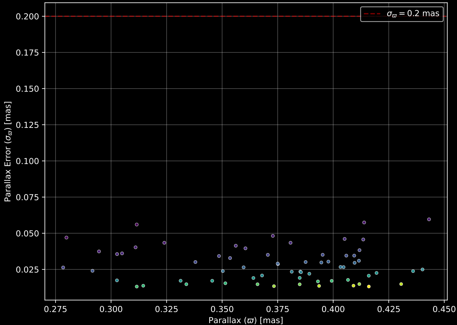
Gaia Cluster: [UBC_86] Parallax Quality (n= 65)
