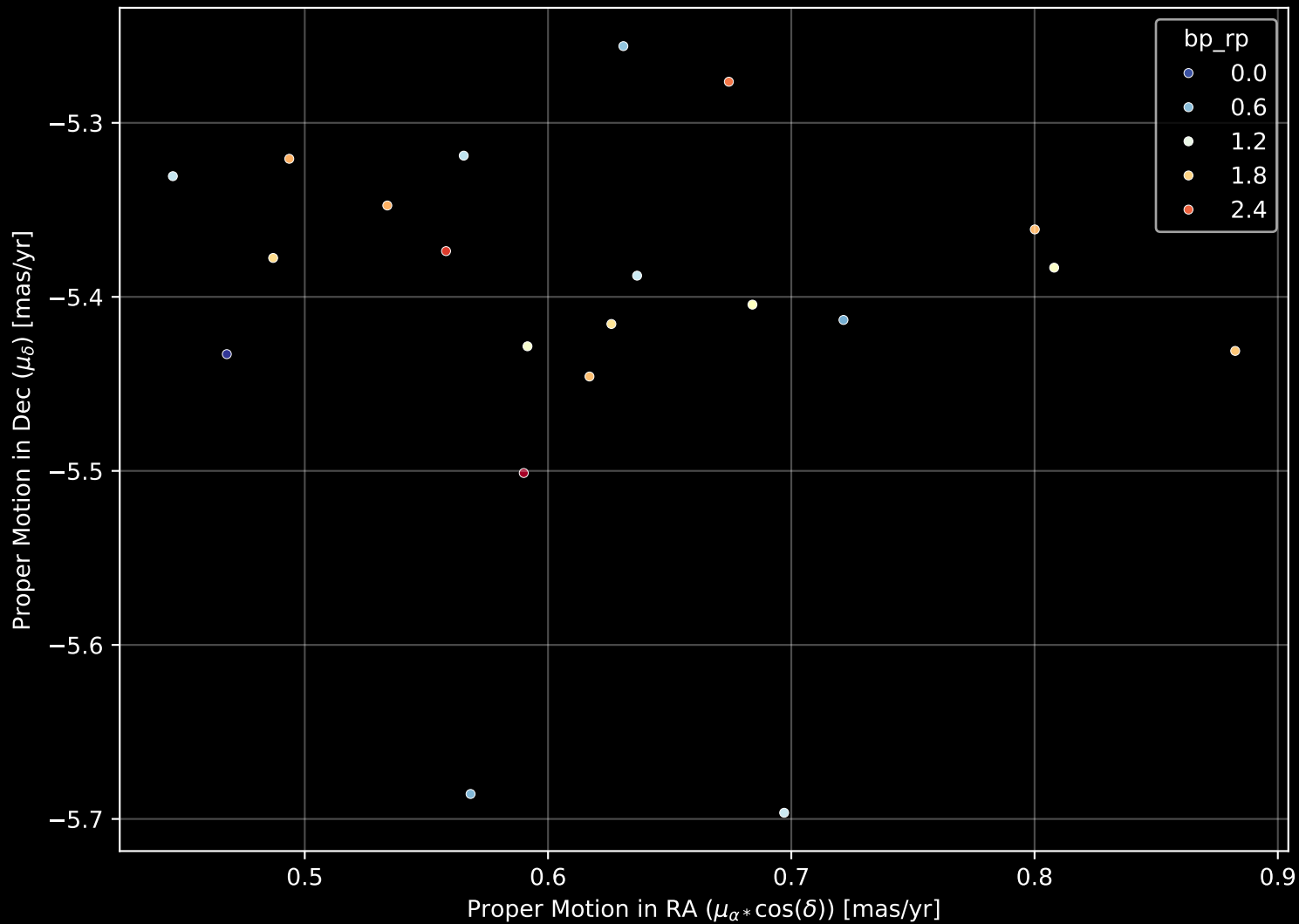
Gaia Cluster: [UBC_9] Proper Motion Diagram (n= 21)
