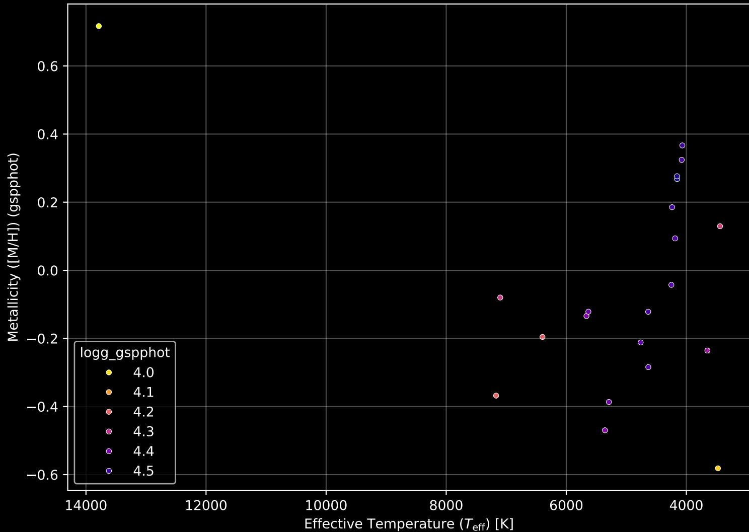
Gaia Cluster: [UBC_9] Stellar Population Parameters (n= 21)
