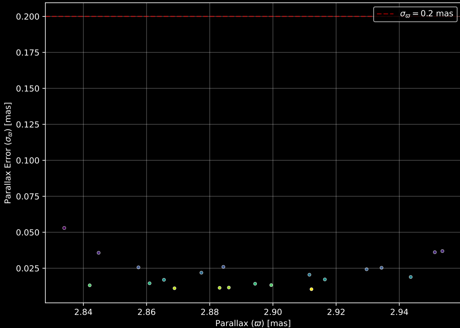
Gaia Cluster: [UBC_9] Parallax Quality (n= 21)
