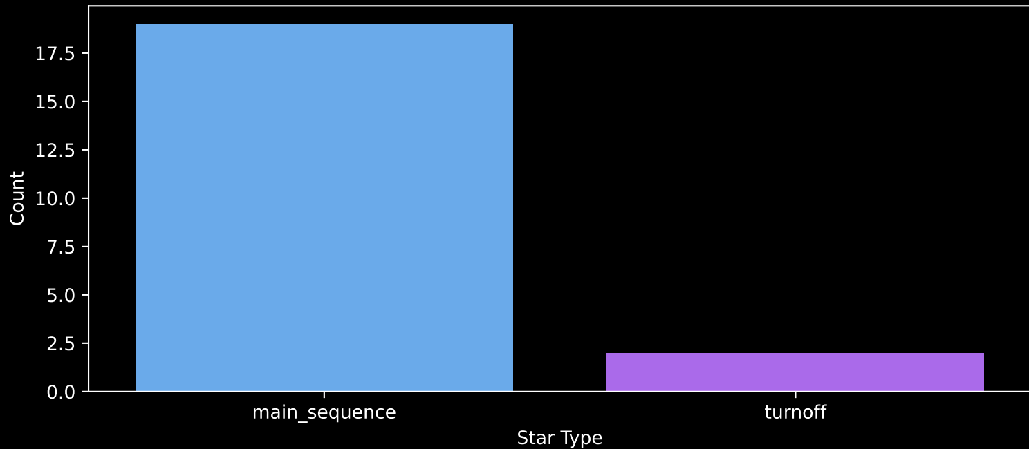
Gaia Cluster: [UBC_9] Count plot of Star Type
