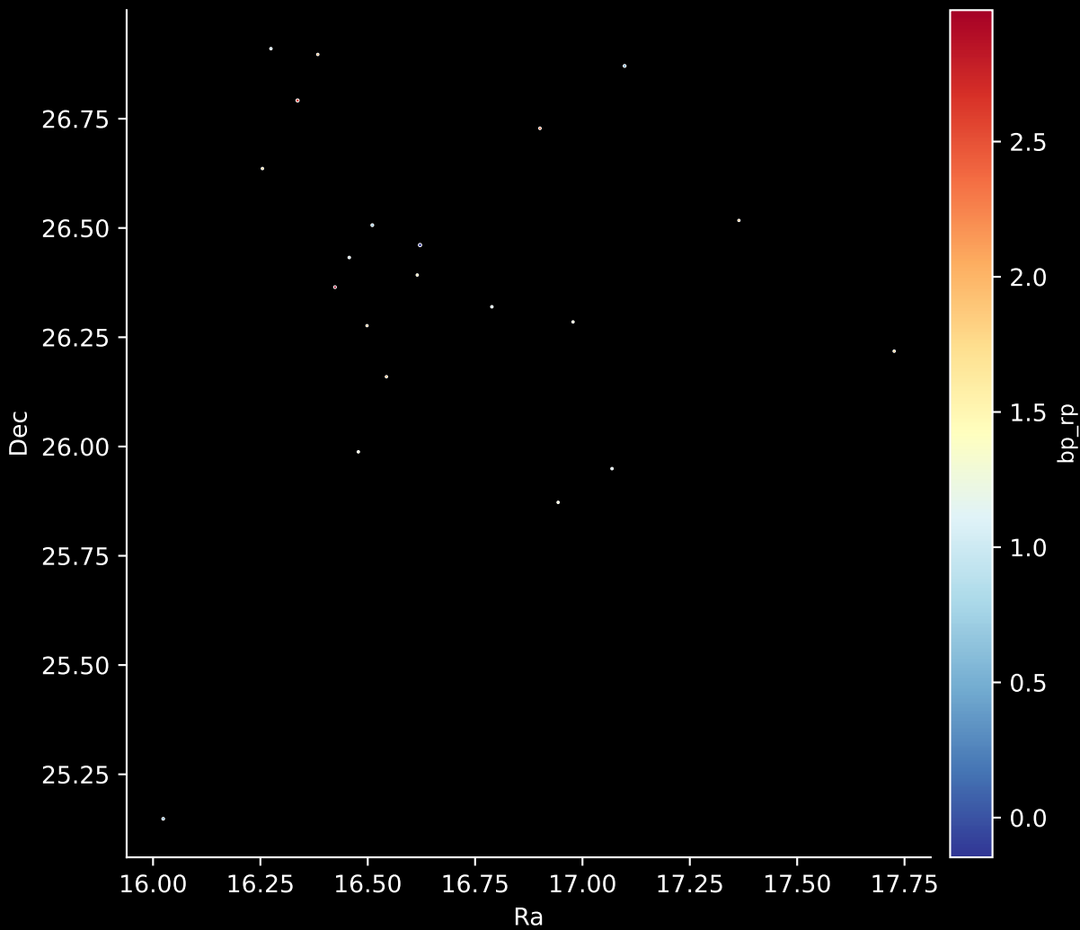
Gaia Cluster: [UBC_9] Stars: 21
