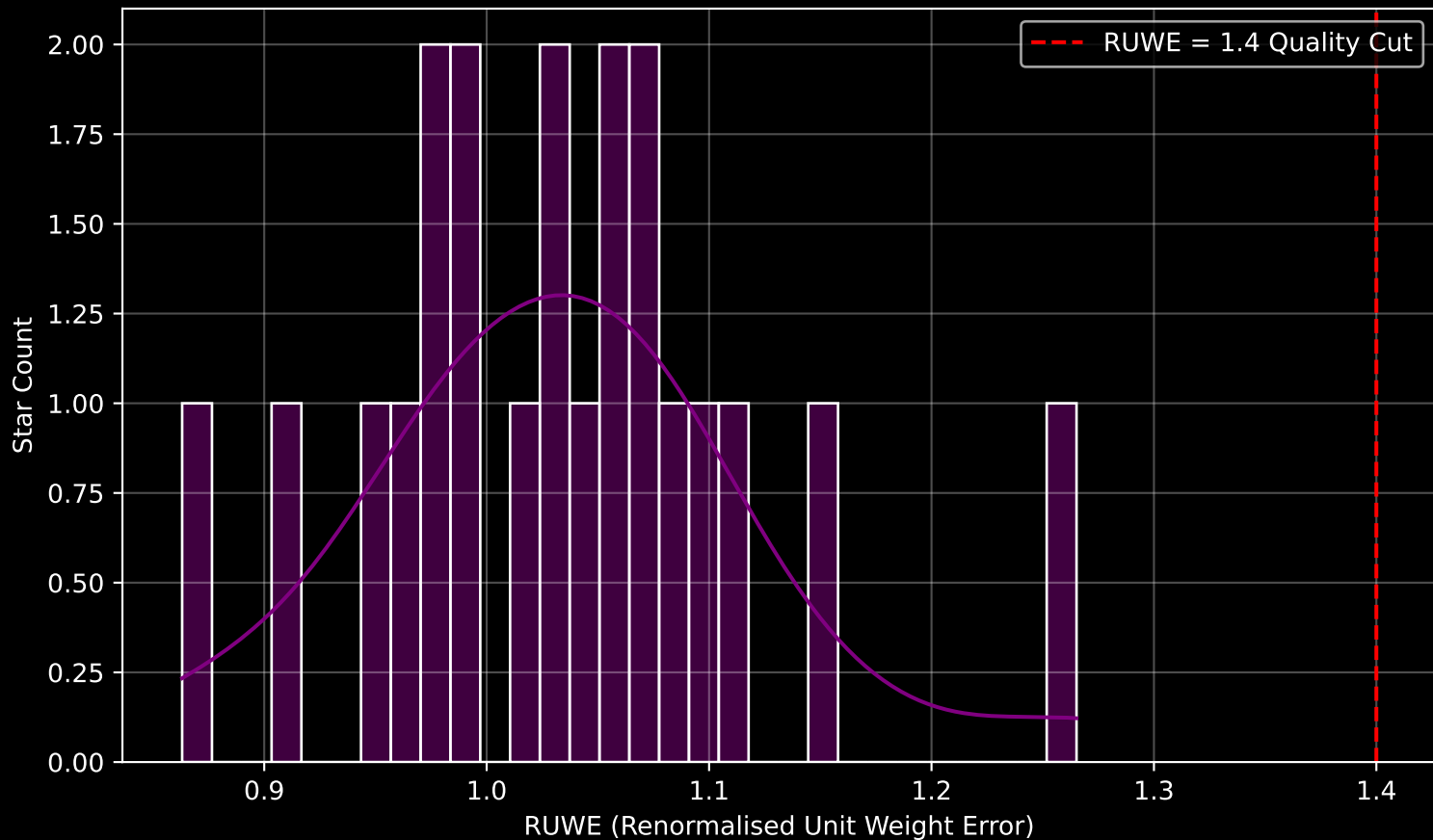
Gaia Cluster: [UBC_9] RUWE Distribution (n= 21)
