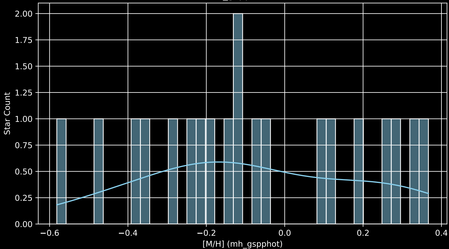
Gaia Cluster: [UBC_9 [M/H] (mh_gspphot) (n= 20)
