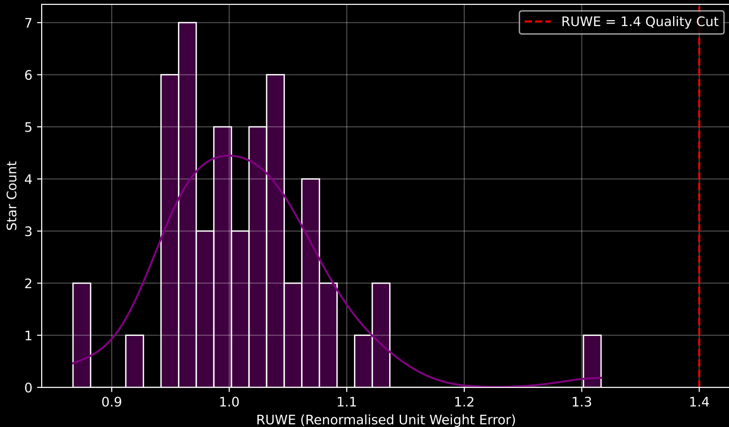
Gaia Cluster: [UBC_90] RUWE Distribution (n= 50)
