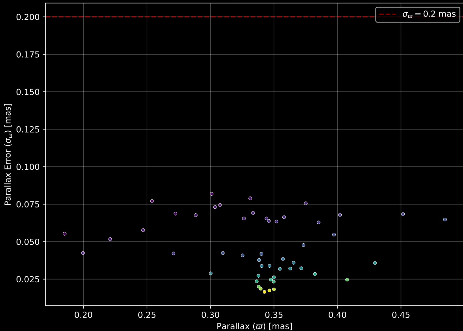
Gaia Cluster: [UBC_90] Parallax Quality (n= 50)
