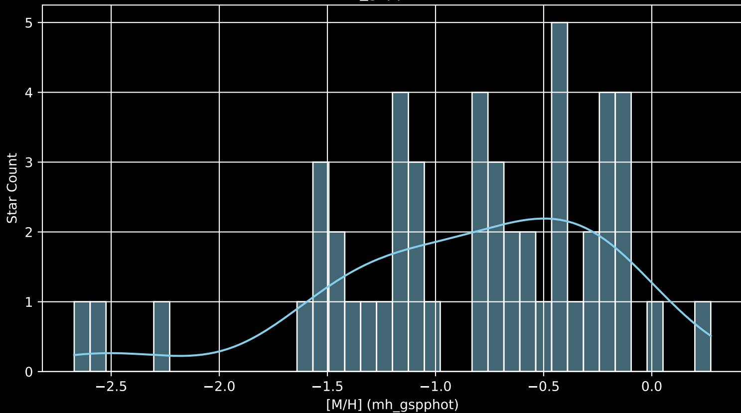
Gaia Cluster: [UBC_90 [M/H] (mh_gspphot) (n= 50)
