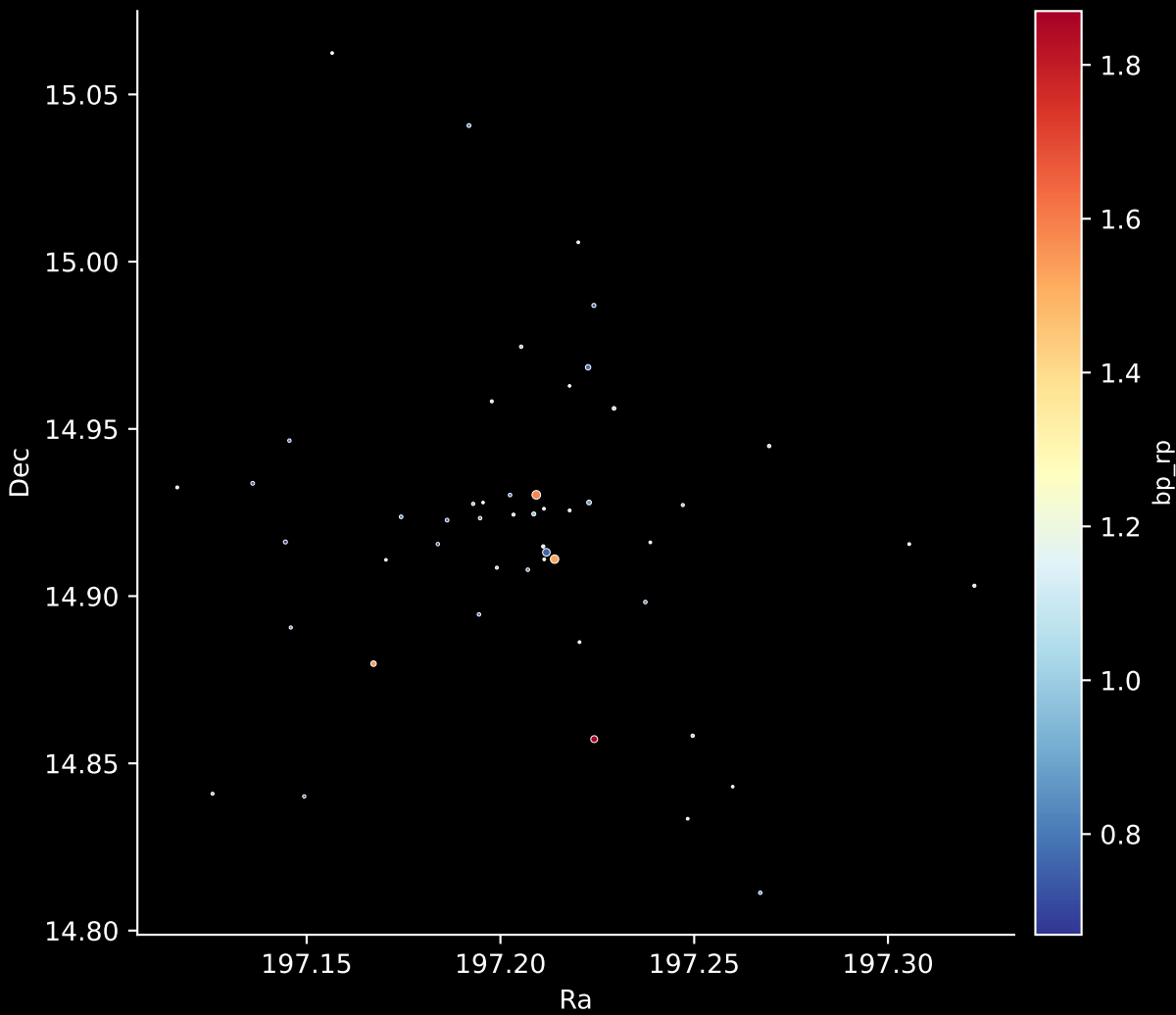
Gaia Cluster: [UBC_90] Stars: 50
