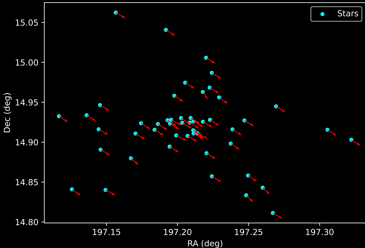
Gaia Cluster: [UBC_90] Proper Motion Vectors for Gaia Star Field (n= 50)
