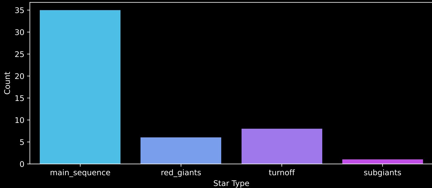
Gaia Cluster: [UBC_90] Count plot of Star Type
