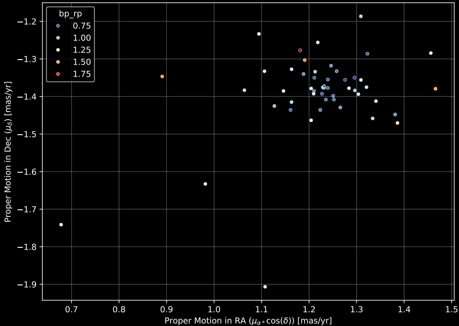
Gaia Cluster: [UBC_90] Proper Motion Diagram (n= 50)
