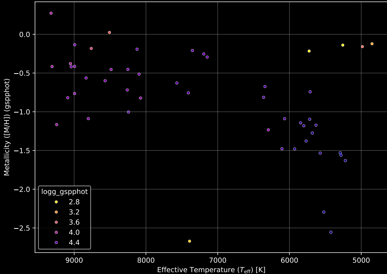
Gaia Cluster: [UBC_90] Stellar Population Parameters (n= 50)
