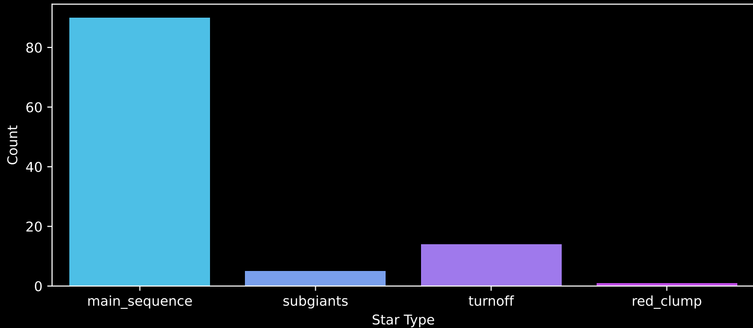
Gaia Cluster: [UPK_108] Count plot of Star Type
