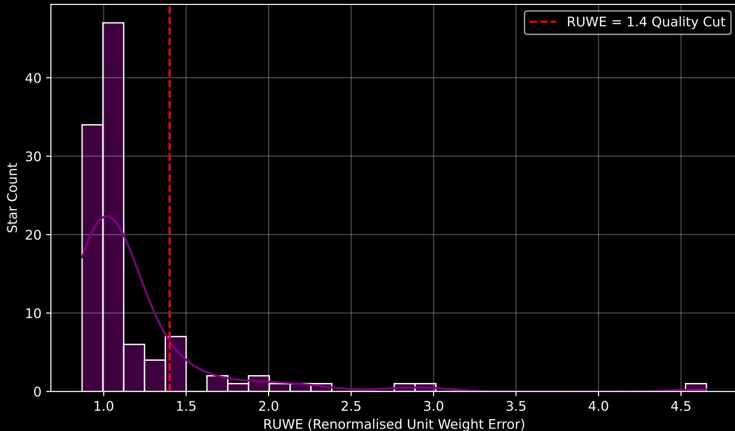
Gaia Cluster: [UPK_108] RUWE Distribution (n= 109)
