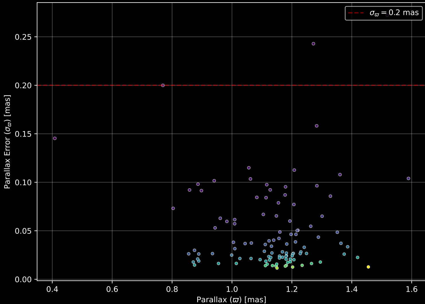
Gaia Cluster: [UPK_108] Parallax Quality (n= 110)
