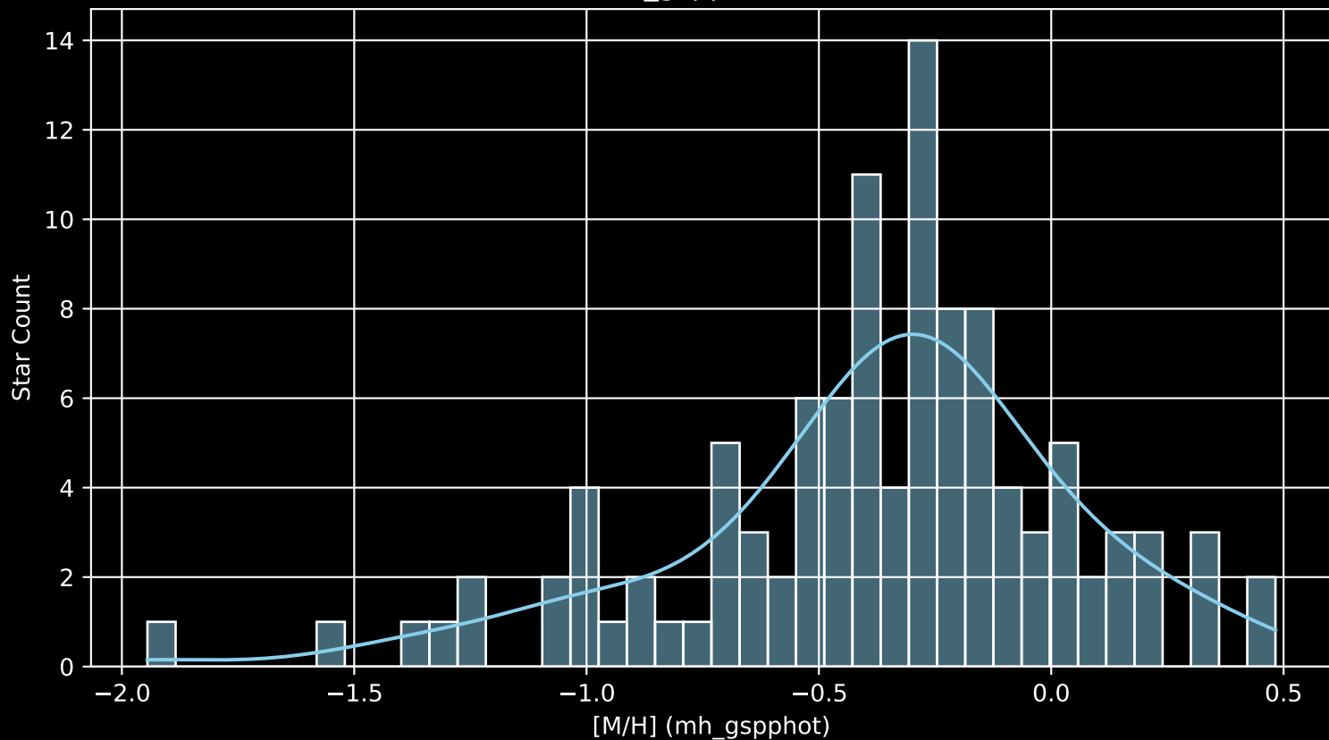
Gaia Cluster: [UPK_108 [M/H] (mh_gspphot) (n= 109)
