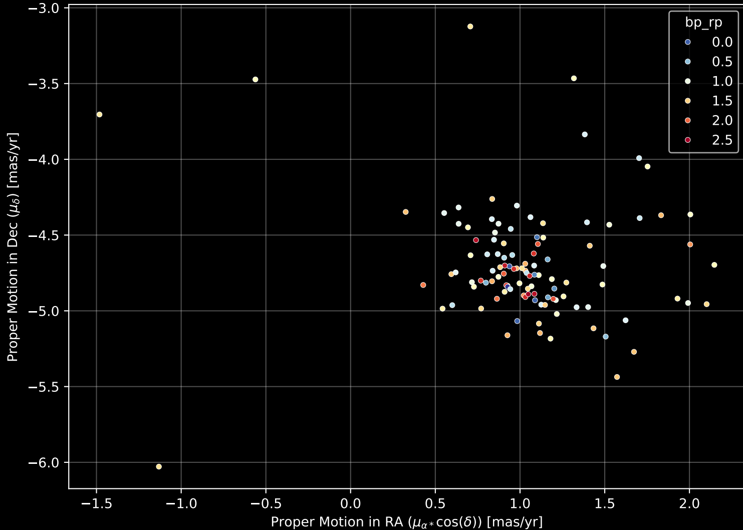
Gaia Cluster: [UPK_108] Proper Motion Diagram (n= 110)
