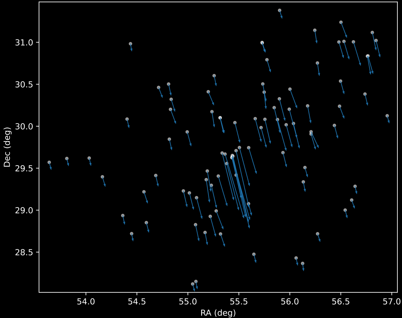
Gaia DR3 Cluster 0 Proper Motion Vectors (n=93)
