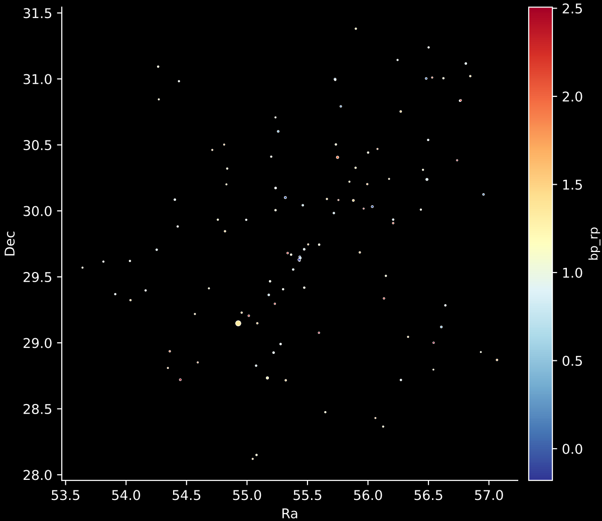
Gaia Cluster: [UPK_108] Stars: 110
