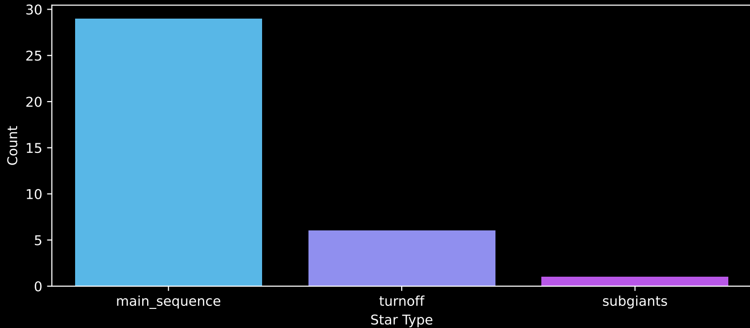
Gaia Cluster: [UPK_119] Count plot of Star Type
