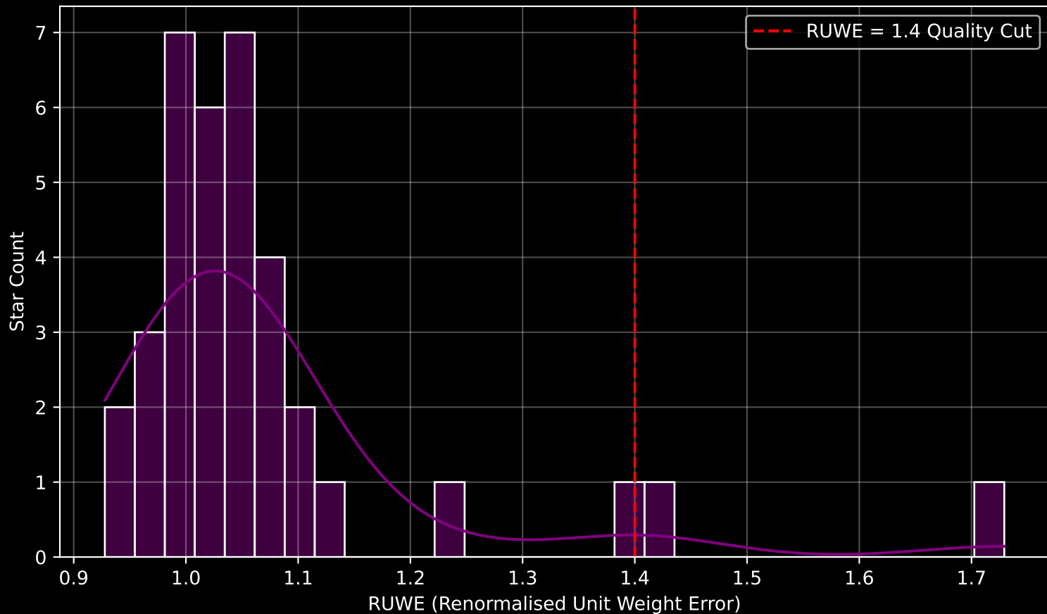
Gaia Cluster: [UPK_119] RUWE Distribution (n= 36)
