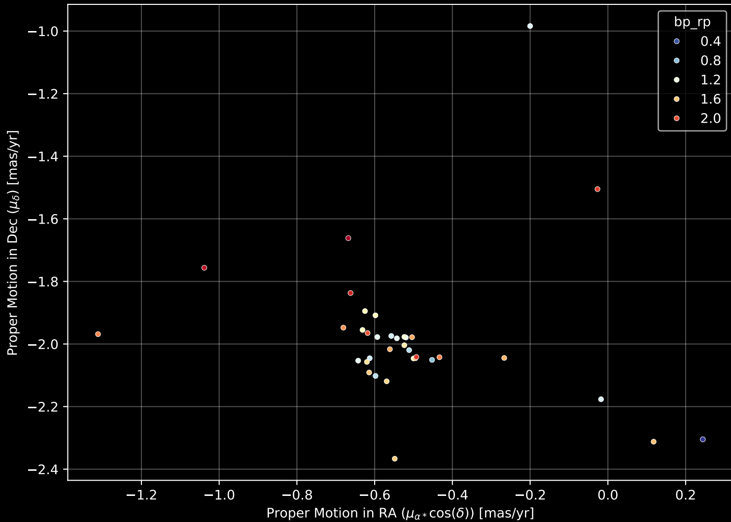
Gaia Cluster: [UPK_119] Proper Motion Diagram (n= 36)
