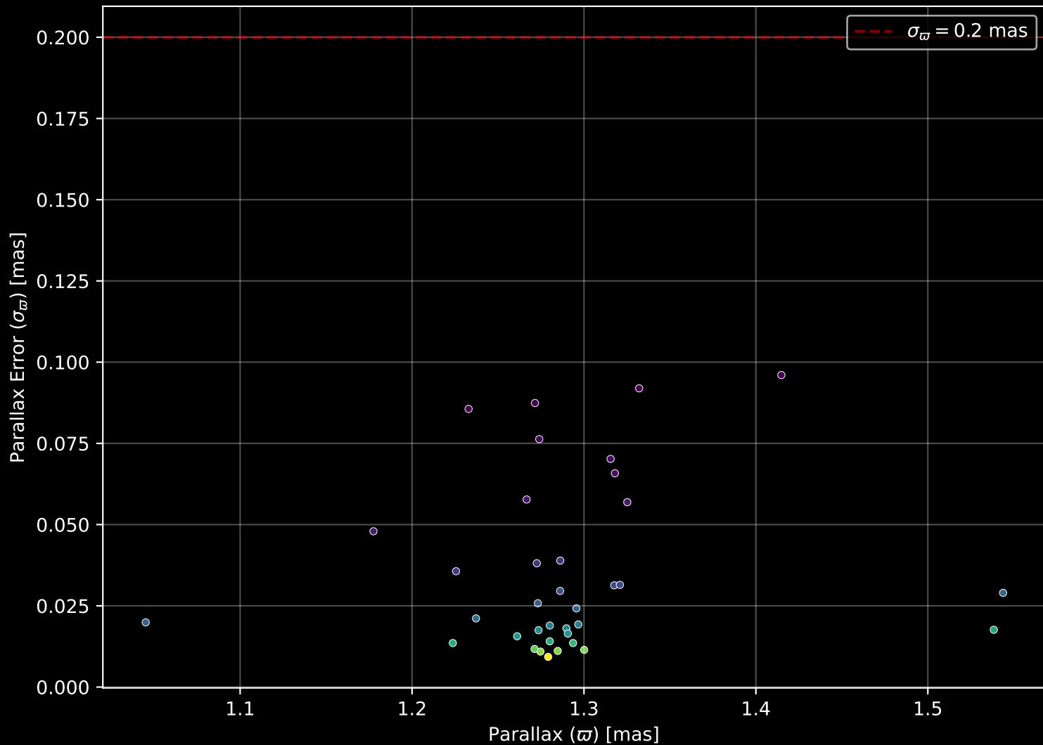
Gaia Cluster: [UPK 119] Parallax Quality (n= 36)
