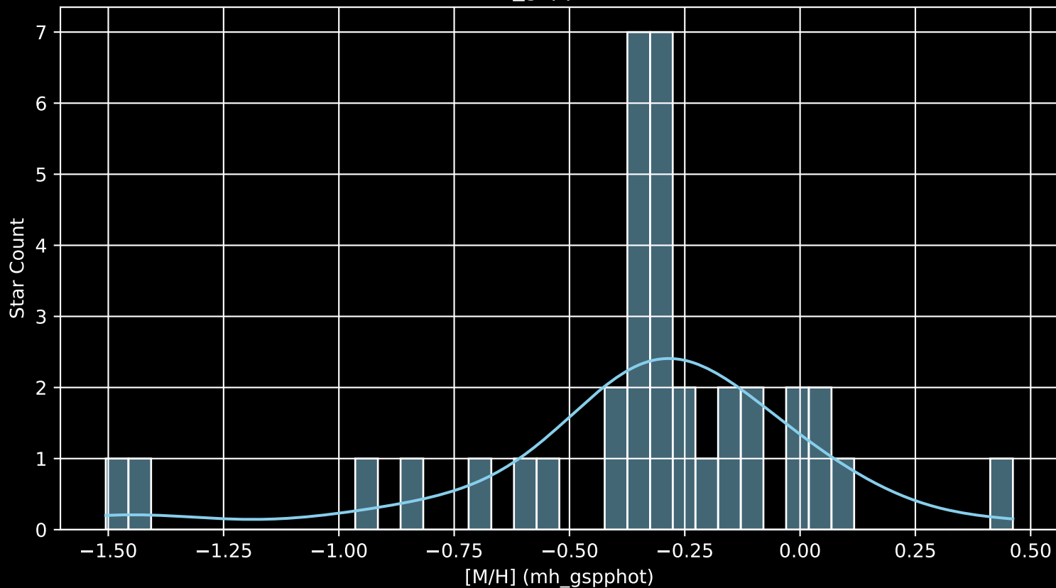
Gaia Cluster: [UPK_119 [M/H] (mh_gspphot) (n= 36)
