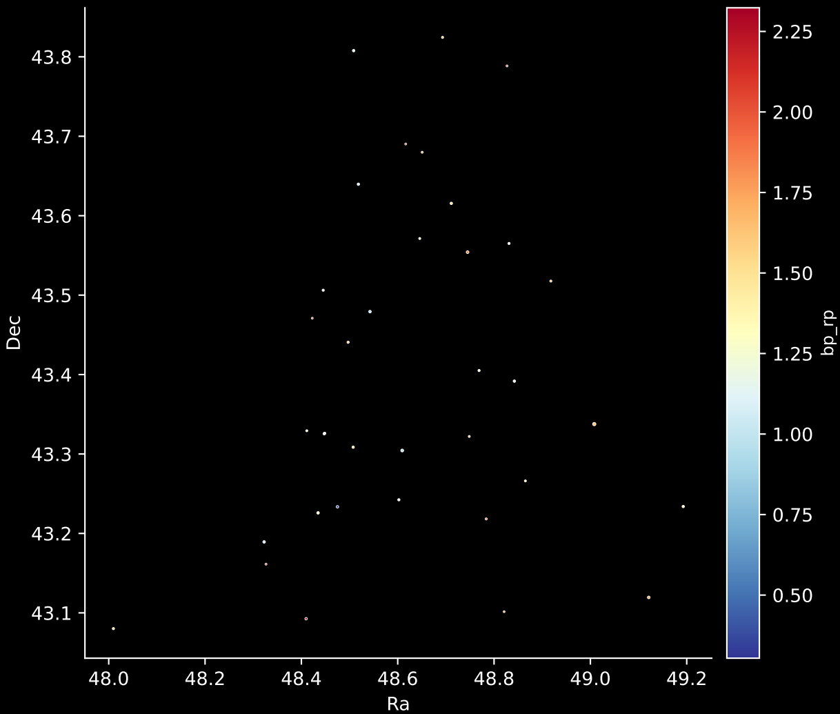
Gaia Cluster: [UPK_119] Stars: 36
