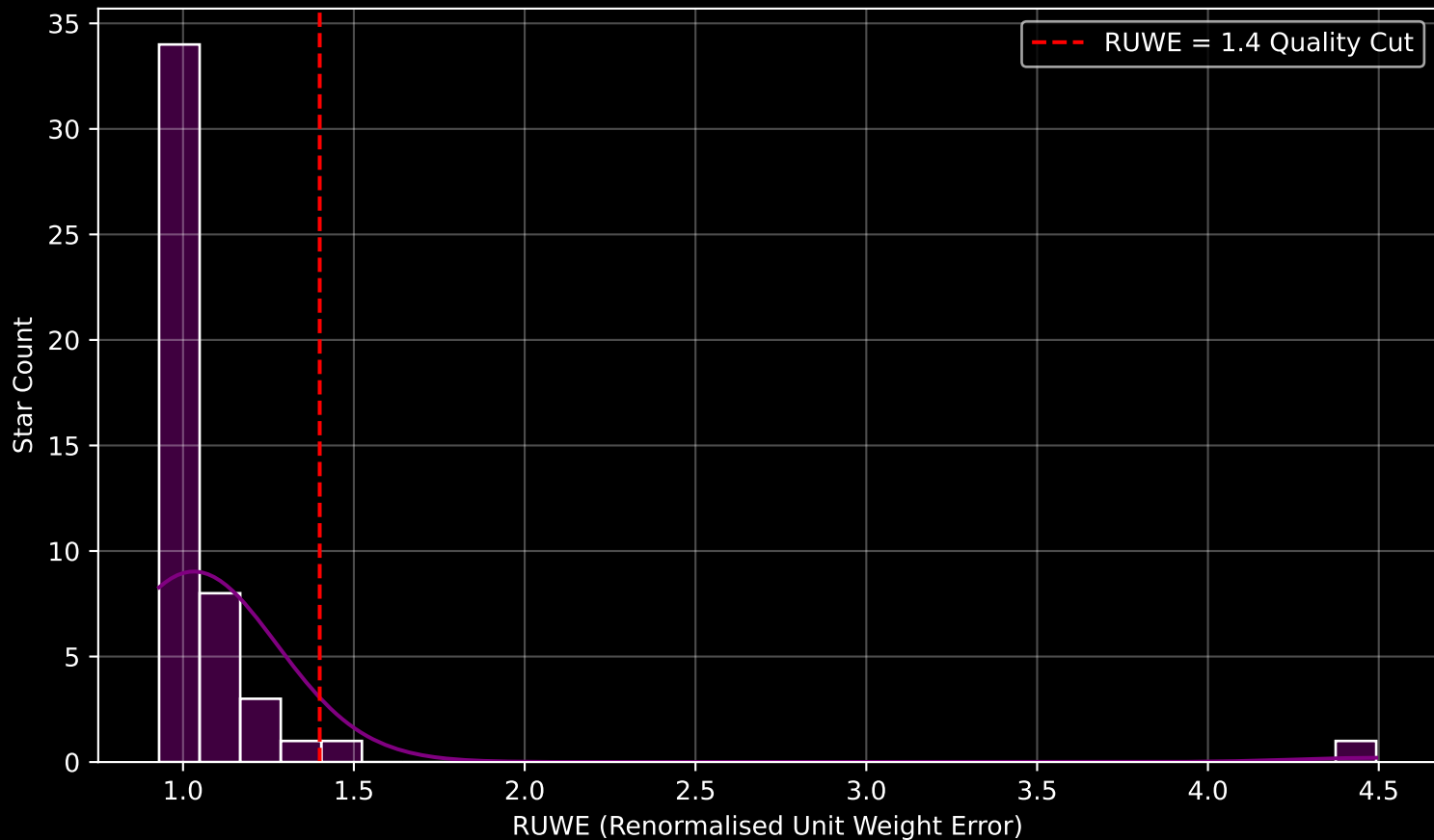
Gaia Cluster: [UPK_131] RUWE Distribution (n= 48)
