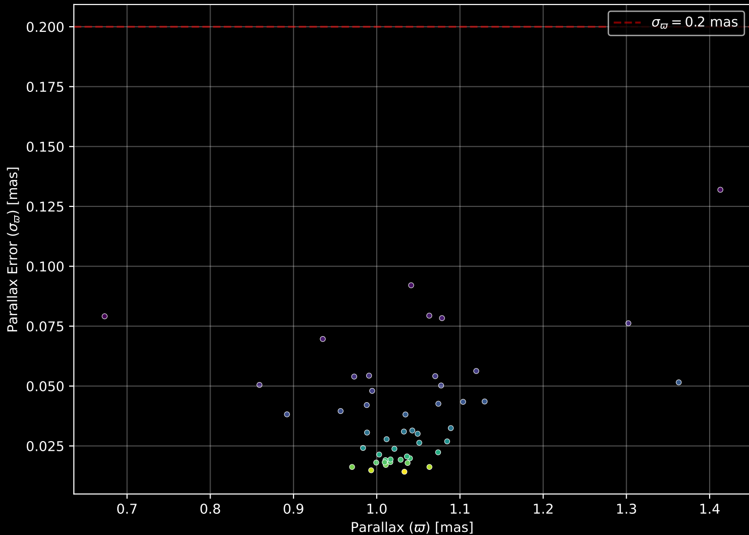
Gaia Cluster: [UPK_131] Parallax Quality (n= 48)
