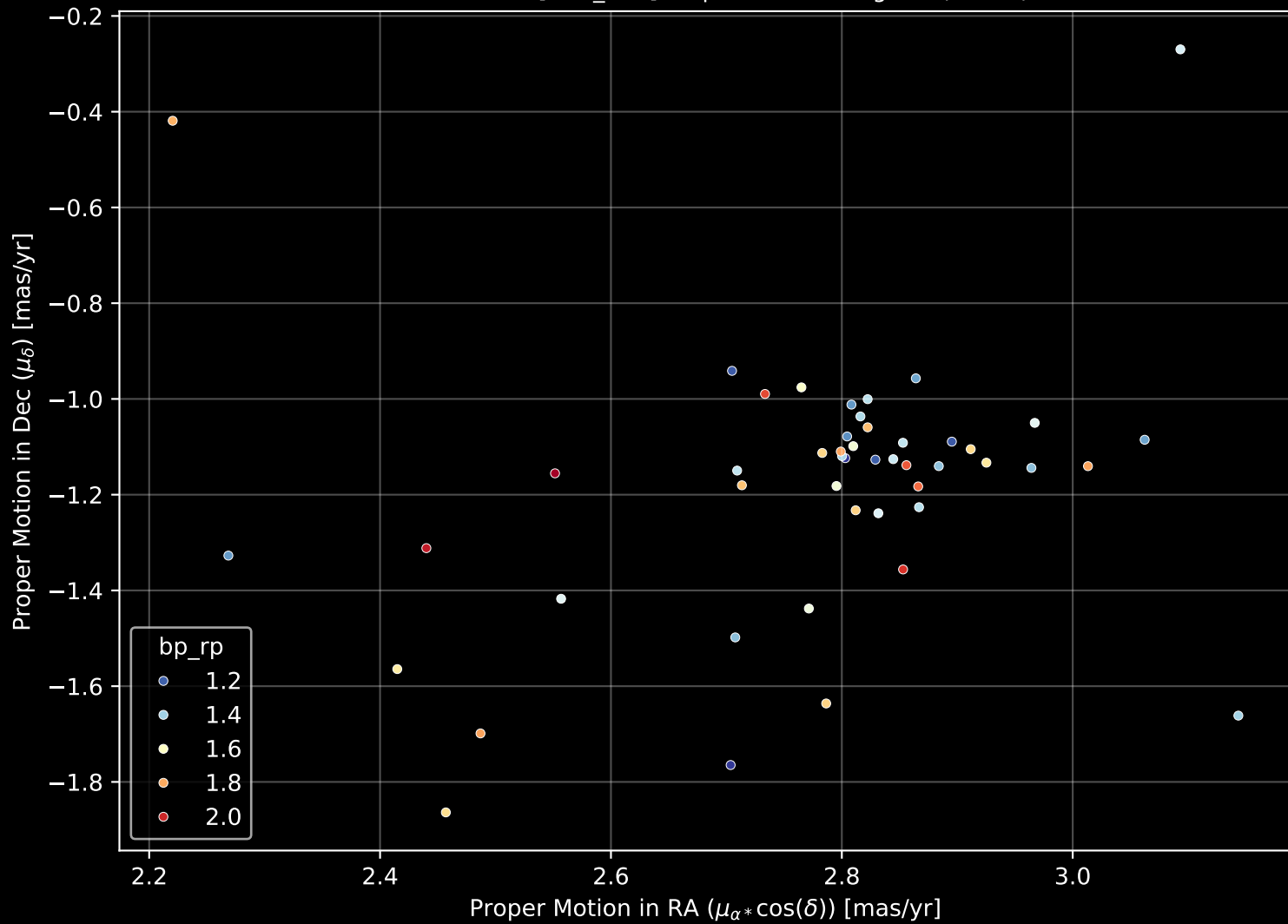
Gaia Cluster: [UPK_131] Proper Motion Diagram (n= 48)
