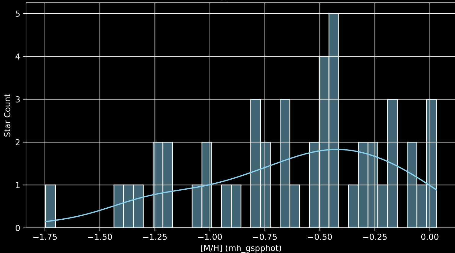
Gaia Cluster: [UPK_131 [M/H] (mh_gspphot) (n= 48)
