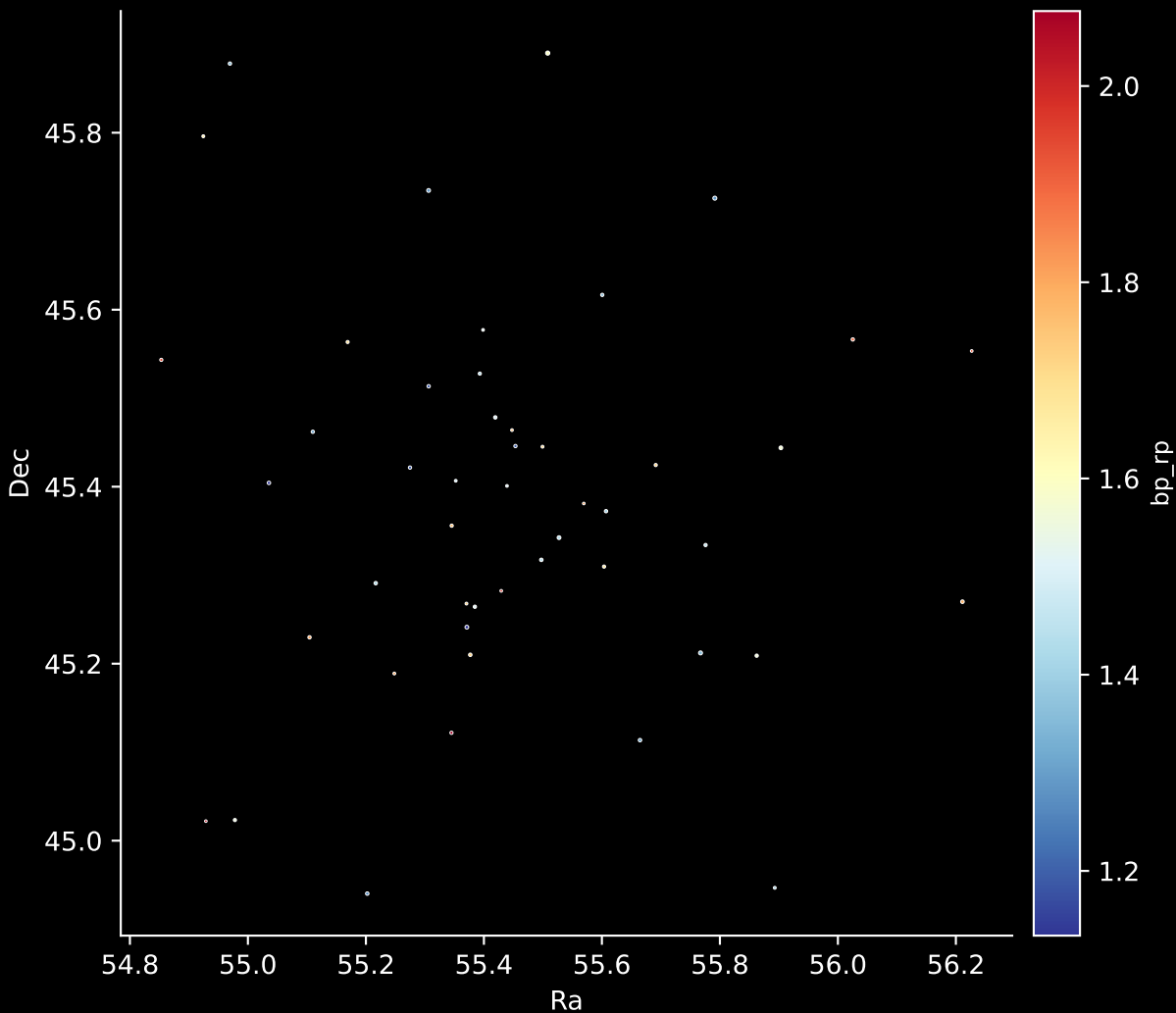
Gaia Cluster: [UPK_131] Stars: 48
