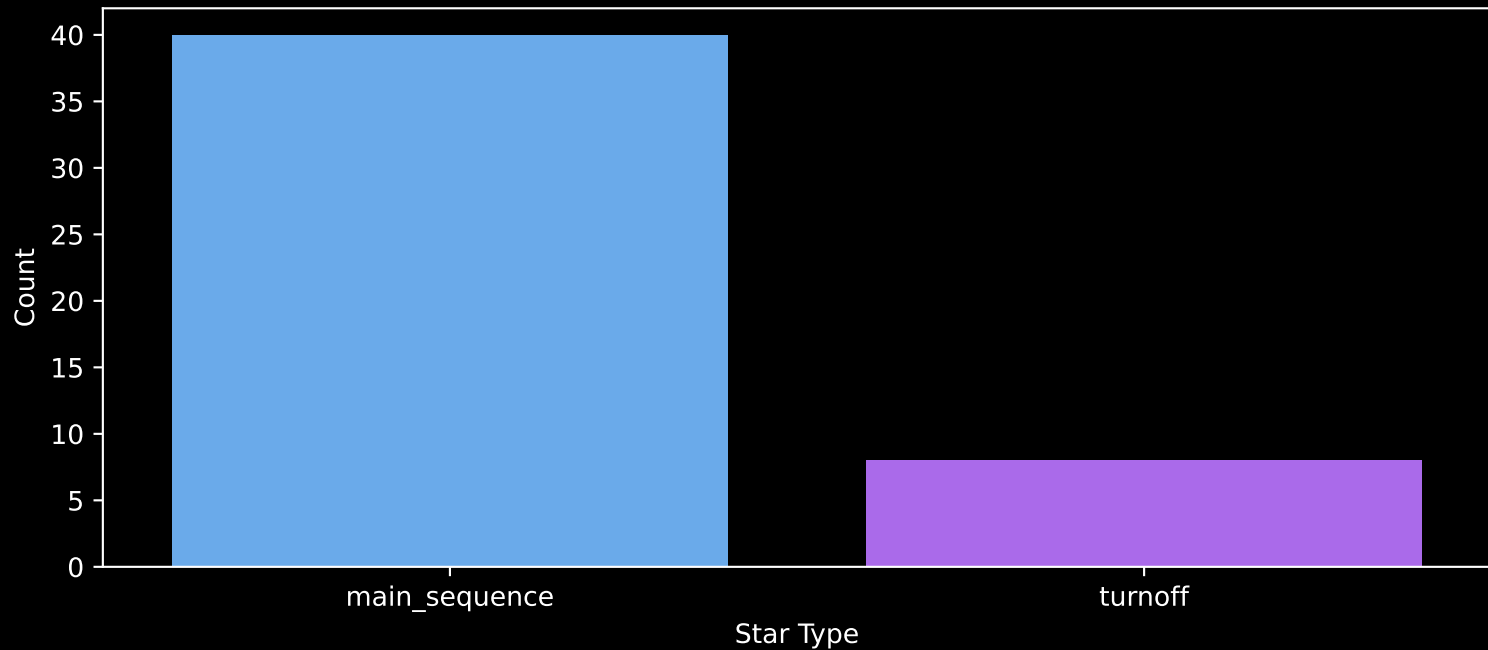
Gaia Cluster: [UPK_131] Count plot of Star Type
