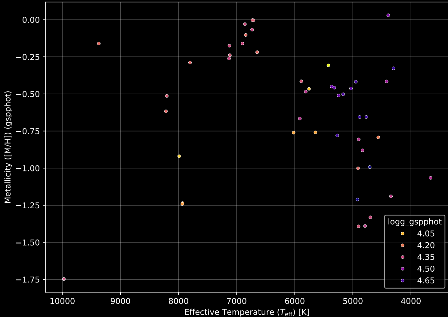
Gaia Cluster: [UPK_131] Stellar Population Parameters (n= 48)
