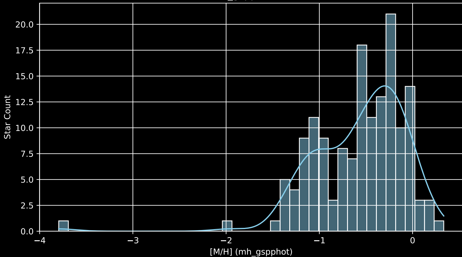
Gaia Cluster: [UPK_143 [M/H] (mh_gspphot) (n= 153)
