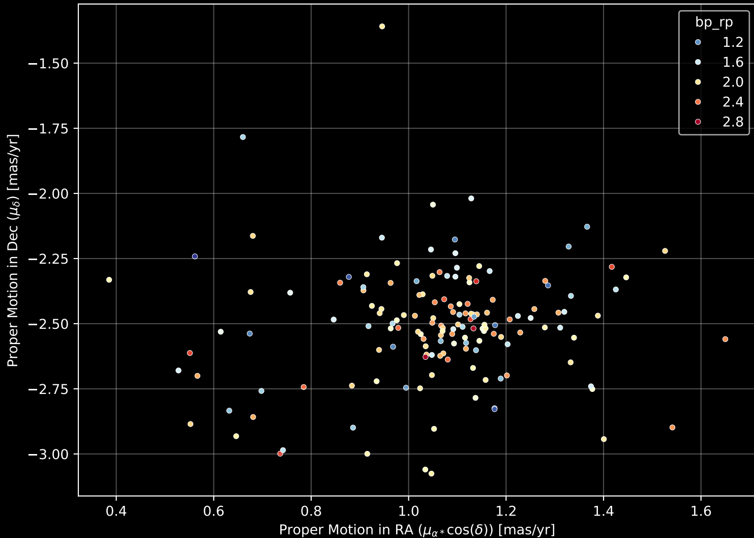
Gaia Cluster: [UPK_143] Proper Motion Diagram (n= 153)
