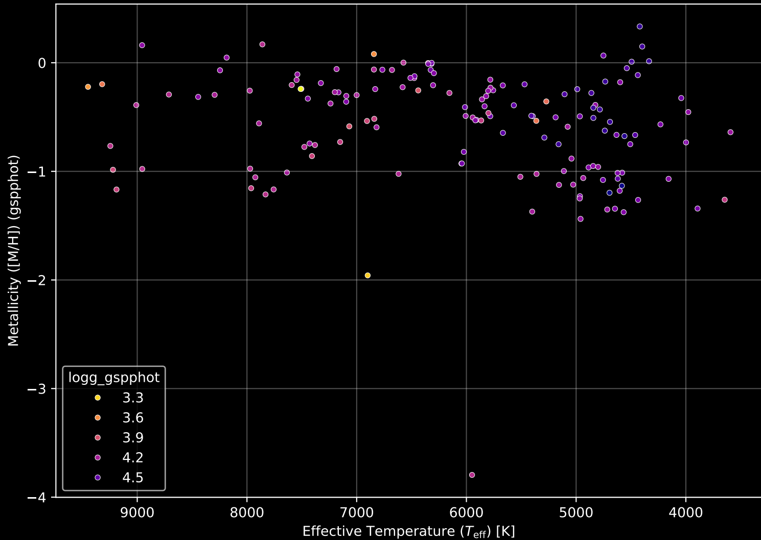
Gaia Cluster: [UPK_143] Stellar Population Parameters (n= 153)
