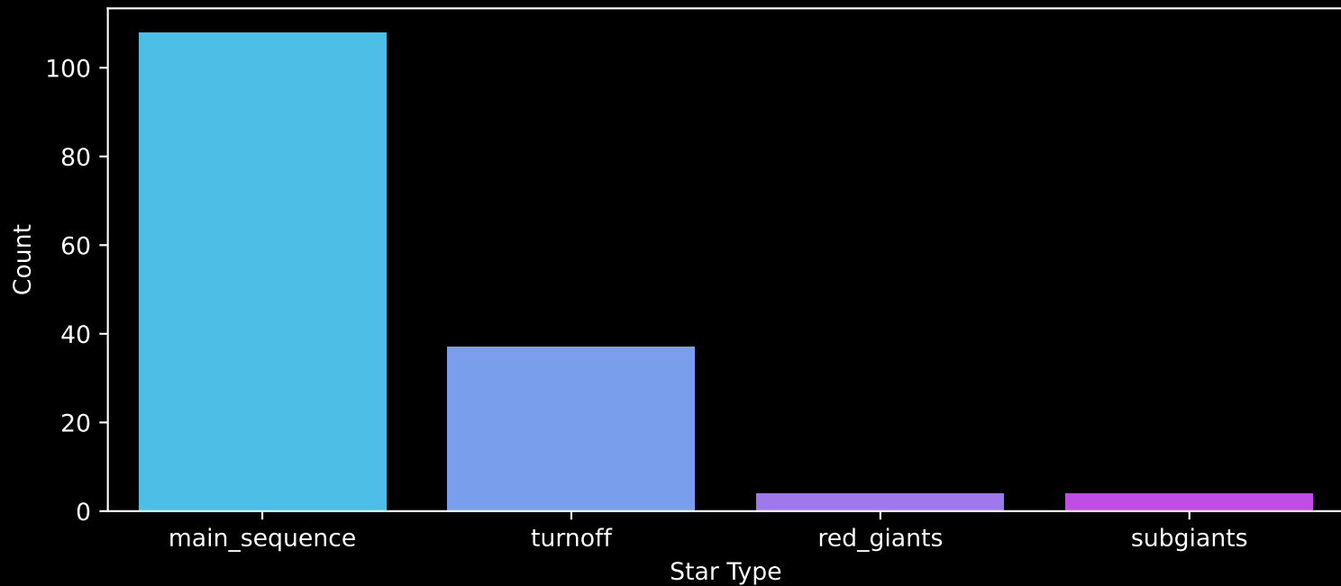
Gaia Cluster: [UPK_143] Count plot of Star Type
