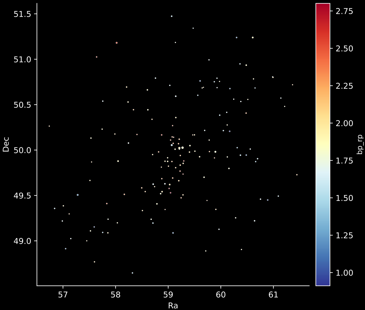
Gaia Cluster: [UPK_143] Stars: 153
