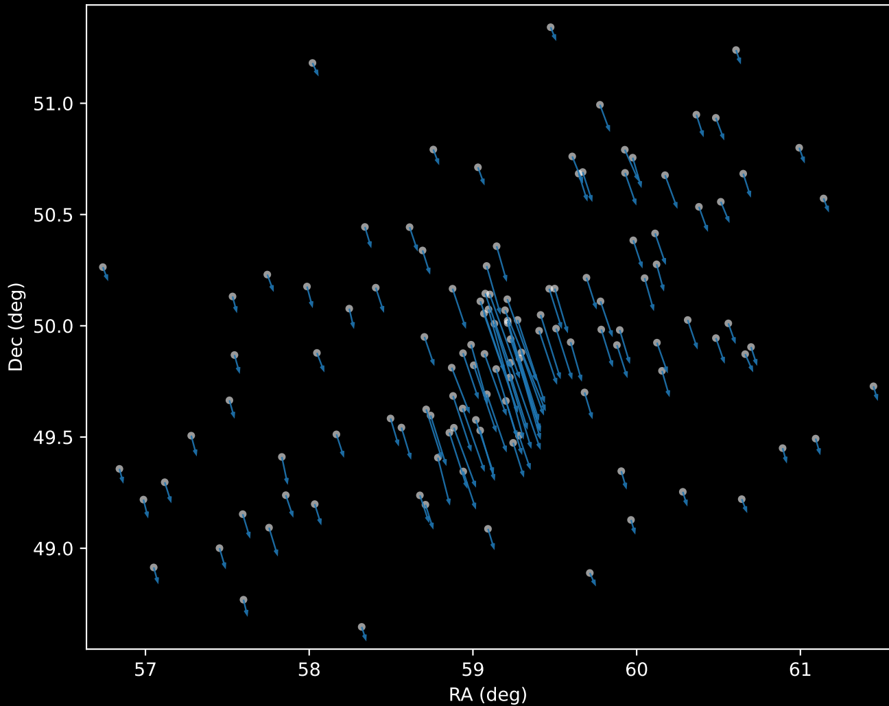
Gaia DR3 Cluster 0 Proper Motion Vectors (n=122)
