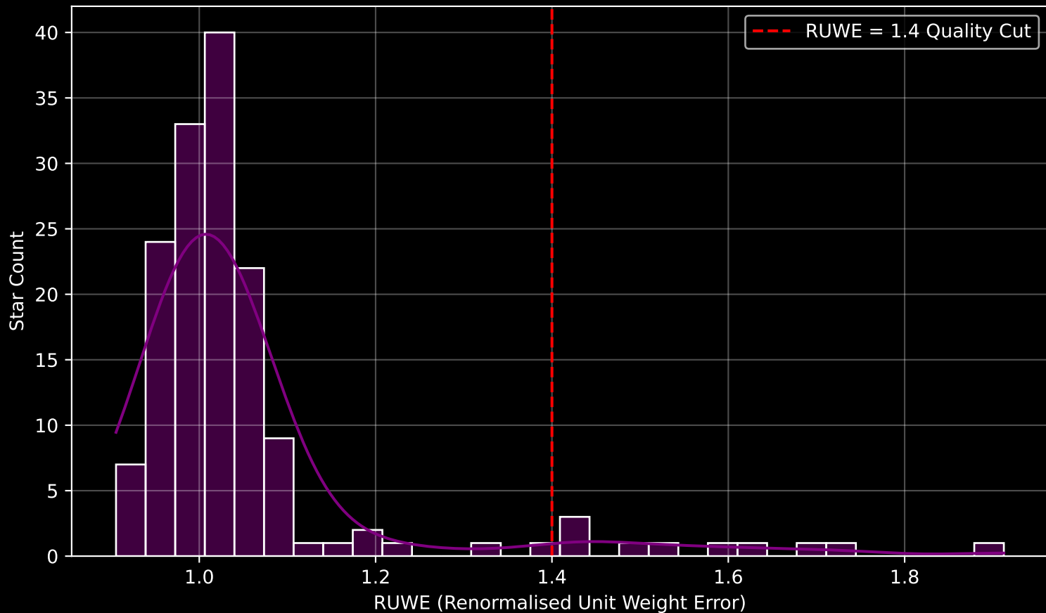
Gaia Cluster: [UPK_143] RUWE Distribution (n= 152)
