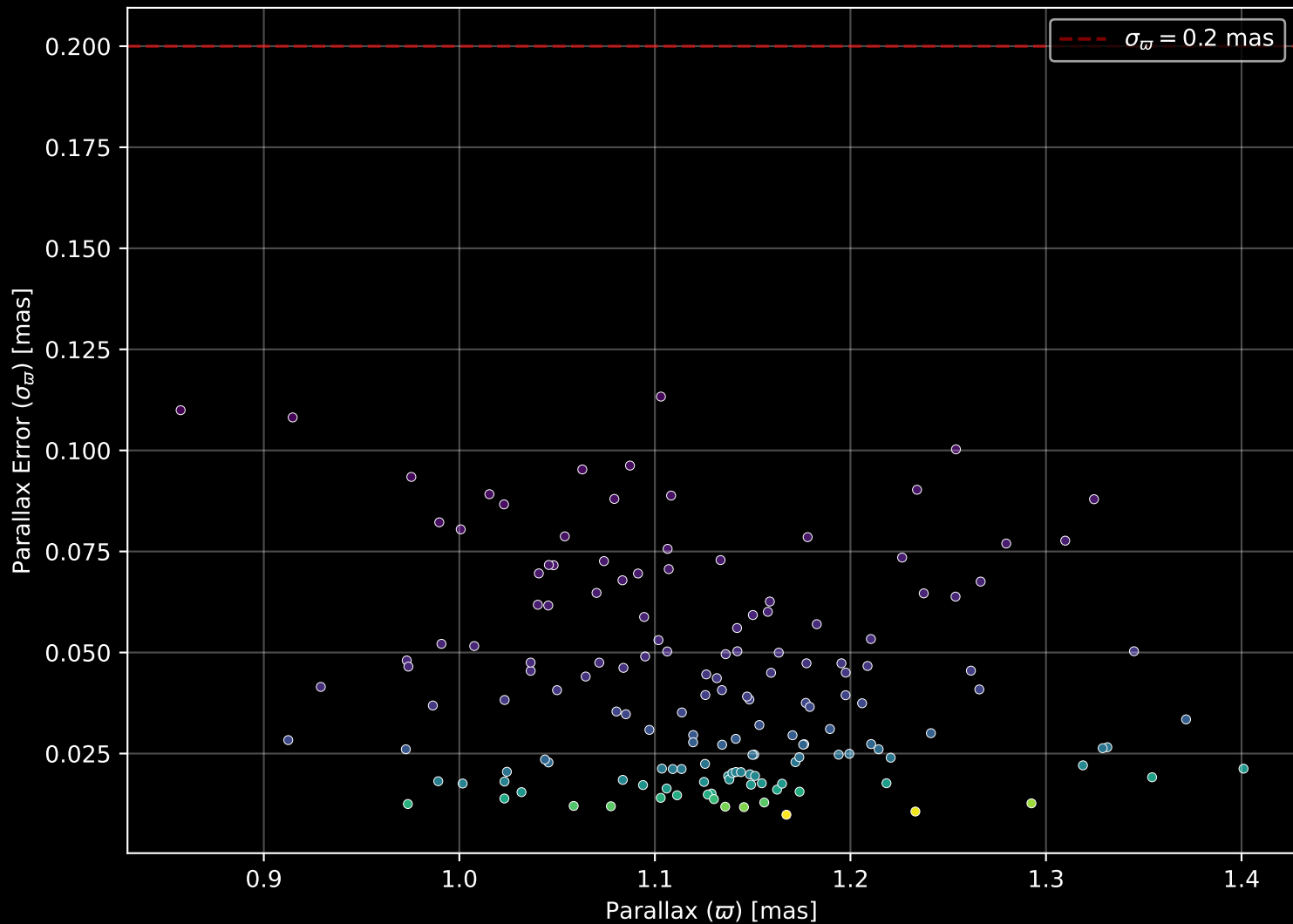
Gaia Cluster: [UPK_143] Parallax Quality (n= 153)
