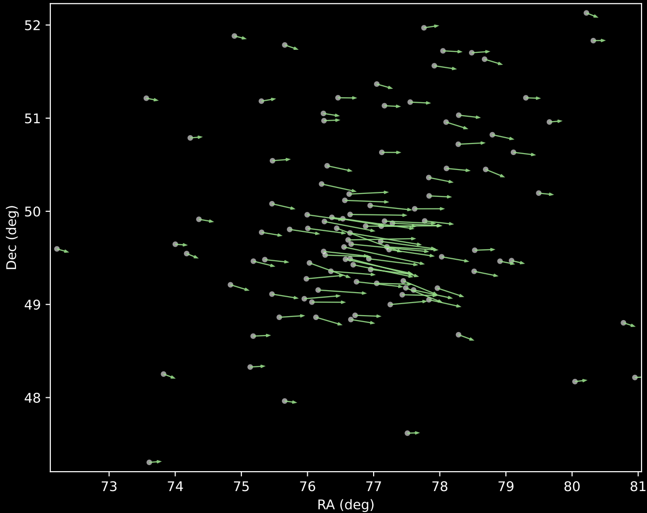
Gaia DR3 Cluster 5 Proper Motion Vectors (n=109)
