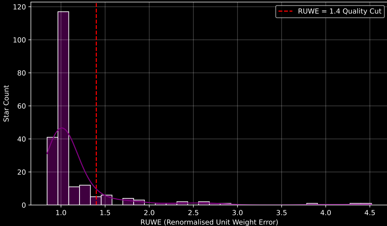
Gaia Cluster: [UPK_167] RUWE Distribution (n= 210)
