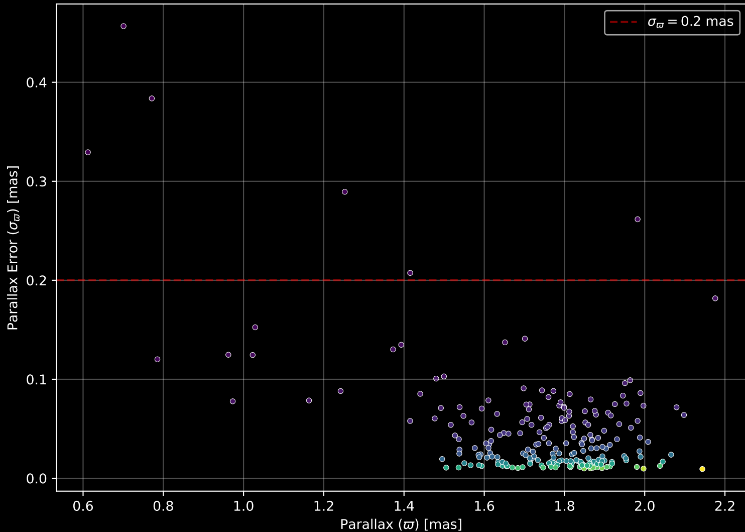
Gaia Cluster: [UPK_167] Parallax Quality (n= 221)
