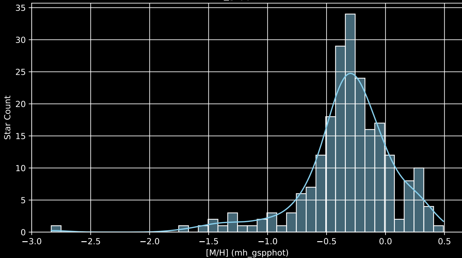
Gaia Cluster: [UPK_167 [M/H] (mh_gspphot) (n= 220)
