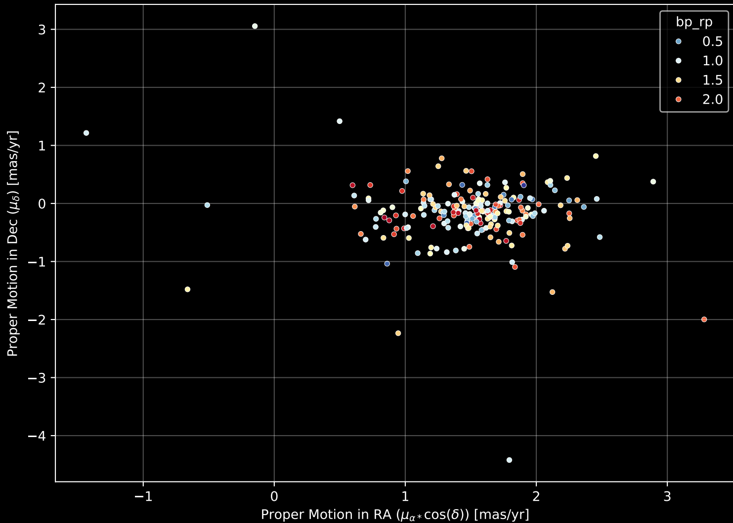
Gaia Cluster: [UPK_167] Proper Motion Diagram (n= 221)
