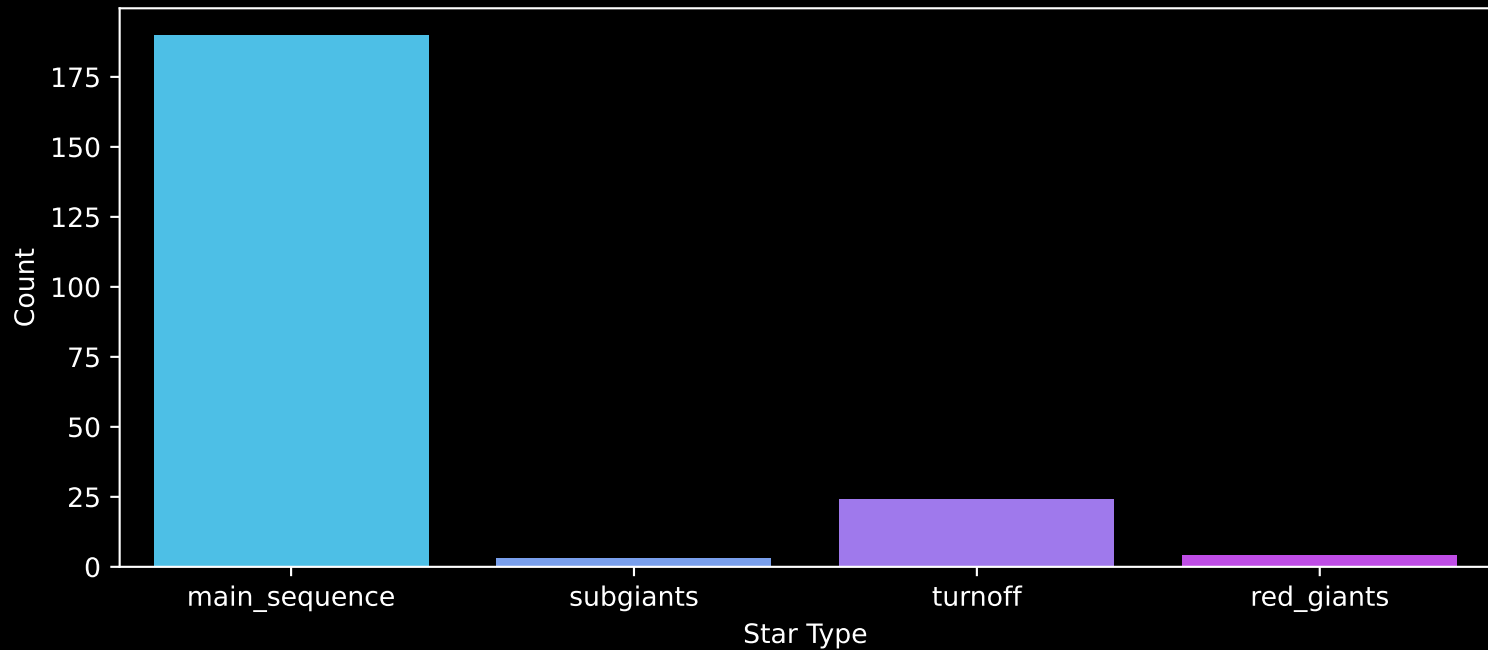
Gaia Cluster: [UPK_167] Count plot of Star Type
