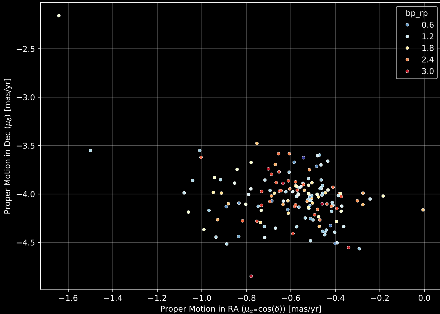
Gaia Cluster: [UPK_168] Proper Motion Diagram (n= 156)
