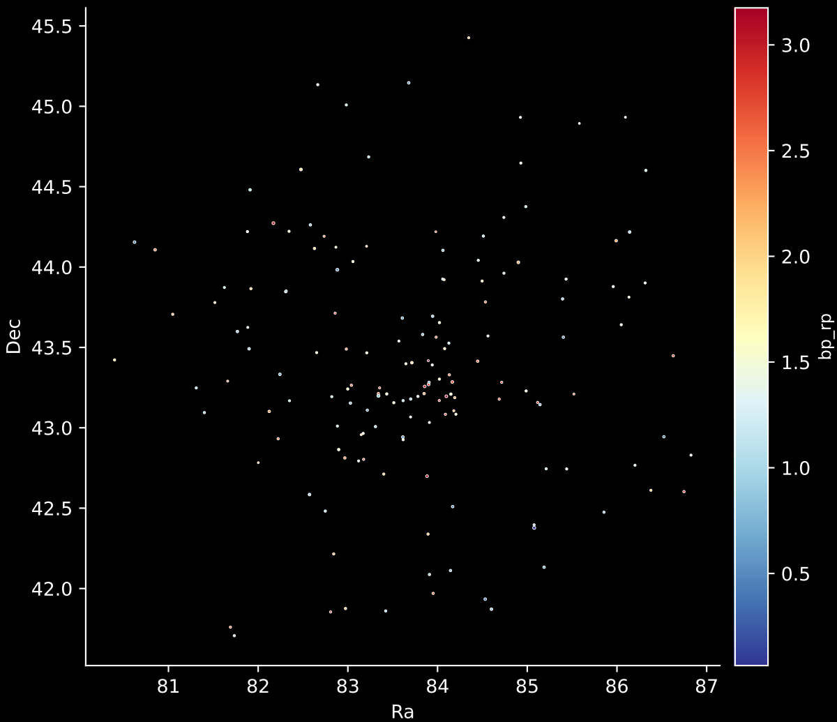
Gaia Cluster: [UPK_168] Stars: 156
