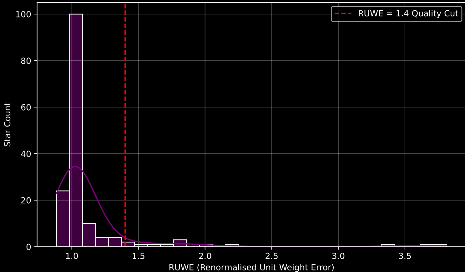
Gaia Cluster: [UPK_168] RUWE Distribution (n= 155)
