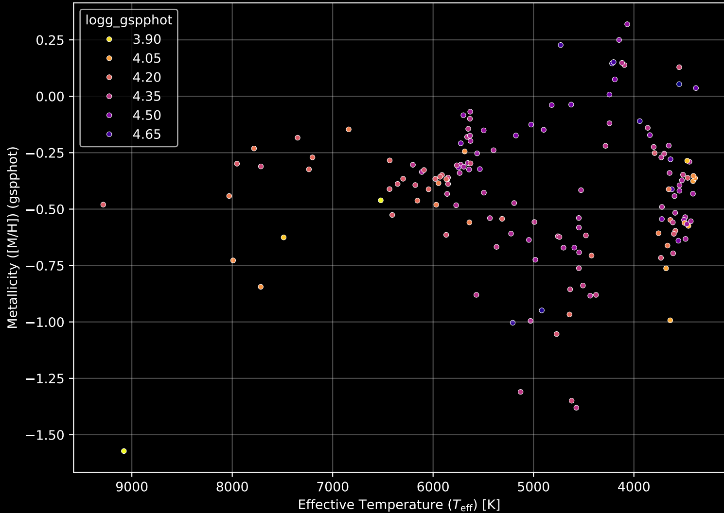
Gaia Cluster: [UPK_168] Stellar Population Parameters (n= 156)
