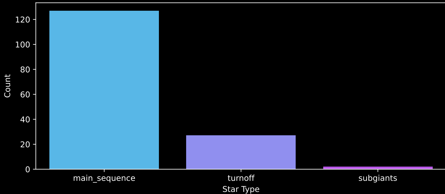
Gaia Cluster: [UPK_168] Count plot of Star Type
