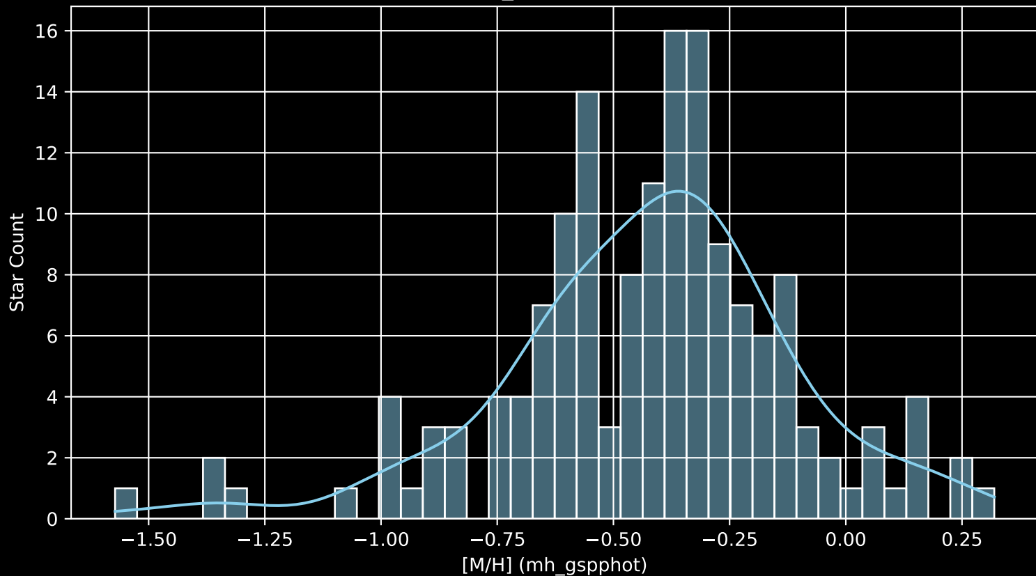
Gaia Cluster: [UPK_168 [M/H] (mh_gspphot) (n= 156)
