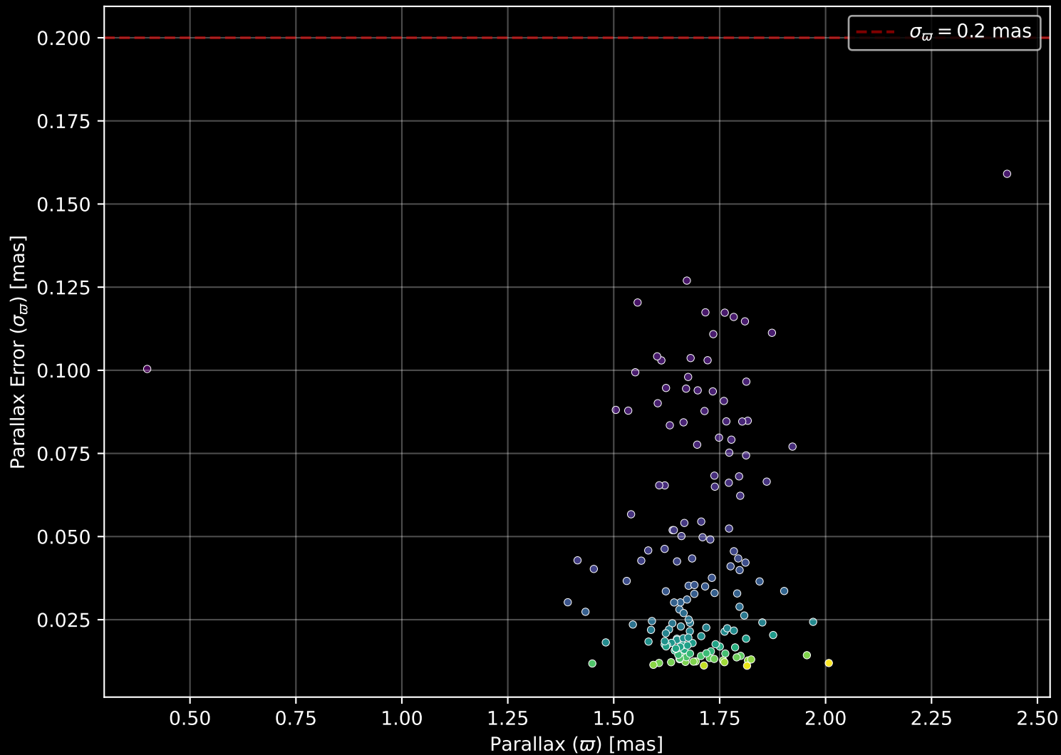
Gaia Cluster: [UPK_168] Parallax Quality (n= 156)
