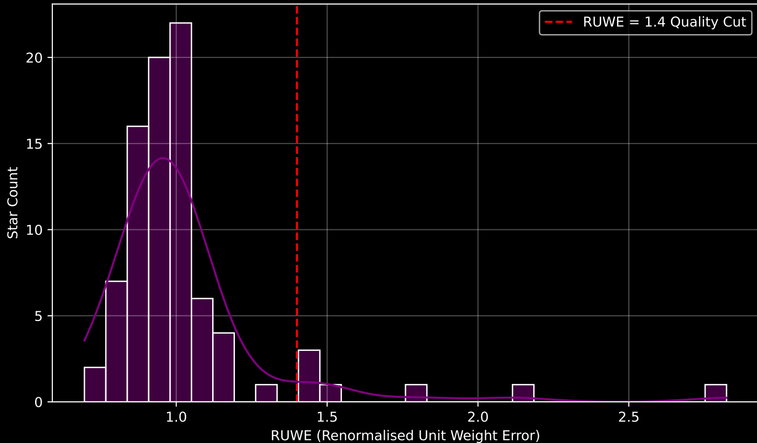
Gaia Cluster: [UPK_17] RUWE Distribution (n= 85)
