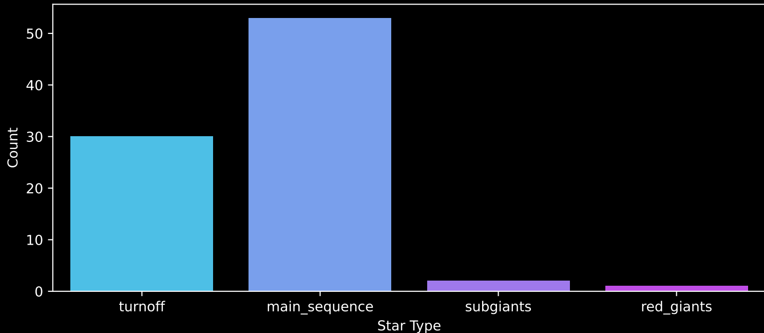
Gaia Cluster: [UPK_17] Count plot of Star Type
