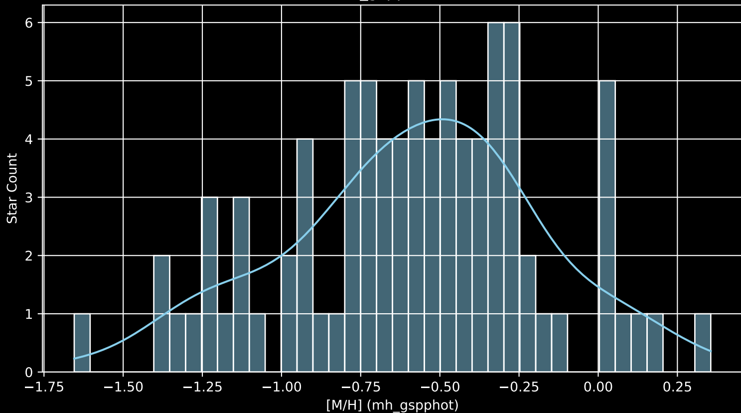
Gaia Cluster: [UPK_17 [M/H] (mh_gspphot) ( \bar{n}= 86 )
