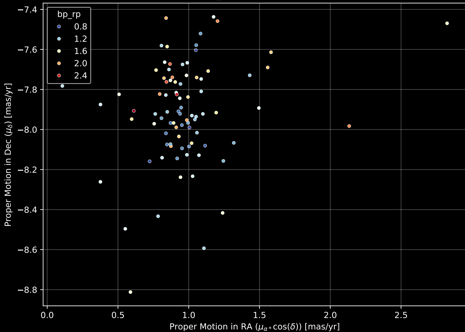
Gaia Cluster: [UPK_17] Proper Motion Diagram (n= 86)
