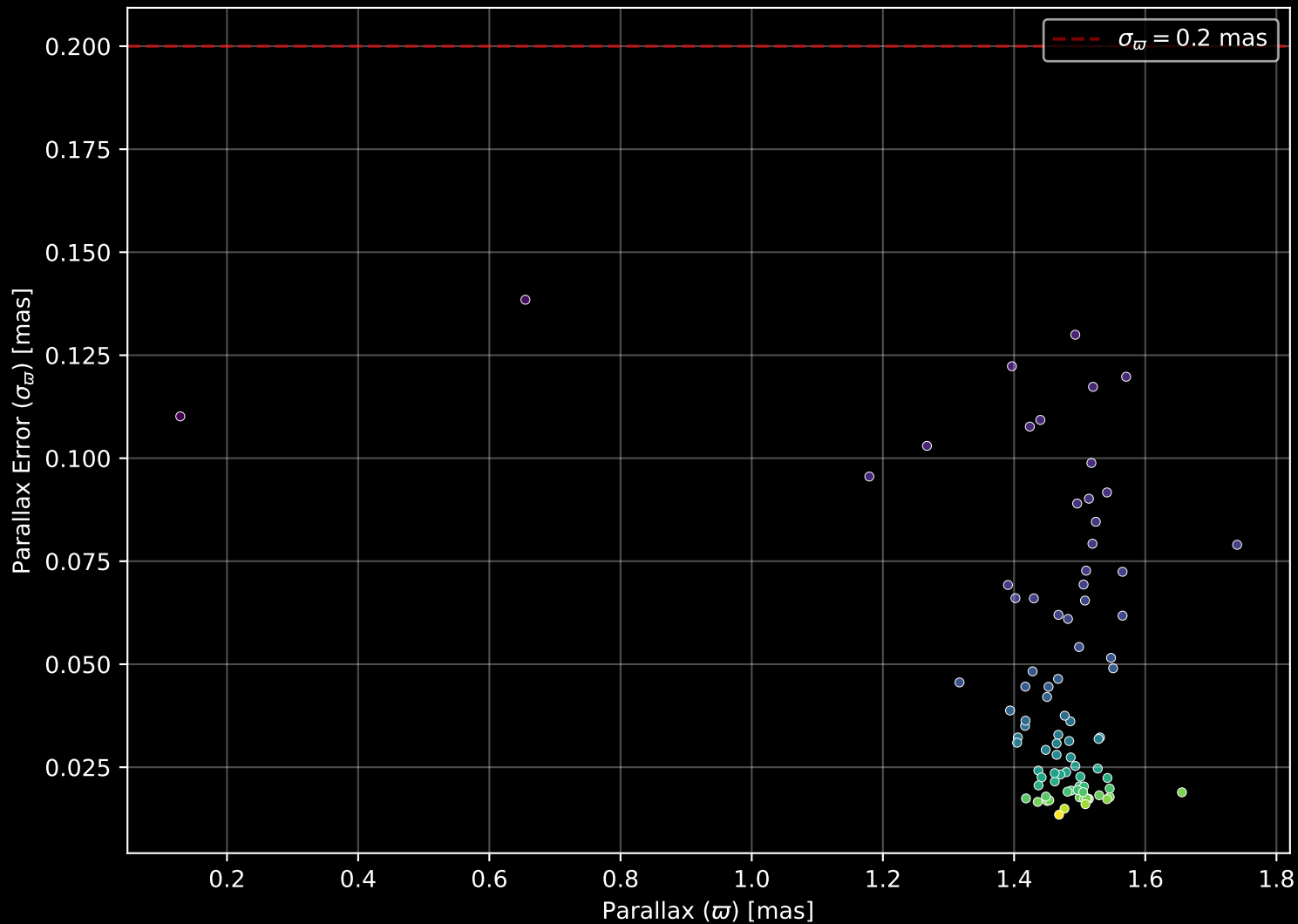
Gaia Cluster: [UPK_17] Parallax Quality (n= 86)
