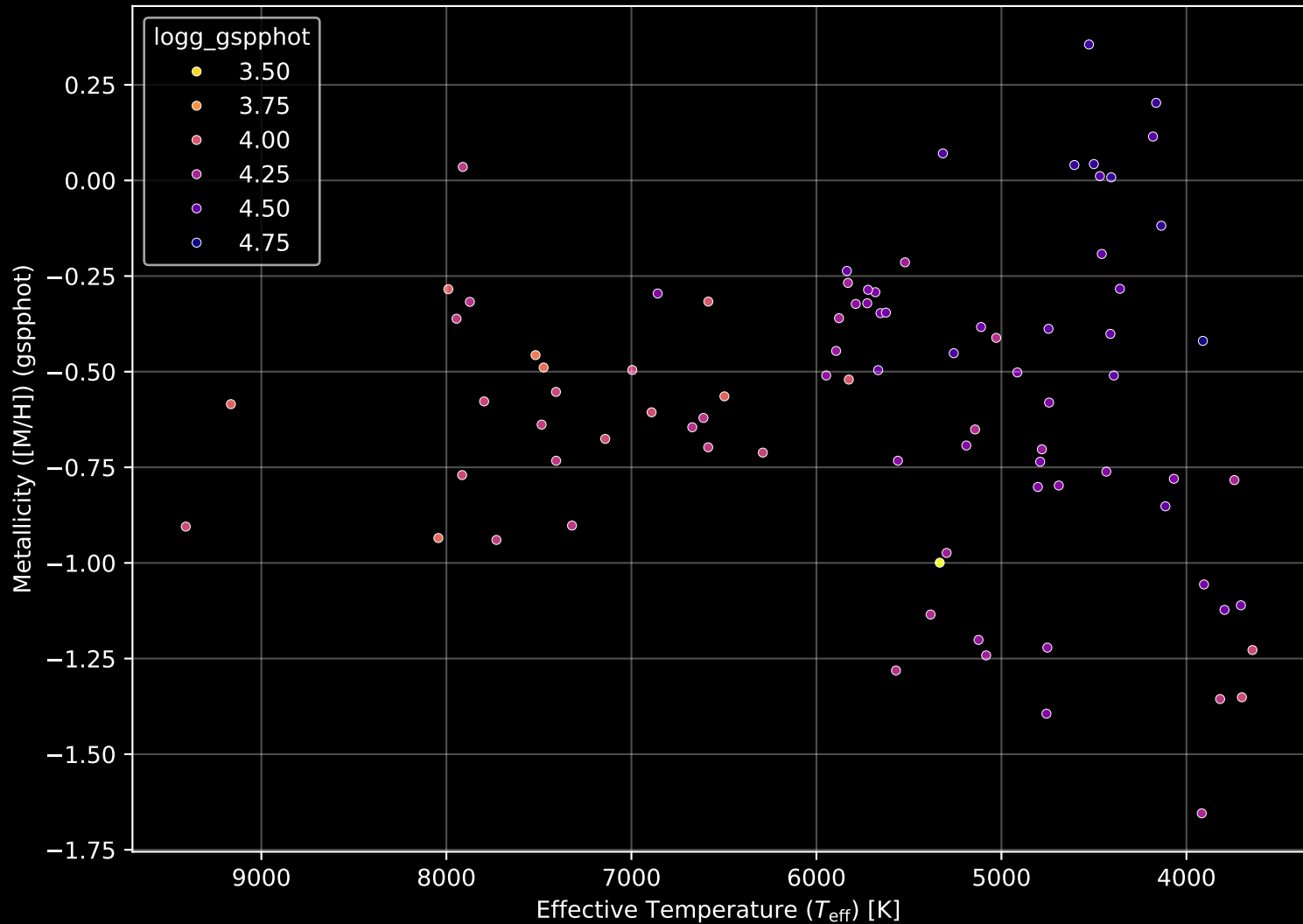
Gaia Cluster: [UPK_17] Stellar Population Parameters (n= 86)
