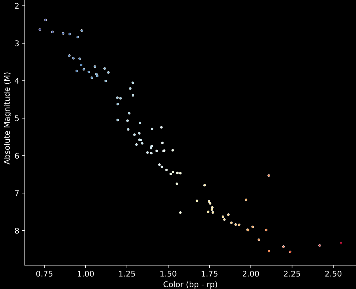
Gaia Cluster: [UPK_17] Stars (n = 86) Hertzsprung-Russel Diagram
