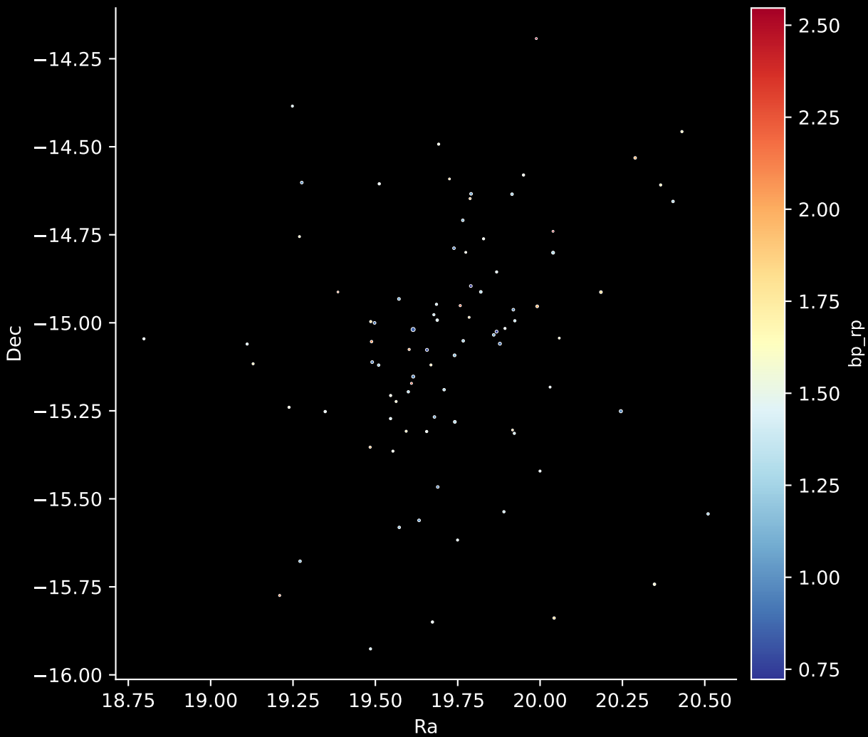
Gaia Cluster: [UPK_17] Stars: 86
