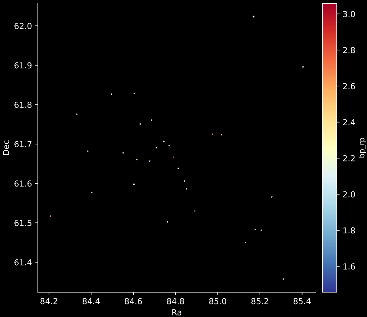
Gaia Cluster: [UPK_201] Stars: 30
