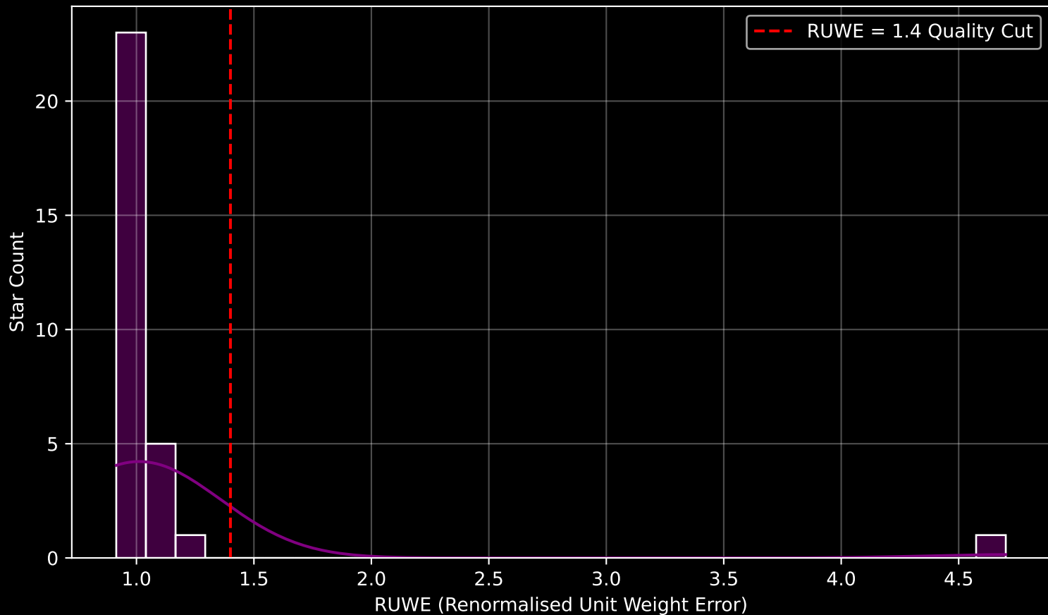
Gaia Cluster: [UPK_201] RUWE Distribution (n= 30)
