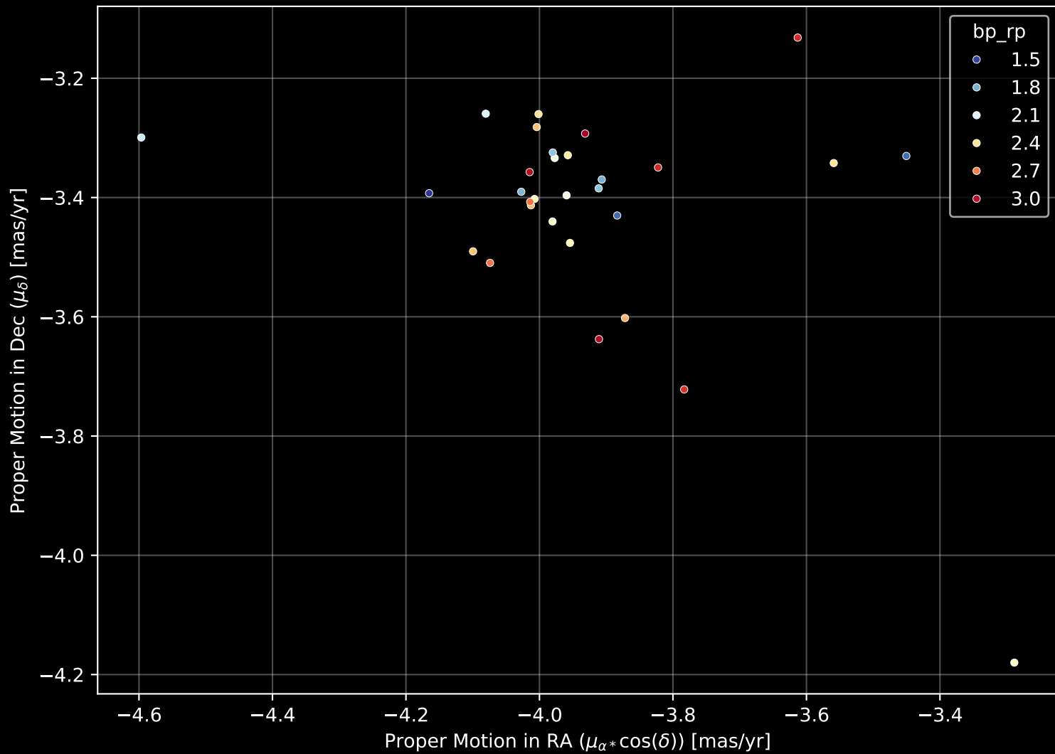
Gaia Cluster: [UPK_201] Proper Motion Diagram (n= 30)
