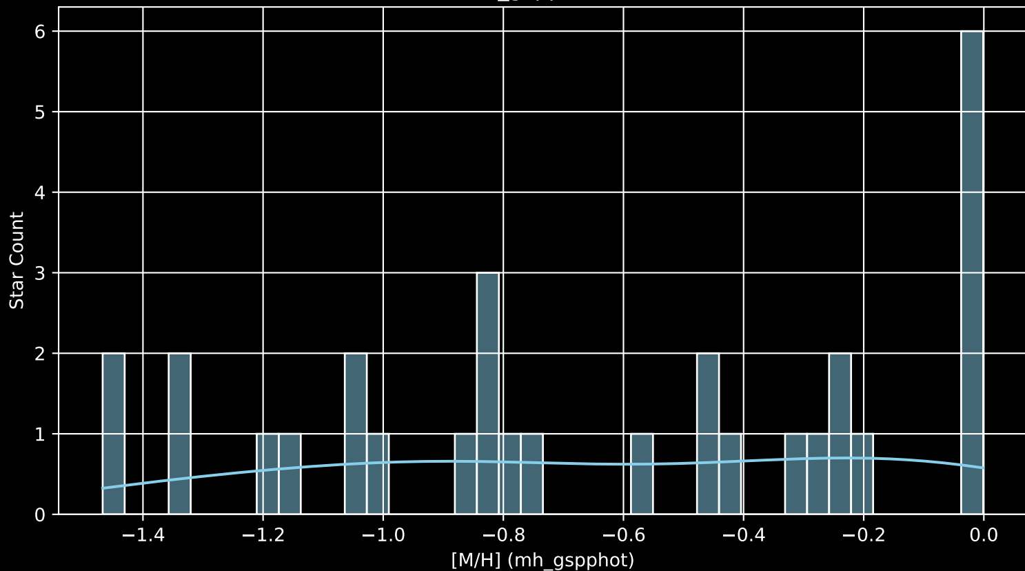
Gaia Cluster: [UPK_201 [M/H] (mh_gspphot) (n= 30)
