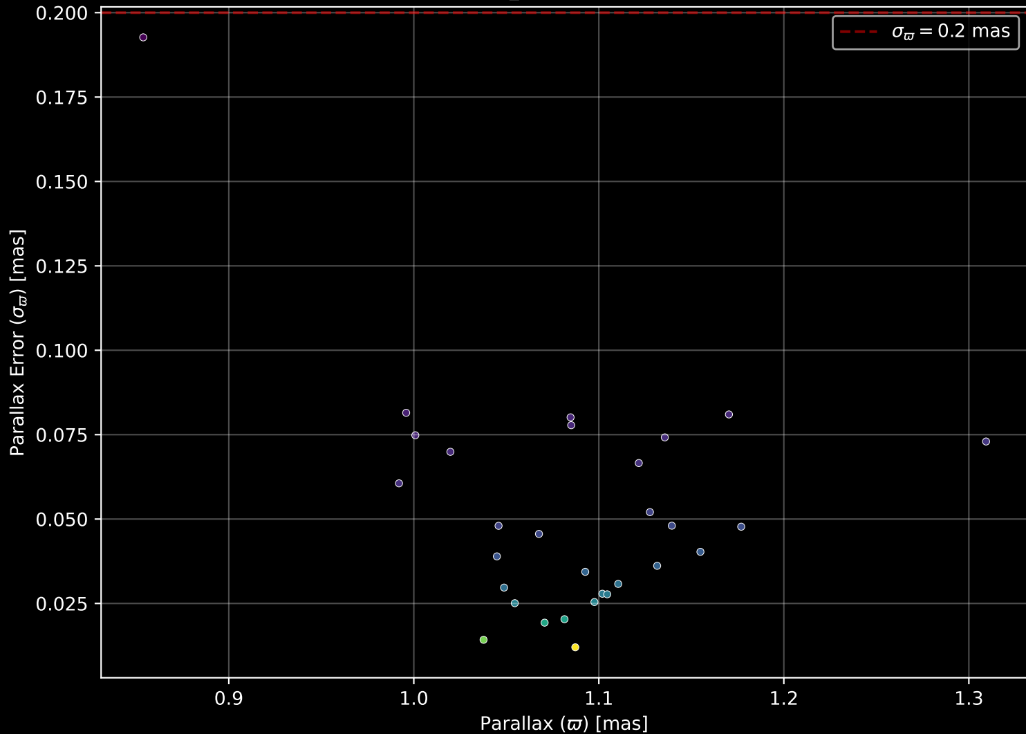
Gaia Cluster: [UPK_201] Parallax Quality (n= 30)
