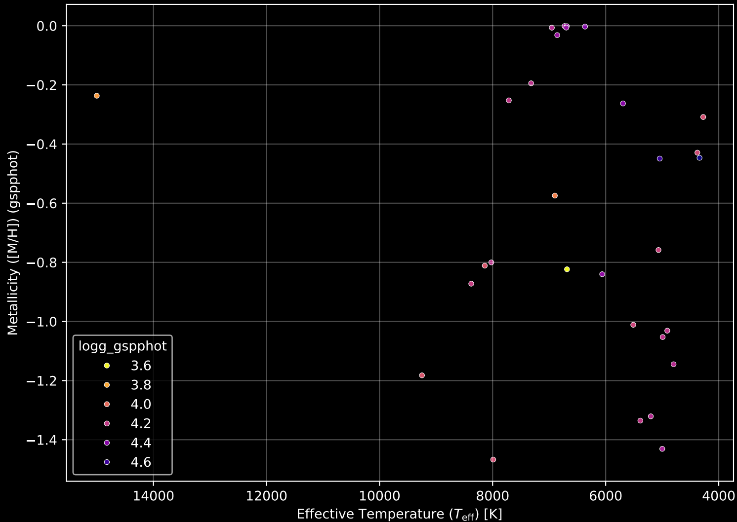
Gaia Cluster: [UPK_201] Stellar Population Parameters (n= 30)
