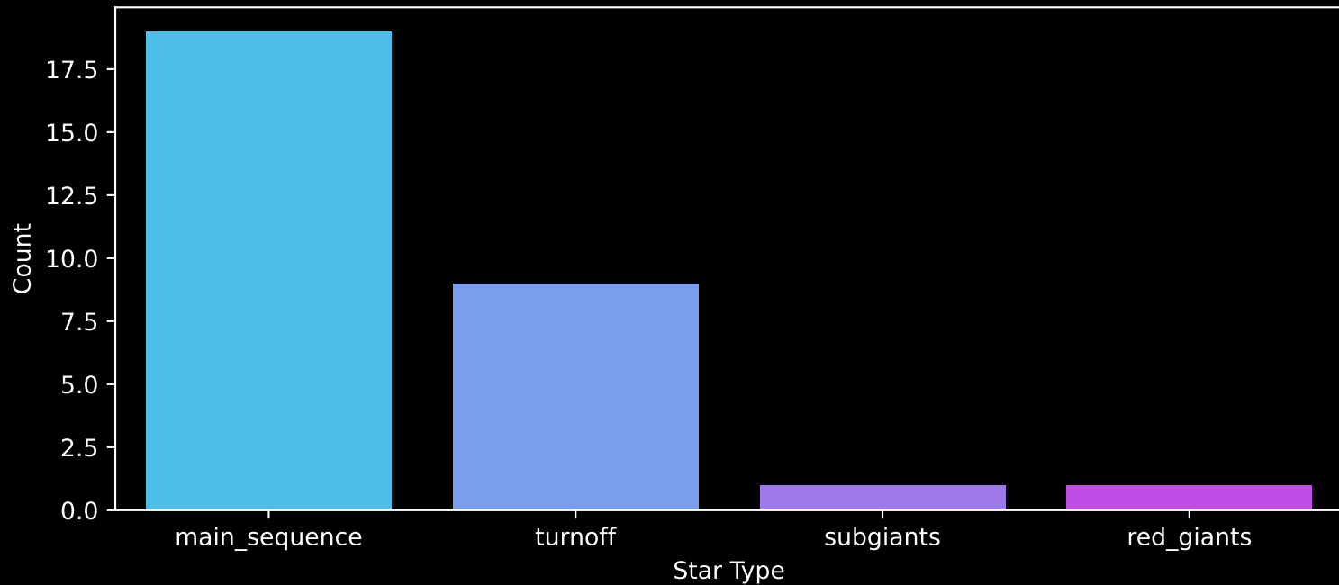
Gaia Cluster: [UPK_201] Count plot of Star Type
